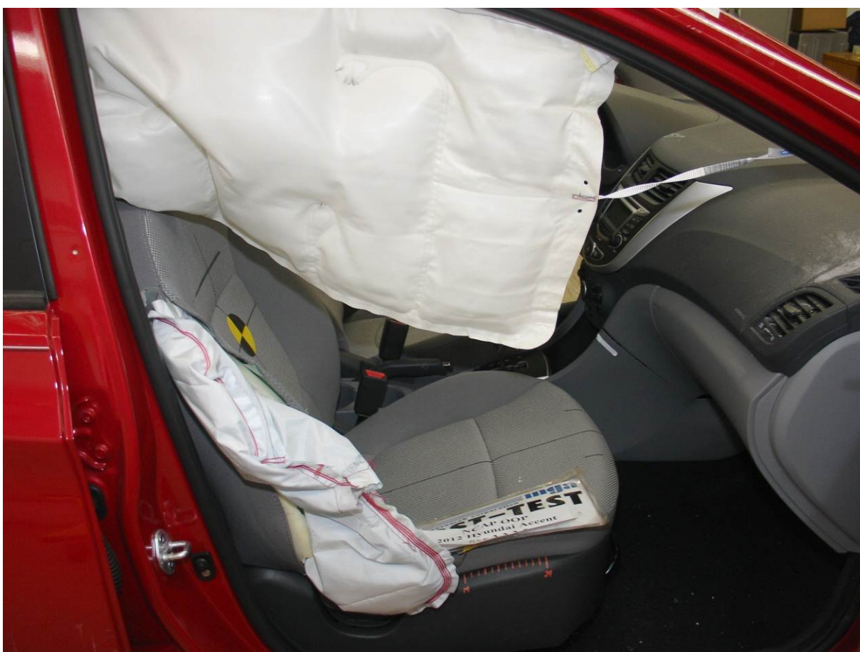
Post-Test Curtain Airbag Right Side View With Door Open
