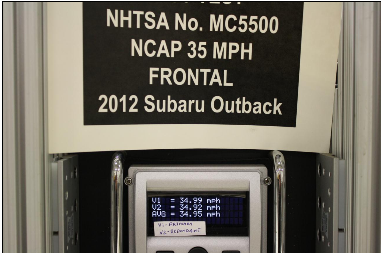
Figure A-65: Post-Test Speed Trap Read-Out
