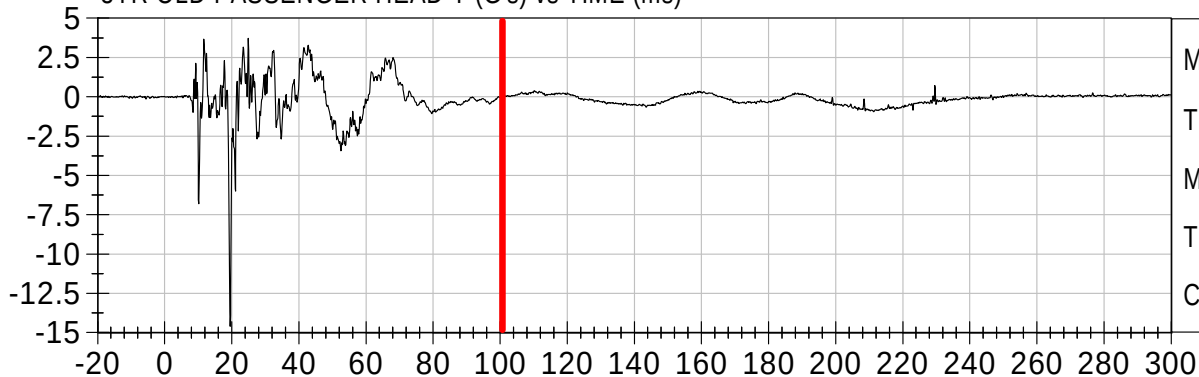
3YR OLD PASSENGER HEAD Z (G's) vs TIME (ms)
