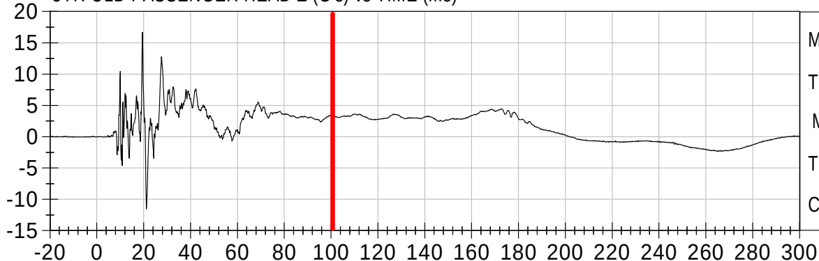
3YR OLD PASSENGER HEAD Resultant (G's) vs TIME (ms)
