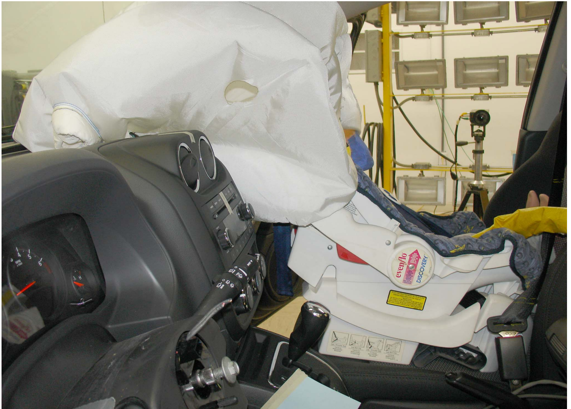
Post-Test 12 Mo Pass. Dummy Airbag Left Side View
