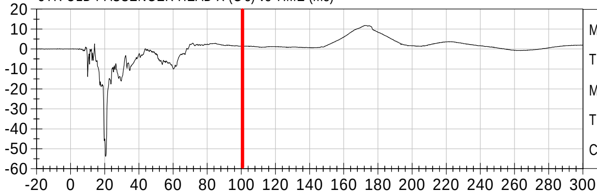
3YR OLD PASSENGER HEAD Y (G's) vs TIME (ms)
