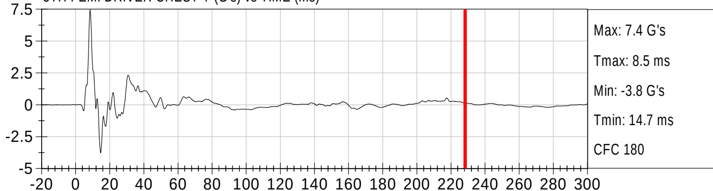
5TH FEM. DRIVER CHEST Z (G's) vs TIME (ms)
