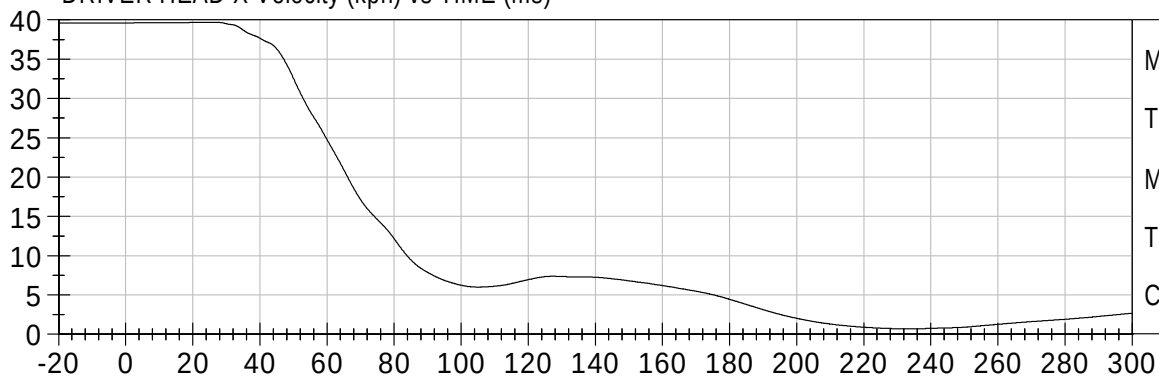
DRIVER HEAD Y Velocity (kph) vs TIME (ms)
