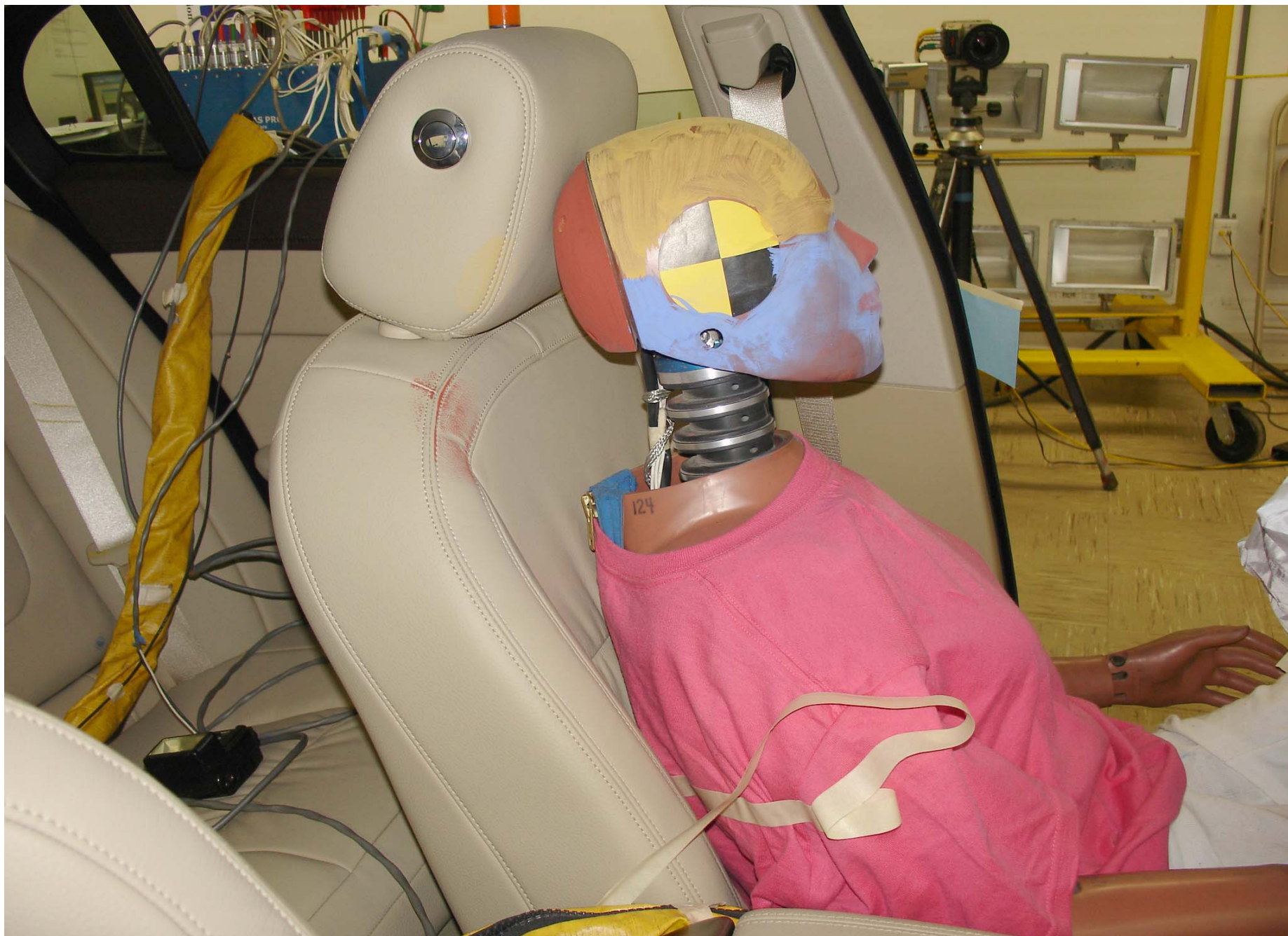
Post-Test 5th Fem. P1 Driver Dummy Head Contact (headrest)
