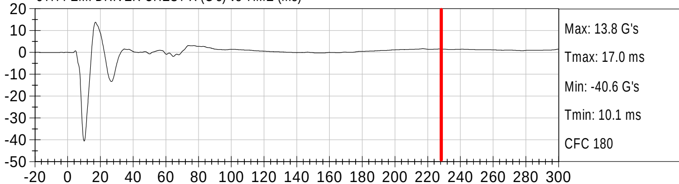
5TH FEM. DRIVER CHEST Y (G's) vs TIME (ms)
