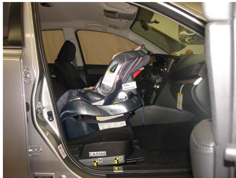
Graco Snugride WBase, Unbelted, Rear Facing, Rearward Seat Track
