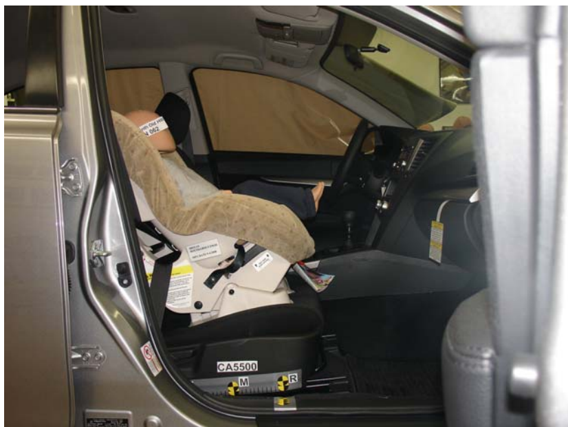
Britax Roundabout Forward Facing Belted, Rearward Seat Track
