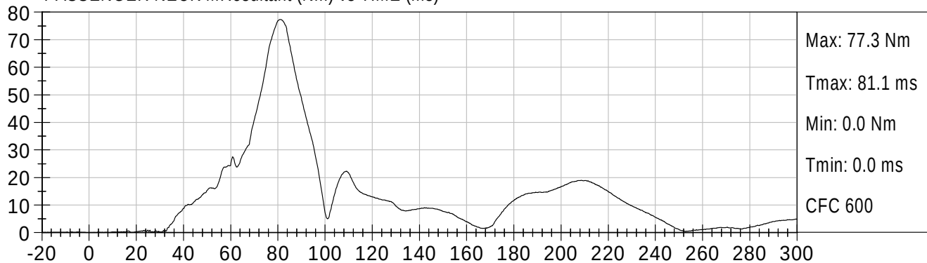
PASSENGER NECK MResultant (Nm) vs TIME (ms)
