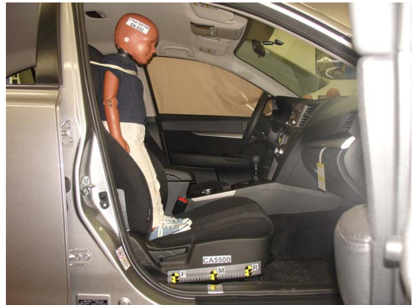
3-Year-Old Unbelted, Middle Seat Track, Position 5
