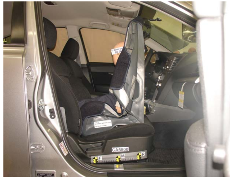
Cosco High Back Booster Rear Facing Unbelted, Middle Seat Track
