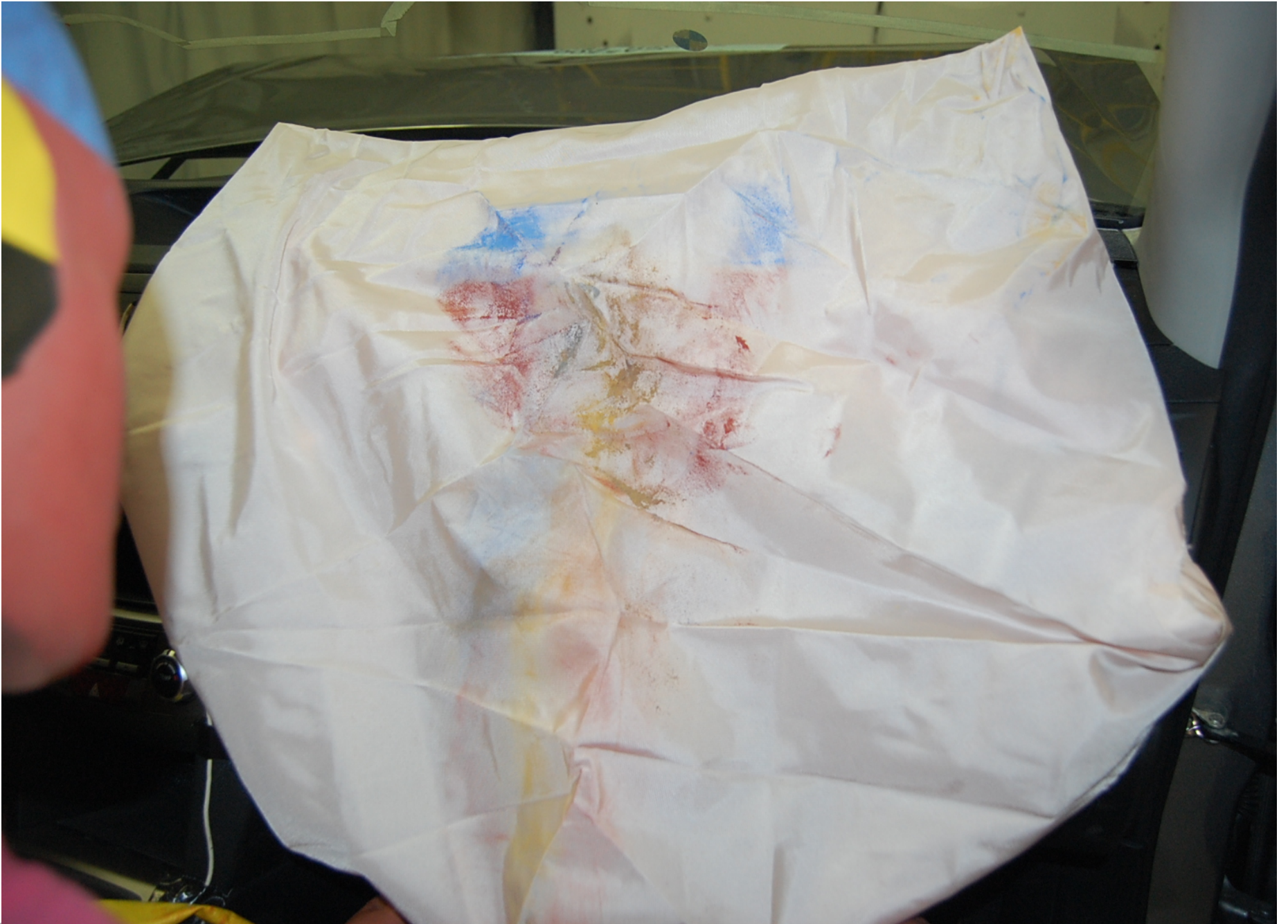
Post-Test Passenger Dummy Airbag Contact View
