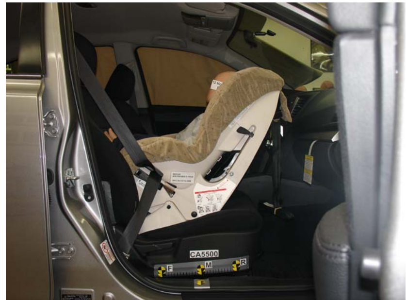
Britax Roundabout Rear Facing Belted, Middle Seat Track
