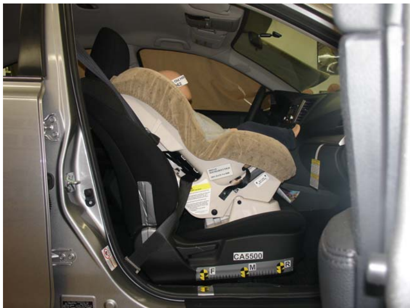
Britax Roundabout Forward Facing Belted, Forward Seat Track
