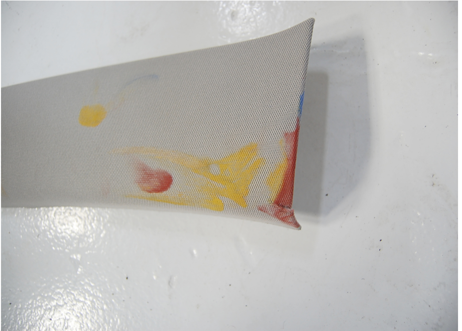
Post-Test Passenger Dummy Head Contact (C-pillar)
