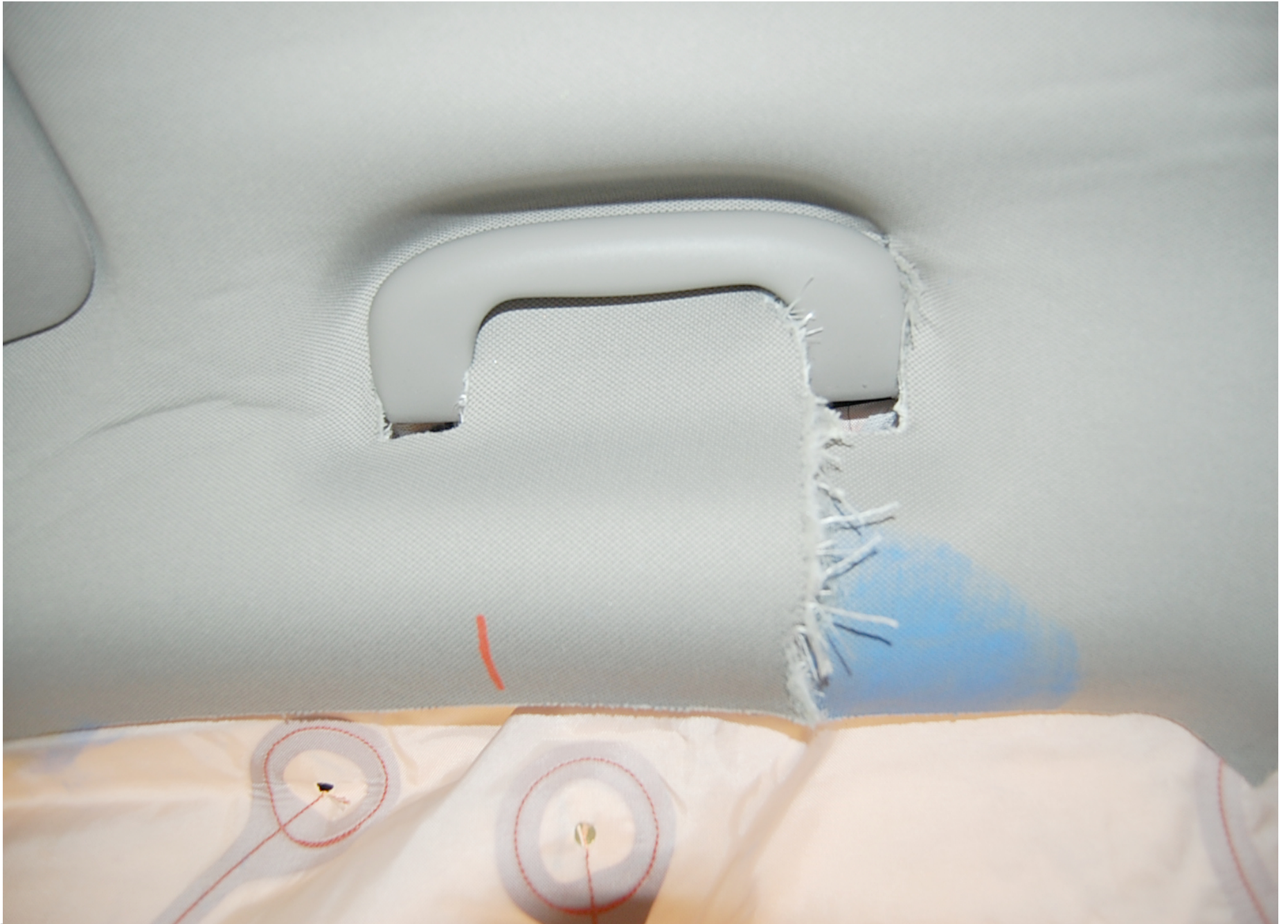
Post-Test Passenger Dummy Head Contact (side header)
