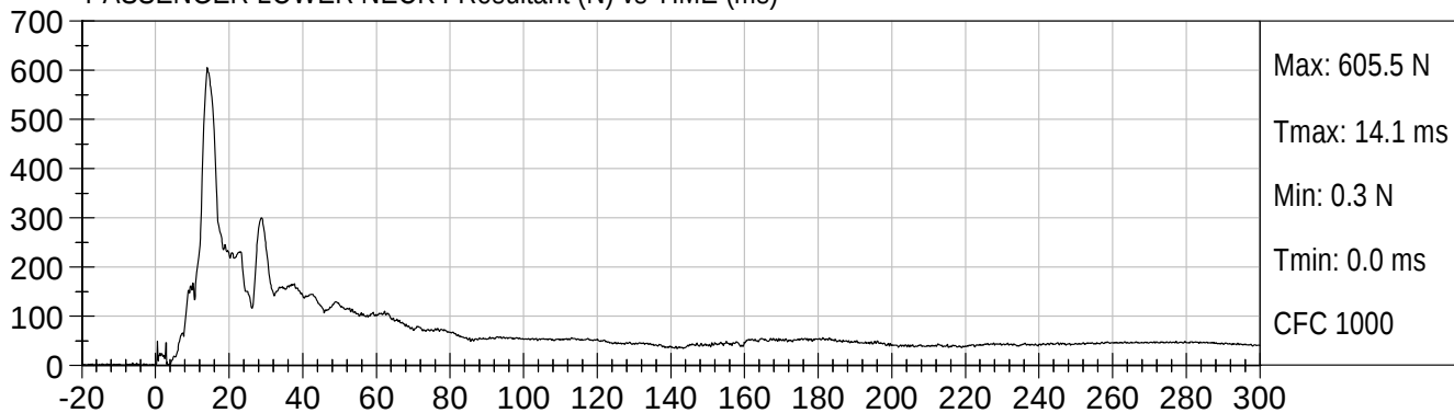
PASSENGER LOWER NECK FResultant (N) vs TIME (ms)
