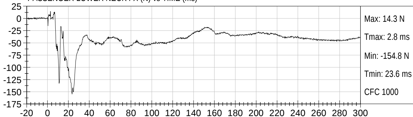
PASSENGER LOWER NECK FY (N) vs TIME (ms)
