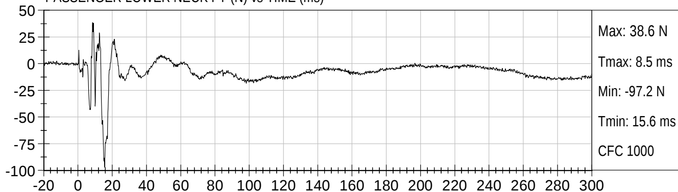
PASSENGER LOWER NECK FZ (N) vs TIME (ms)
