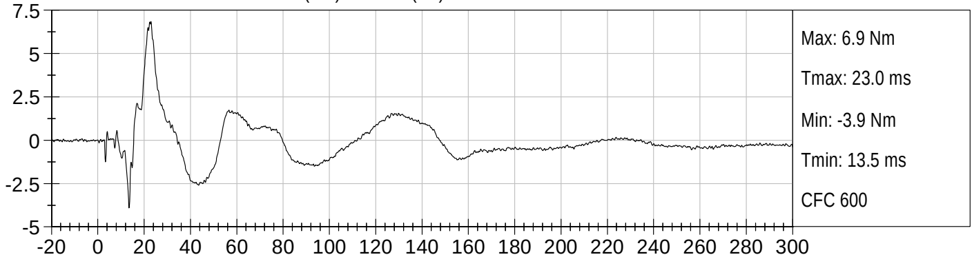
PASSENGER UPPER NECK MX (Nm) vs TIME (ms)
