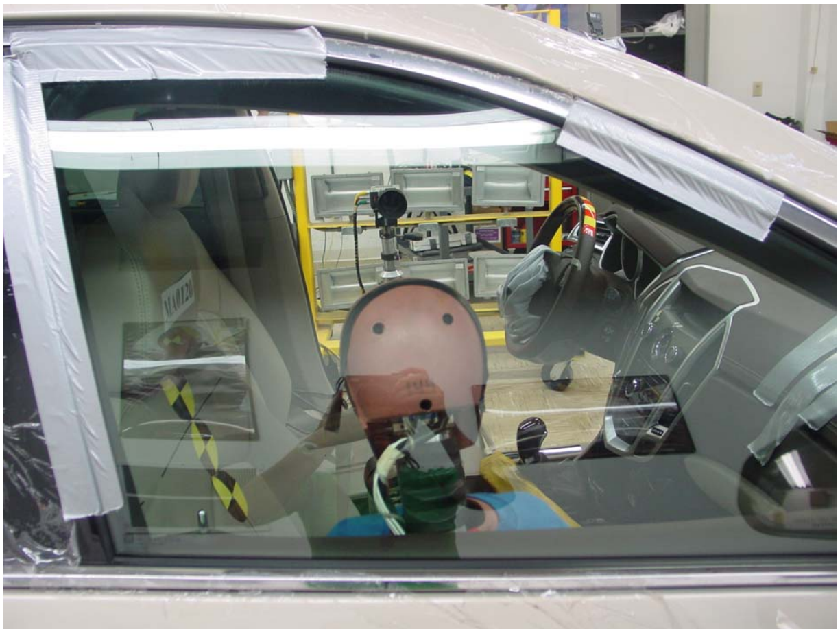
Pre-Test 6-Year-Old Child Dummy Right Side View
