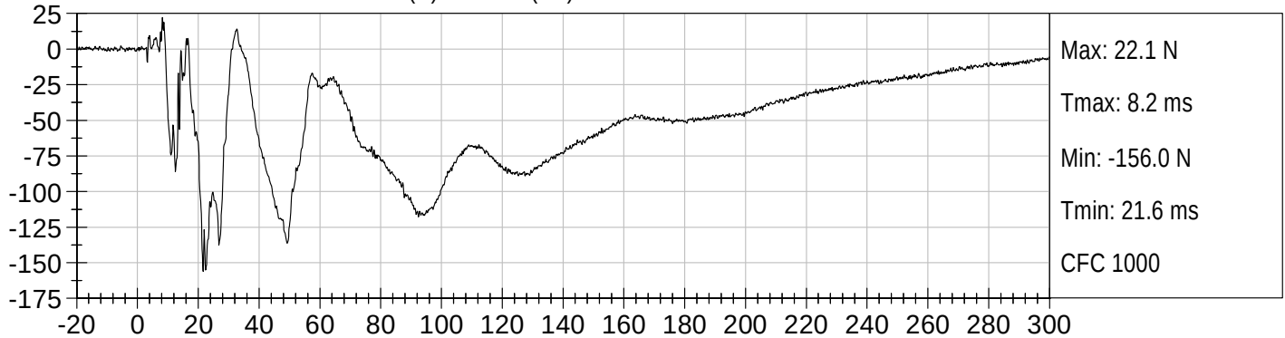
PASSENGER LOWER NECK FX (N) vs TIME (ms)
