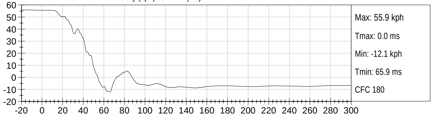
RIGHT BRAKE CALIPER X (G's) vs TIME (ms)
