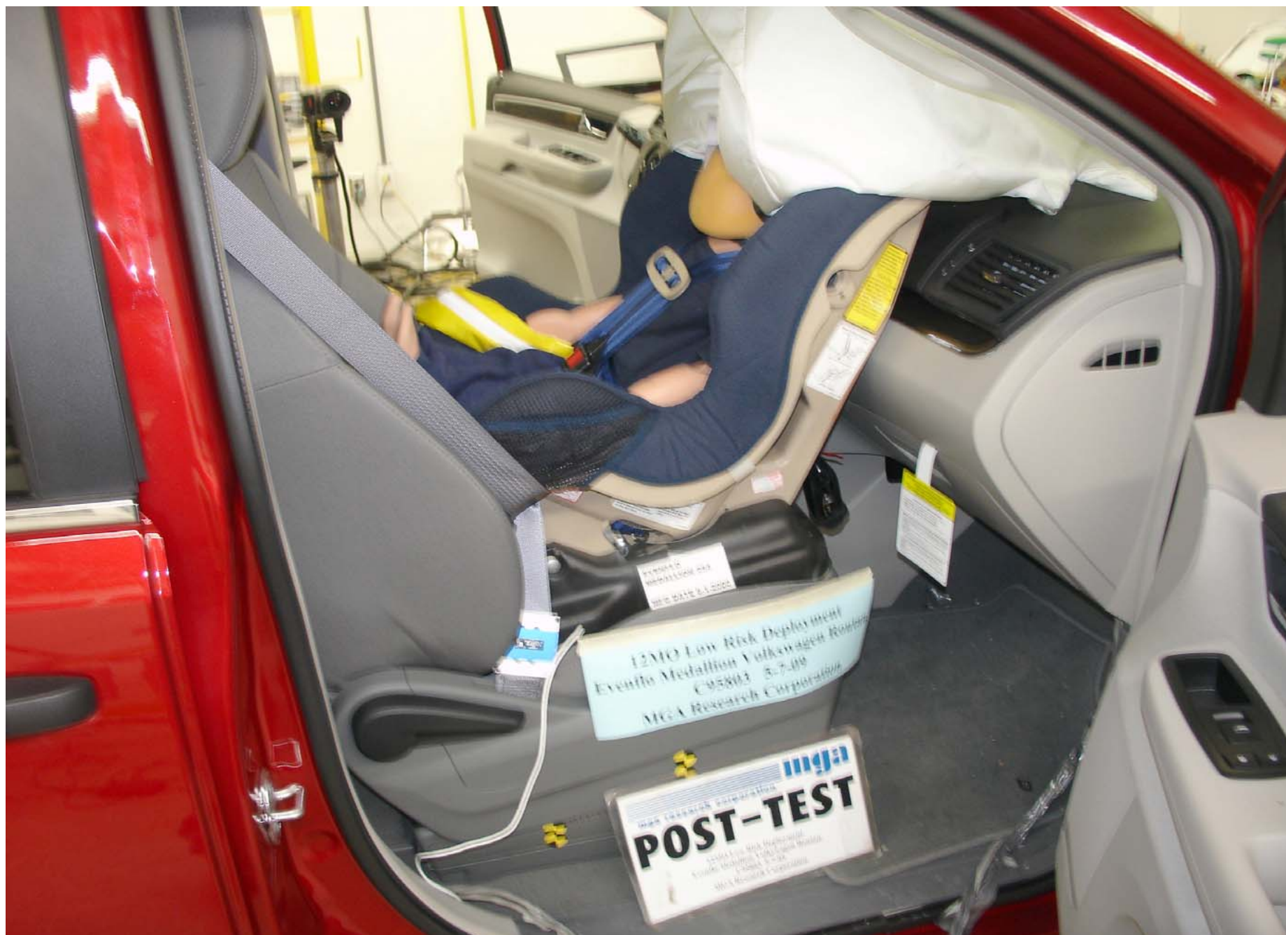
Post-Test 12 Mo Pass. Dummy Right Side View (Eventflo Medallion)
