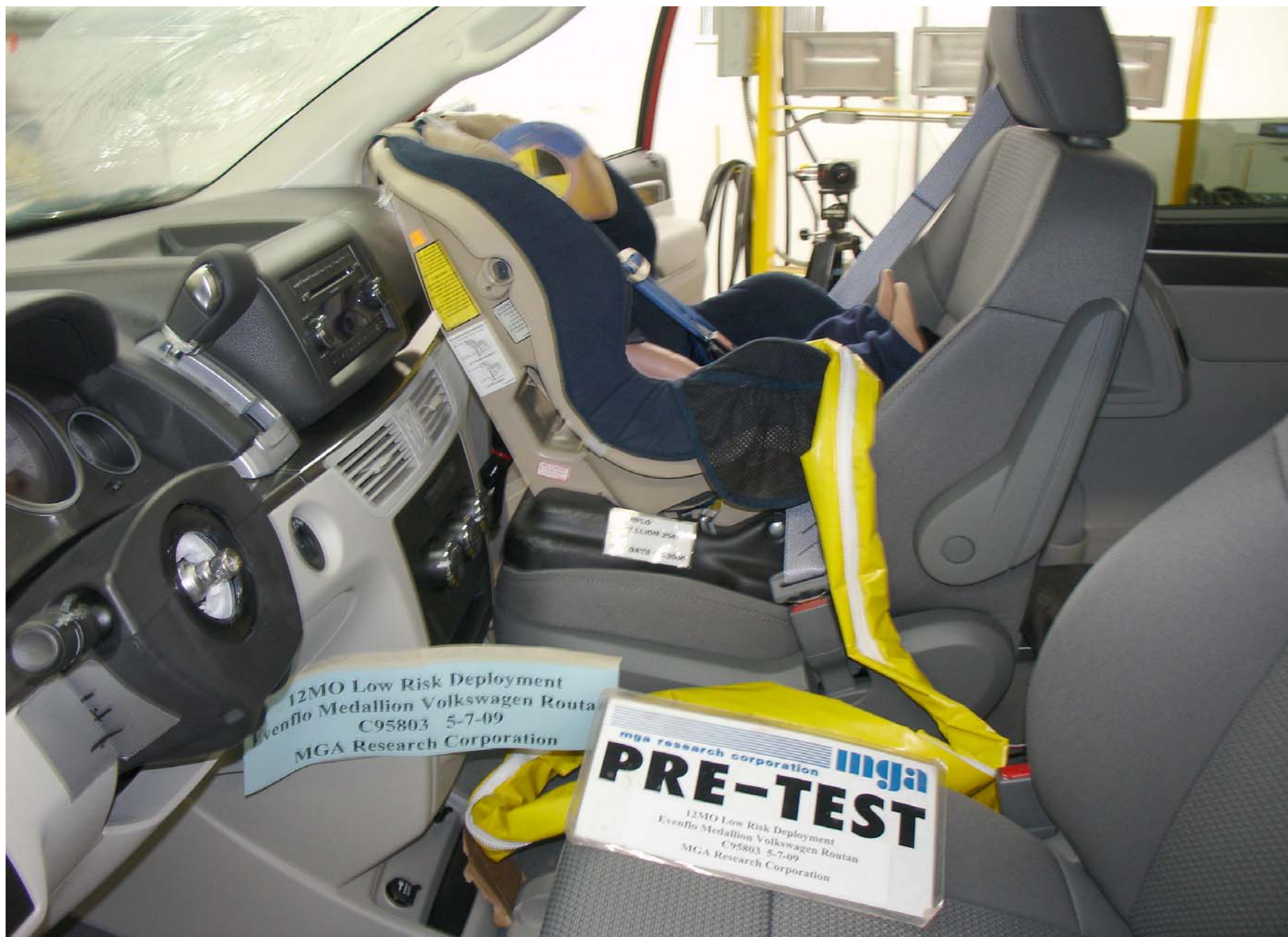
Pre-Test 12 Mo Pass. Dummy Left Side View (Evenflo Medallion)
