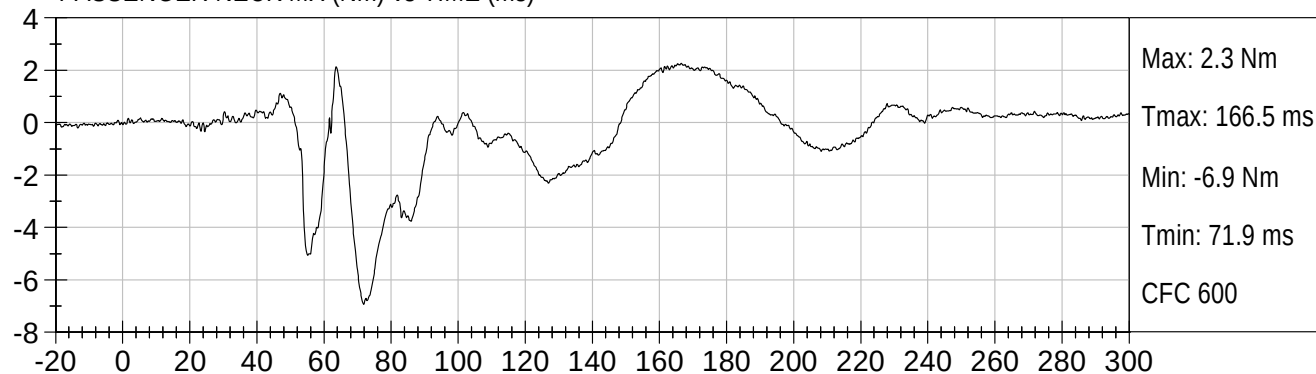
PASSENGER NECK MY (Nm) vs TIME (ms)
