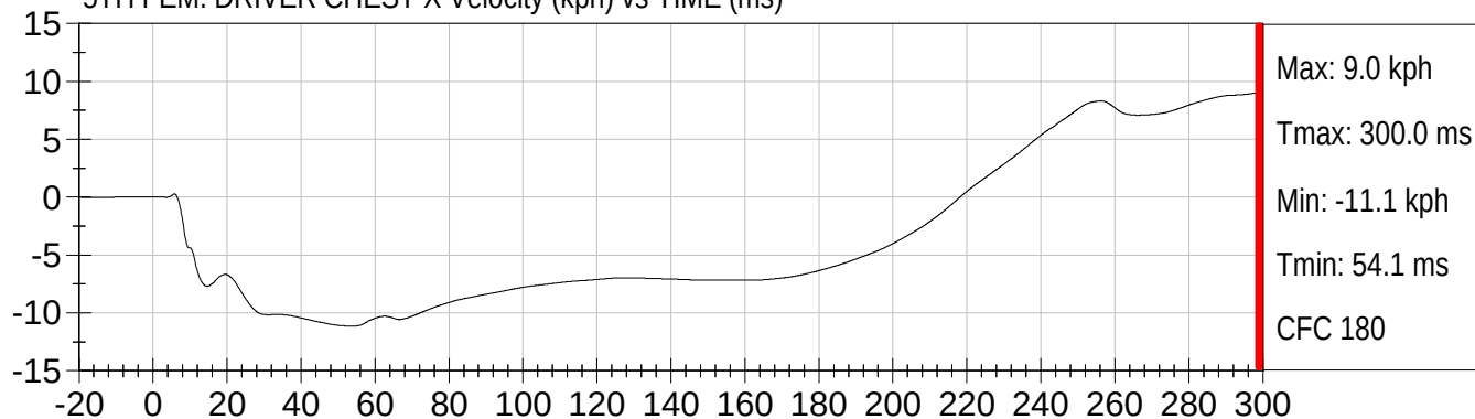
5TH FEM. DRIVER CHEST Y Velocity (kph) vs TIME (ms)
