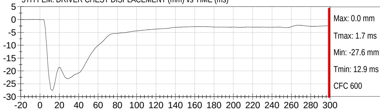
5TH FEM. DRIVER CHEST DISPLACEMENT (mm) vs TIME (ms)
