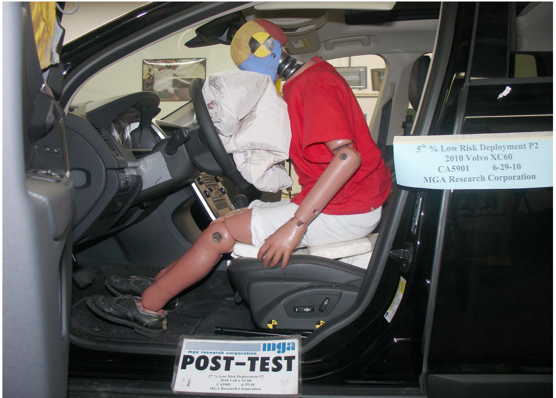
Post-Test 5th Fem. P2 Driver Dummy Left Side View
