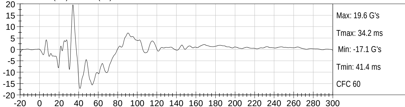
TRUNK Z (G's) vs TIME (ms)
