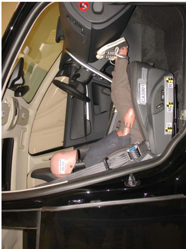
6-Year-Old Unbelted, Forward Seat Track, Position 2
