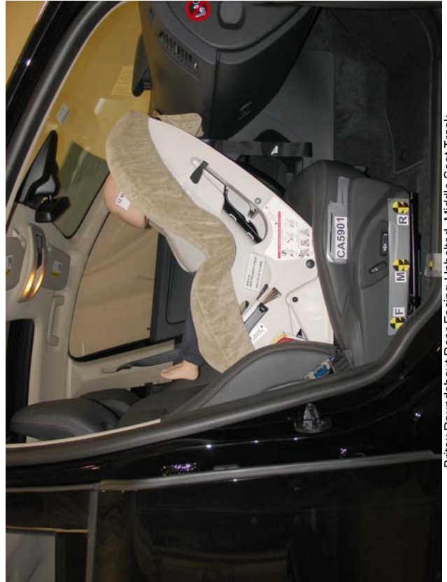
Britax Roundabout Rear Facing Unbelted, Middle Seat Track
