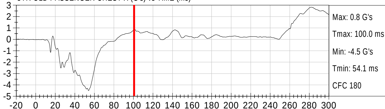
3YR OLD PASSENGER CHEST Y (G's) vs TIME (ms)
