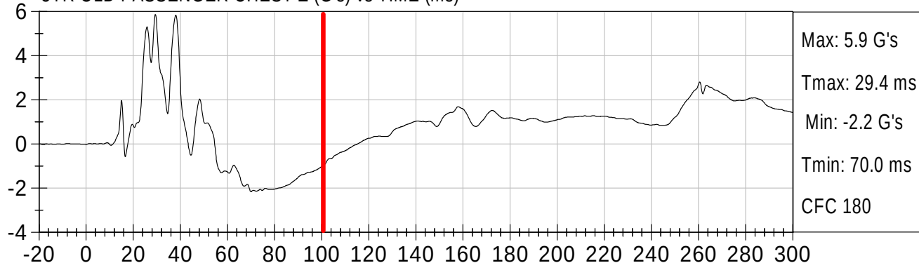
3YR OLD PASSENGER CHEST Resultant (G's) vs TIME (ms)
