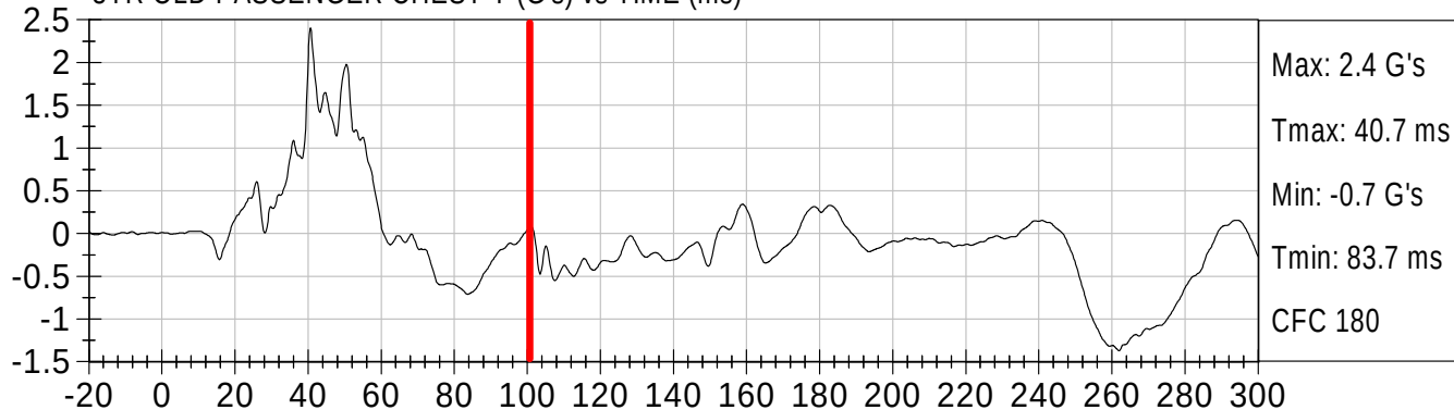
3YR OLD PASSENGER CHEST Z (G's) vs TIME (ms)
