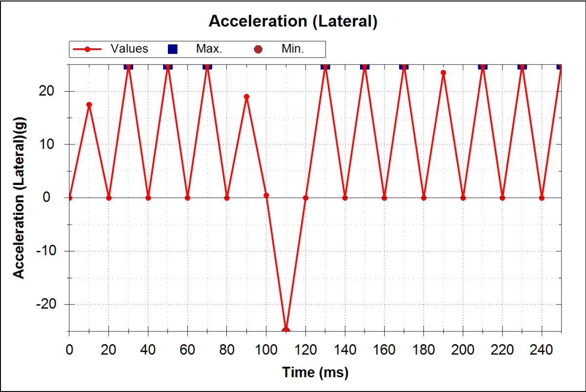
# 2 [ Acceleration (Lateral) ]
