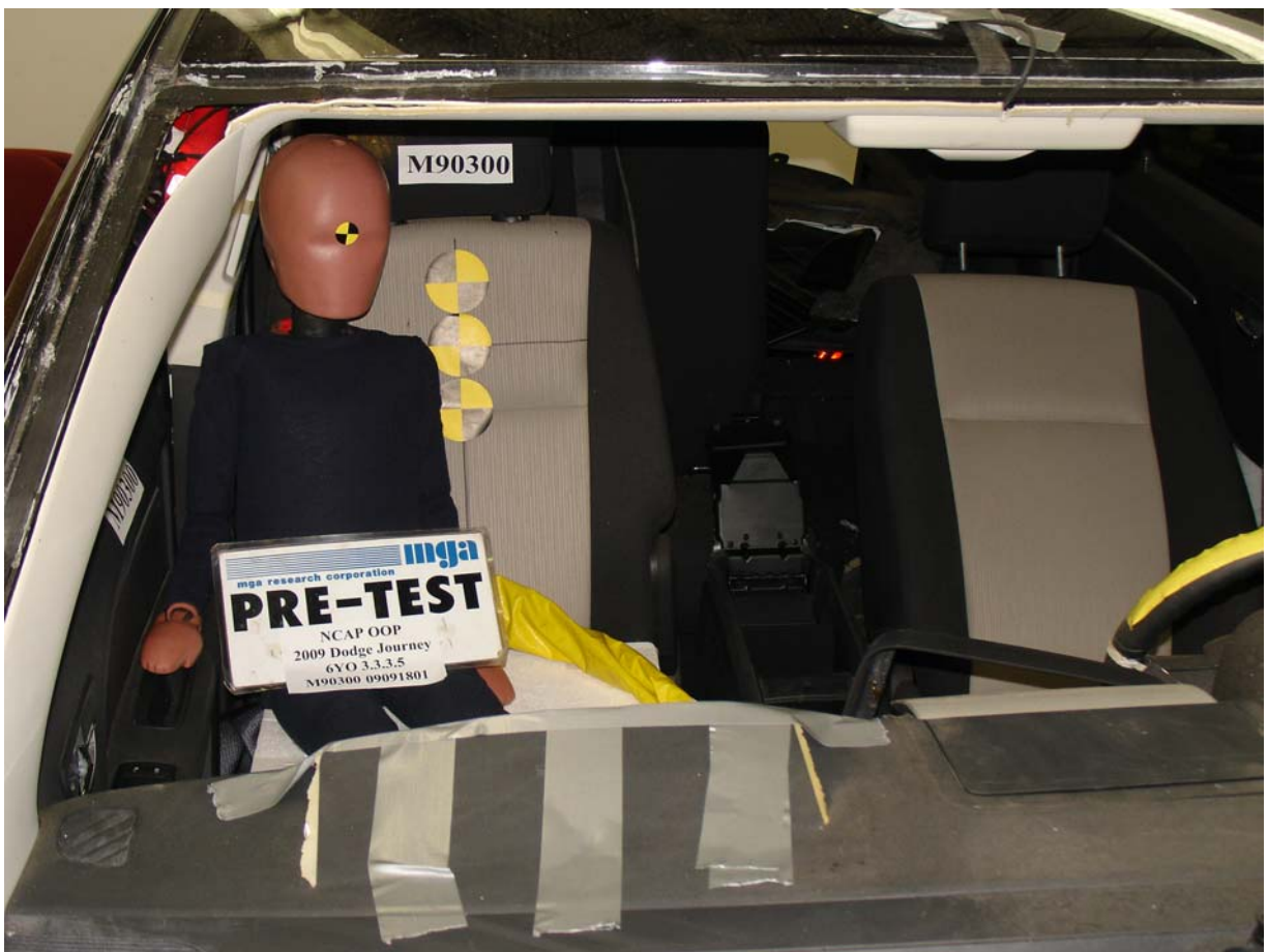
Pre-Test 6-Year-Old Child Dummy Front View
