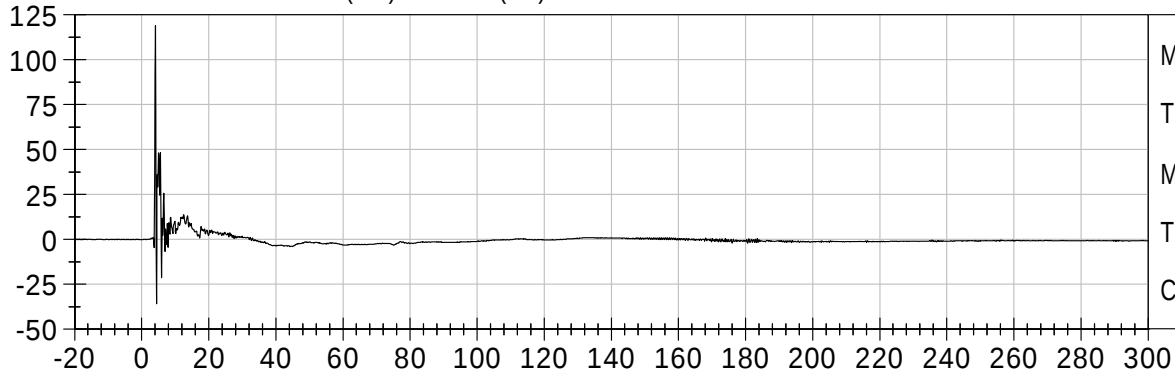
PASSENGER CHEST Y (G's) vs TIME (ms)
