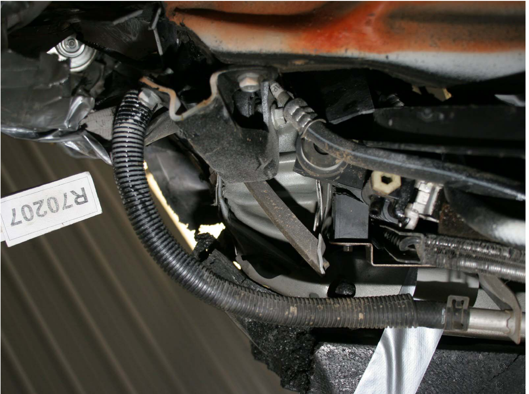
Figure A-162: Test Vehicle Post-Test Left Side Crush Initiators
