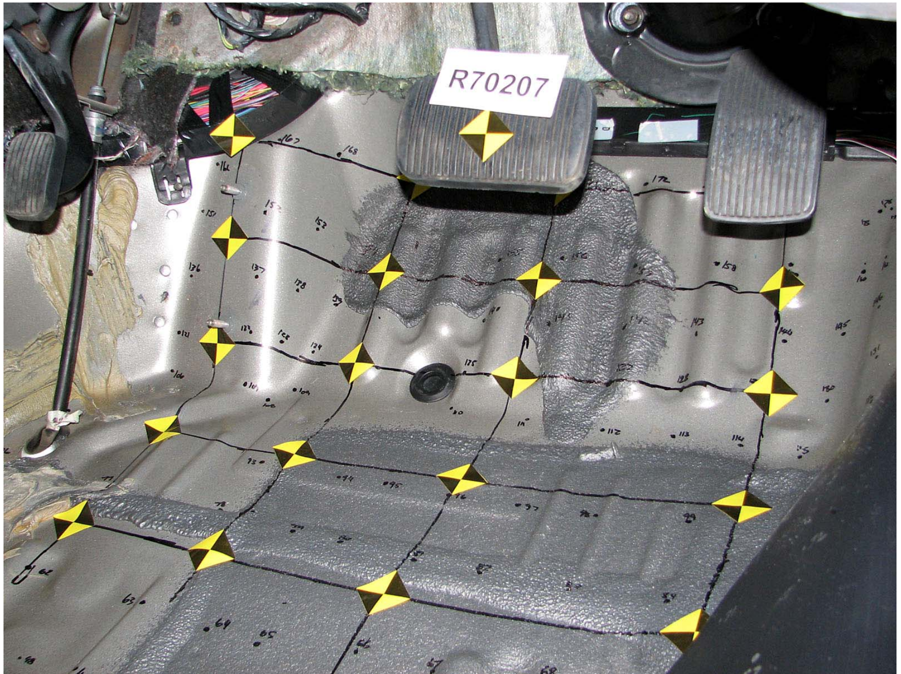
Figure A-295: Test Vehicle Pre-Test Driver Floorpan Right \frac{3}{4} View, Seat Cushion Height
