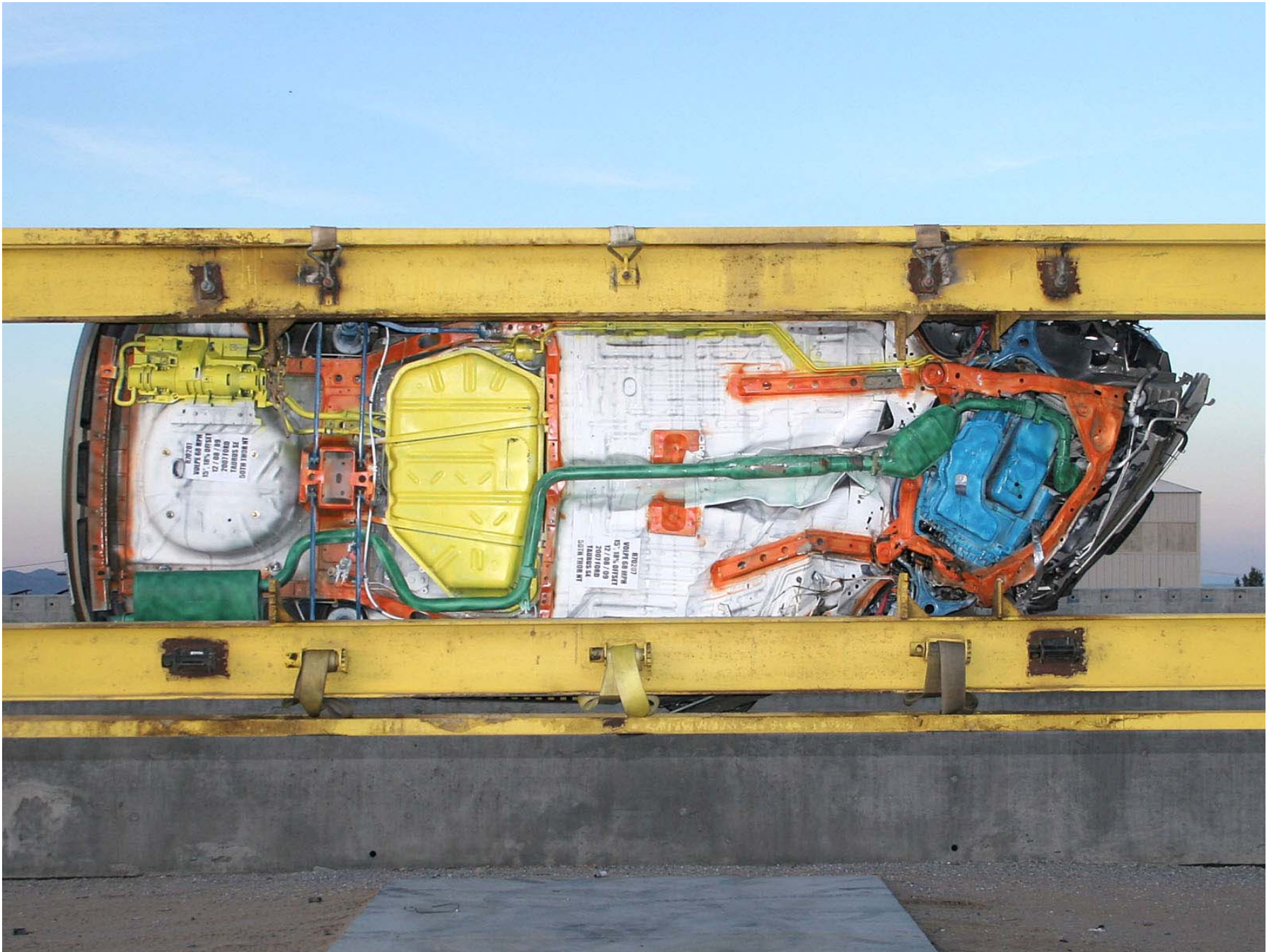
Figure A-335: Test Vehicle on Rollover Device (270°)
