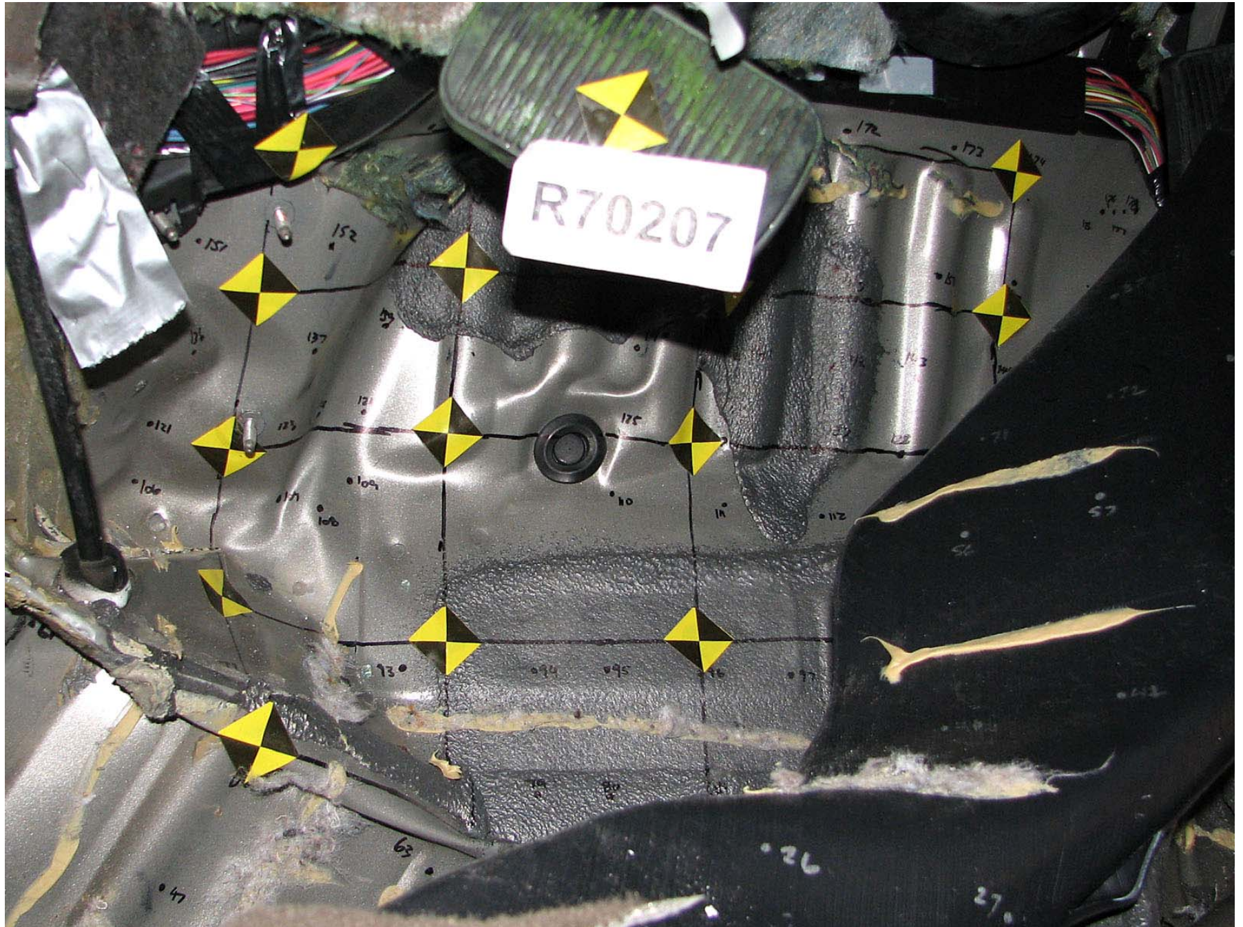
Figure A-292: Test Vehicle Post-Test Driver Floorpan, Seat Cushion Height
