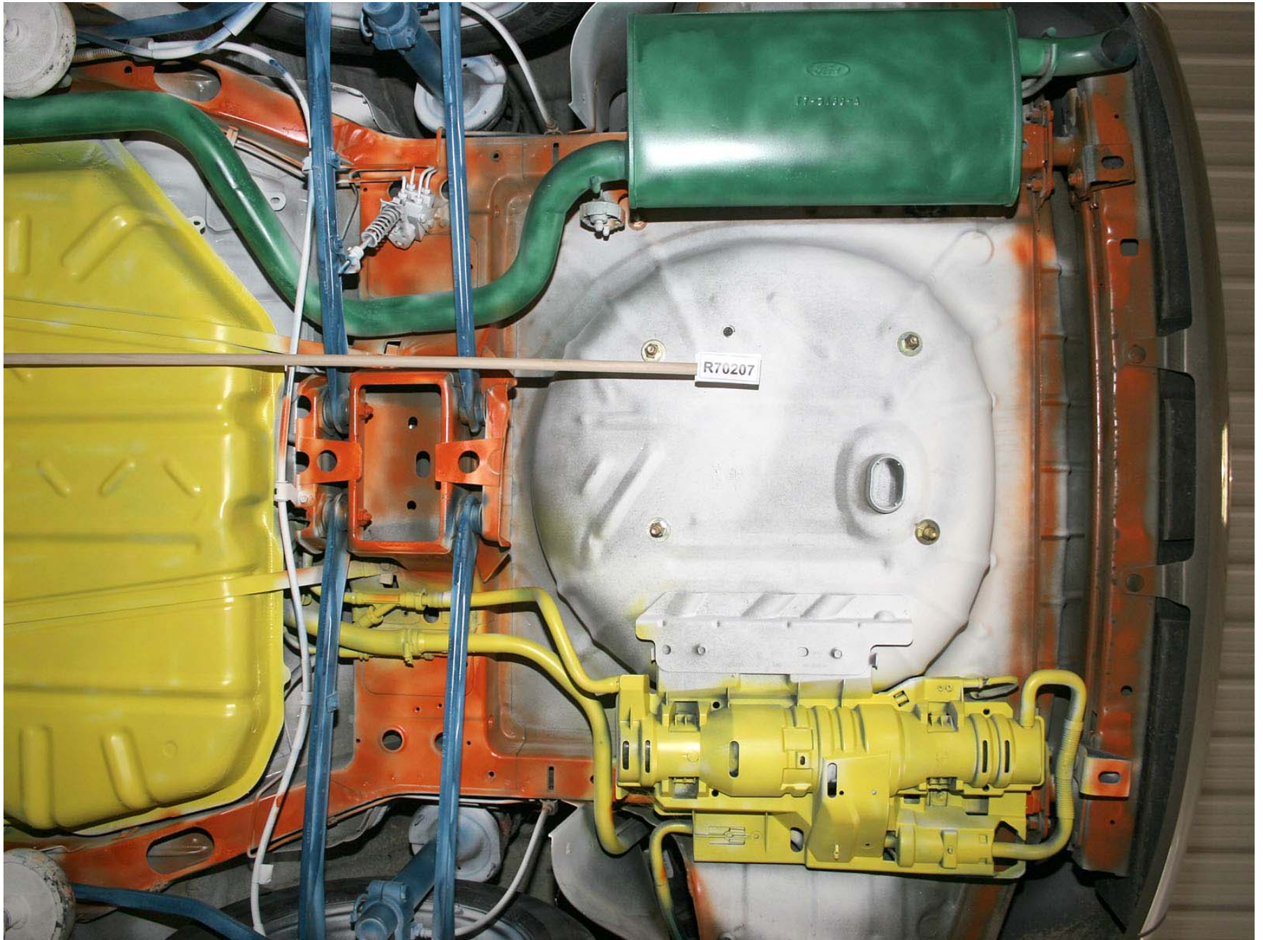
Figure A-209: Test Vehicle Pre-Test Rear Underbody
