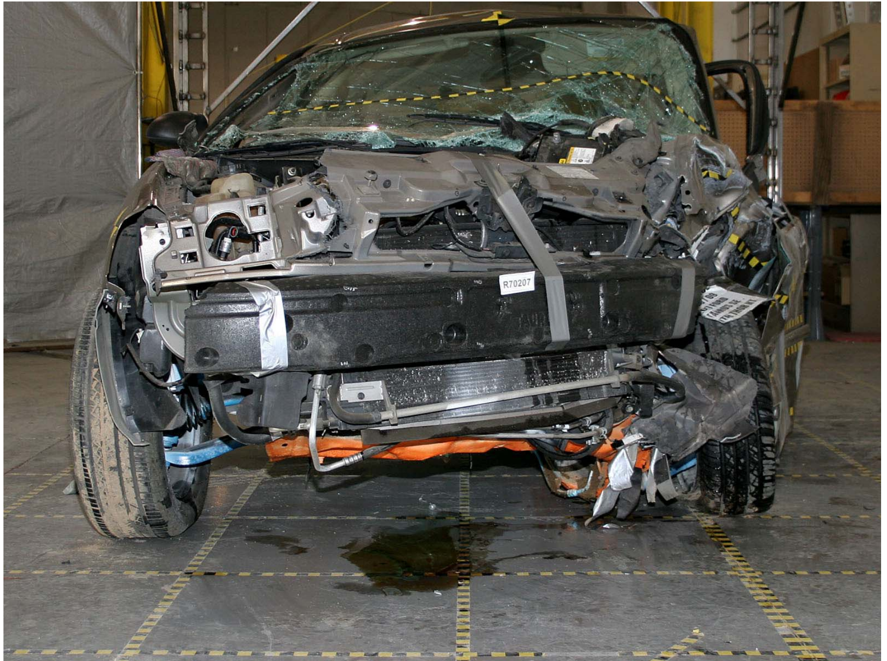
Figure A-313: Test Vehicle Post-Test Structural Member Crush Measurement
