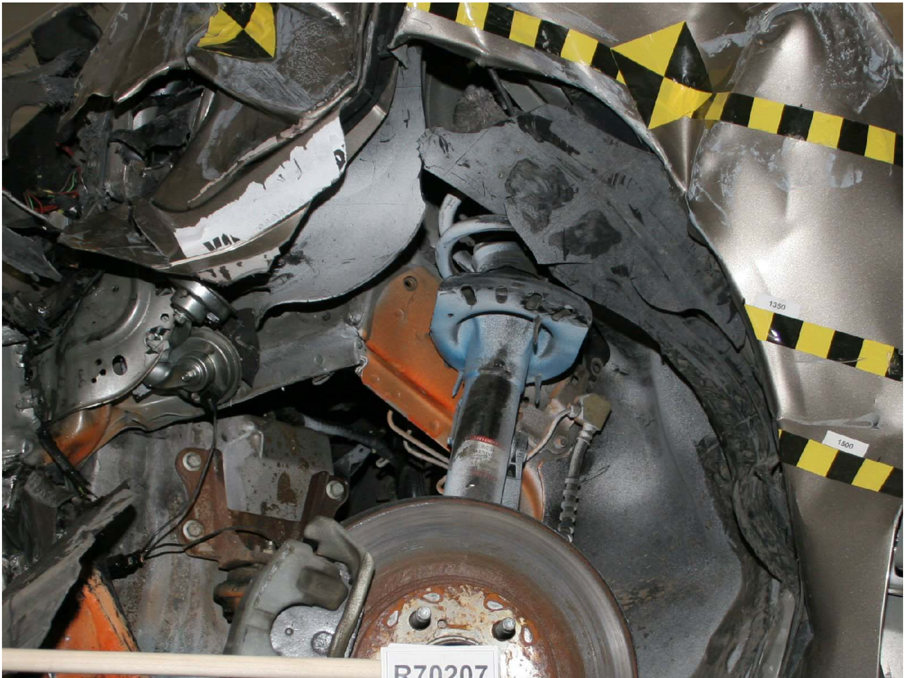
Figure A-152: Test Vehicle Post-Test Left Front Frame Rail View
