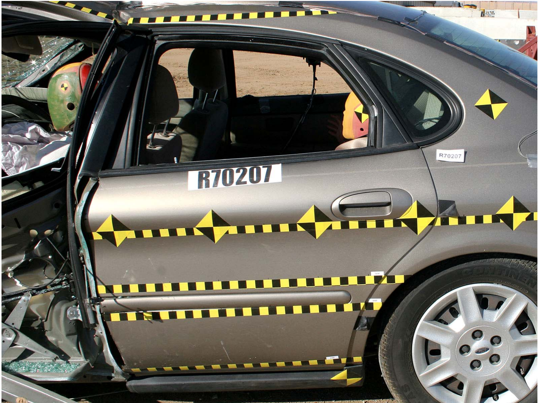
Figure A-40: Test Vehicle Post-Test Left Rear Door
