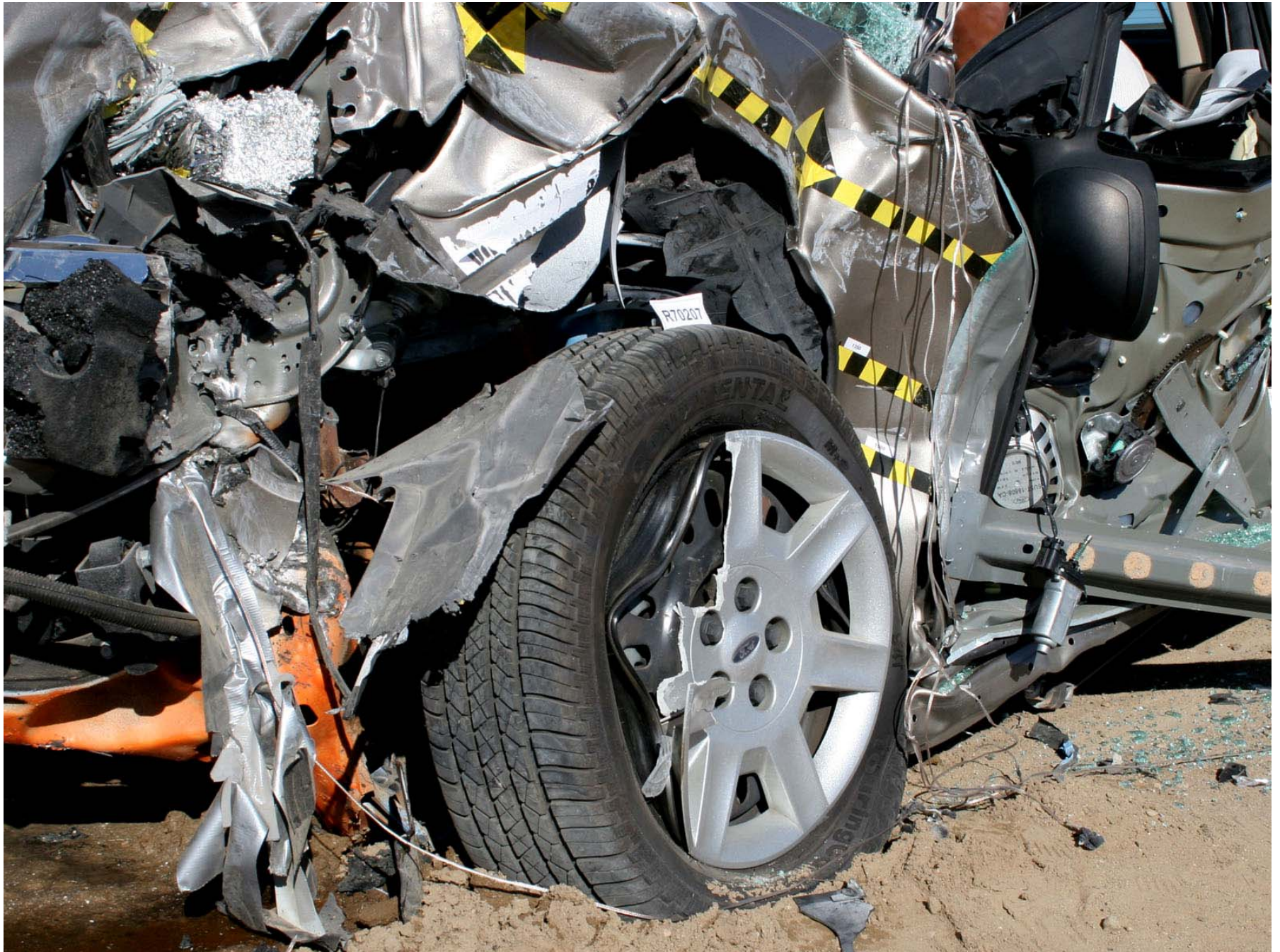
Figure A-110: Test Vehicle Post-Test Left Front Wheel Front \frac{3}{4} View
