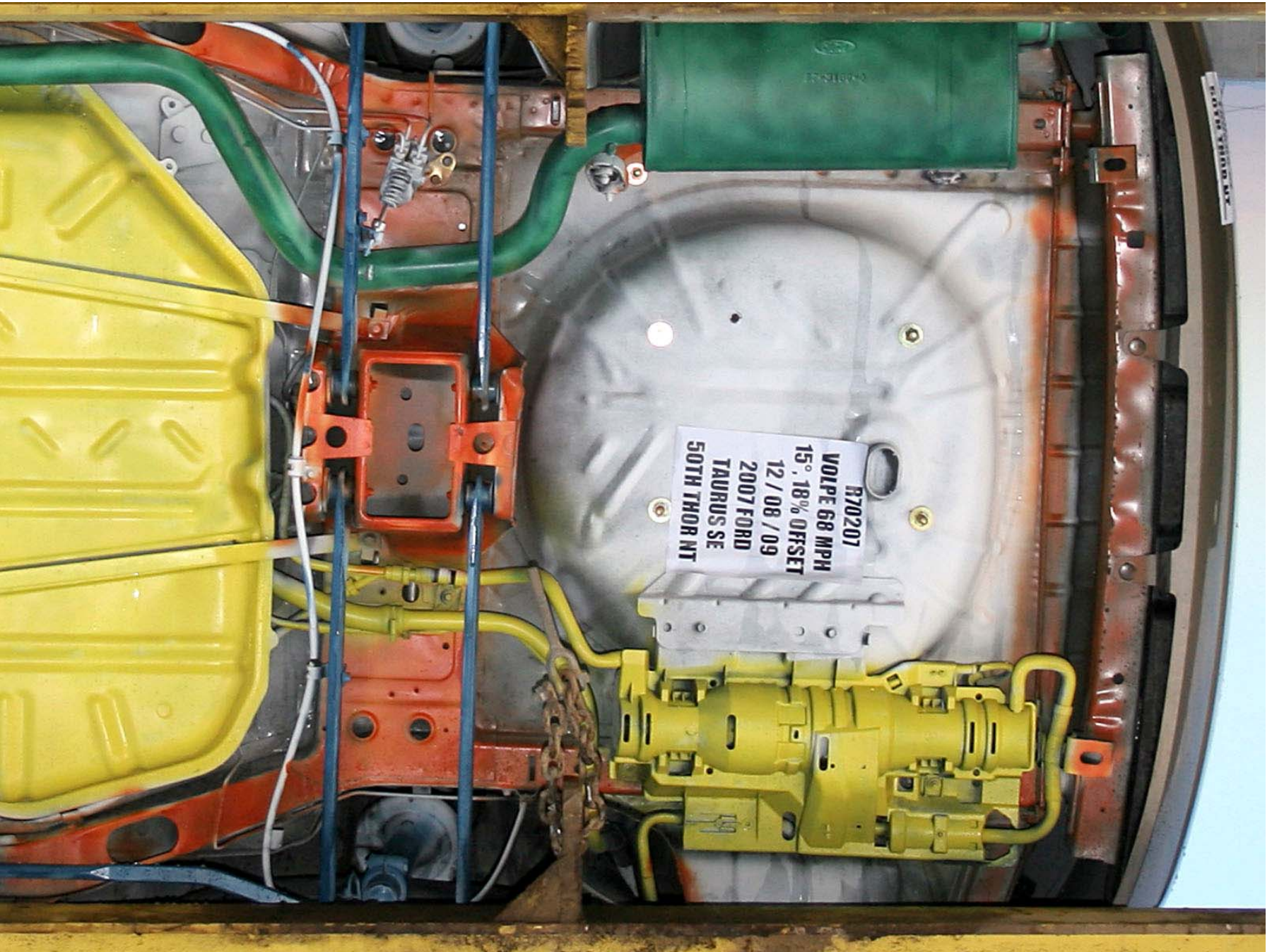
Figure A-210: Test Vehicle Post-Test Rear Underbody
