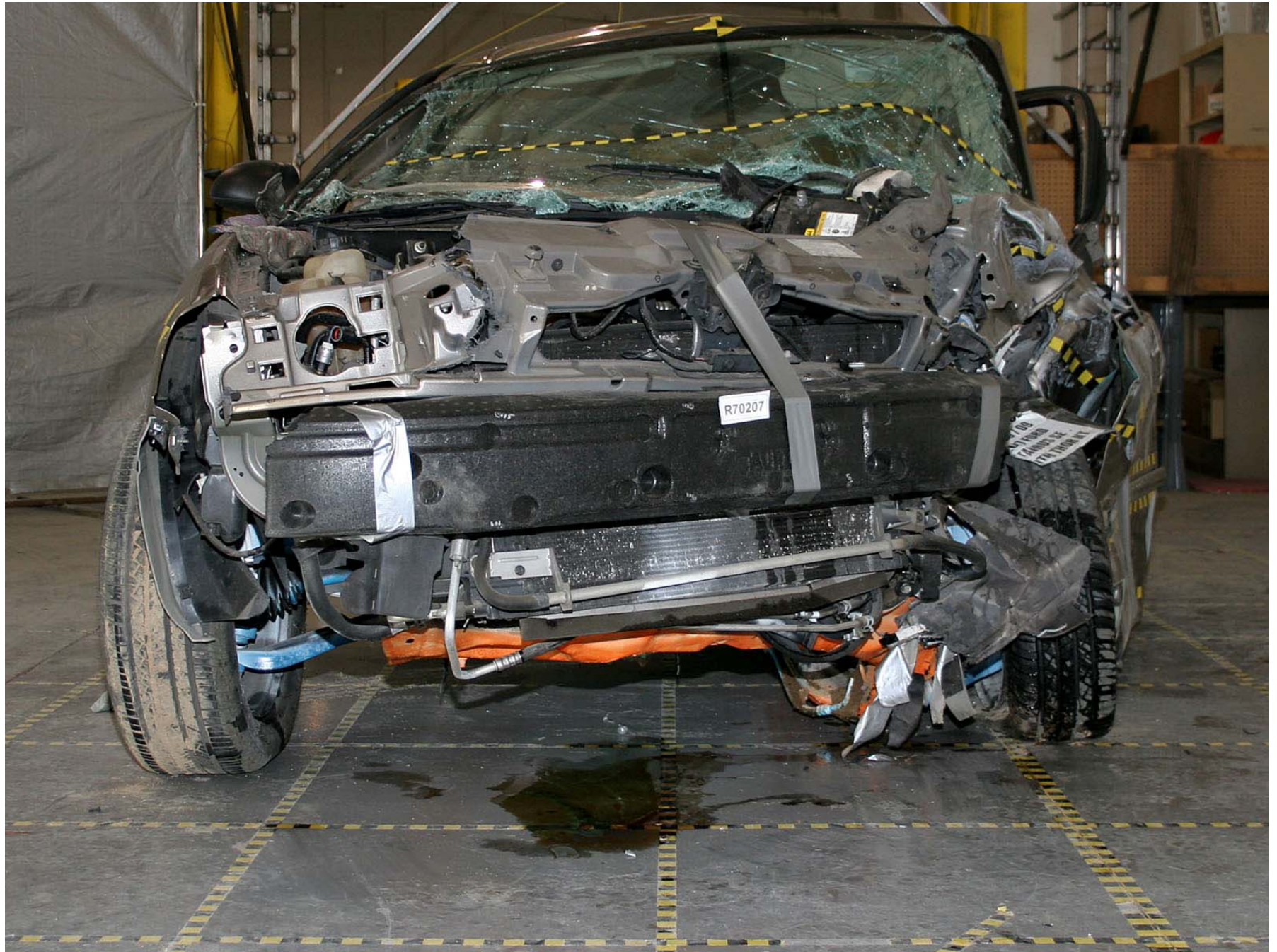
Figure A-317: Test Vehicle Post-Test Structural Member Crush Measurement
