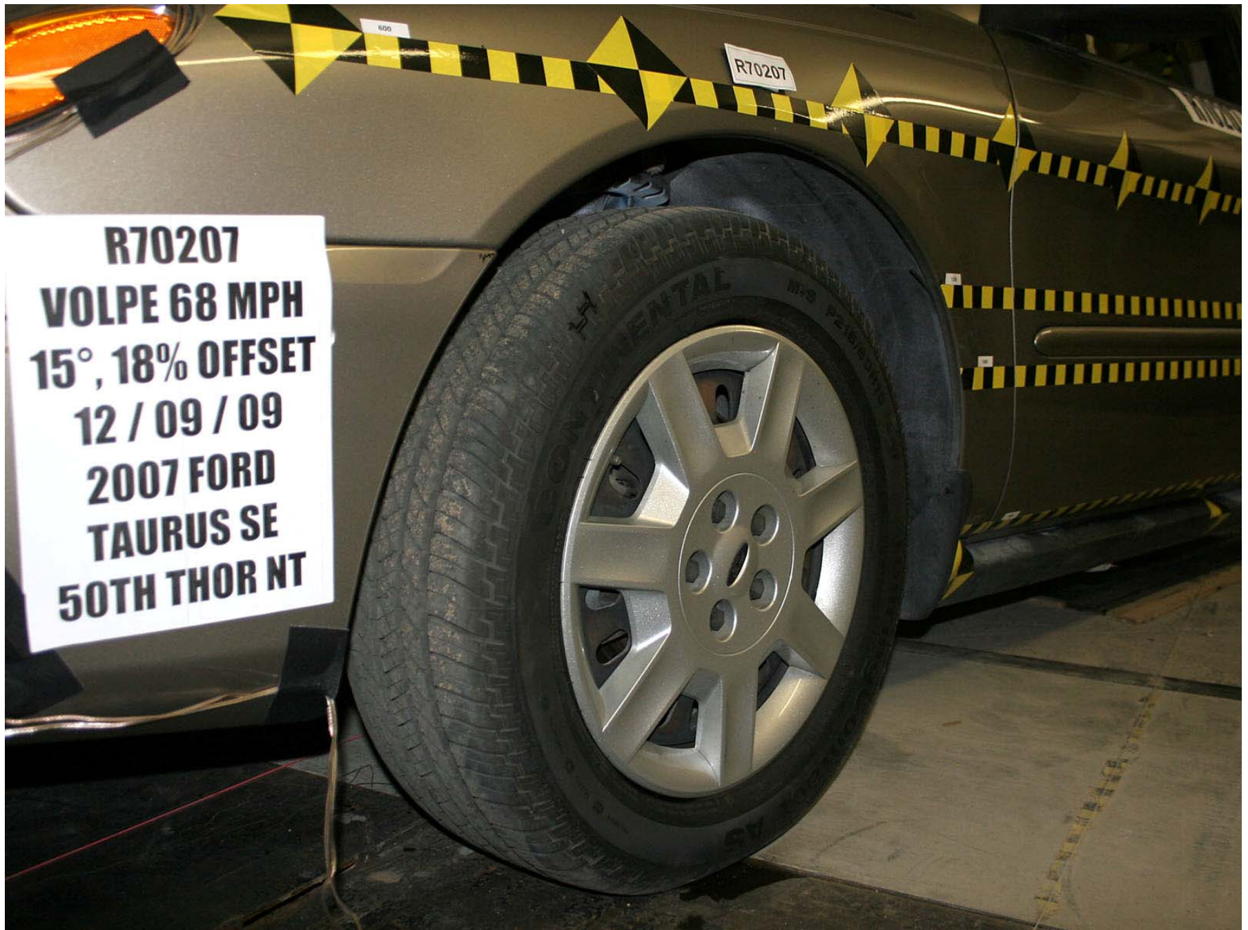
Figure A-109: Test Vehicle Pre-Test Left Front Wheel Front \frac{3}{4} View
