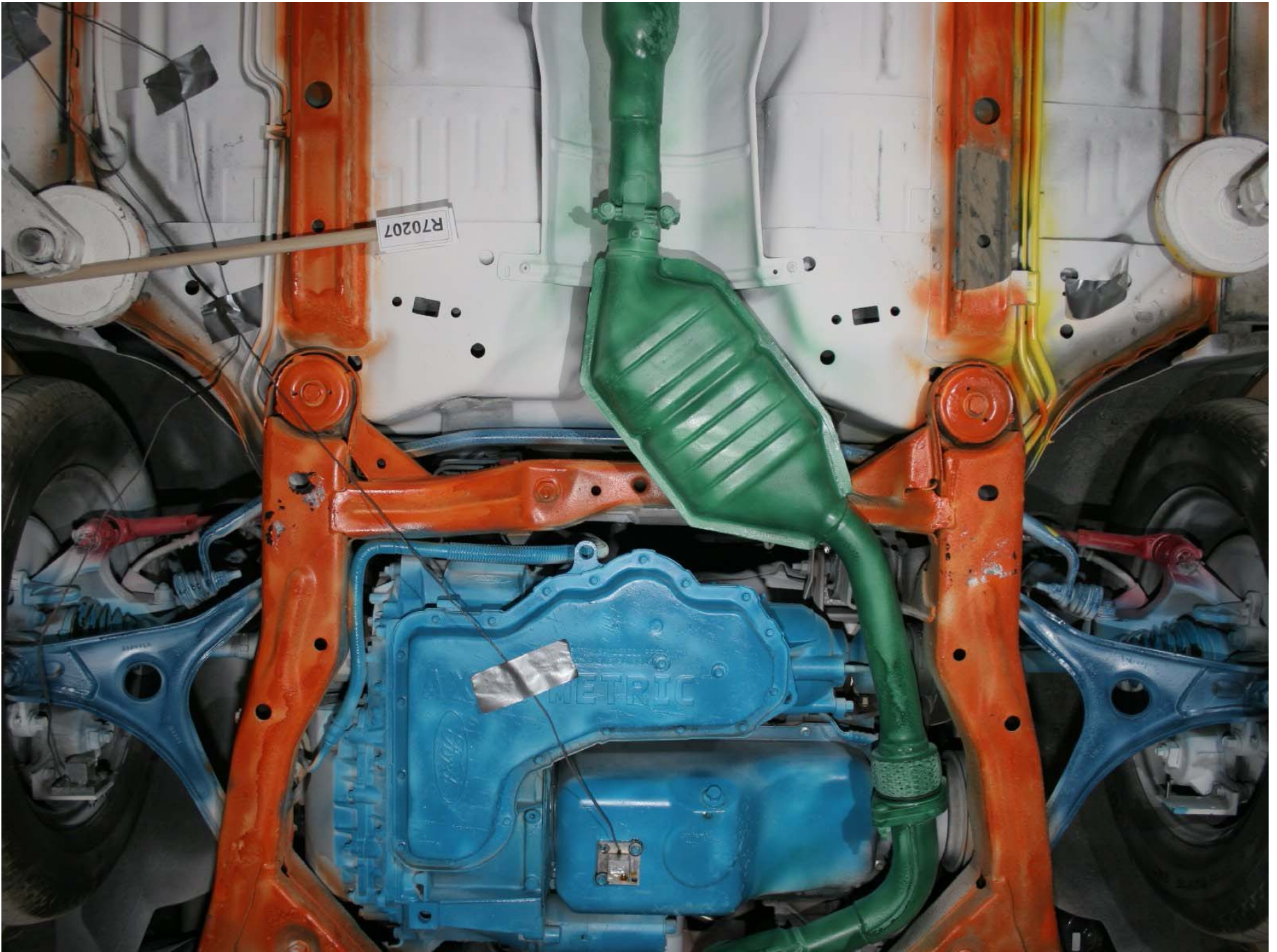
Figure A-211: Test Vehicle Pre-Test Steering Rack and Sway Bar View
