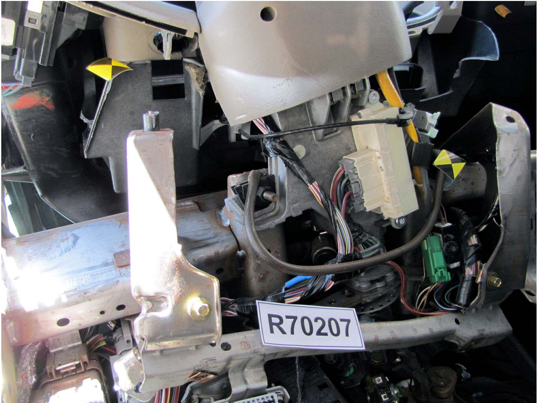
Figure A-249: Test Vehicle Post-Test Driver's Side Knee Bolster
