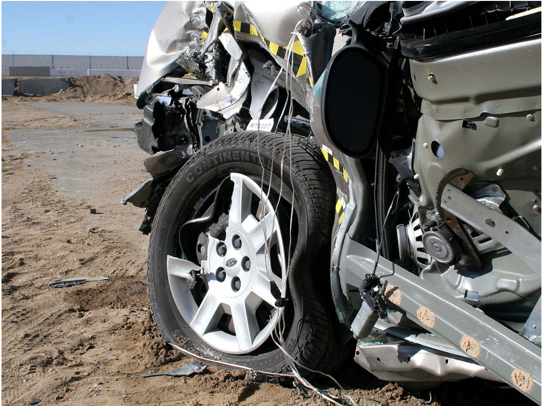
Figure A-112: Test Vehicle Post-Test Left Front Wheel Rear \frac{3}{4} View
