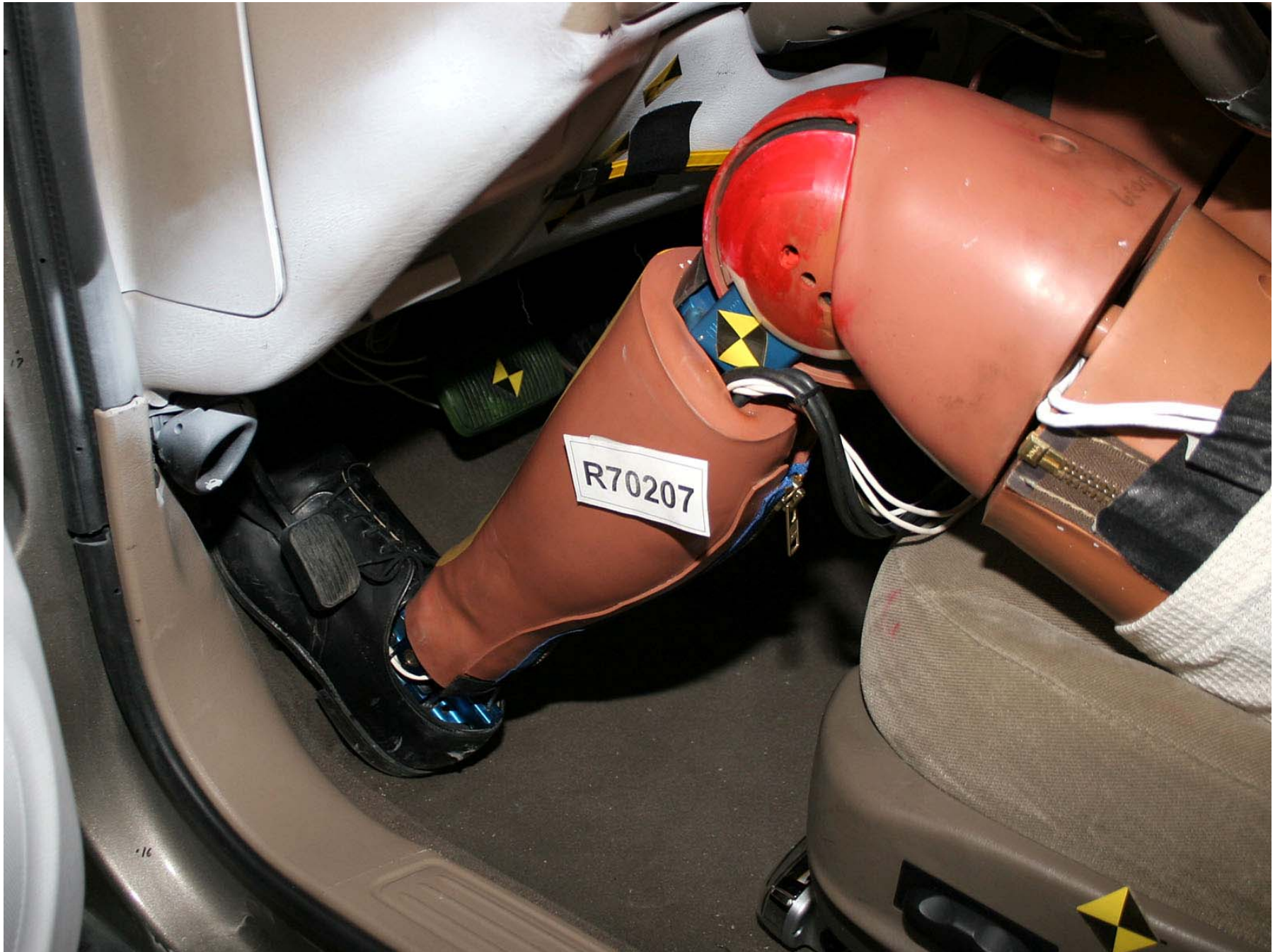
Figure A-233: Test Vehicle Pre-Test Driver Dummy Feet Positioning
