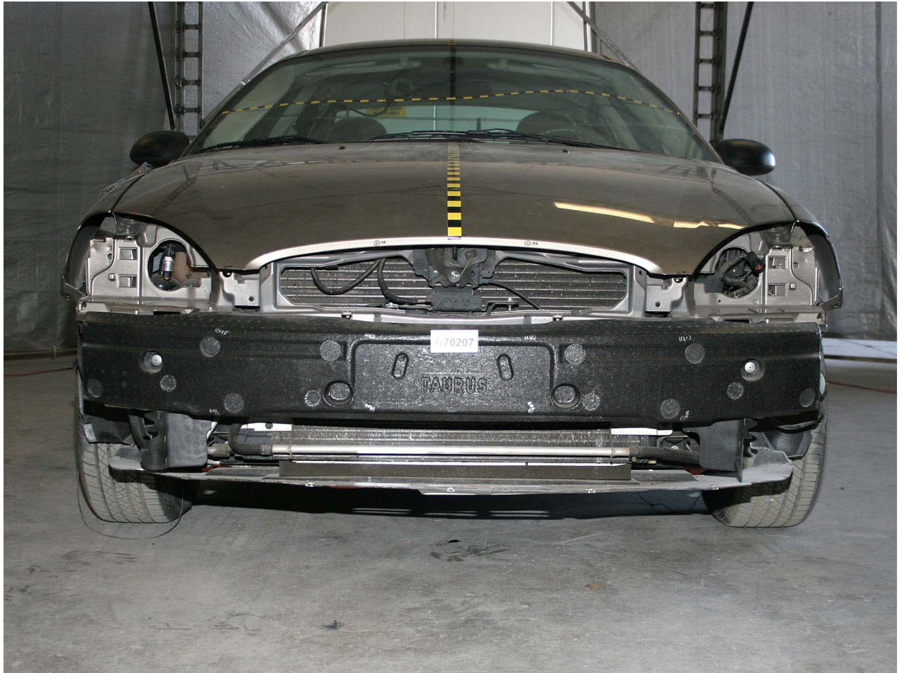
Figure A-312: Test Vehicle Pre-Test Structural Member Crush Measurement
