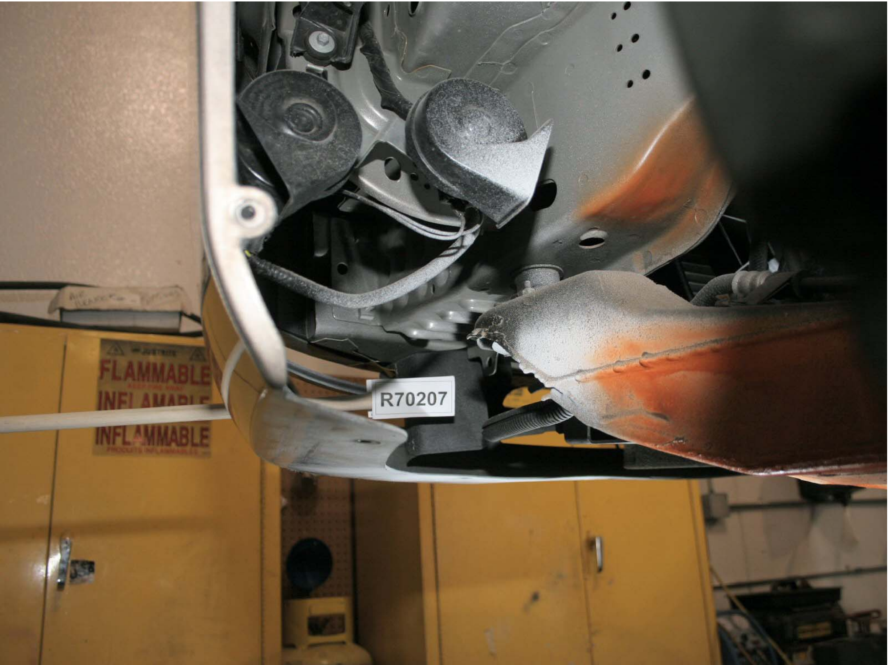
Figure A-159: Test Vehicle Pre-Test Left Side Crush Initiators
