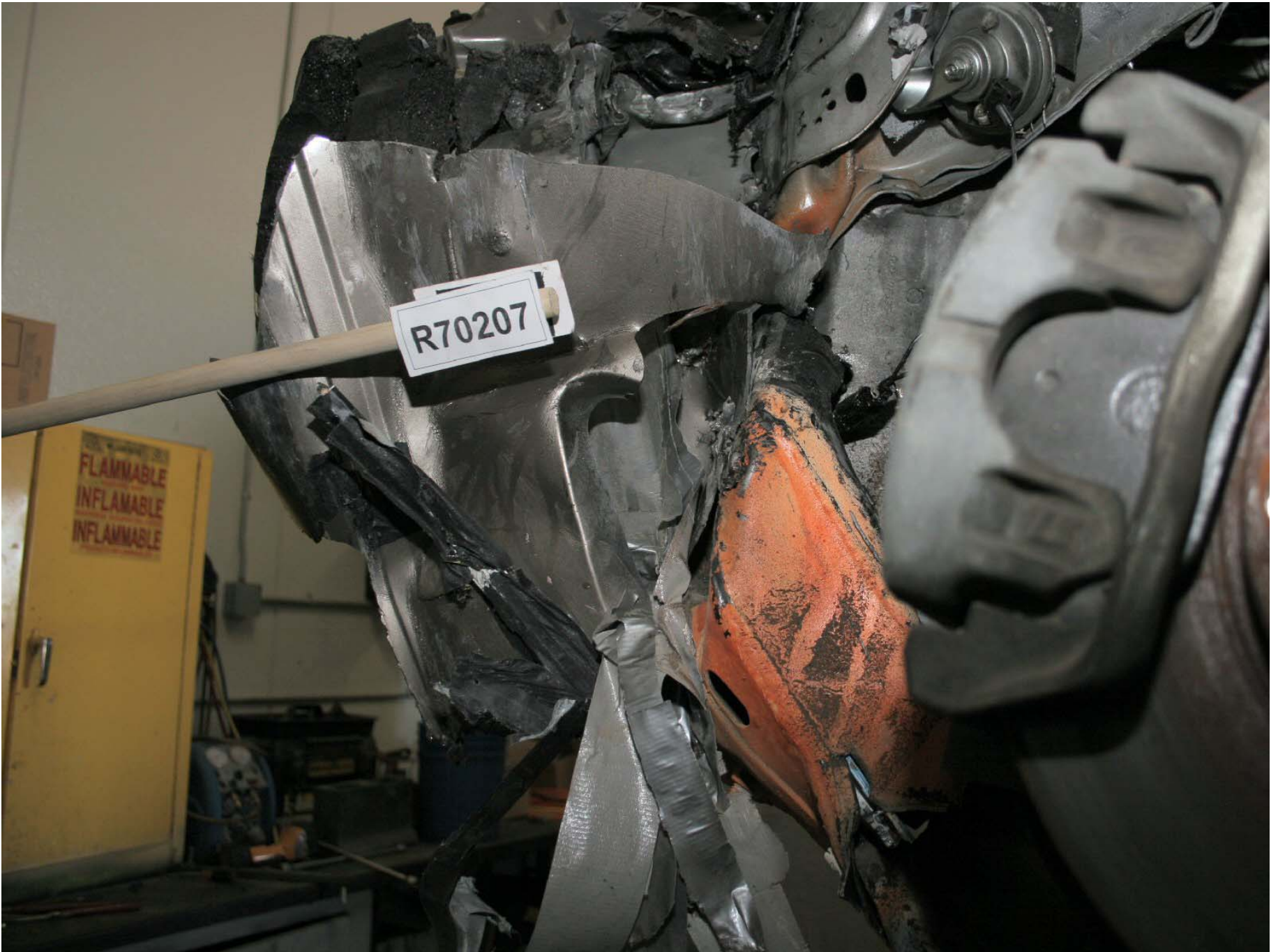
Figure A-160: Test Vehicle Post-Test Left Side Crush Initiators
