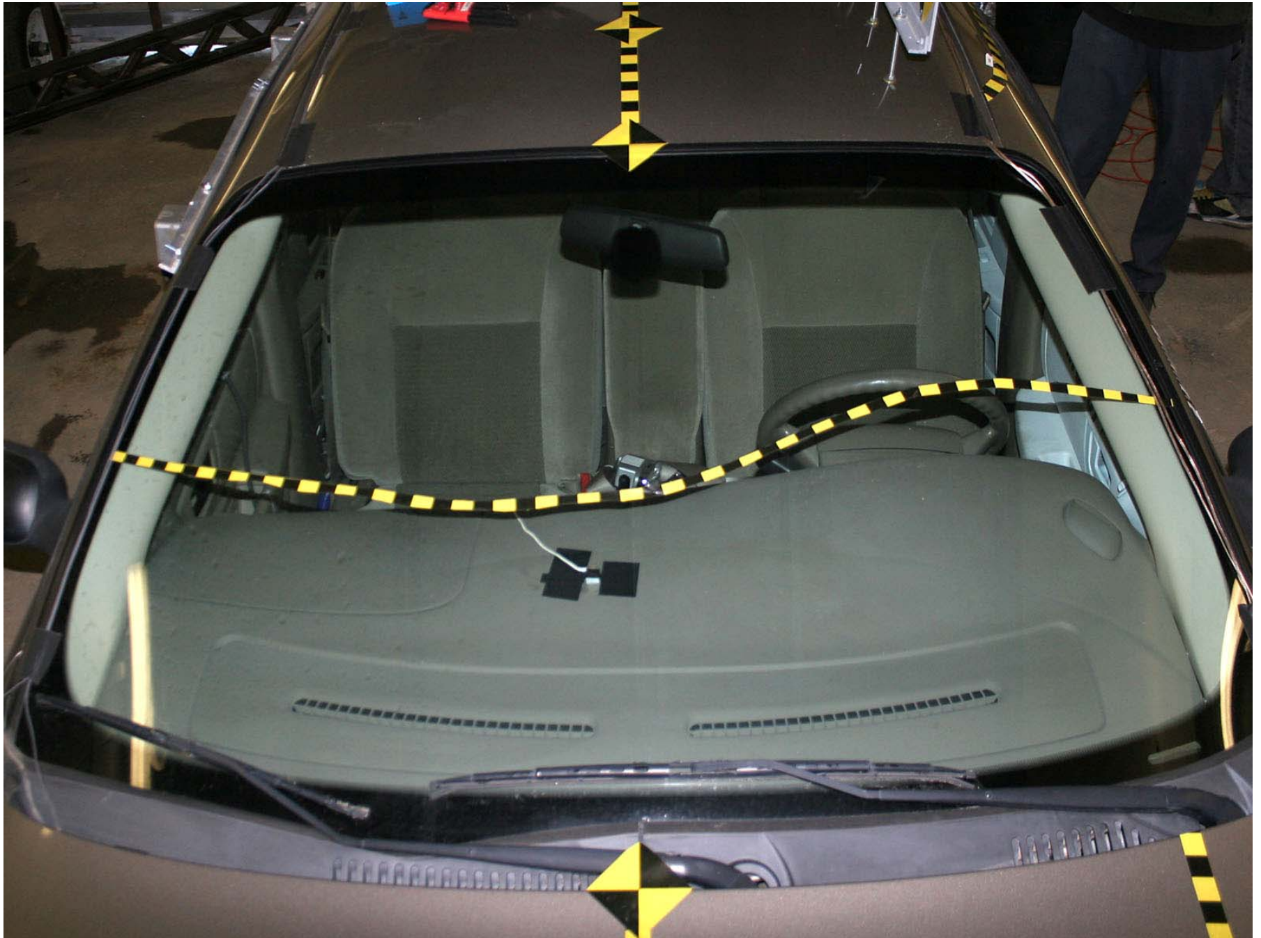
Figure A-45: Test Vehicle Pre-Test Windshield View
