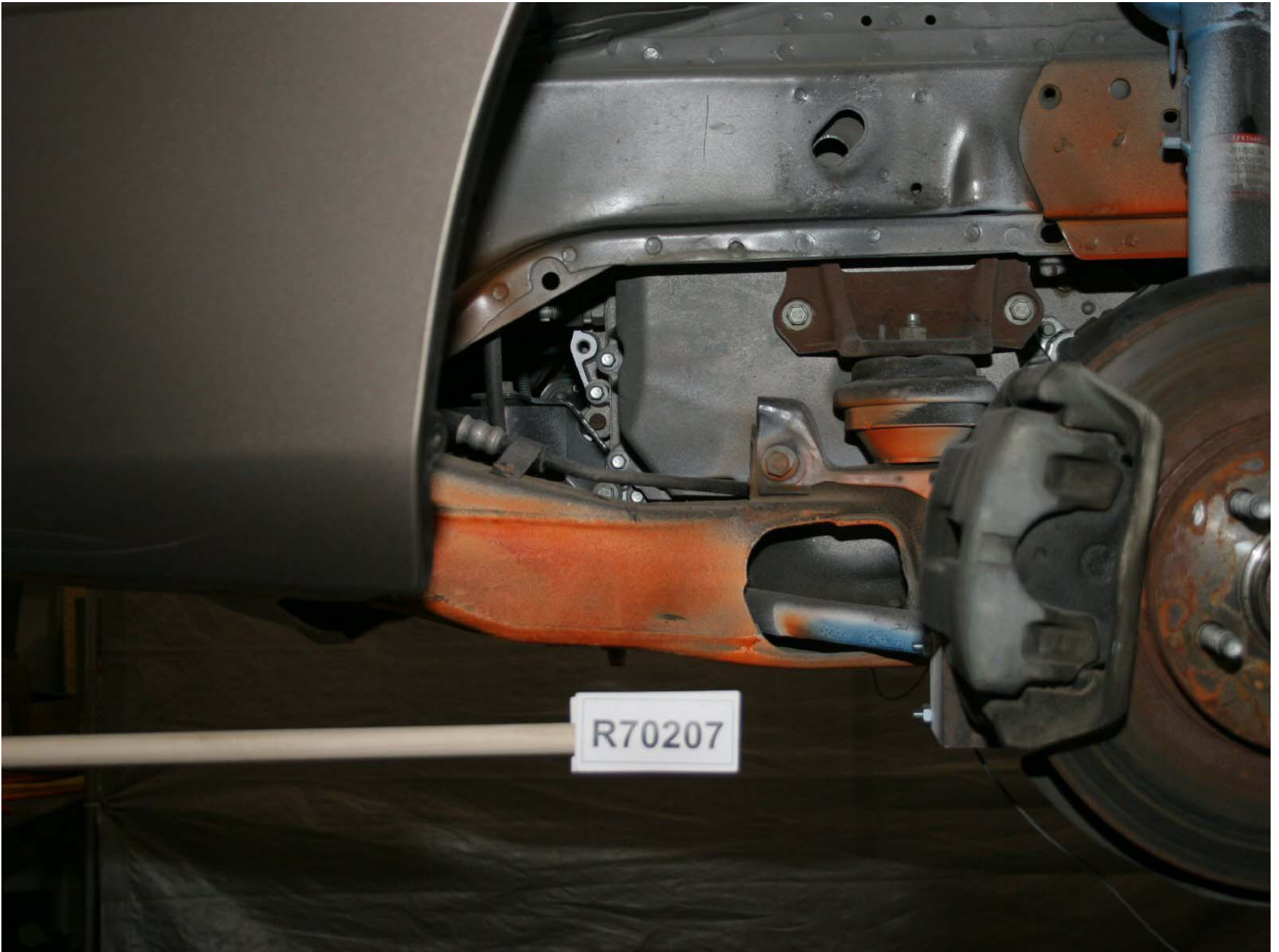
Figure A-147: Test Vehicle Pre-Test Left Front Frame Rail View
