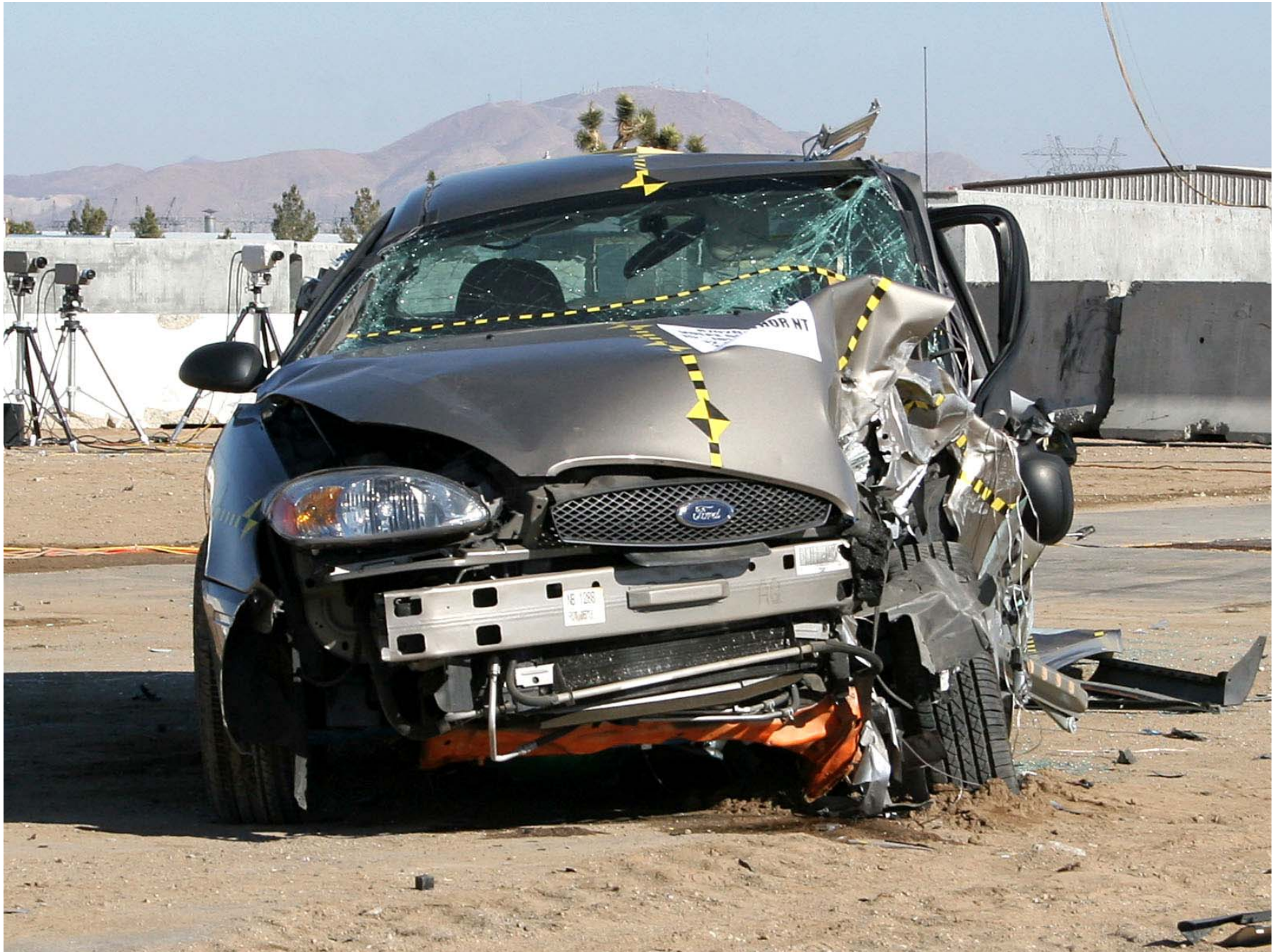
Figure A-6: Test Vehicle Post-Test Front View
