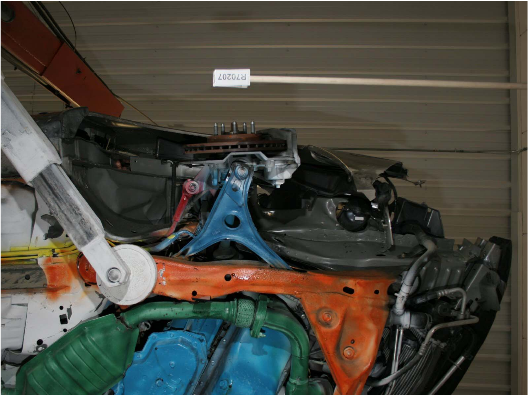
Figure A-176: Test Vehicle Post-Test Right Inner Fender Well View
