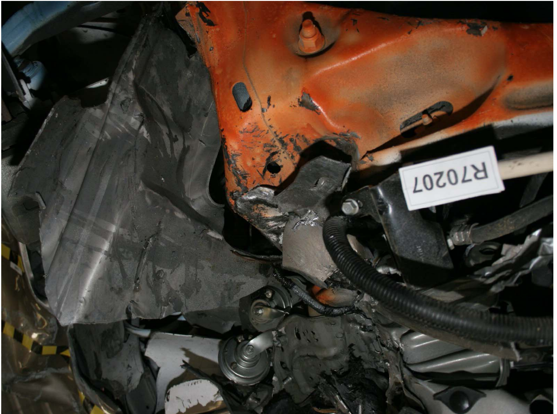
Figure A-166: Test Vehicle Post-Test Left Front Sub-Frame Mounting Point
