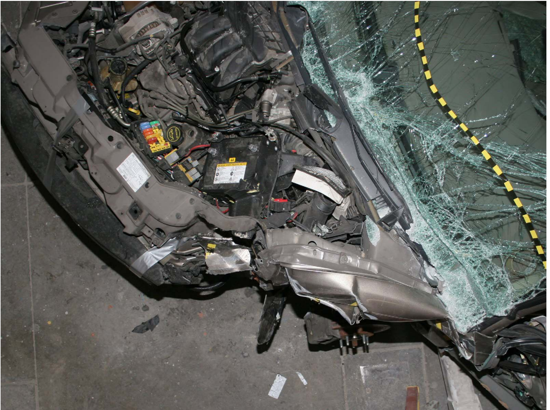
Figure A-146: Test Vehicle Post-Test Top Fender View
