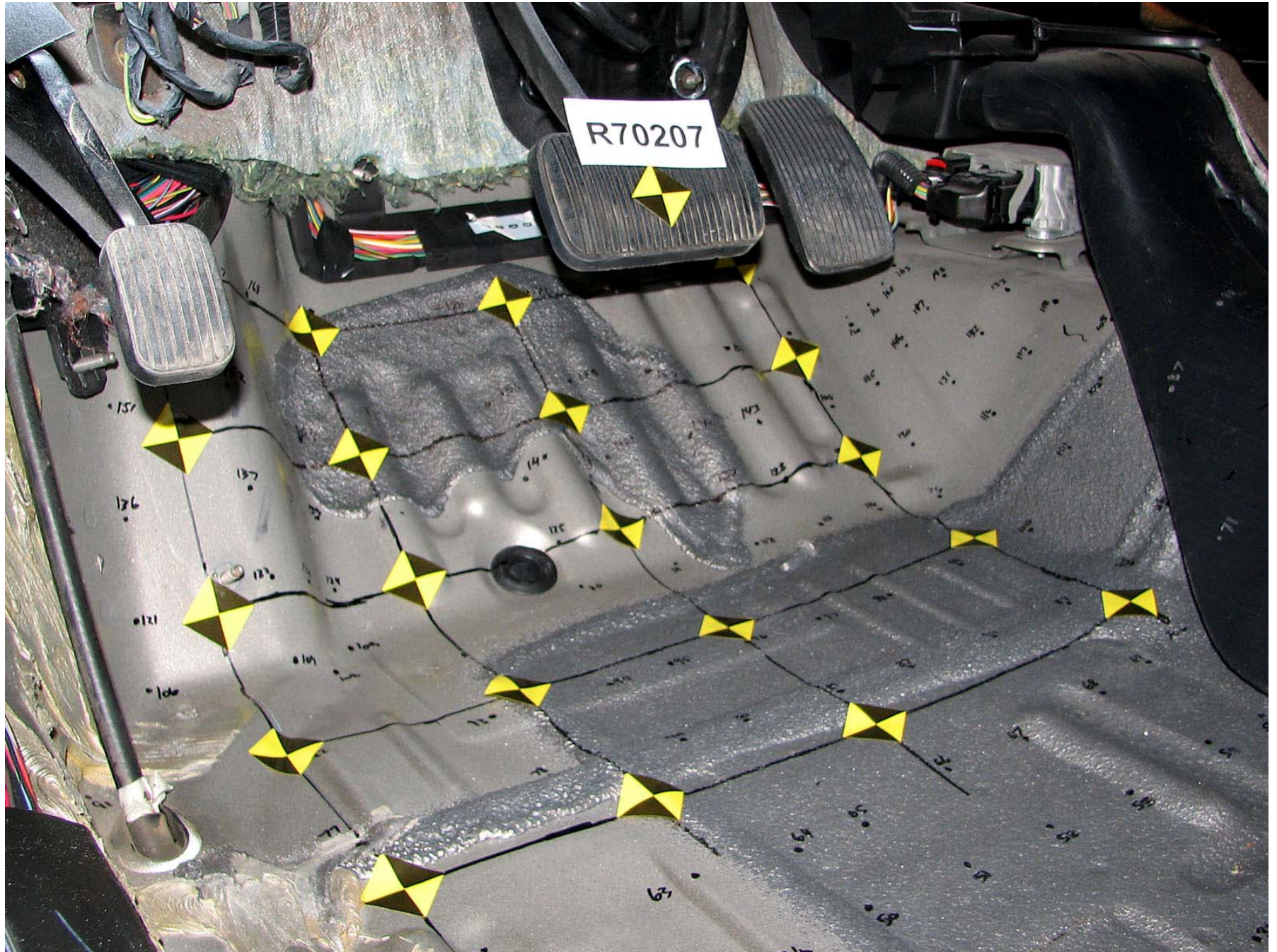
Figure A-287: Test Vehicle Pre-Test Driver Floorpan Left \frac{3}{4} View, Seat Cushion Height
