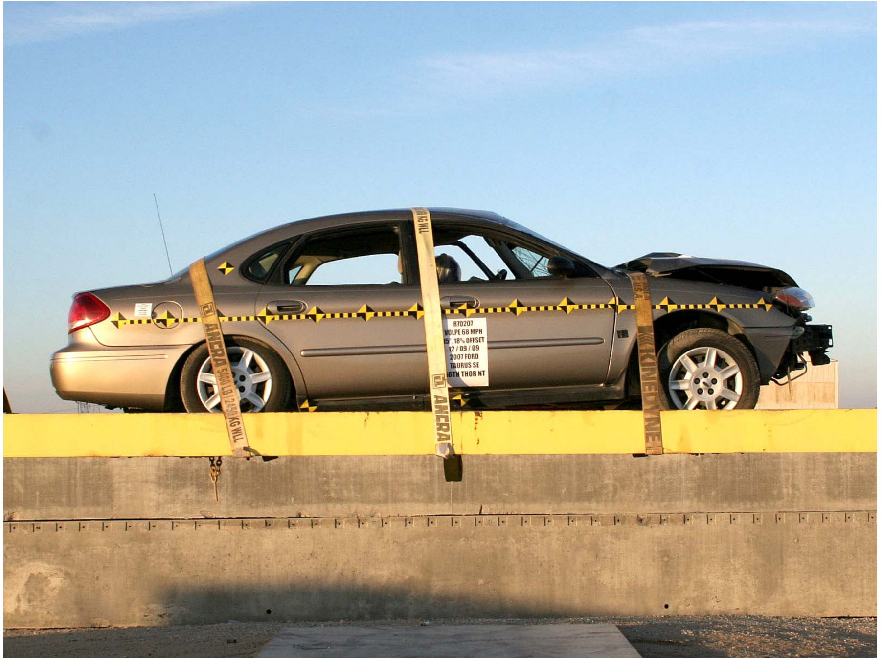
Figure A-332: Test Vehicle on Rollover Device (0°)
