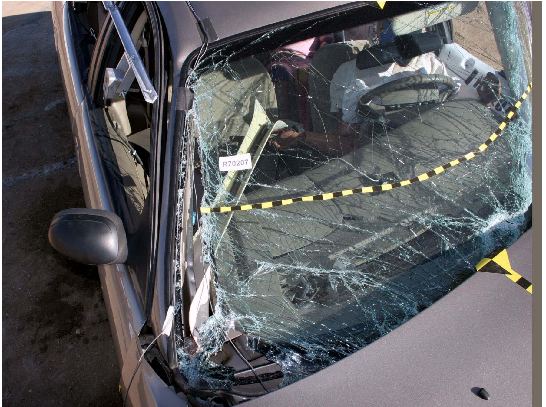
Figure A-318: Test Vehicle Post-Test Windshield Separation
