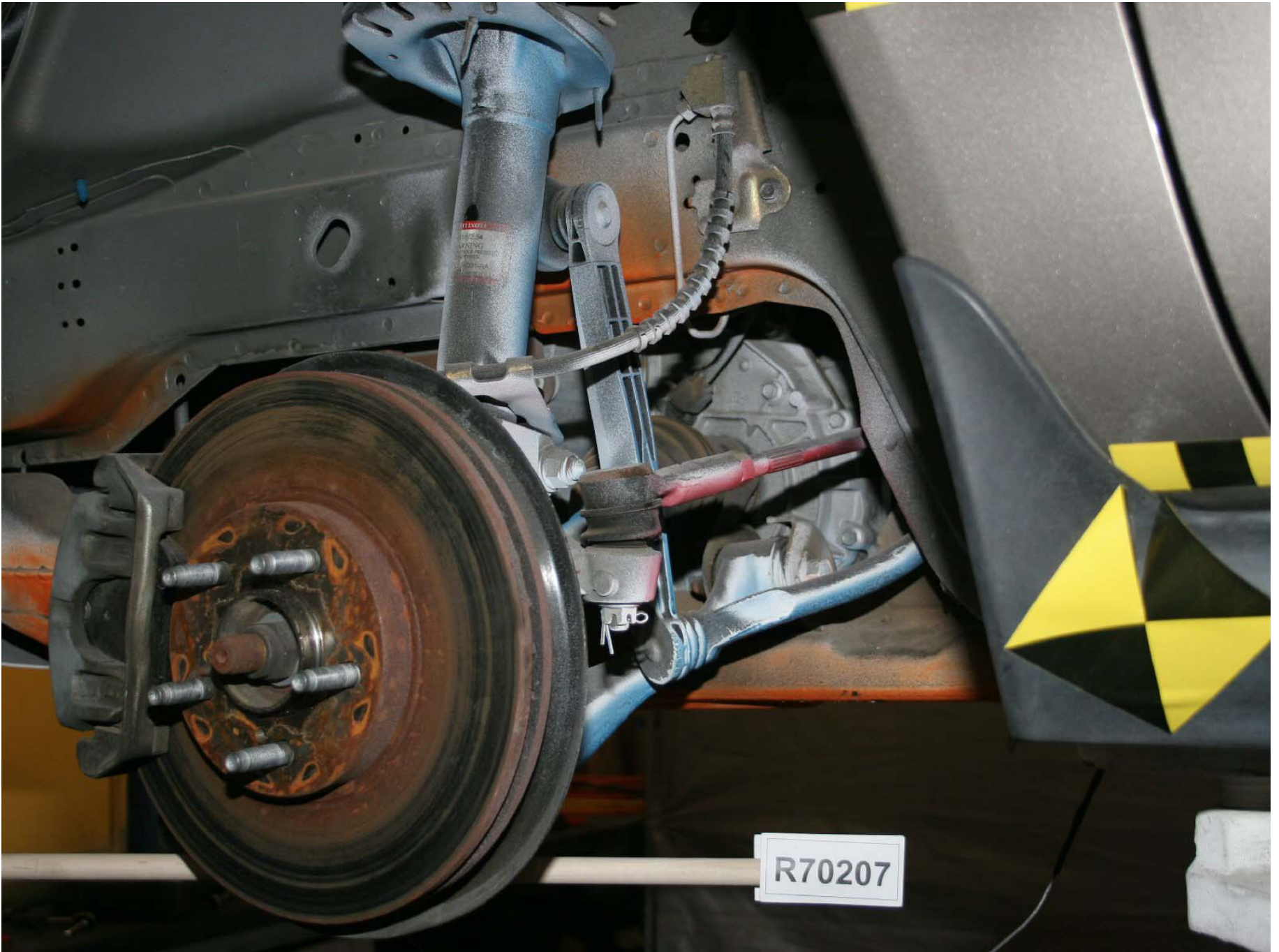
Figure A-153: Test Vehicle Pre-Test Left Side Tie Rod and Sway Bar Attachments Points
