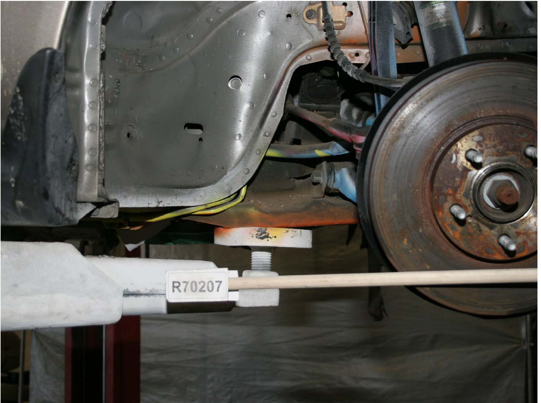
Figure A-186: Test Vehicle Post-Test Right Front Frame Rail View
