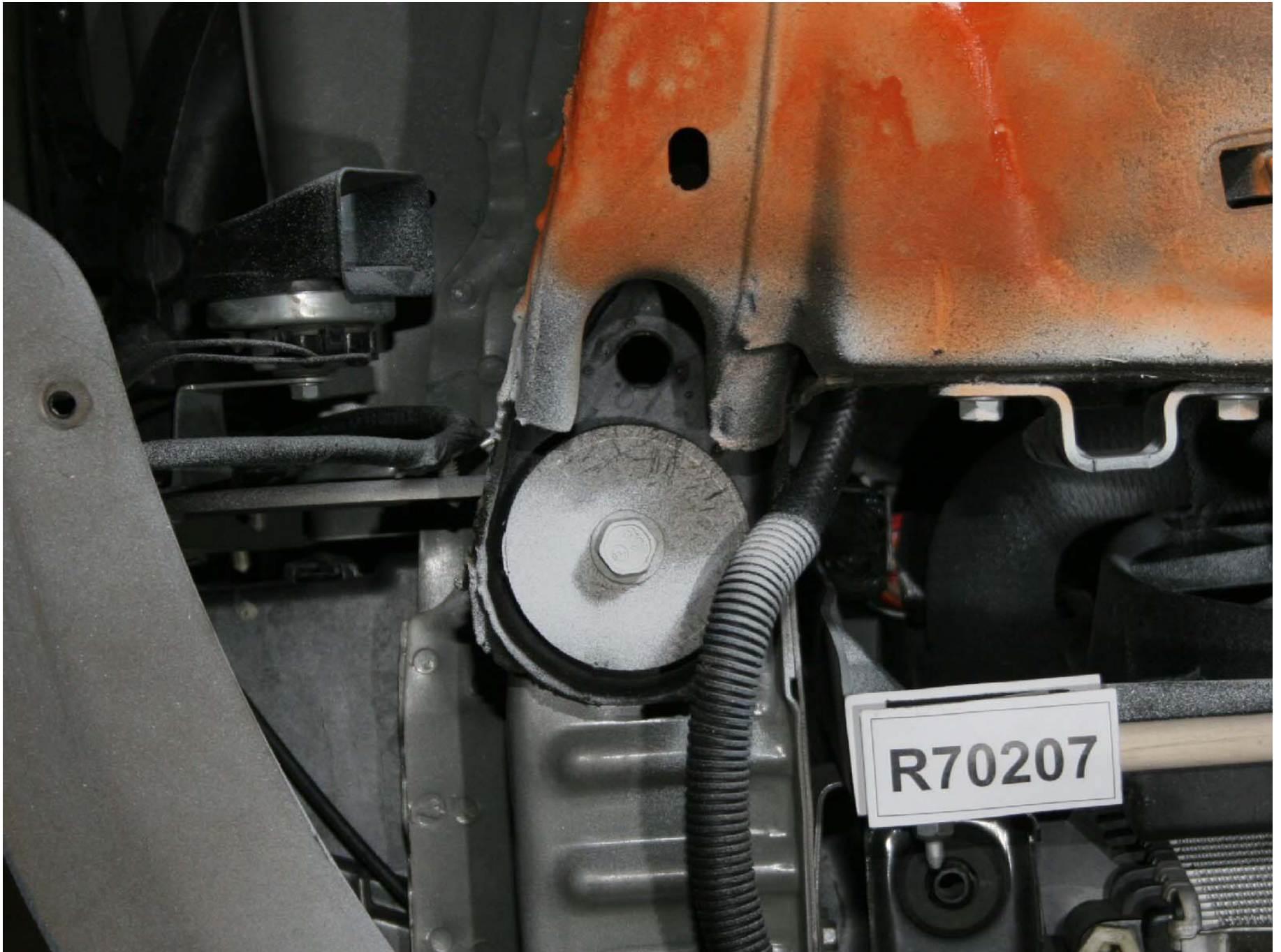
Figure A-165: Test Vehicle Pre-Test Left Front Sub-Frame Mounting Point
