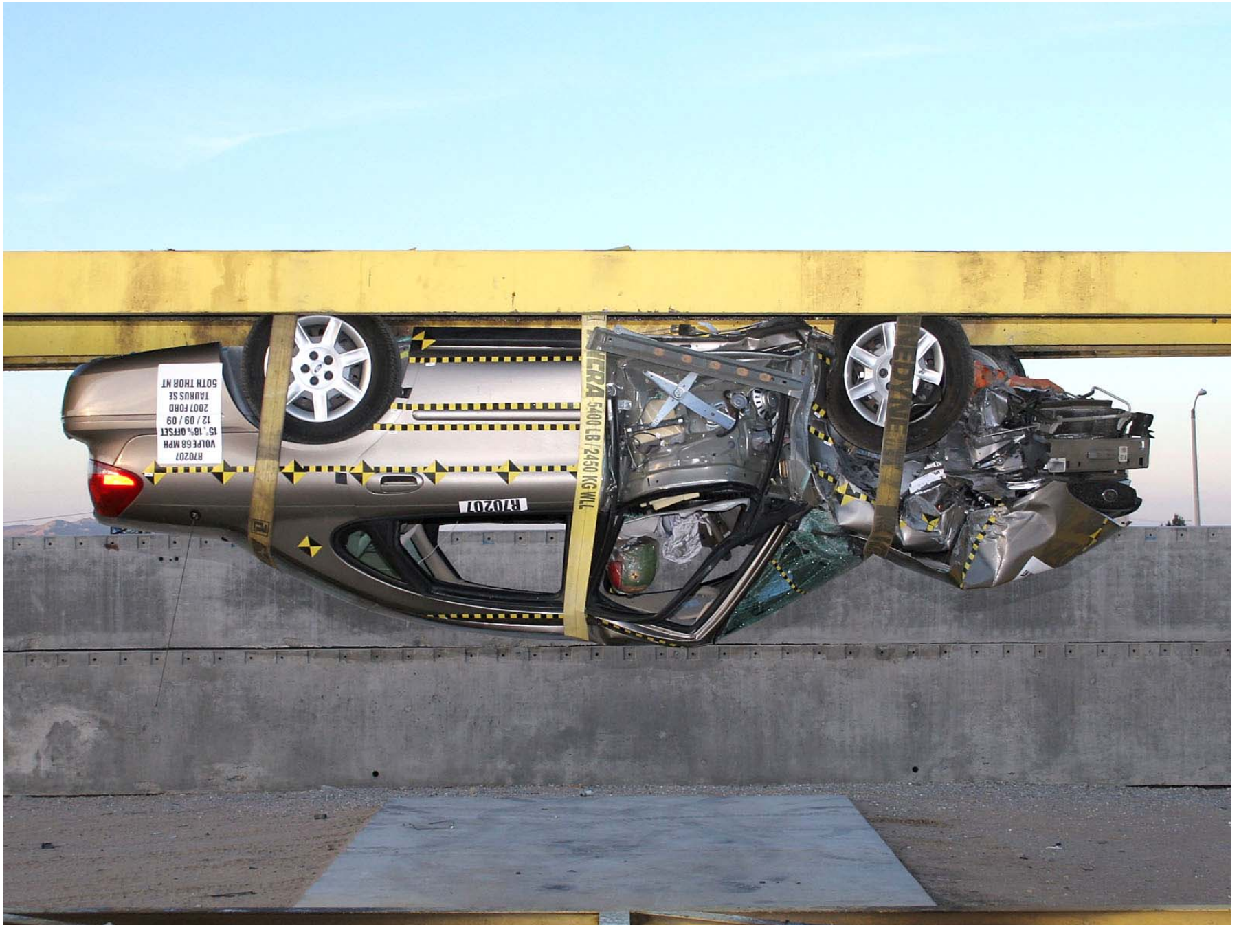
Figure A-334: Test Vehicle on Rollover Device (180°)
