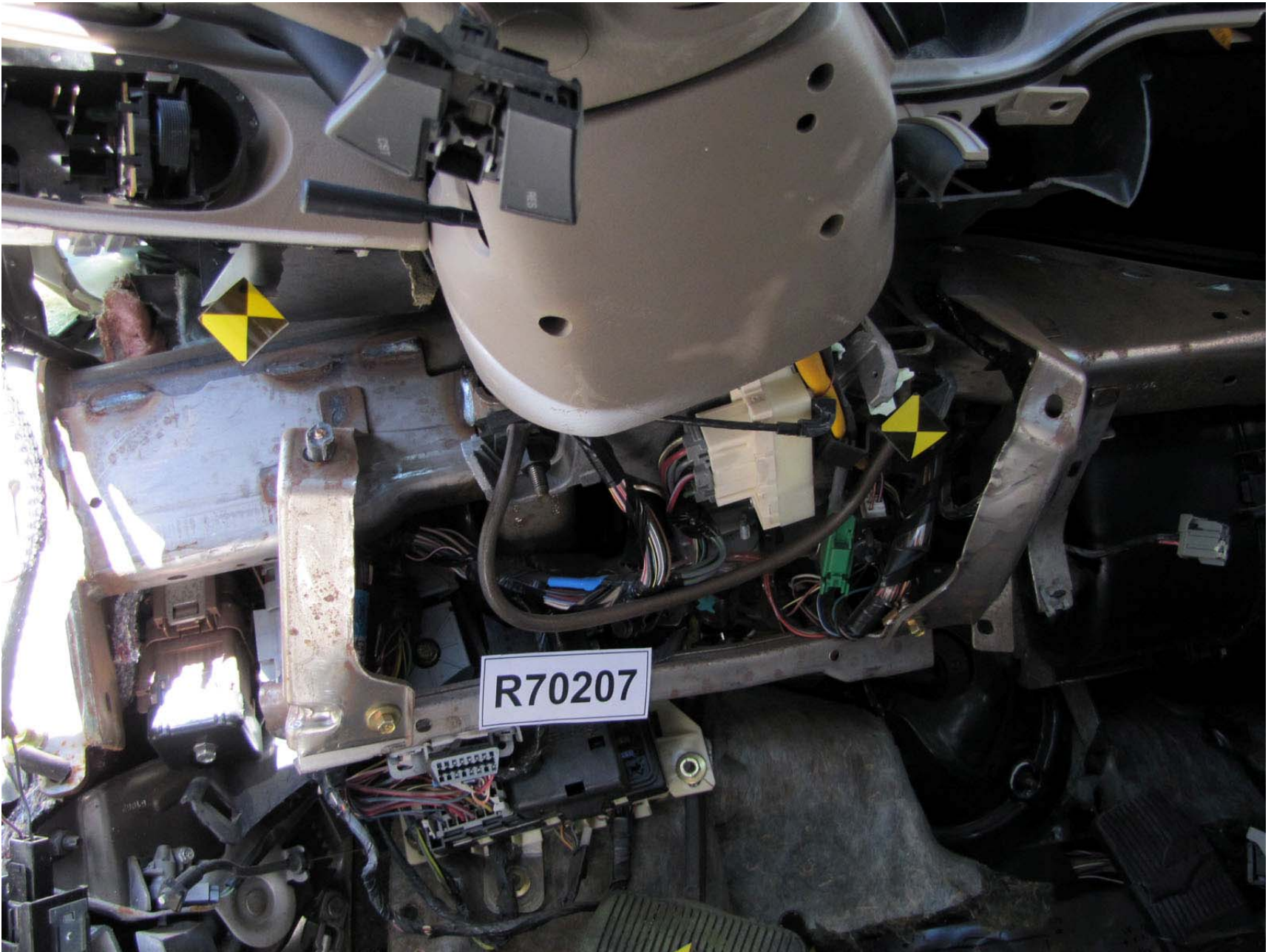
Figure A-248: Test Vehicle Post-Test Driver's Side Knee Bolster
