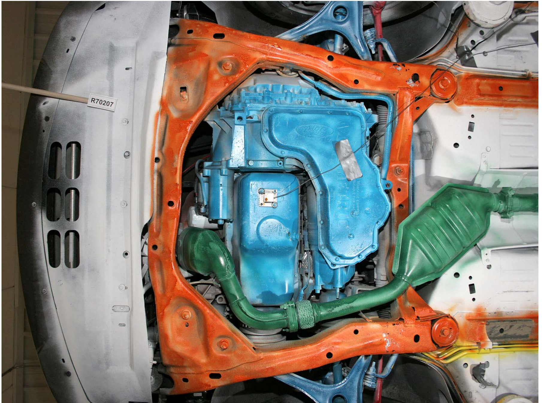
Figure A-205: Test Vehicle Pre-Test Front Underbody
