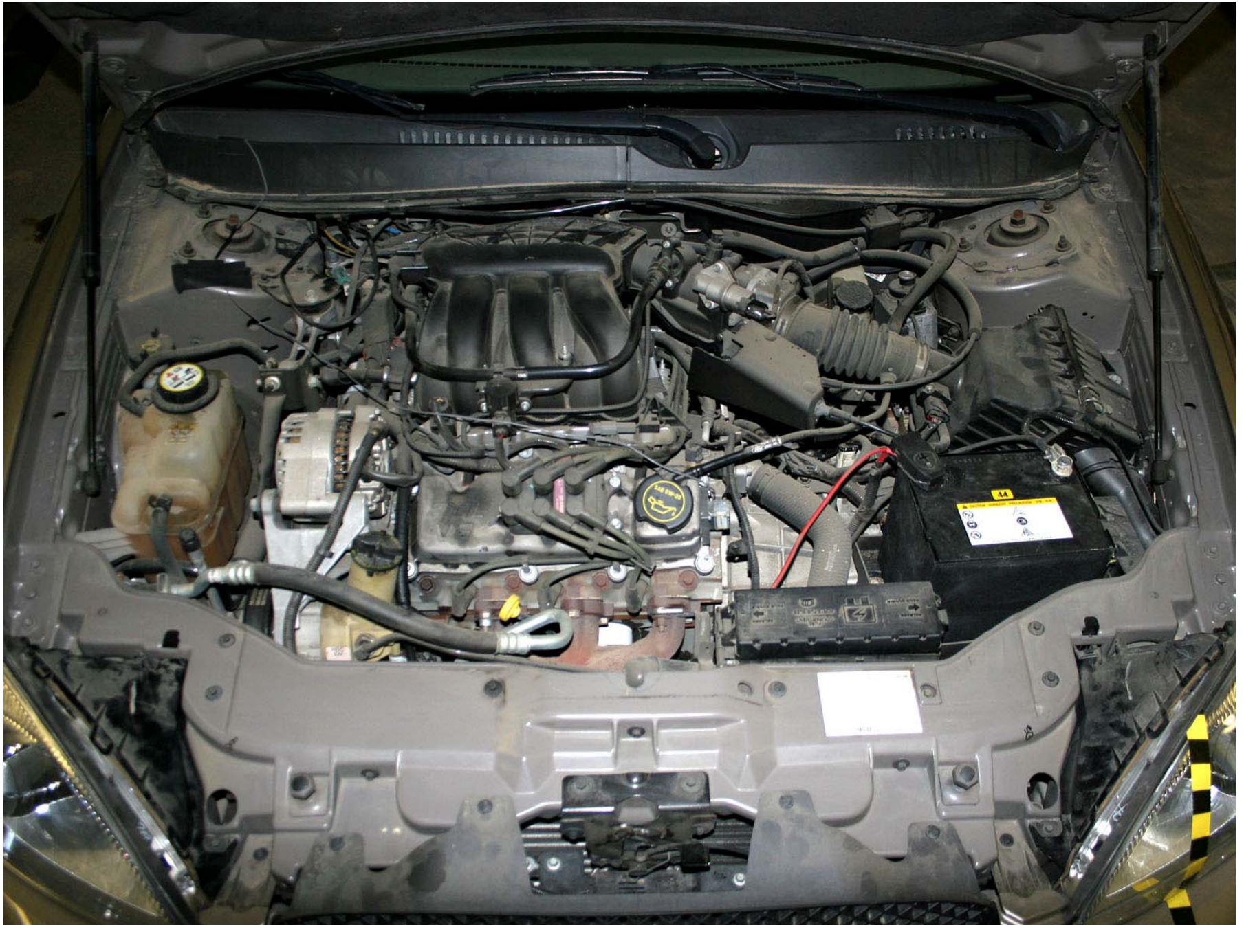
Figure A-47: Test Vehicle Pre-Test Engine Compartment View
