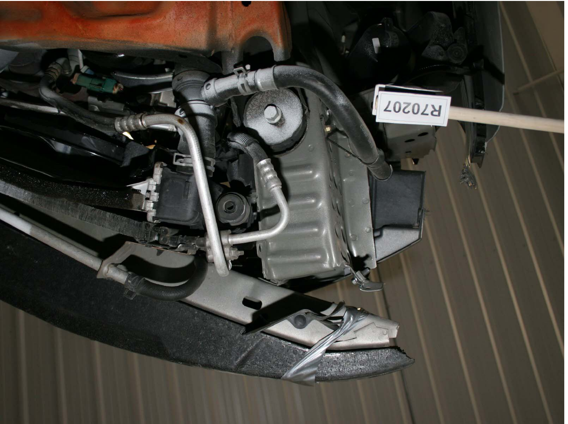
Figure A-198: Test Vehicle Post-Test Right Side Crush Initiators
