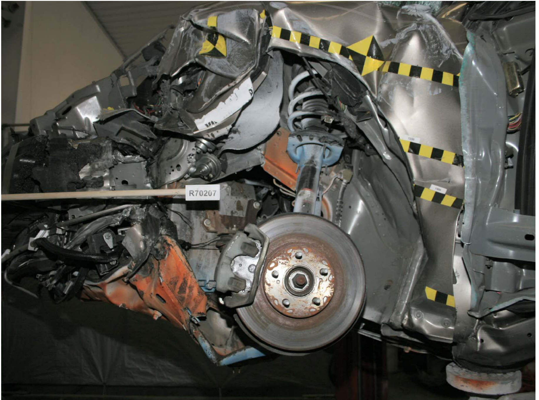
Figure A-138: Test Vehicle Post-Test Left Front Wheel Well (Tire Off), Inner Fender Removed
