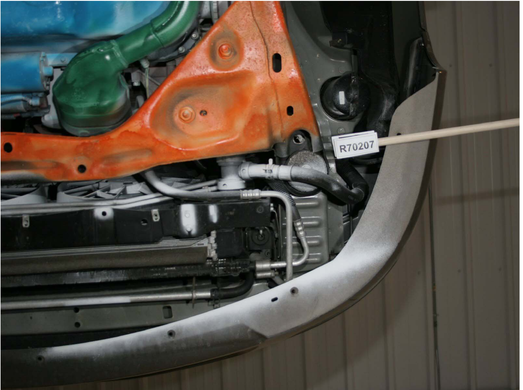
Figure A-197: Test Vehicle Pre-Test Right Side Crush Initiators
