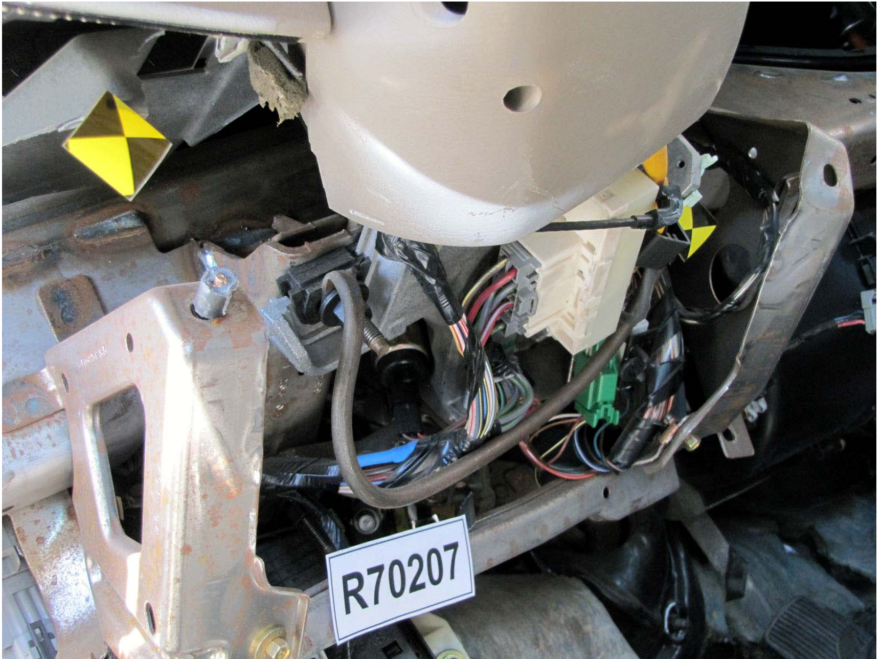
Figure A-245: Test Vehicle Post-Test Driver's Side Knee Bolster \frac{3}{4} View
