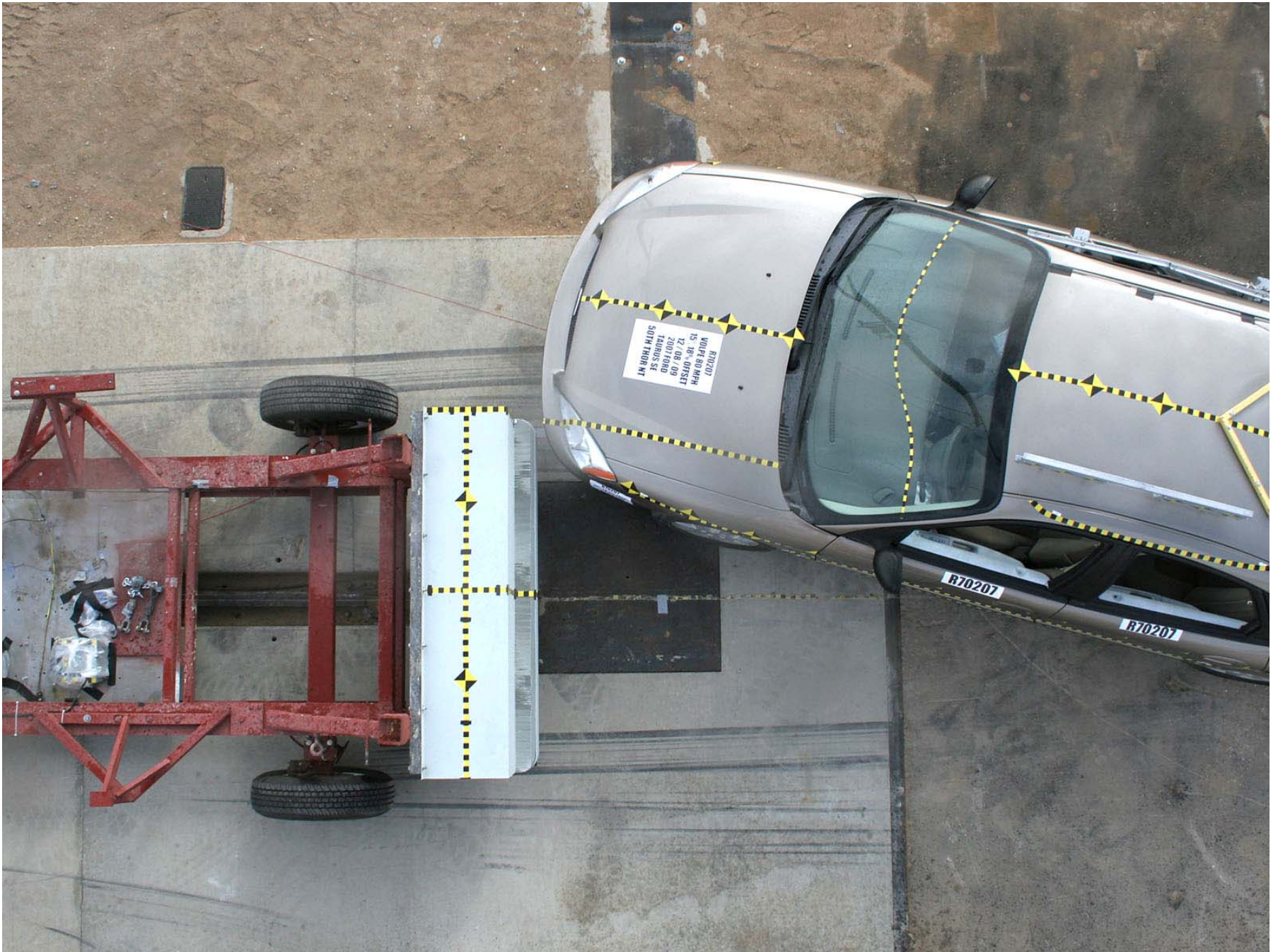
Figure A-21: Test Vehicle Pre-Test Overhead View
