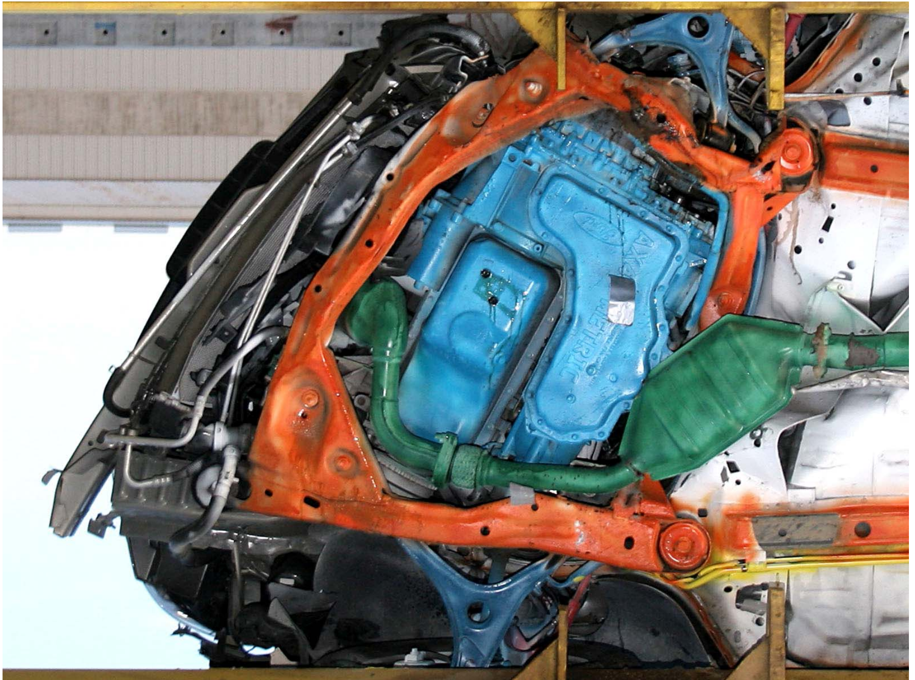
Figure A-206: Test Vehicle Post-Test Front Underbody
