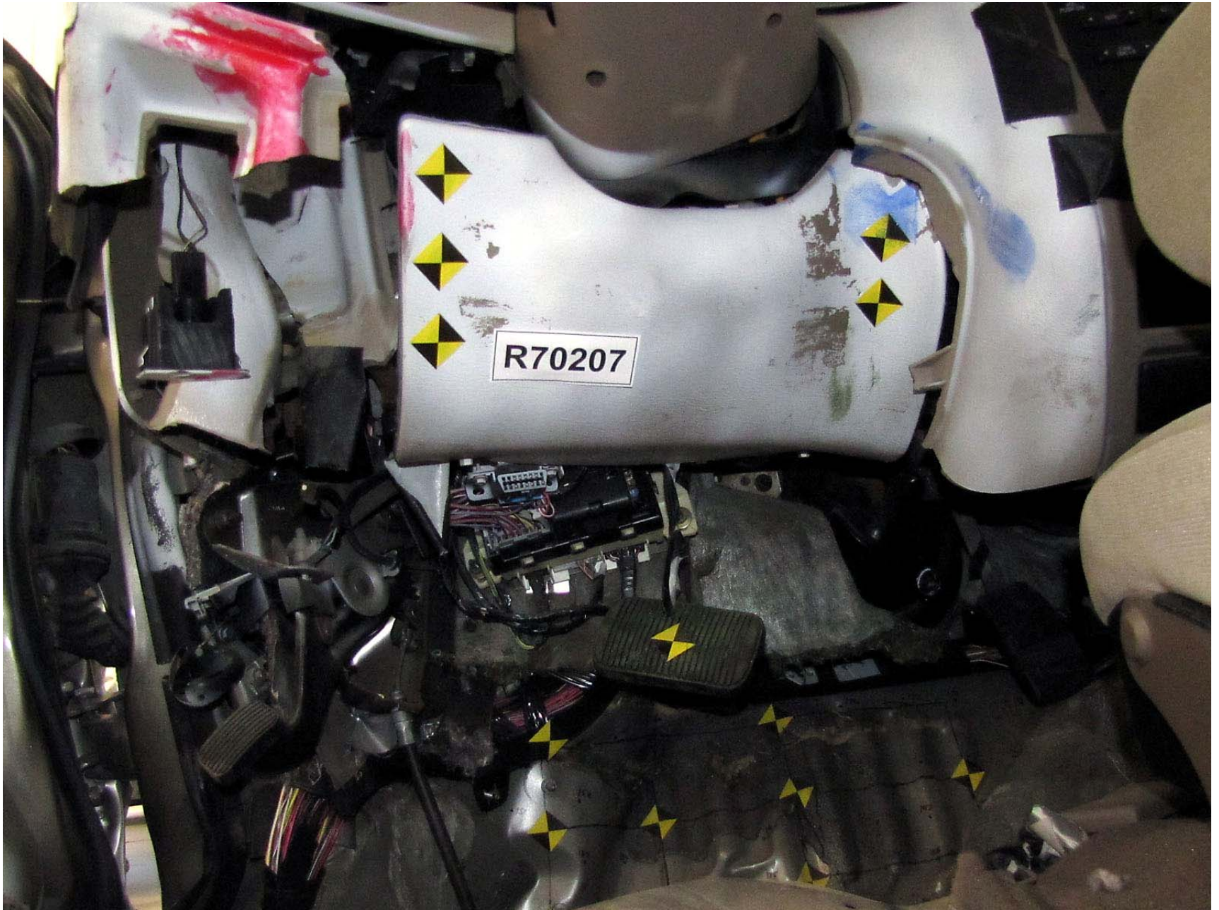
Figure A-246: Test Vehicle Post-Test Driver's Side Knee Bolster
