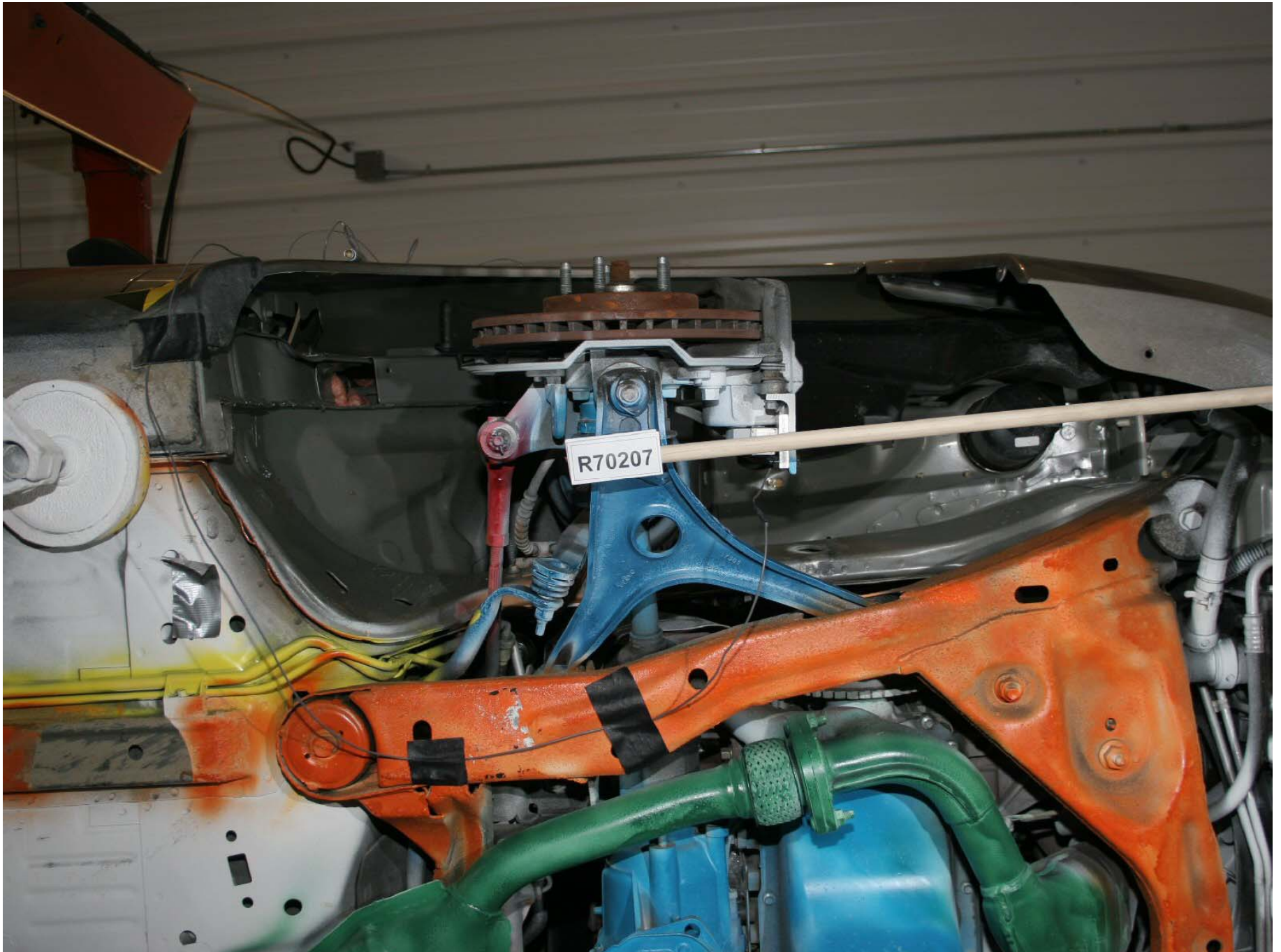
Figure A-175: Test Vehicle Pre-Test Right Inner Fender Well View
