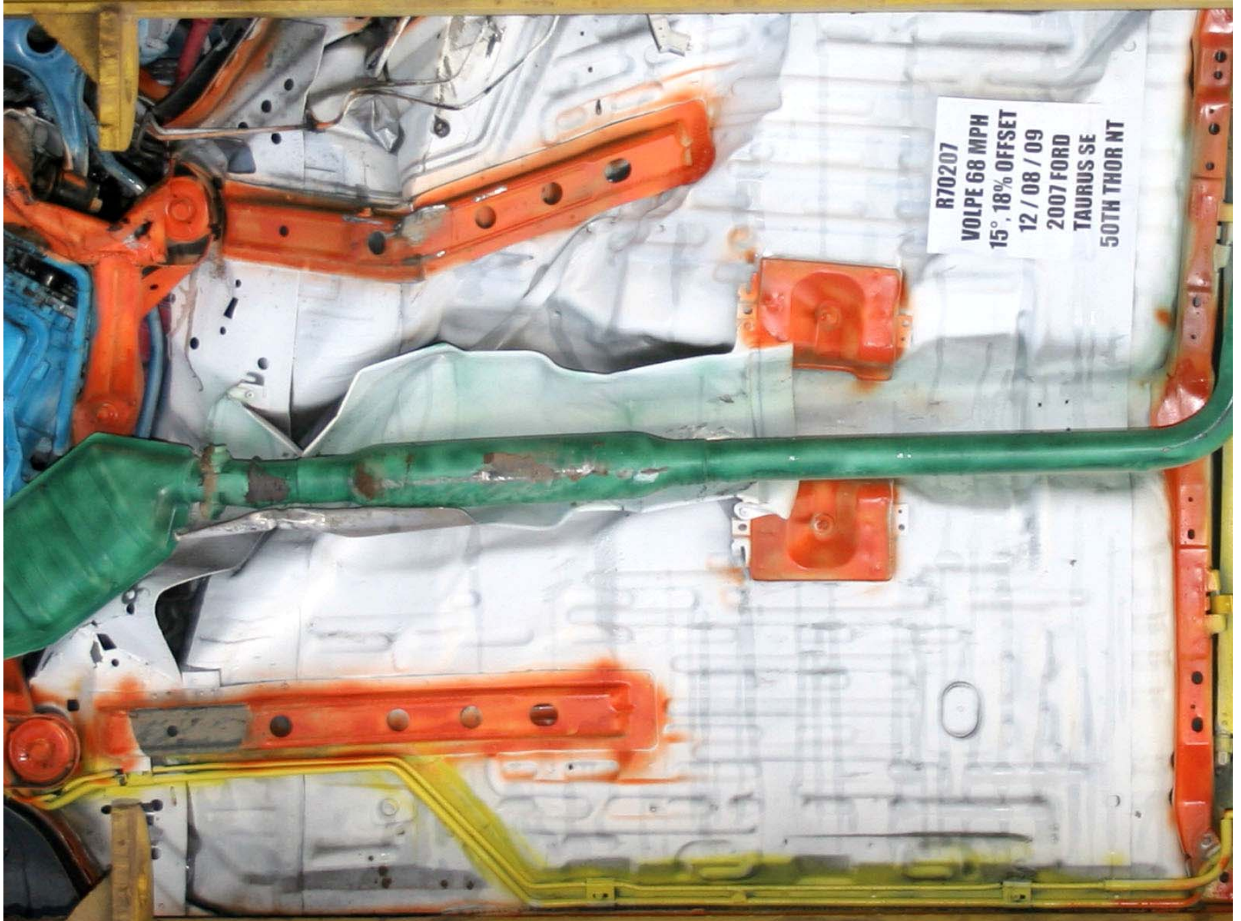
Figure A-208: Test Vehicle Post-Test Mid Underbody
