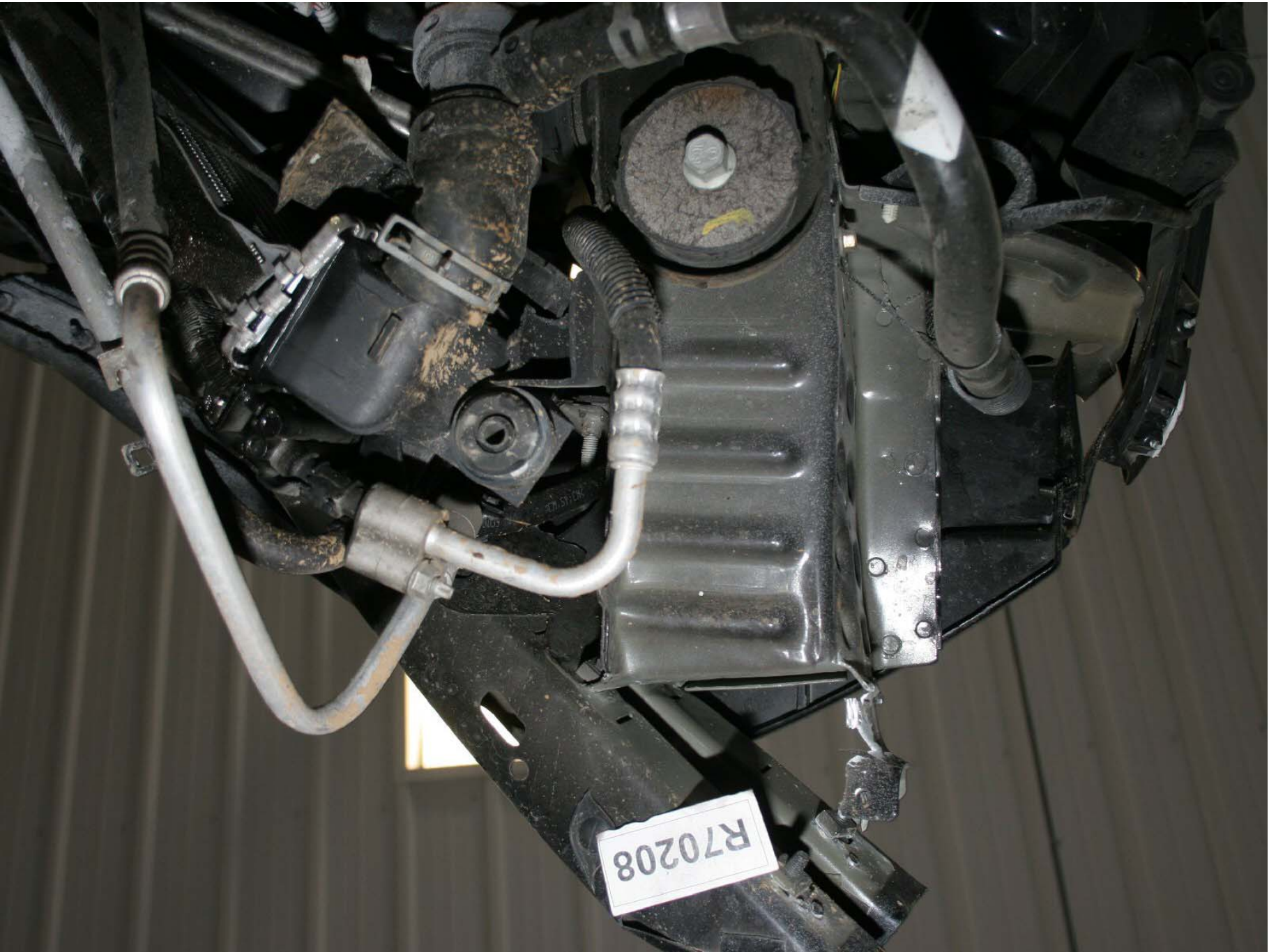
Figure A-197: Test Vehicle Post-Test Right Side Crush Initiators
