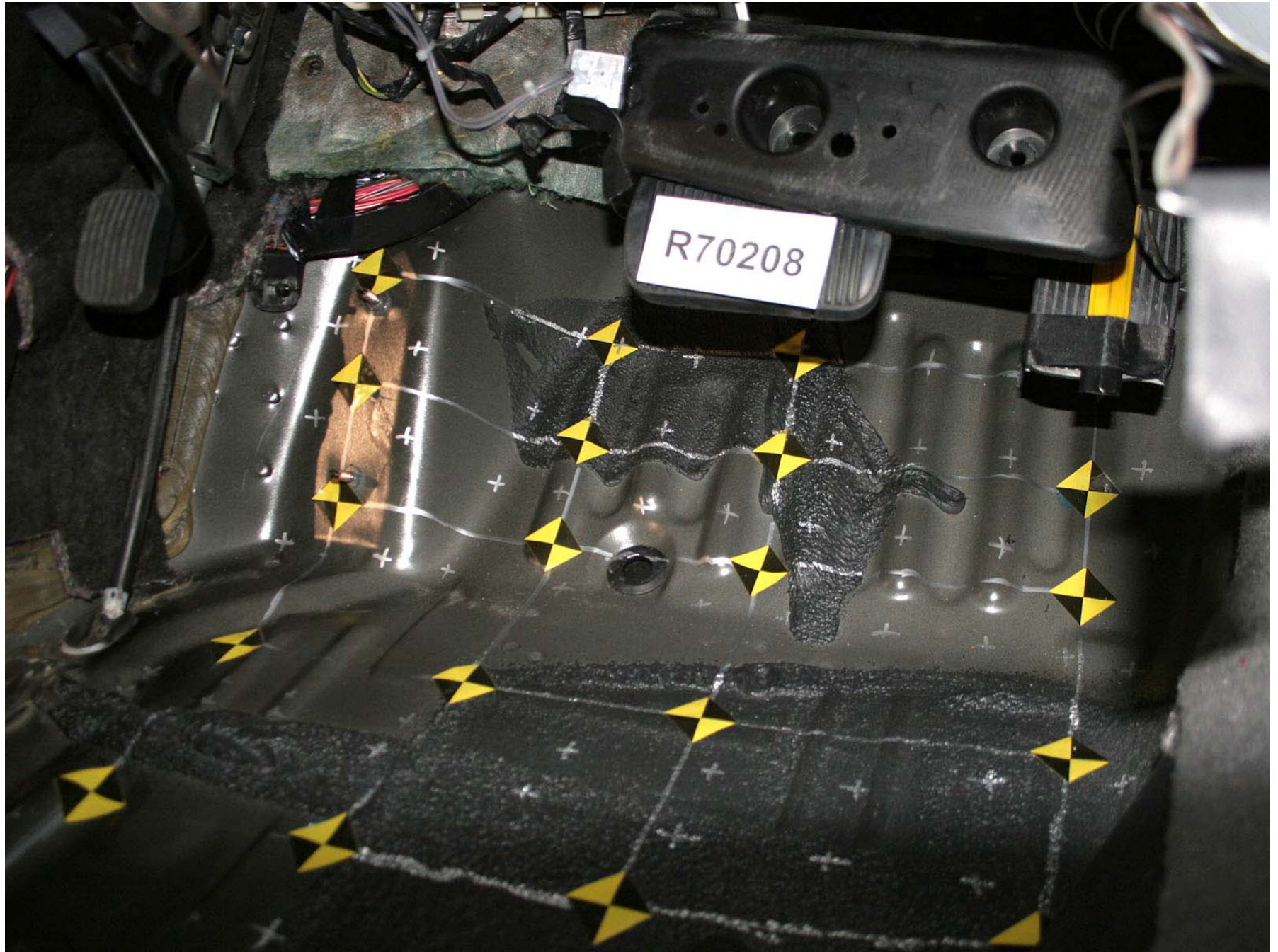
Figure A-289: Test Vehicle Pre-Test Driver Floorpan Right \frac{3}{4} View, Seat Cushion Height
