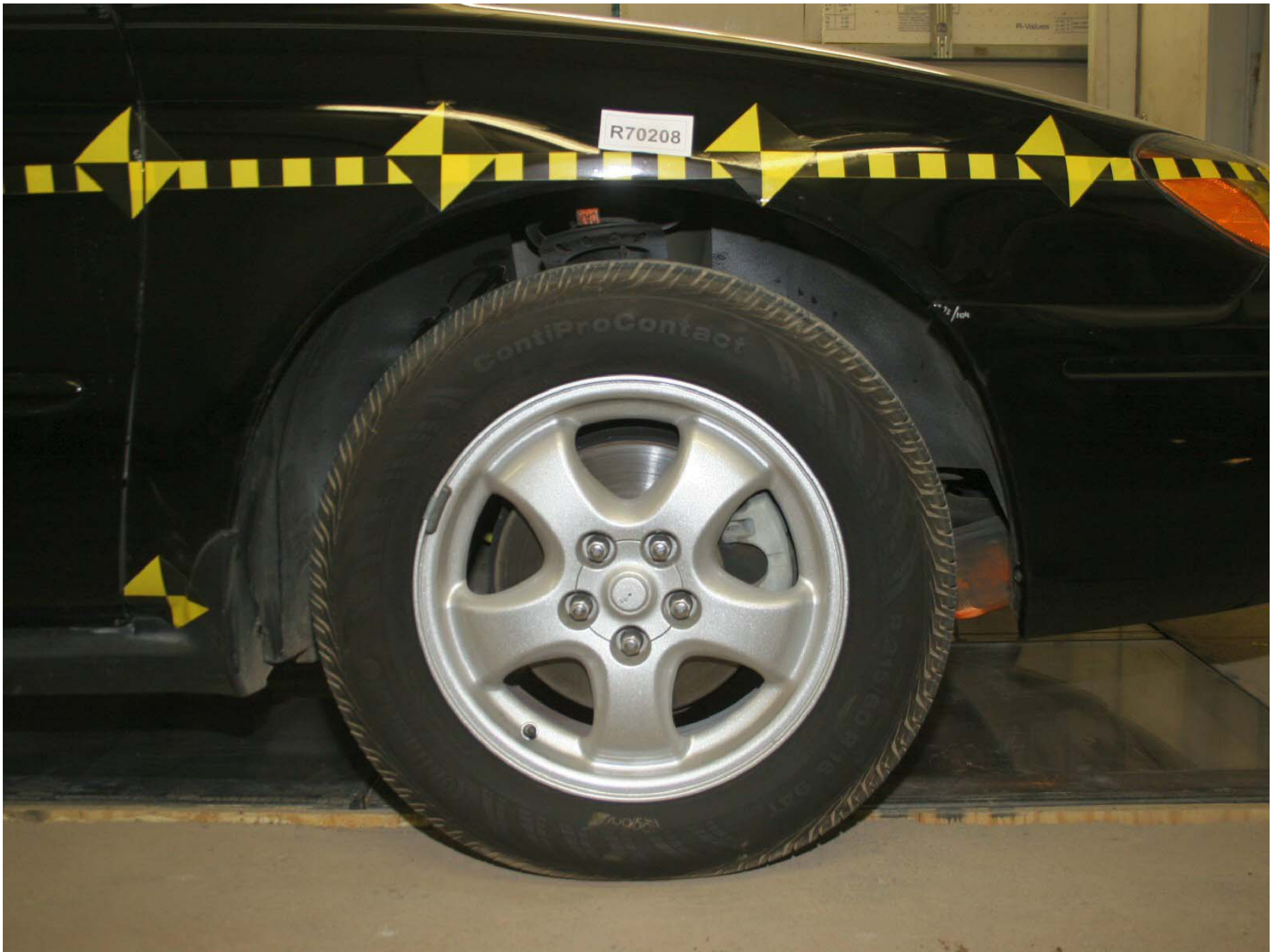
Figure A-168: Test Vehicle Pre-Test Right Front Wheel Well (Tire On)
