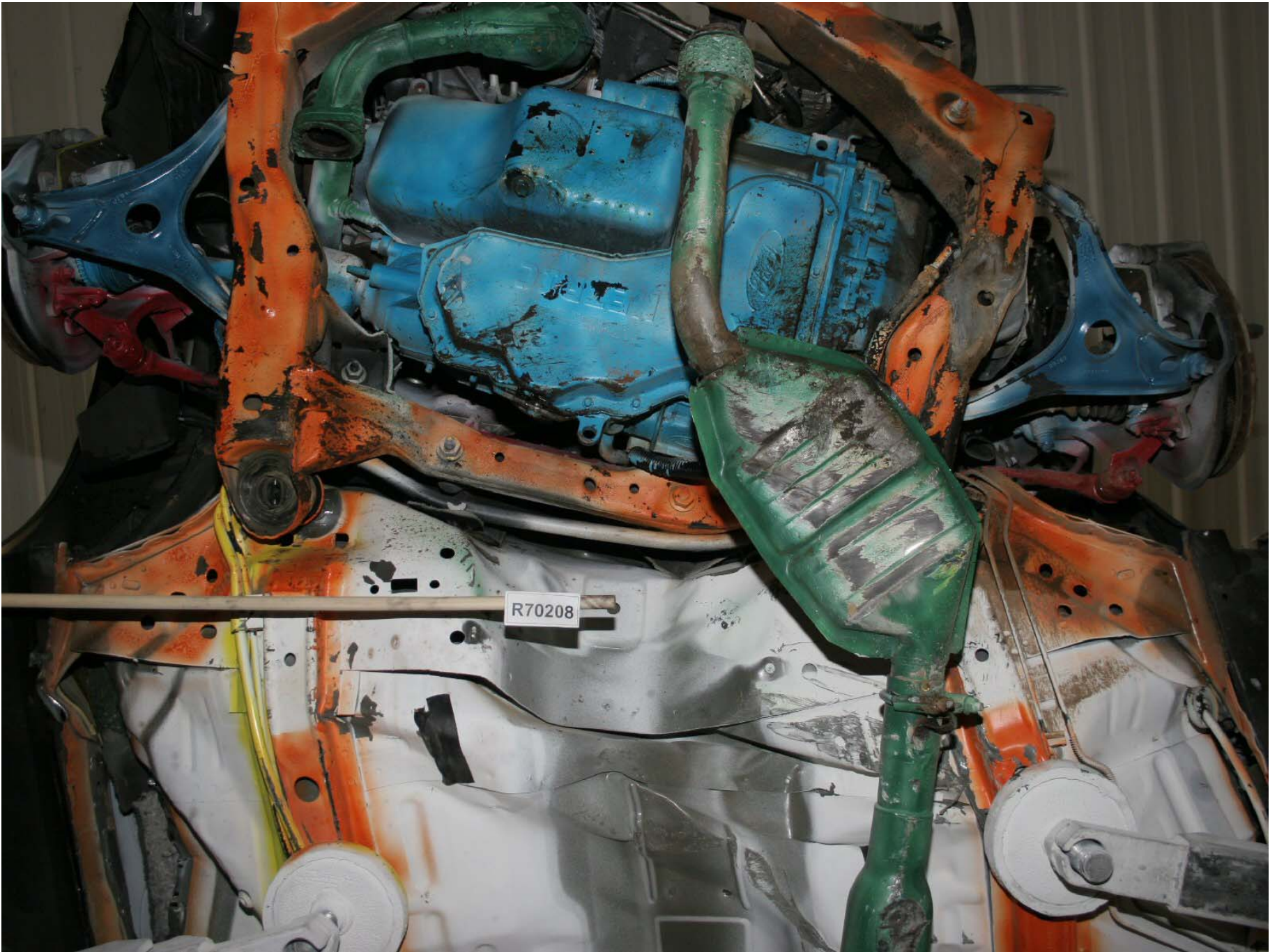
Figure A-211: Test Vehicle Post-Test Steering Rack and Sway Bar View
