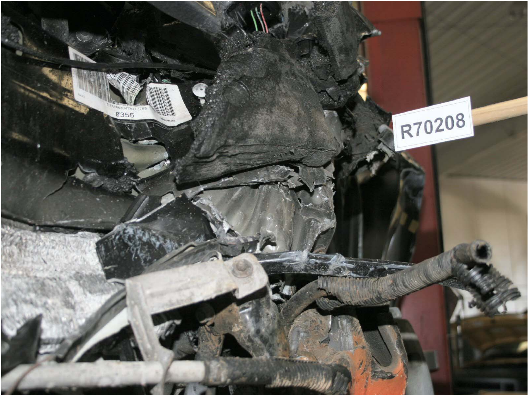
Figure A-159: Test Vehicle Post-Test Left Side Crush Initiators
