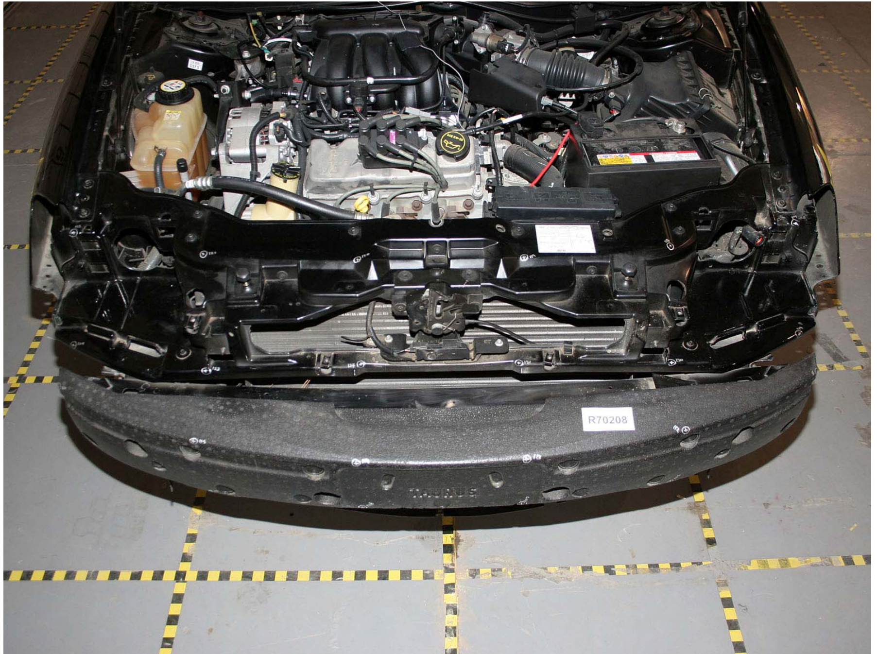
Figure A-307: Test Vehicle Pre-Test Structural Member Crush Measurement (Hood Open)
