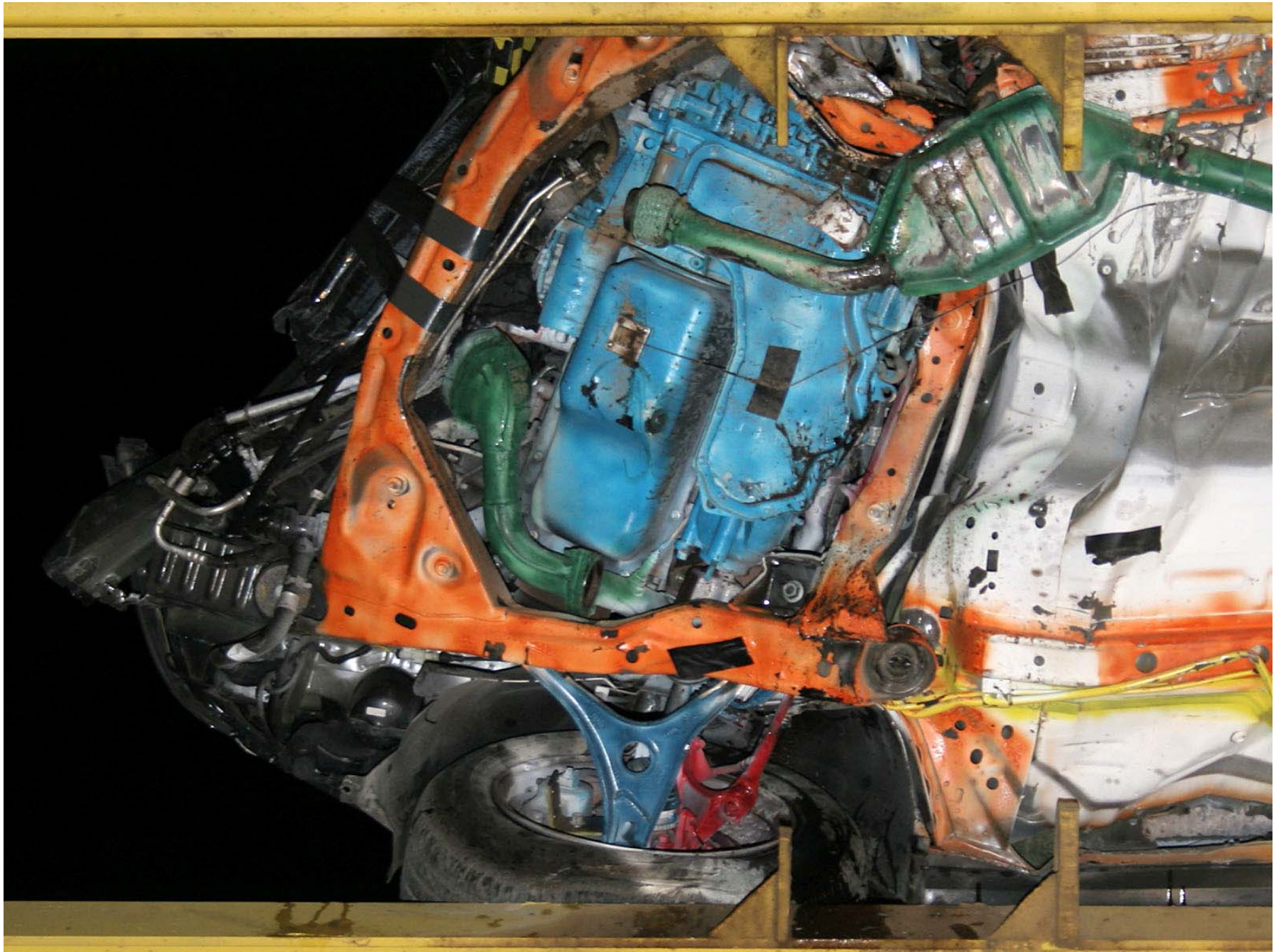
Figure A-205: Test Vehicle Post-Test Front Underbody
