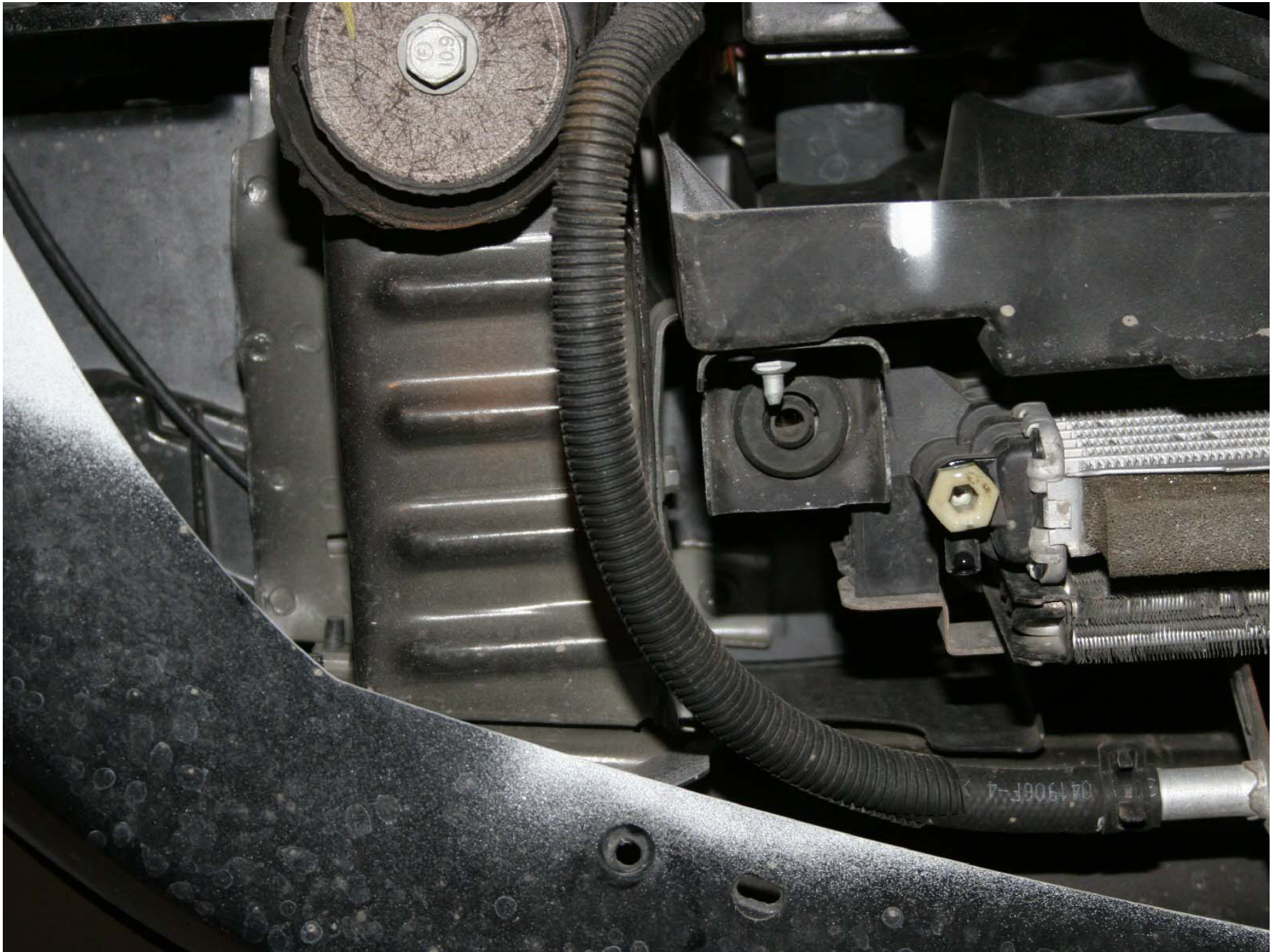
Figure A-160: Test Vehicle Pre-Test Left Side Crush Initiators
