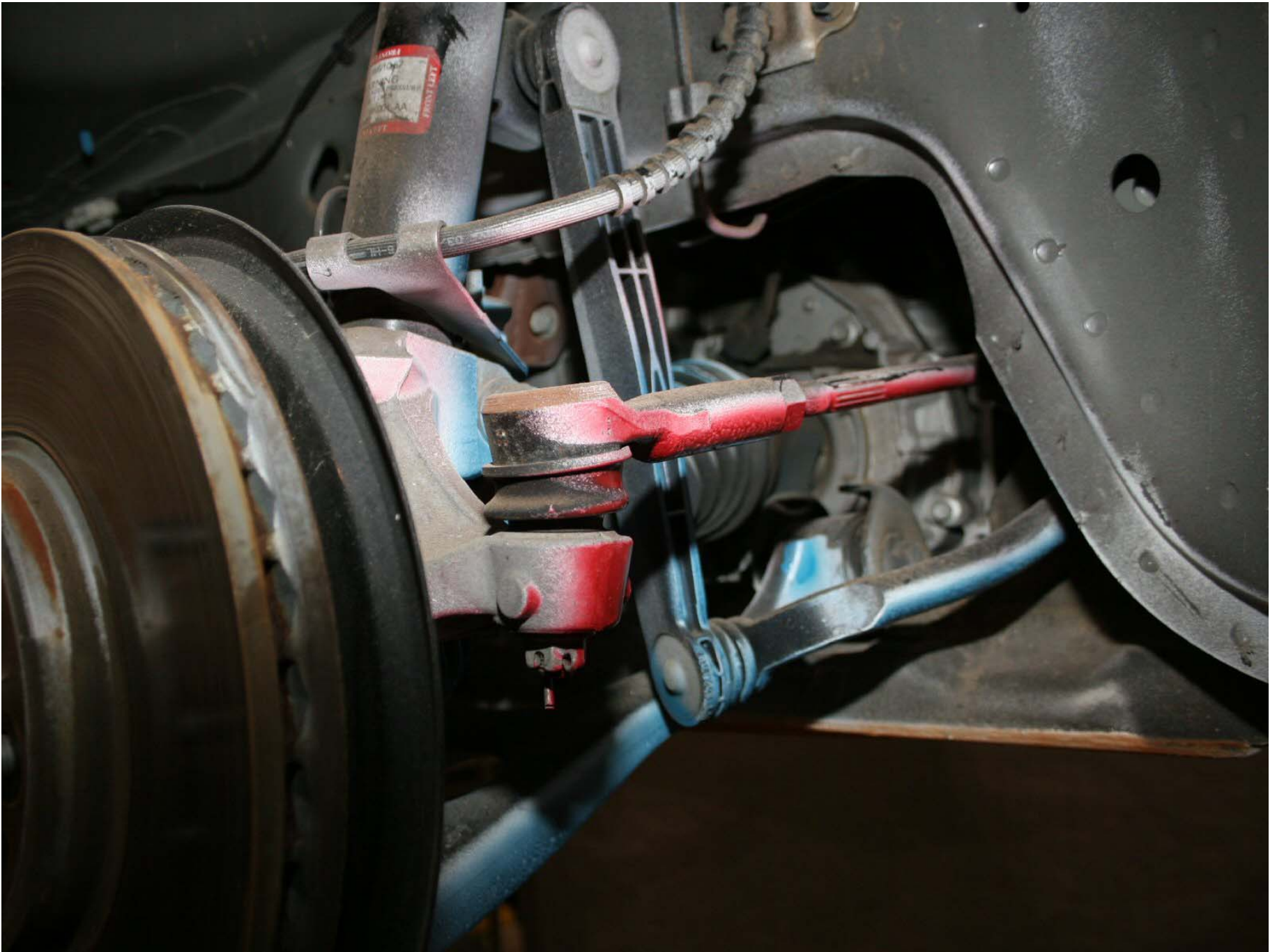
Figure A-152: Test Vehicle Pre-Test Left Side Tie Rod and Sway Bar Attachments Points
