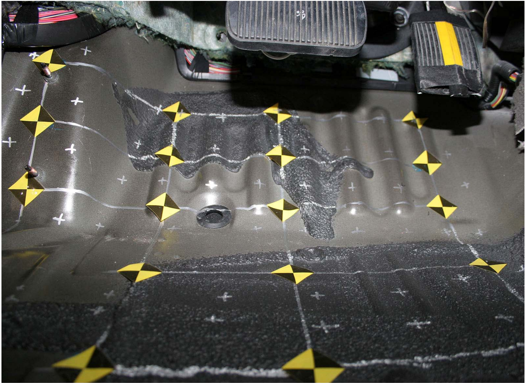
Figure A-287: Test Vehicle Pre-Test Driver Floorpan, Sill Height
