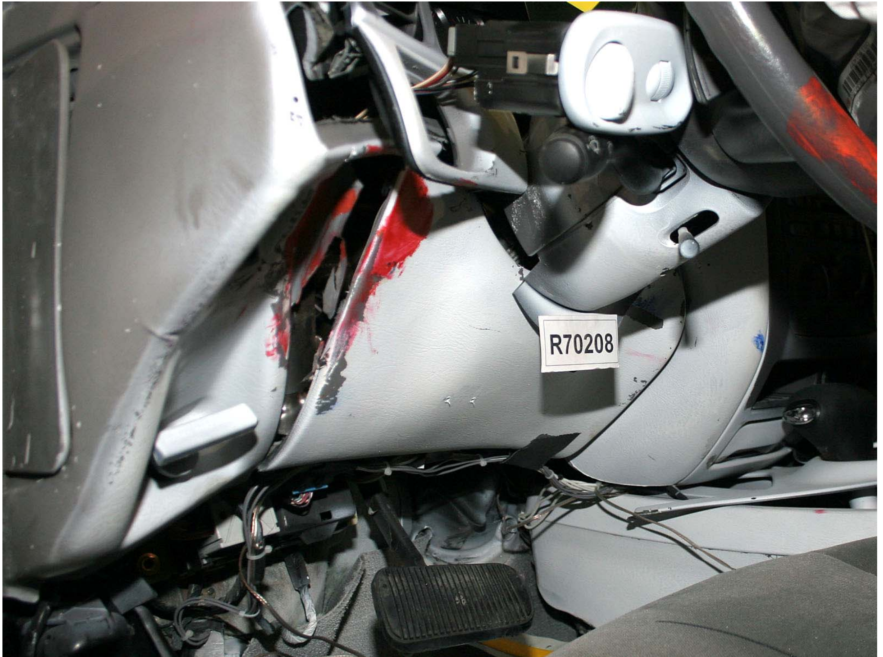
Figure A-242: Test Vehicle Post-Test Driver's Side Knee Bolster
