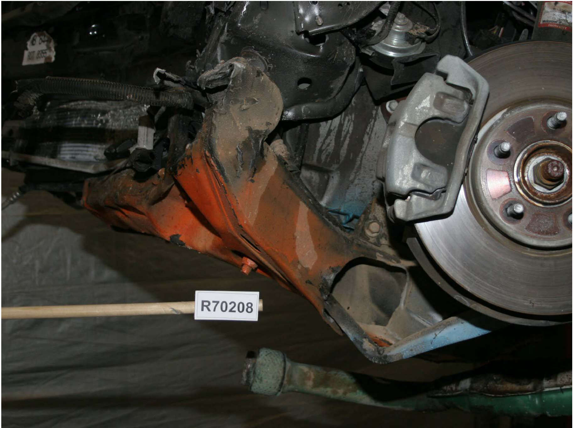
Figure A-147: Test Vehicle Post-Test Left Front Frame Rail View
