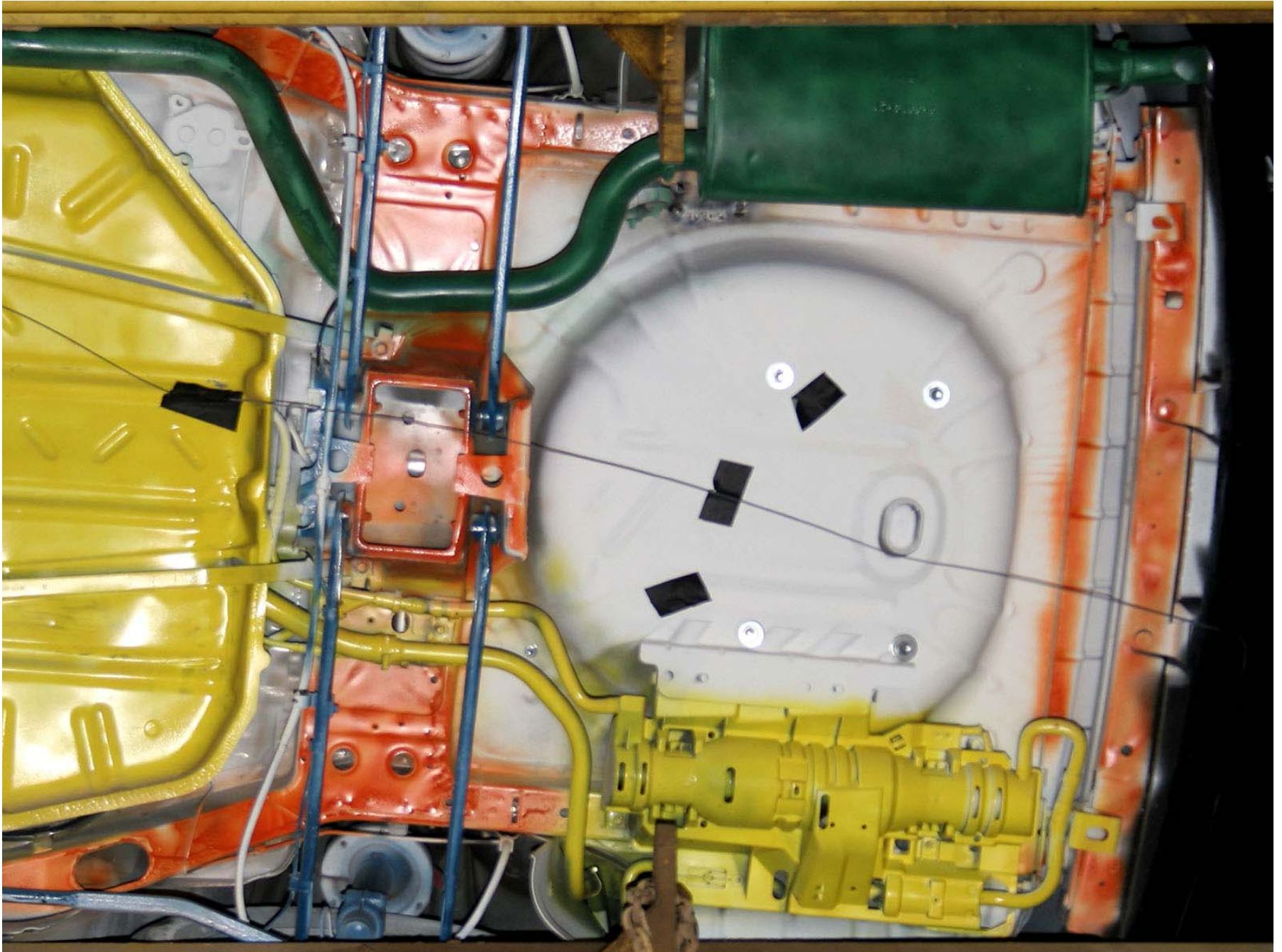
Figure A-209: Test Vehicle Post-Test Rear Underbody
