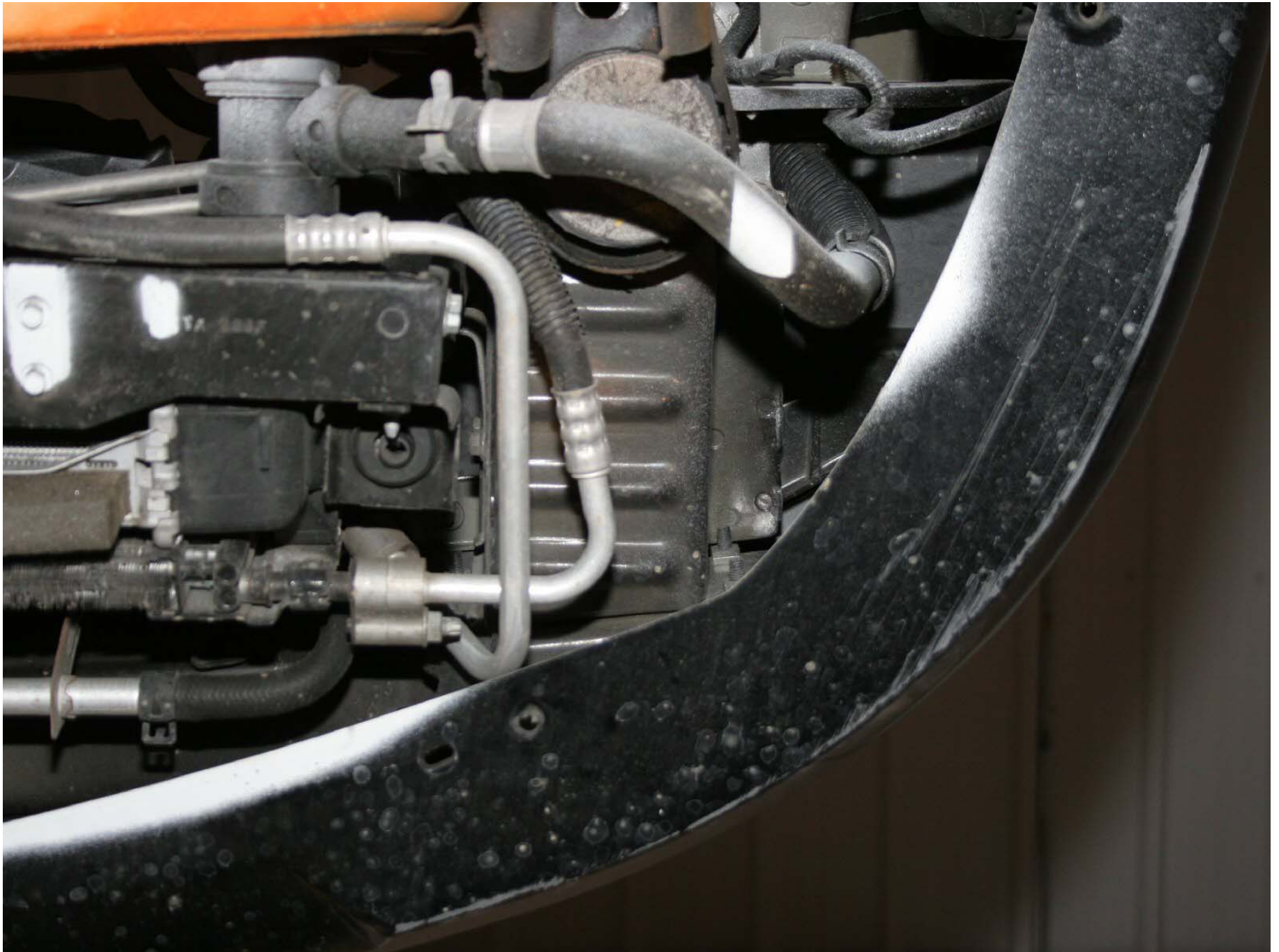
Figure A-196: Test Vehicle Pre-Test Right Side Crush Initiators
