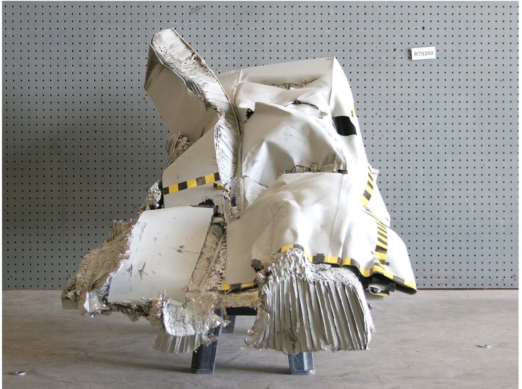
Figure A-322: Test Vehicle Post-Test Left Side View of Deformable Barrier
