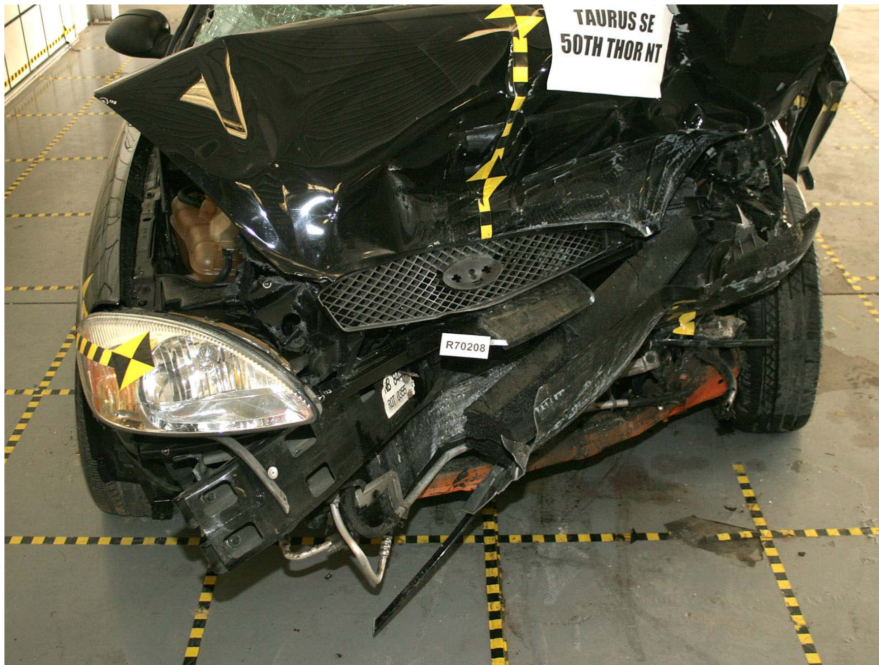
Figure A-304: Test Vehicle Post-Test Structural Member Crush Measurement (Hood Closed)
