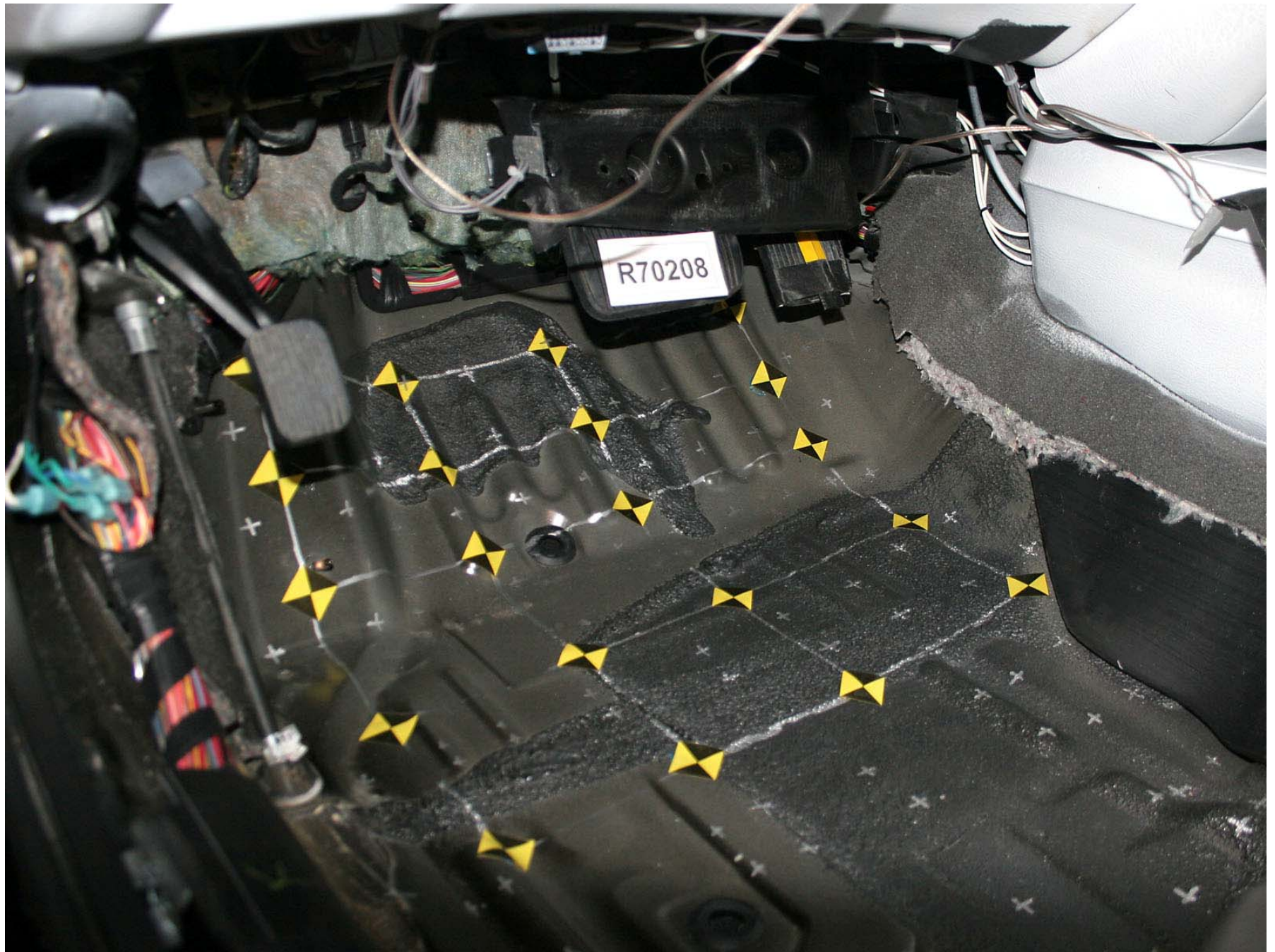
Figure A-279: Test Vehicle Pre-Test Driver Floorpan
