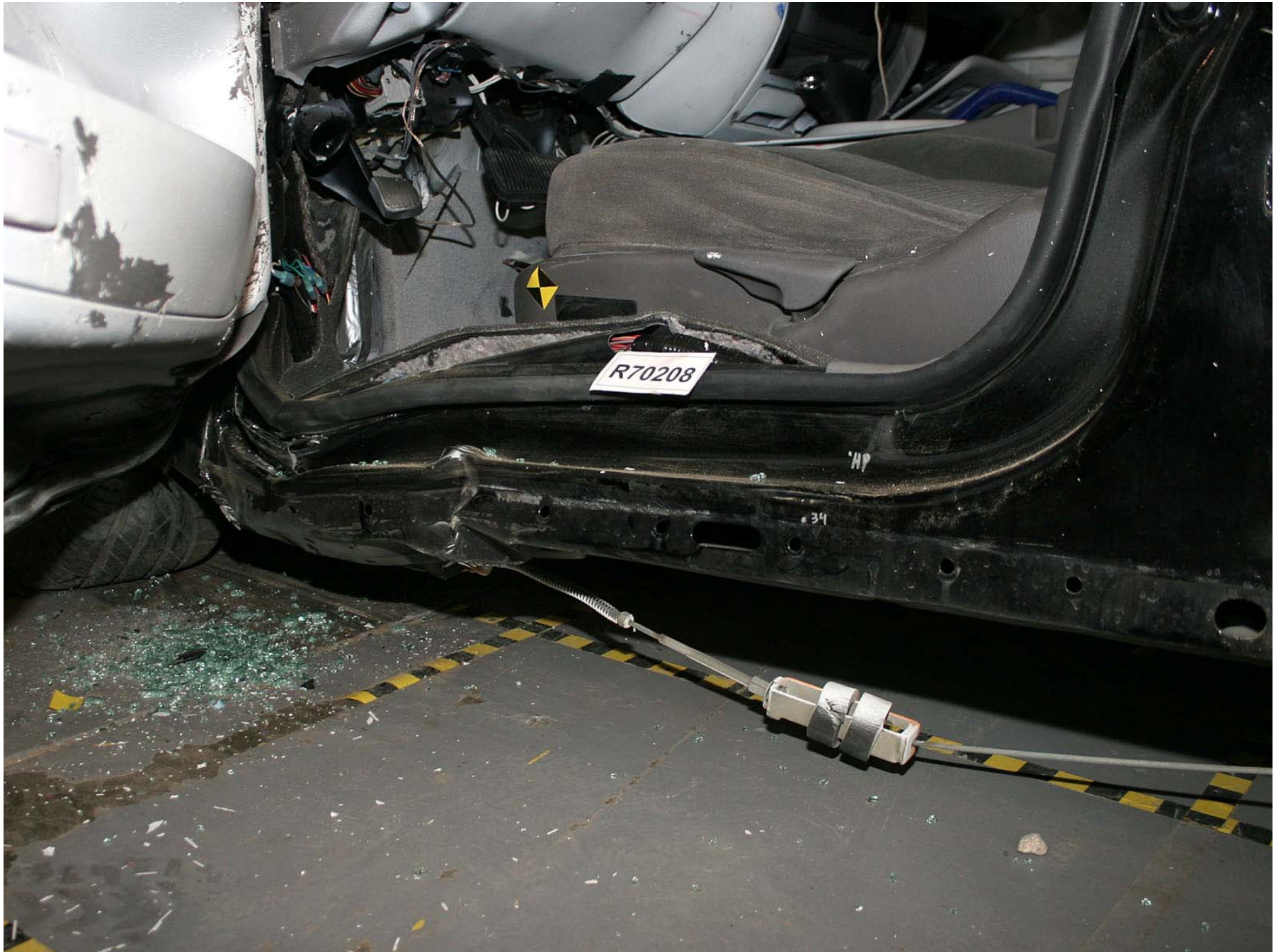
Figure A-70: Test Vehicle Post-Test Left Front Sill Rear \frac{3}{4} View, Door Open
