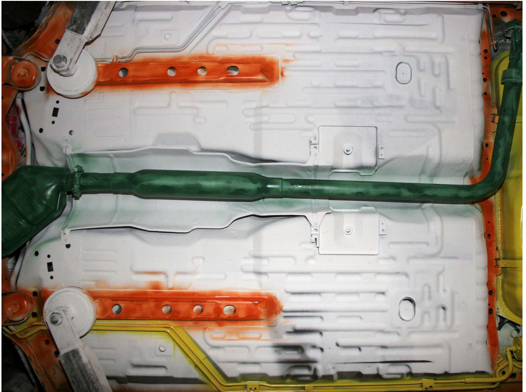
Figure A-206: Test Vehicle Pre-Test Mid Underbody
