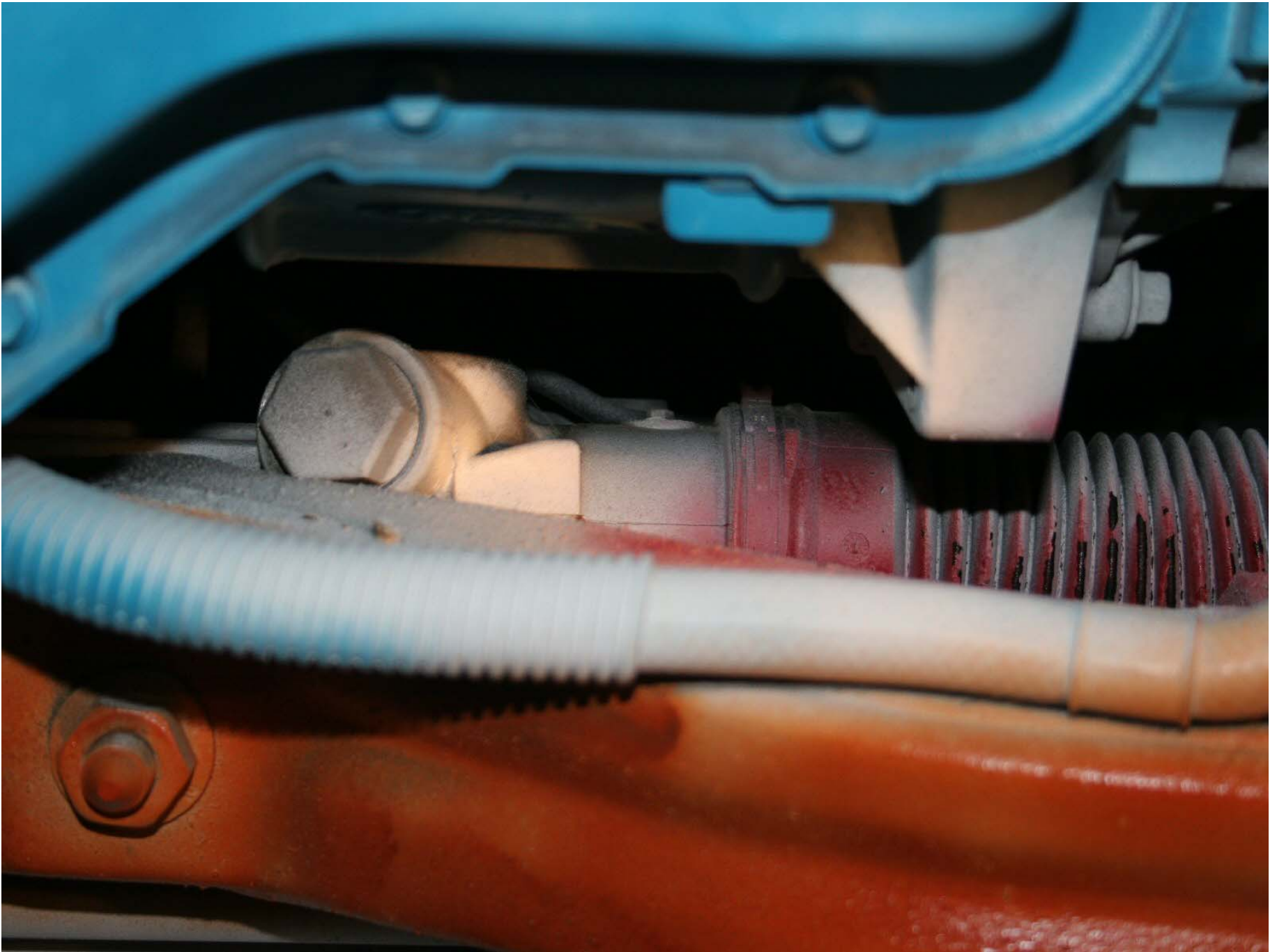
Figure A-214: Test Vehicle Pre-Test Steering Rack Right Side Mounting Bolt
