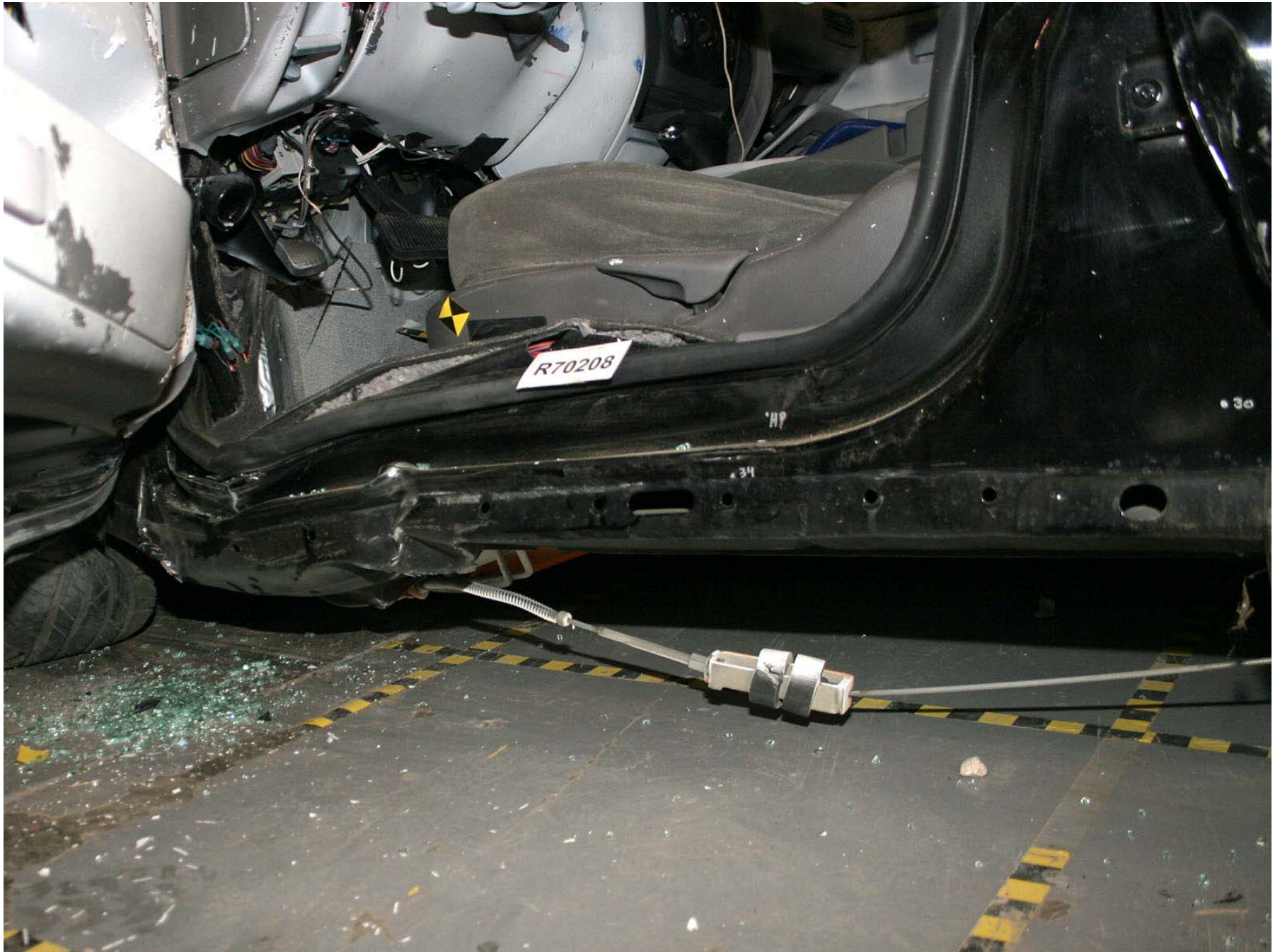
Figure A-66: Test Vehicle Post-Test Left Front Sill Side View, Door Open
