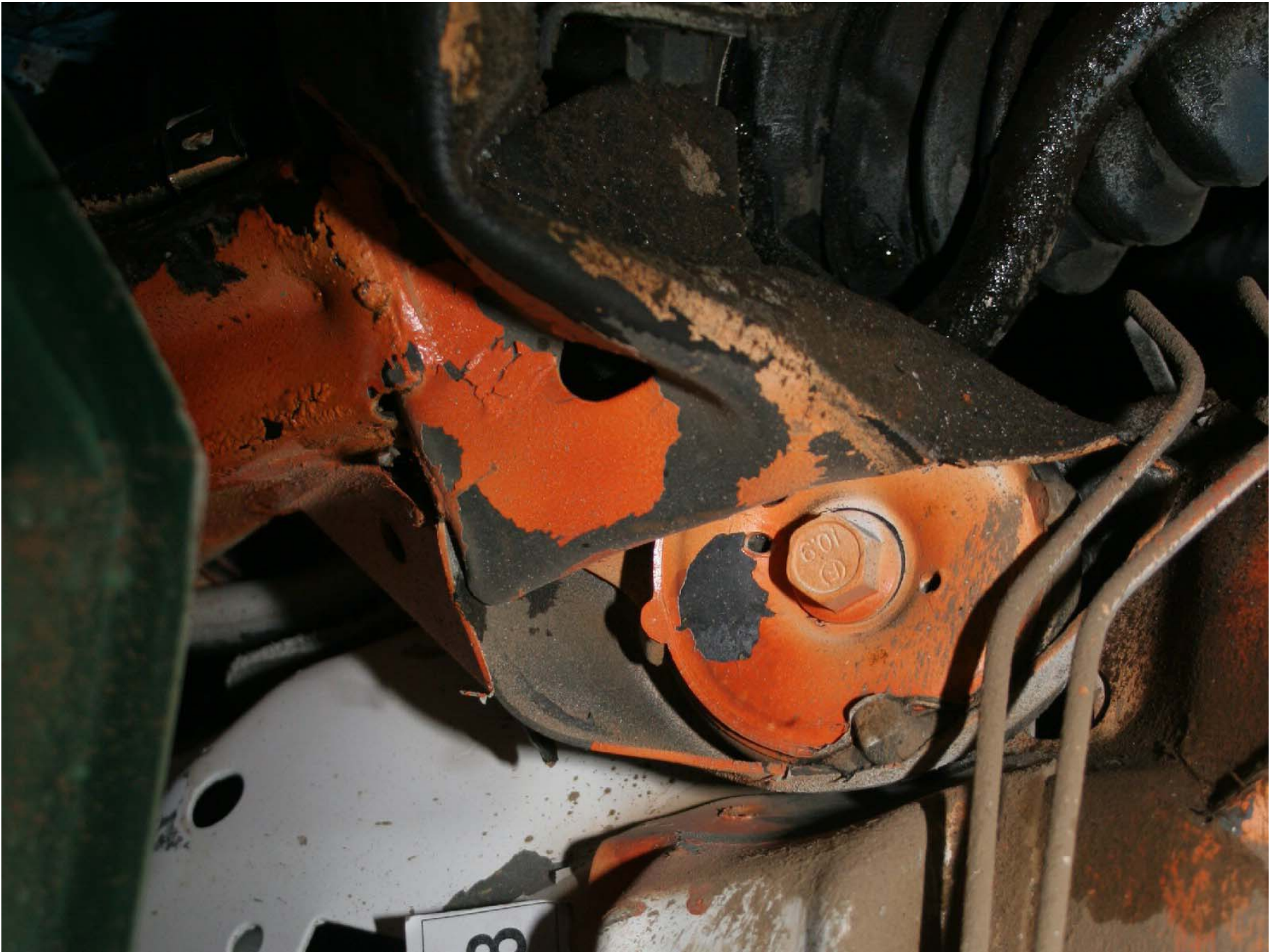
Figure A-167: Test Vehicle Post-Test Left Rear Sub-Frame Mounting Point
