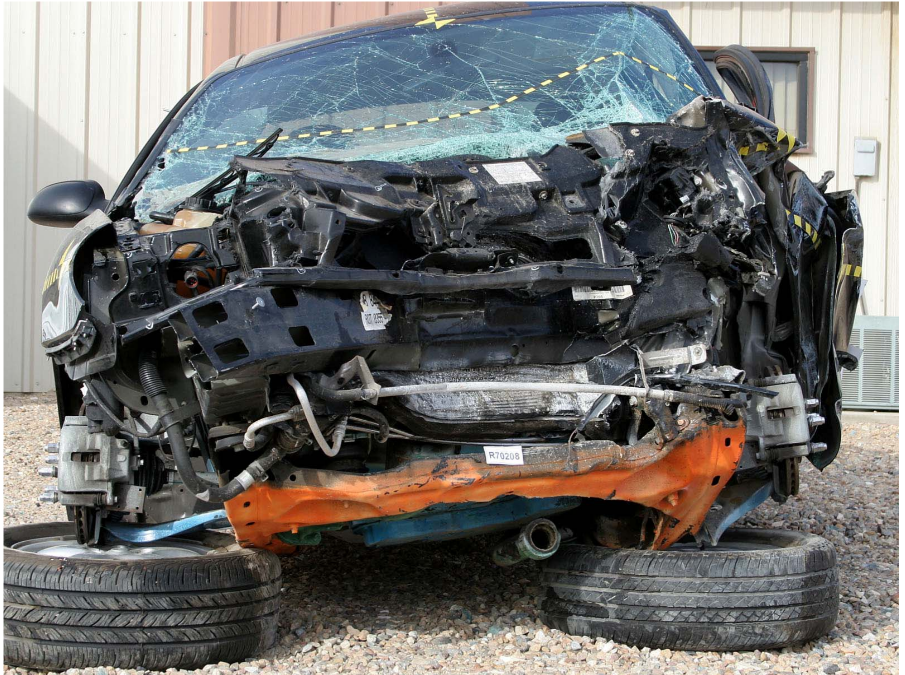
Figure A-310: Test Vehicle Post-Test Structural Member Crush Measurement (Hood Open)
