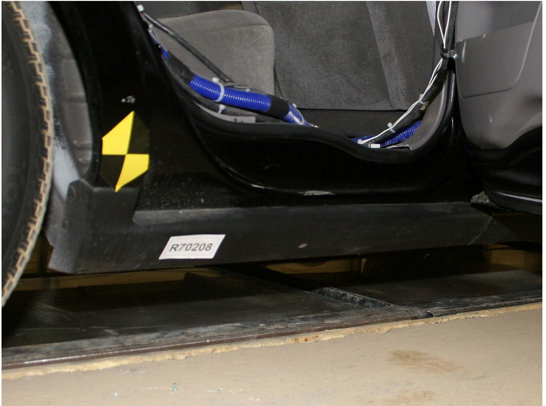
Figure A-105: Test Vehicle Pre-Test Right Rear Sill Rear \frac{3}{4} View, Door Open
