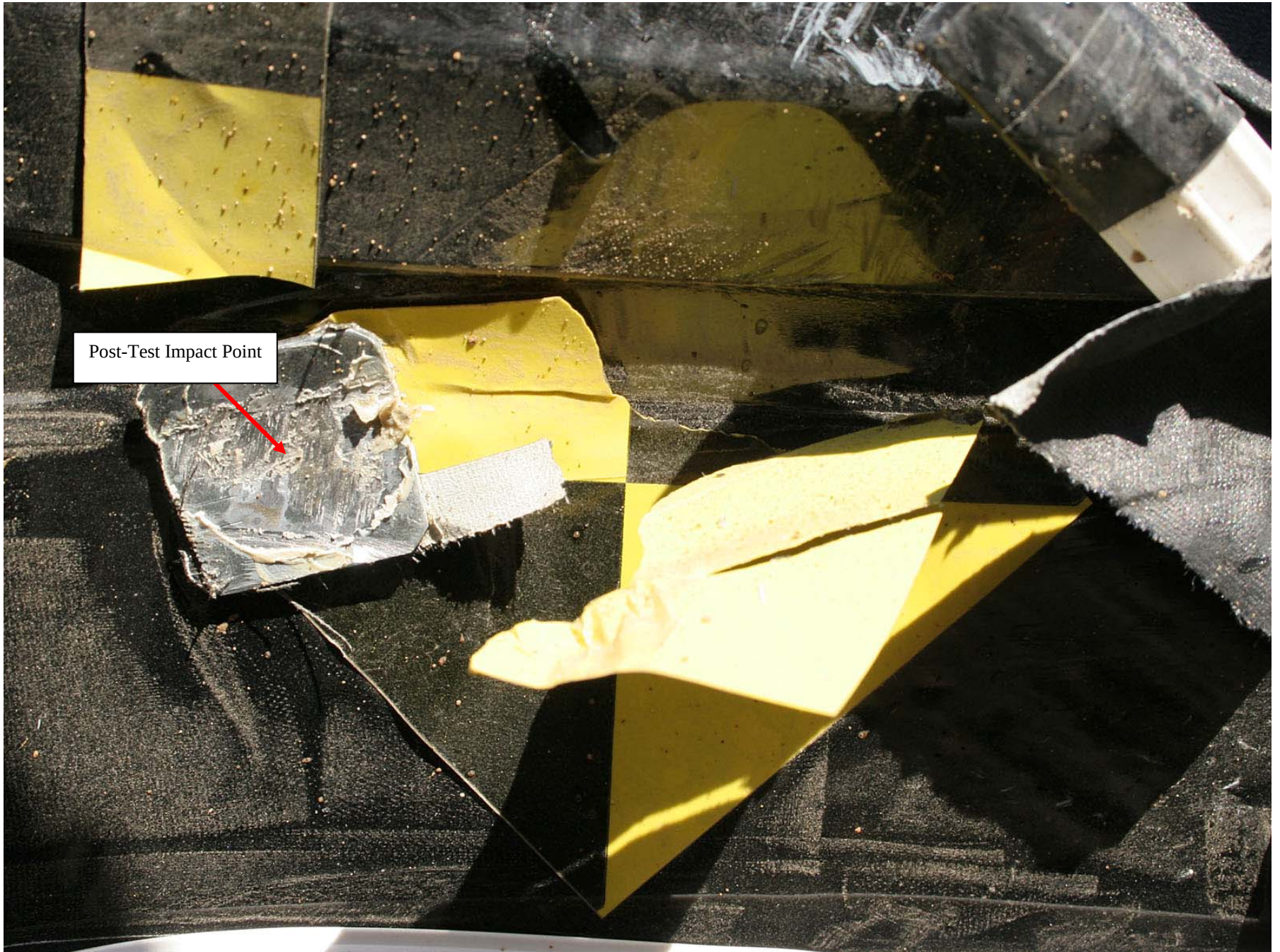
Figure A-26: Test Vehicle Post-Test Impact Point Marker
