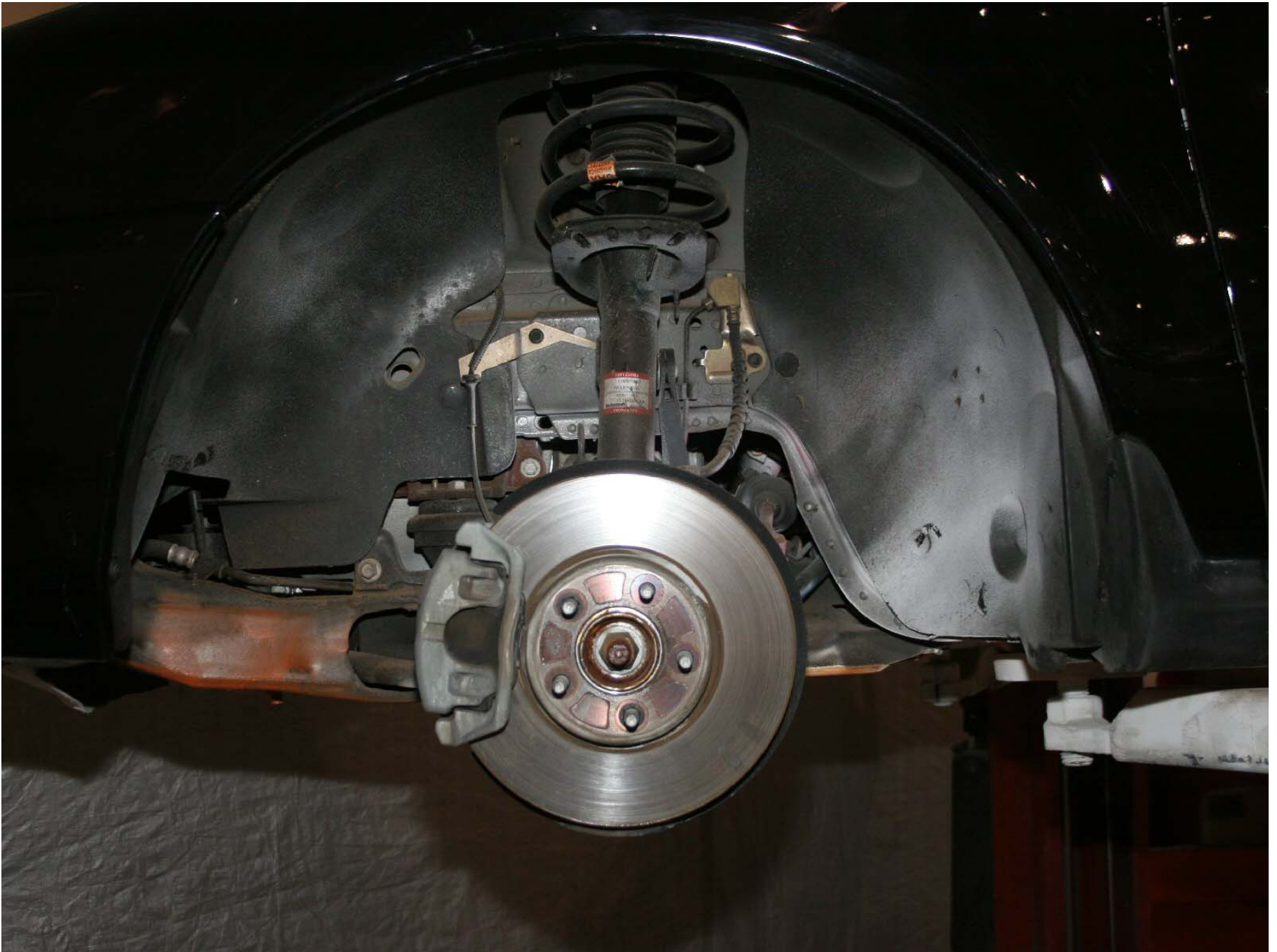
Figure A-134: Test Vehicle Pre-Test Left Front Wheel Well (Tire Off)
