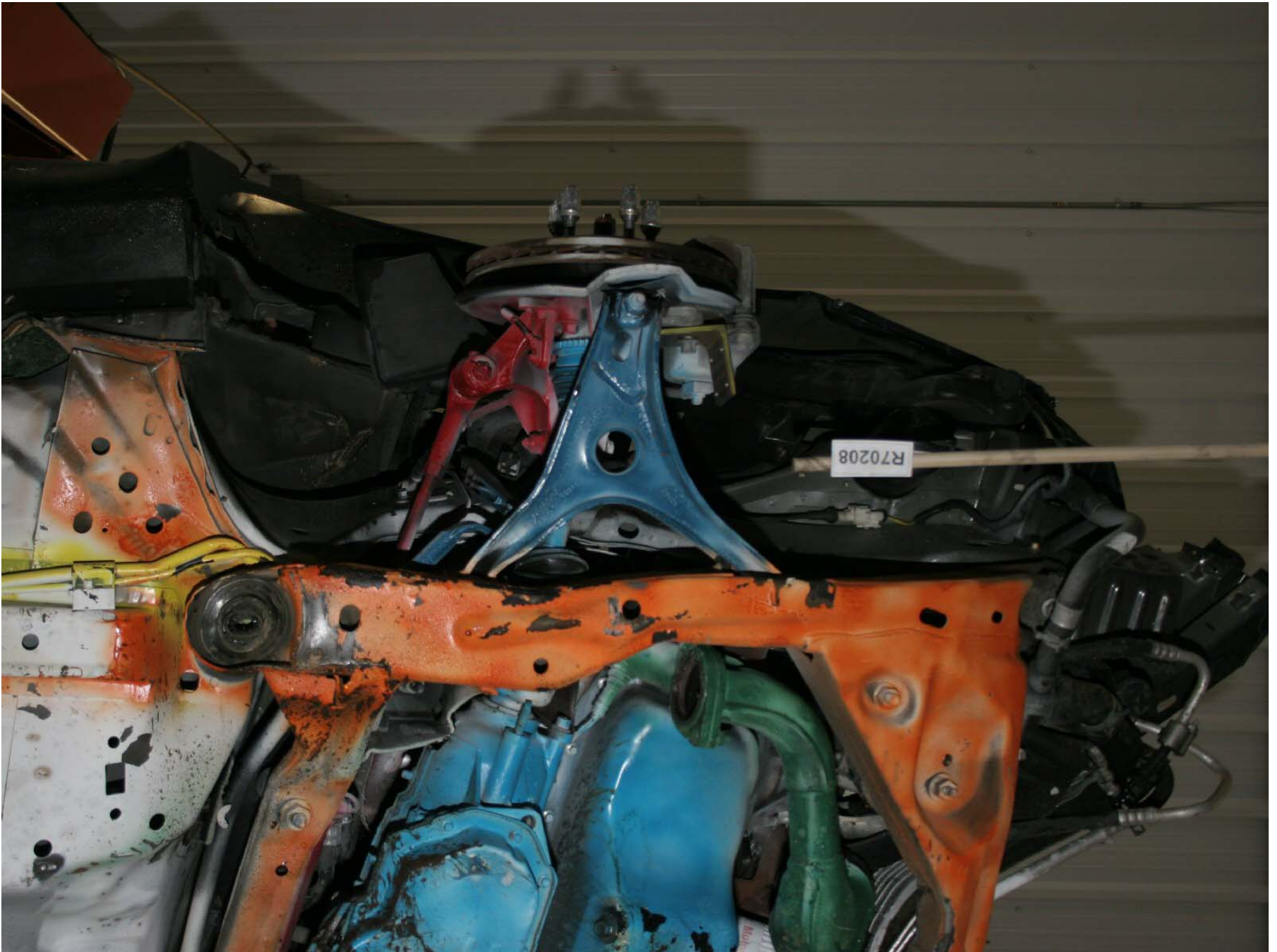
Figure A-175: Test Vehicle Post-Test Right Inner Fender Well View
