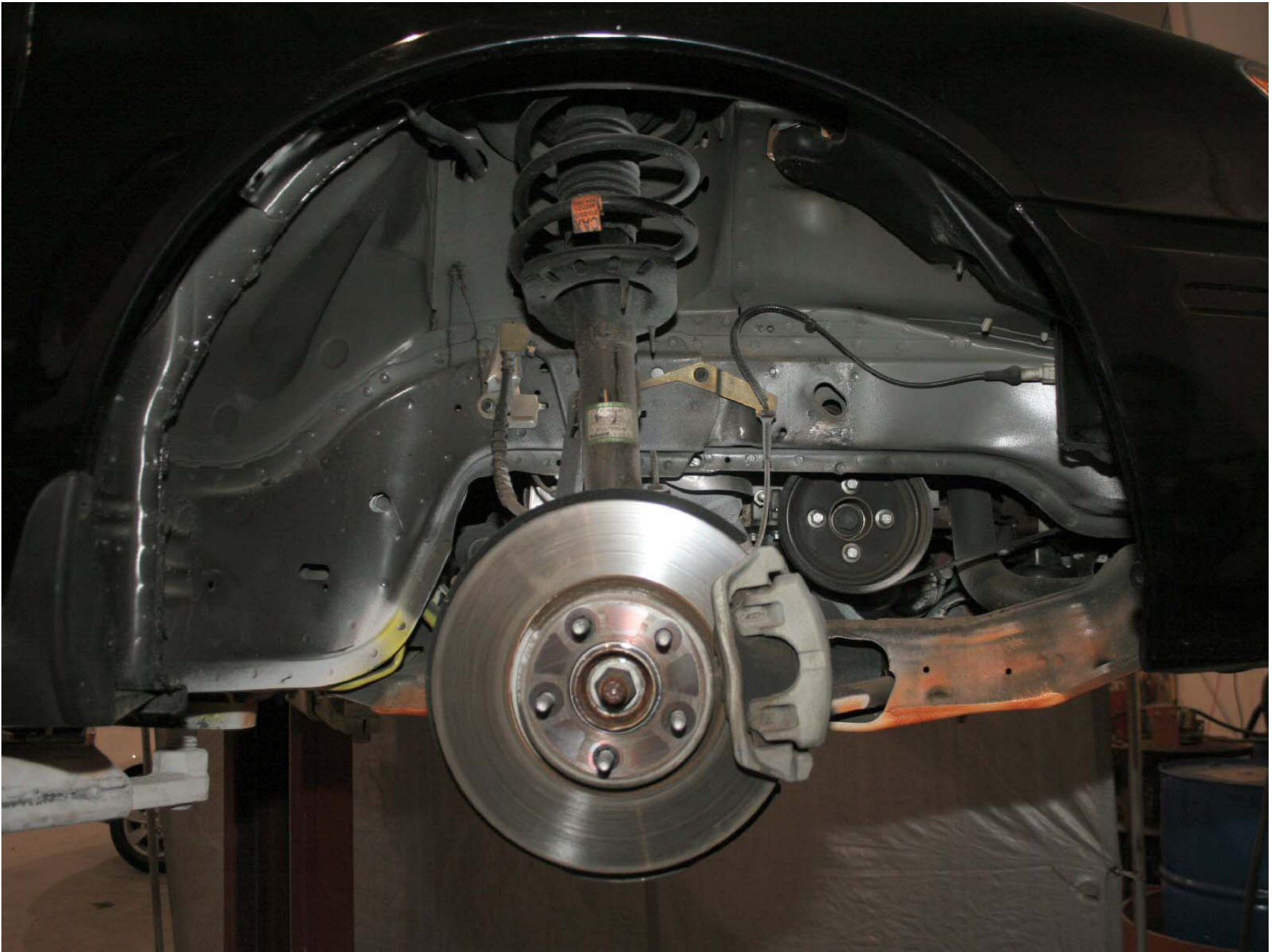
Figure A-172: Test Vehicle Pre-Test Right Front Wheel Well (Tire Off), Inner Fender Removed
