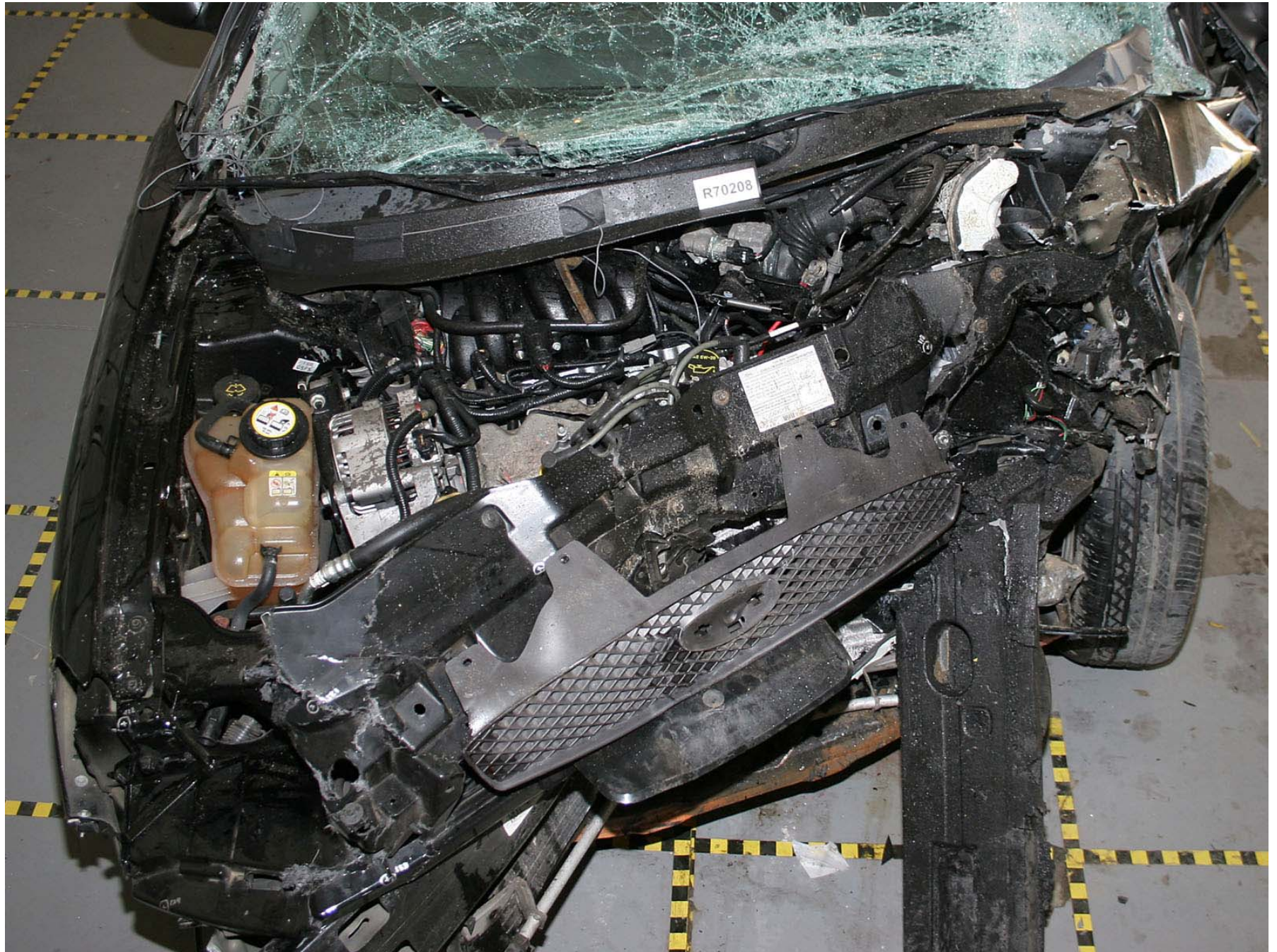
Figure A-308: Test Vehicle Post-Test Structural Member Crush Measurement (Hood Open)
