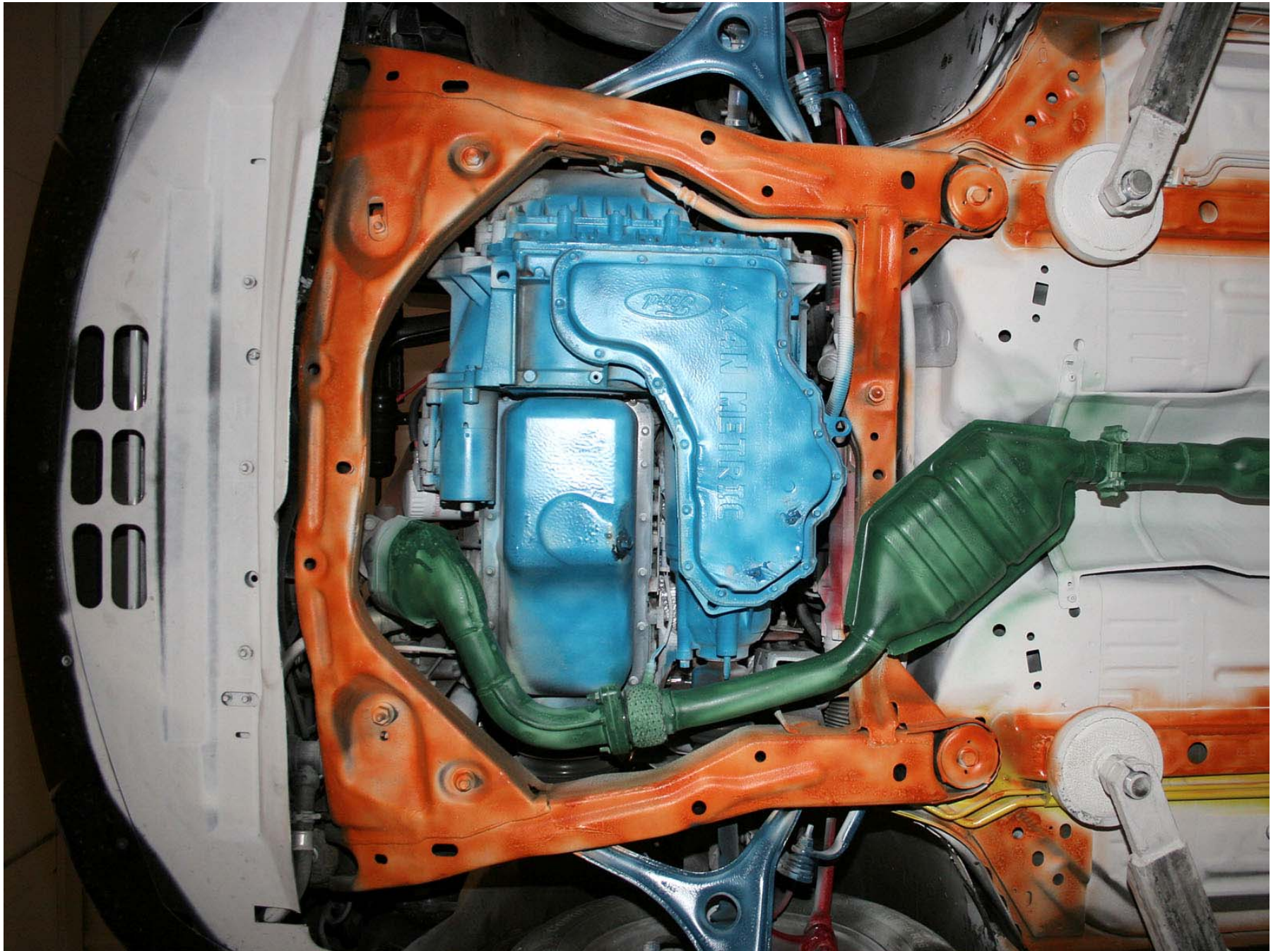
Figure A-204: Test Vehicle Pre-Test Front Underbody
