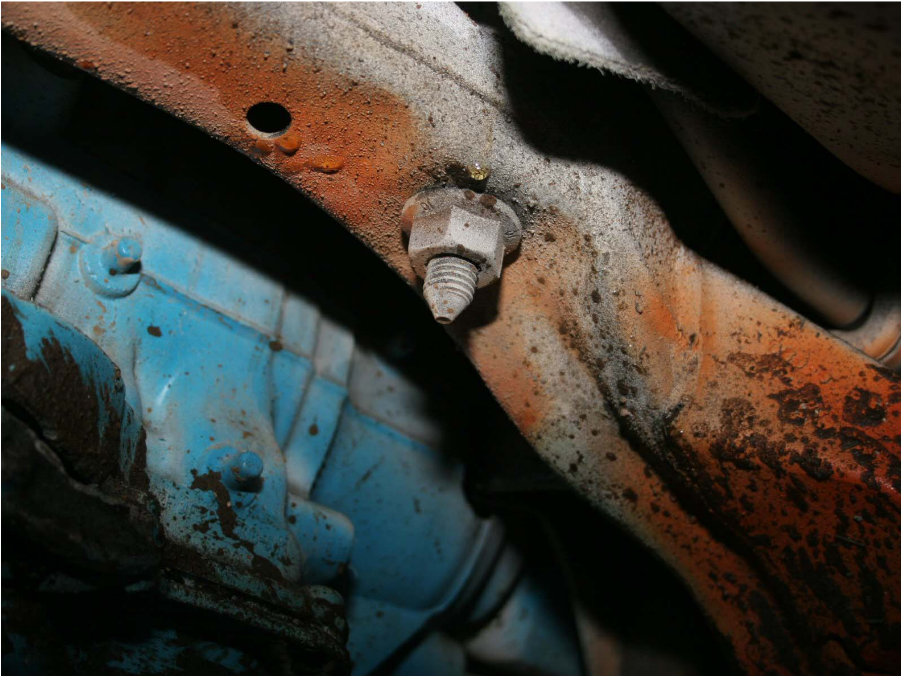
Figure A-215: Test Vehicle Post-Test Steering Rack Right Side Mounting Bolt
