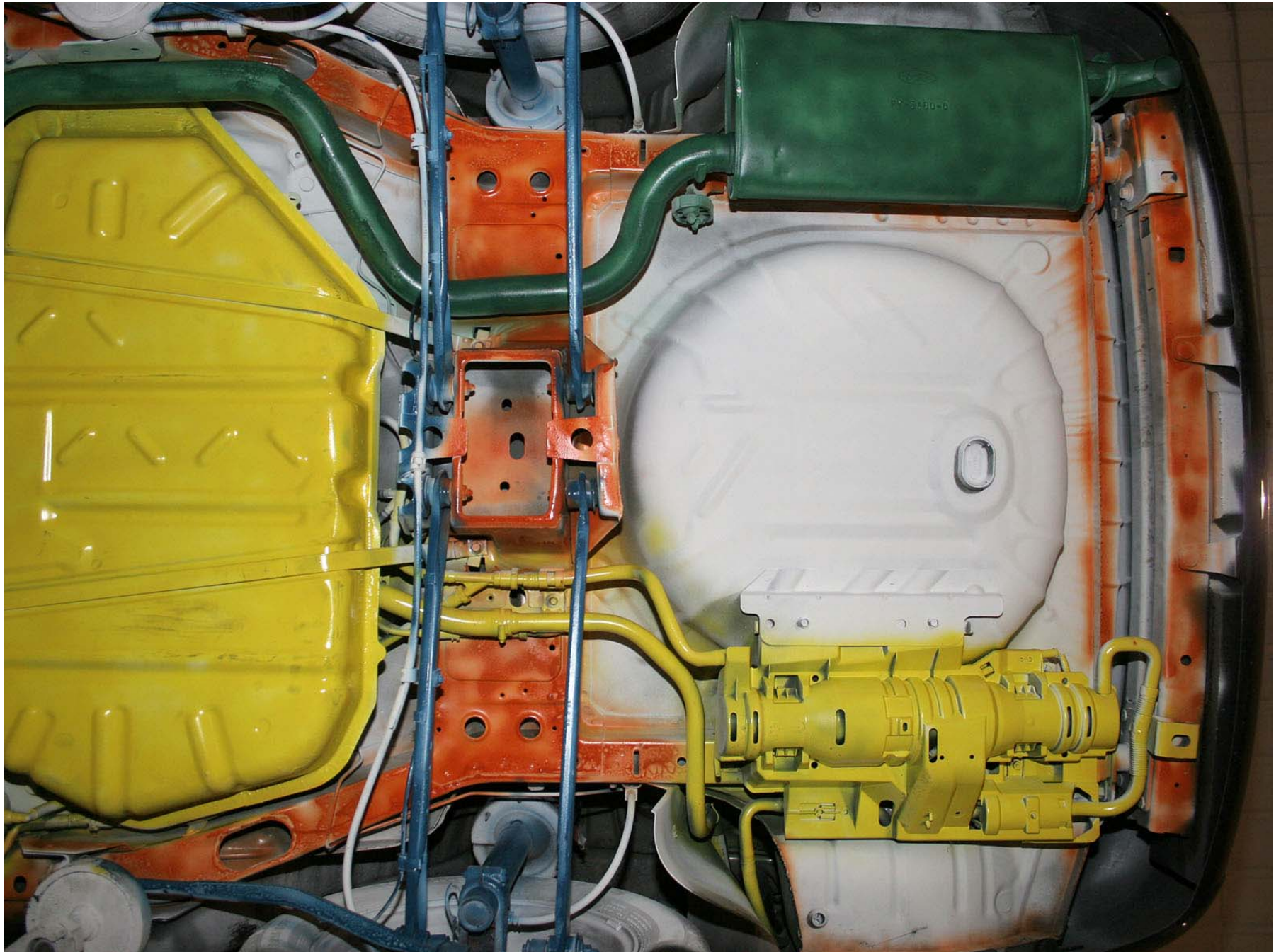
Figure A-208: Test Vehicle Pre-Test Rear Underbody
