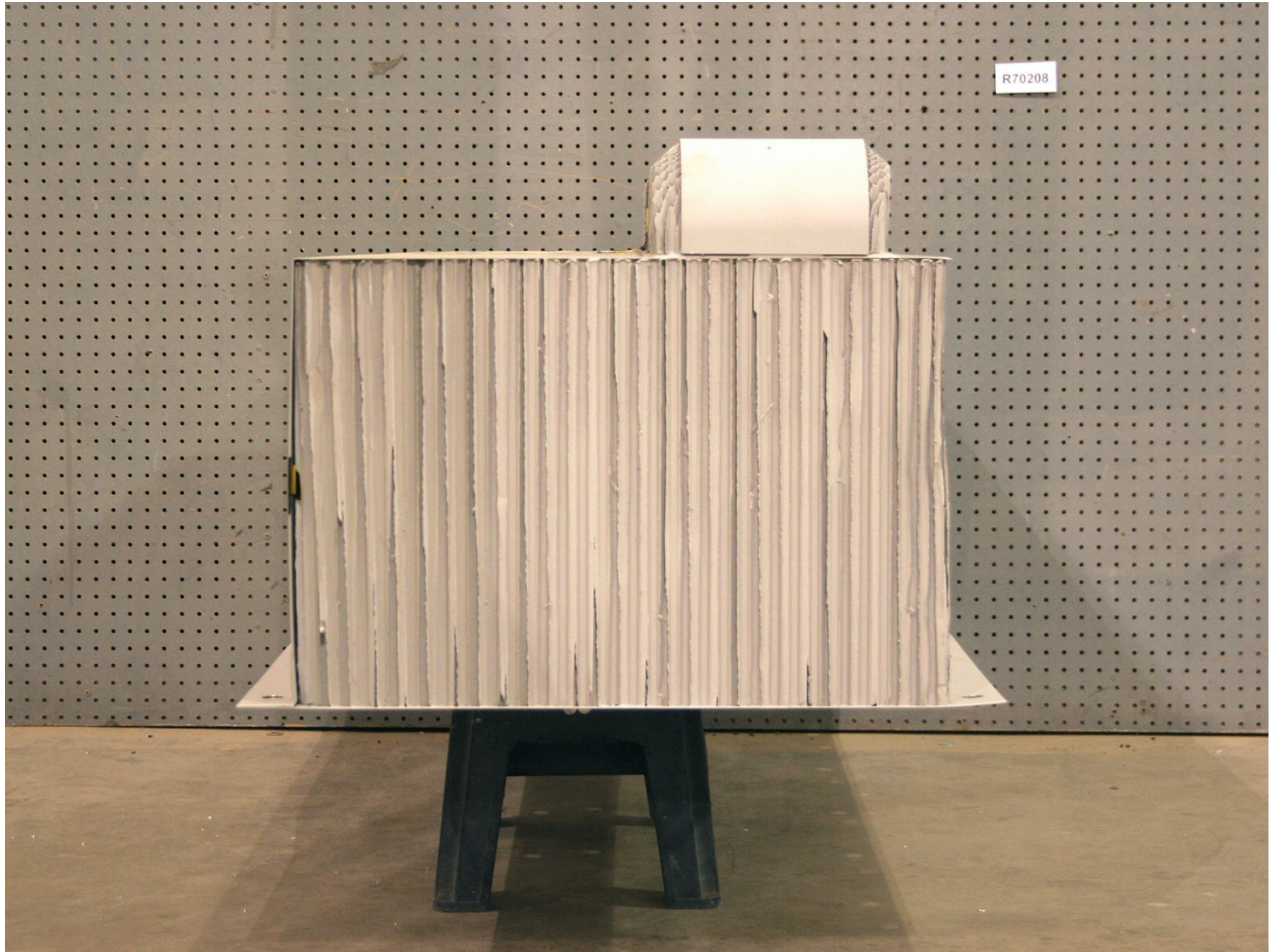
Figure A-319: Test Vehicle Pre-Test Right Side View of Deformable Barrier
