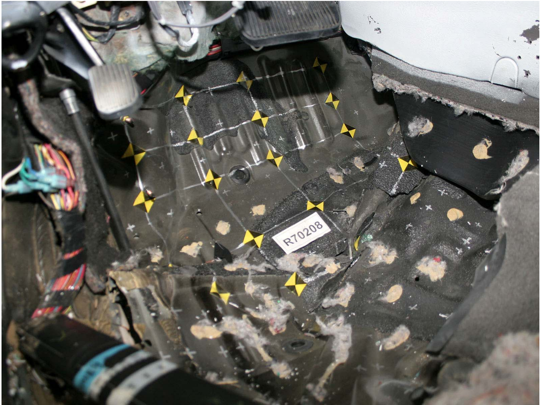
Figure A-282: Test Vehicle Post-Test Driver Floorpan Left \frac{3}{4} View, Seat Cushion Height
