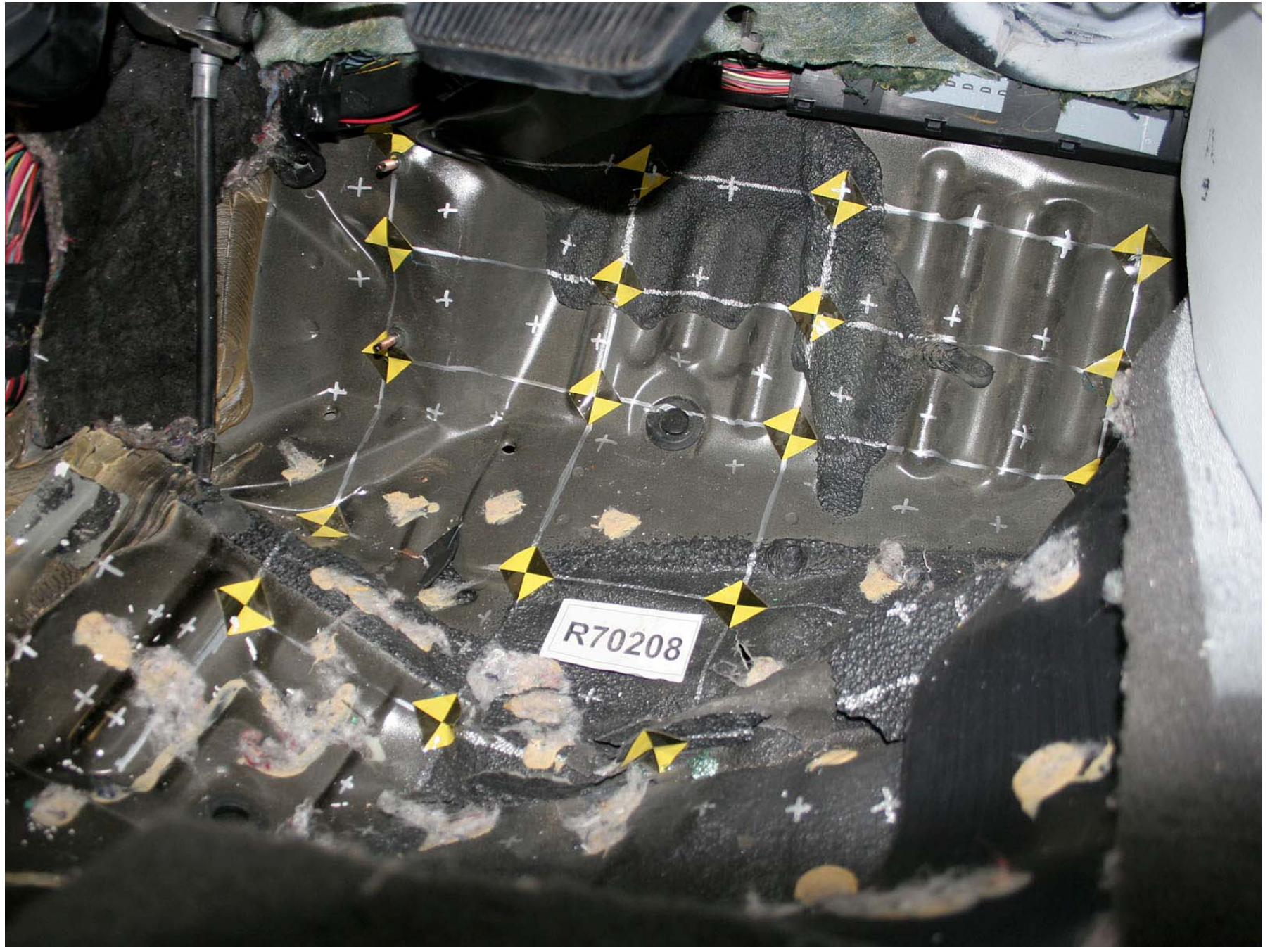
Figure A-290: Test Vehicle Post-Test Driver Floorpan Right \frac{3}{4} View, Seat Cushion Height
