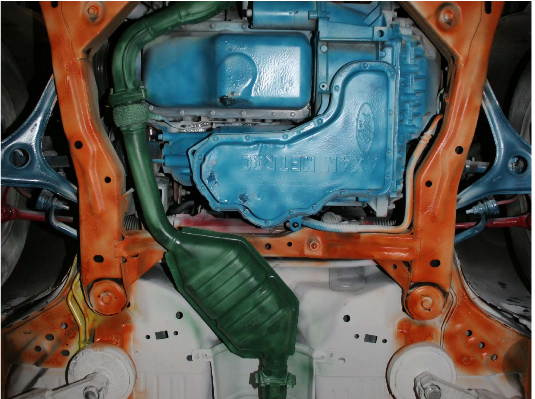
Figure A-210: Test Vehicle Pre-Test Steering Rack and Sway Bar View
