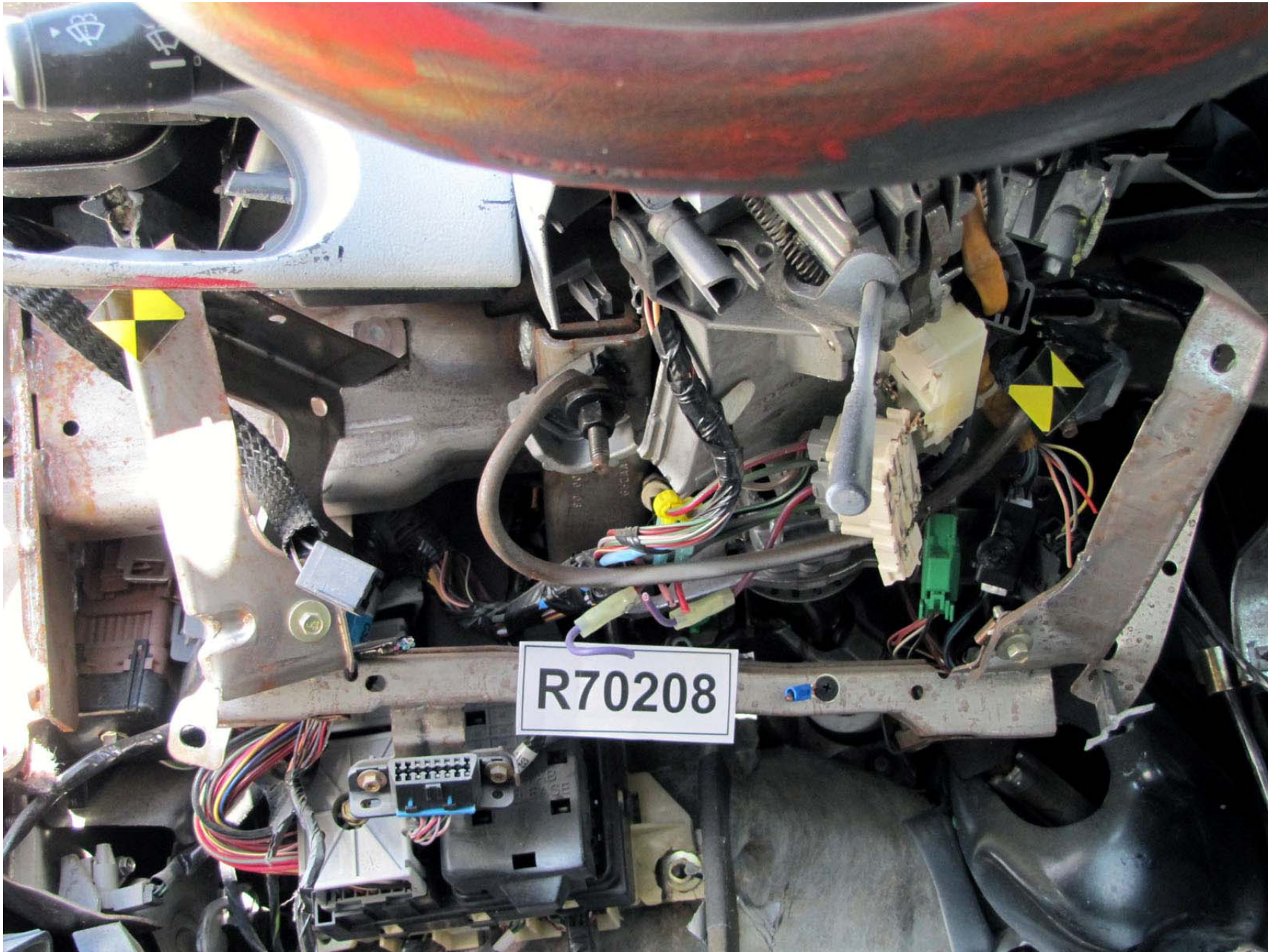
Figure A-246: Test Vehicle Post-Test Driver Side Knee Bolster
