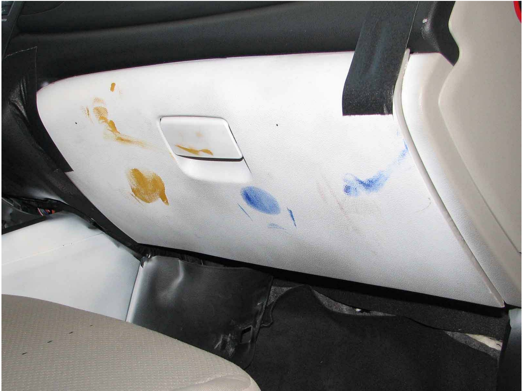
Figure A-58: Post-Test Passenger's Side Knee Bolster
