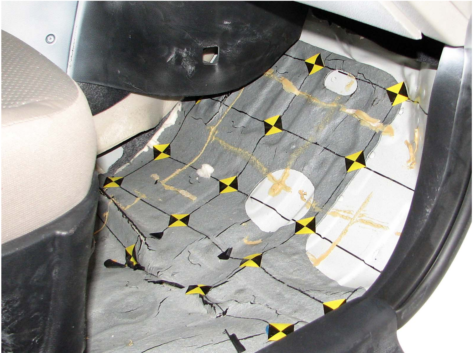
Figure A-60: Post-Test Passenger's Side Floorpan
