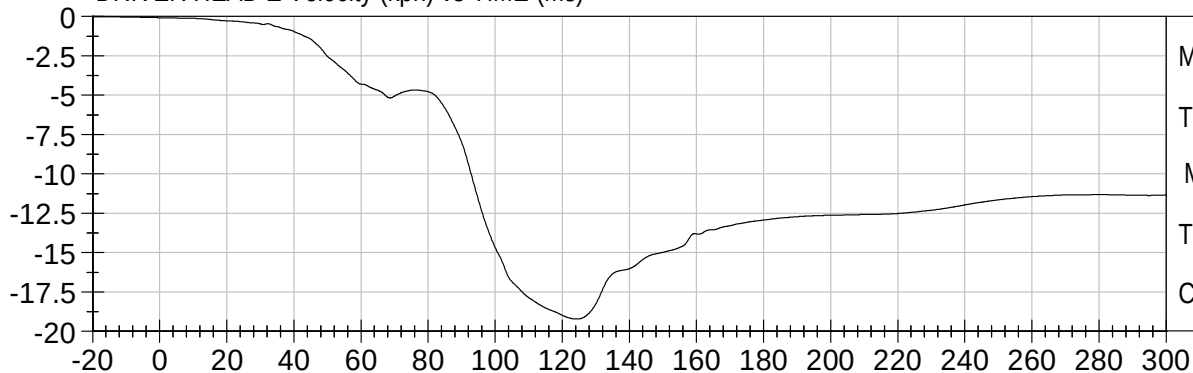
DRIVER HEAD Z Velocity (kph) vs TIME (ms)
