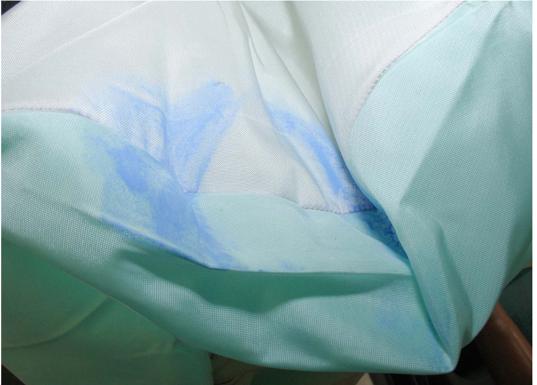
Post-Test 5th Fem. P2 Driver Dummy Airbag Left Side View
