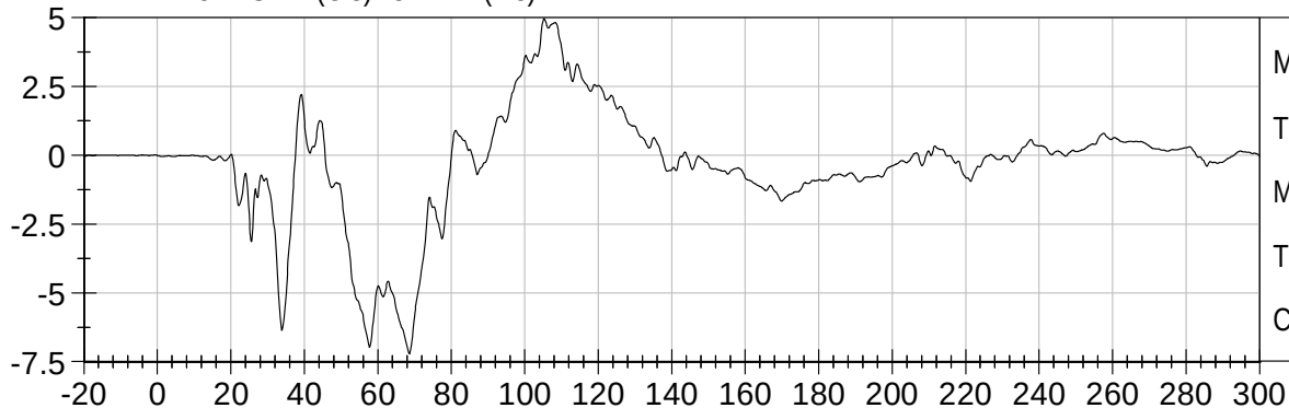
DRIVER CHEST Y (G's) vs TIME (ms)
