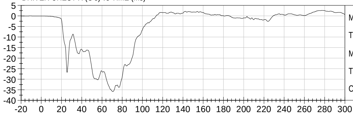
DRIVER CHEST X (G's) vs TIME (ms)
