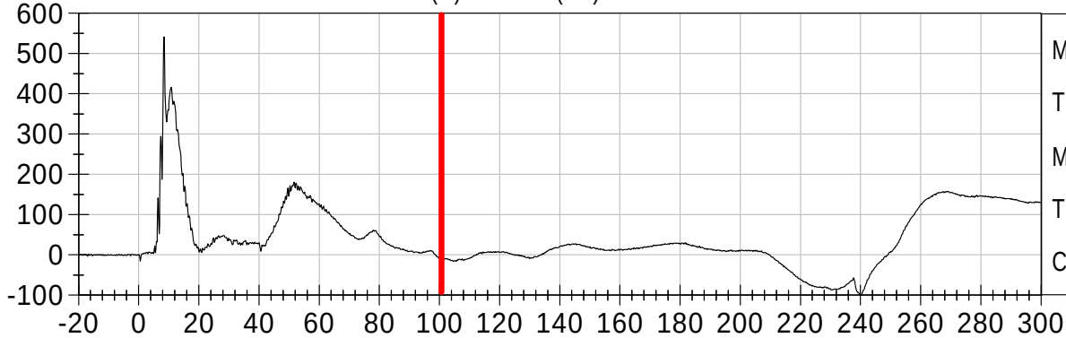
3YR OLD PASSENGER NECK FY (N) vs TIME (ms)
