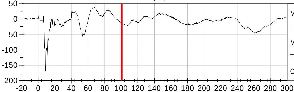
3YR OLD PASSENGER NECK FZ (N) vs TIME (ms)
