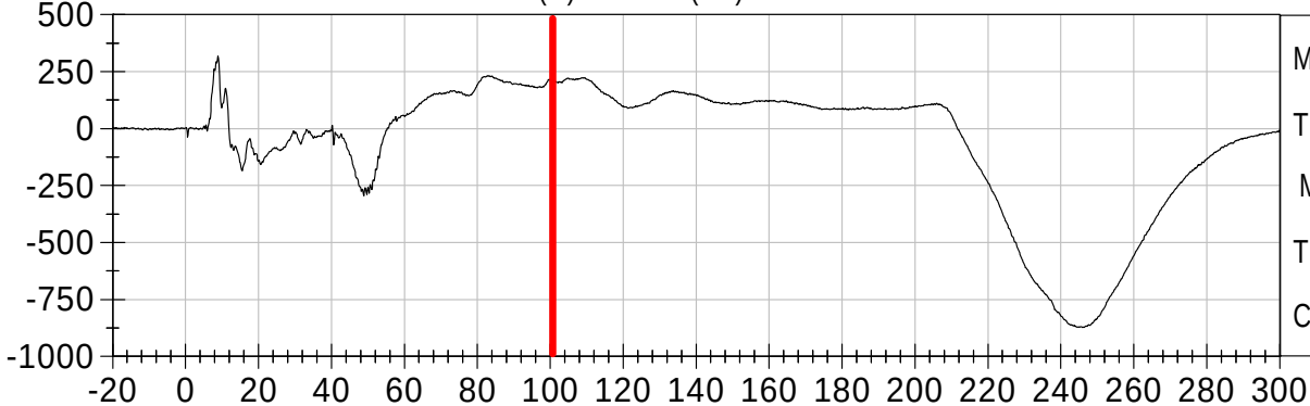
3YR OLD PASSENGER NECK FResultant (N) vs TIME (ms)
