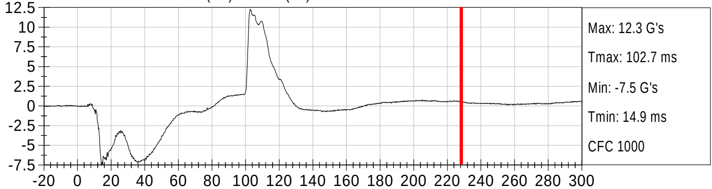
5TH FEM. DRIVER HEAD Y (G's) vs TIME (ms)
