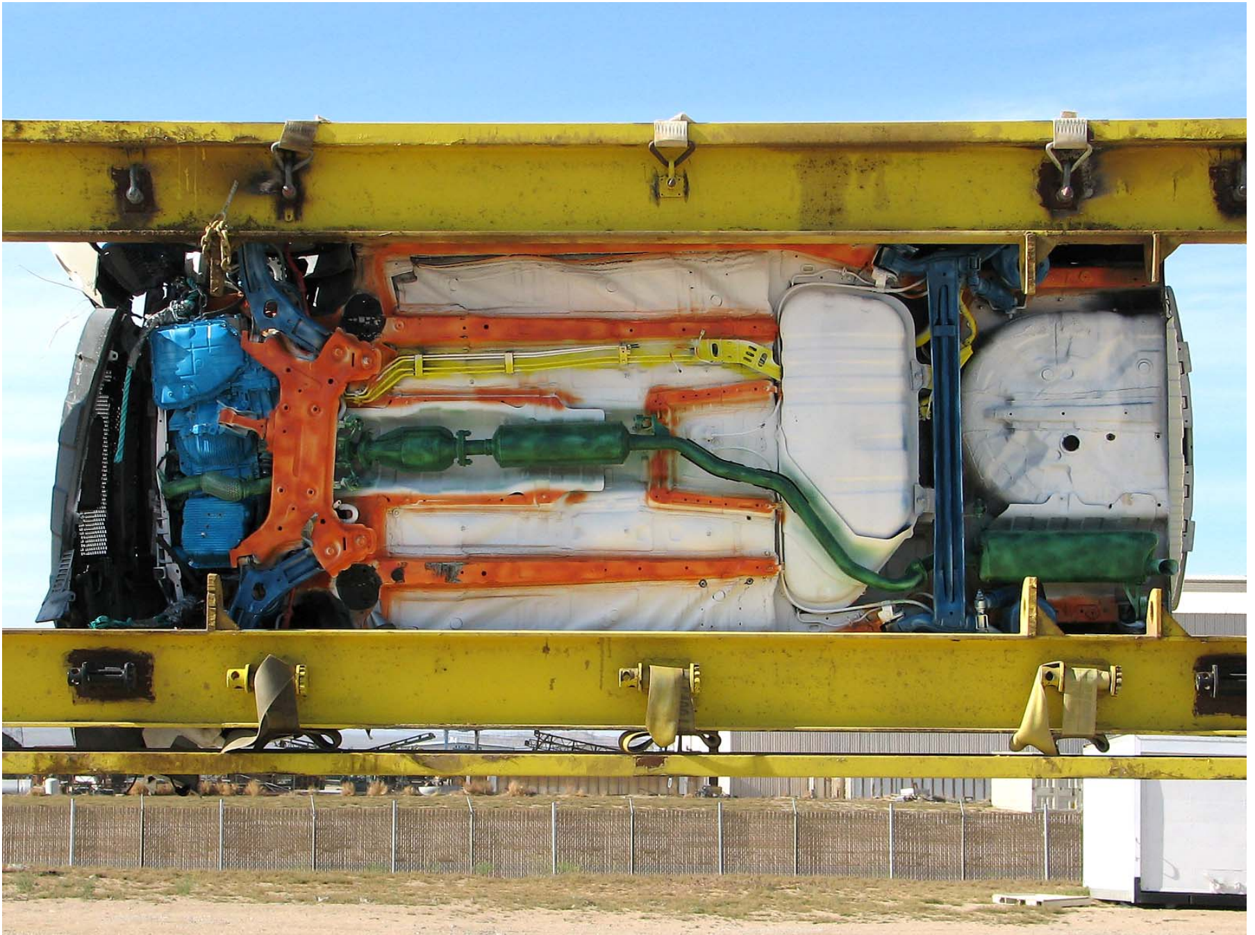
Figure A-70: Vehicle at 270° on Static Rollover Device
