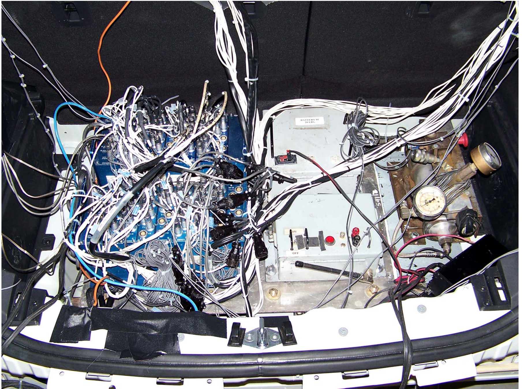
Figure A-65: Pre-Test Ballast Installed in Vehicle
