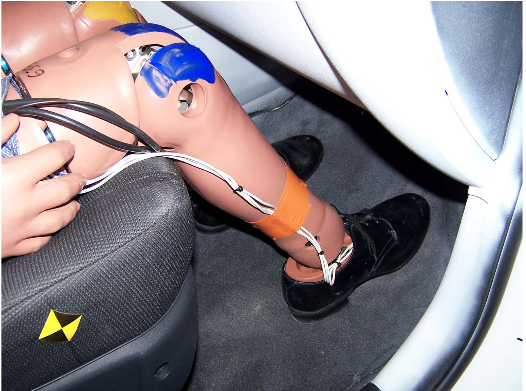
Figure A-55: Pre-Test Passenger Dummy Feet
