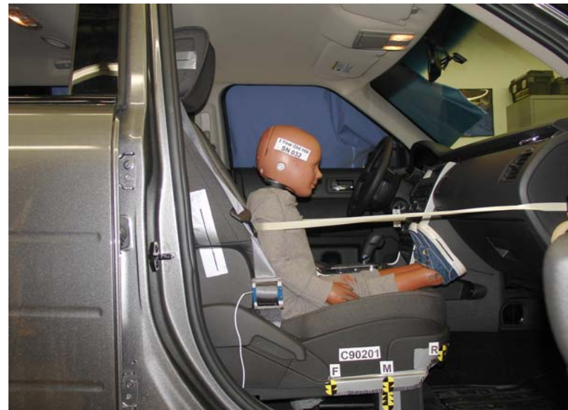
3-Year-Old Unbelted, Middle Seat Track, Position 3
