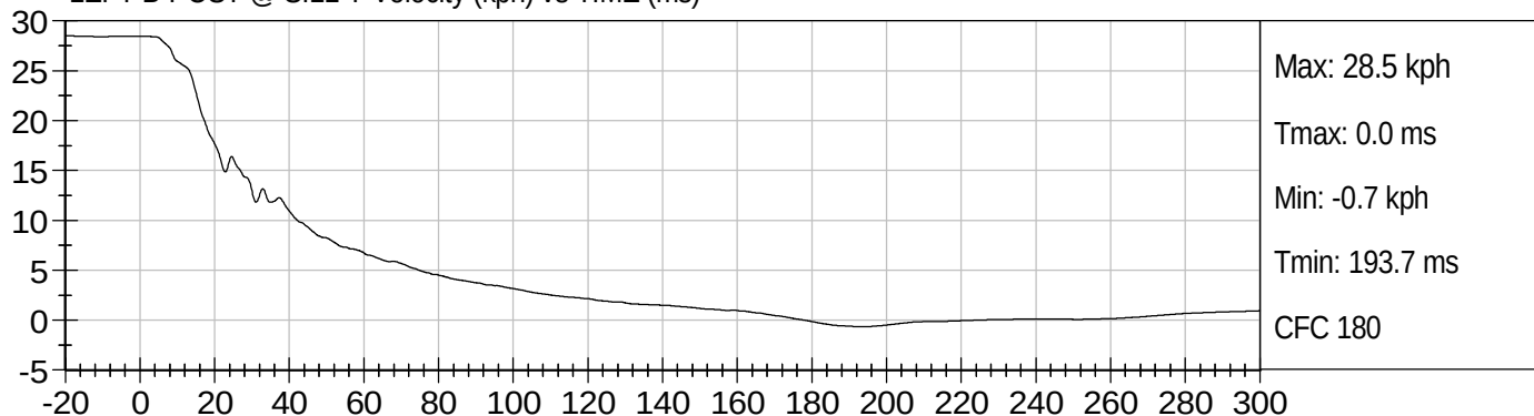
LEFT LOWER B-POST Y (G's) vs TIME (ms)
