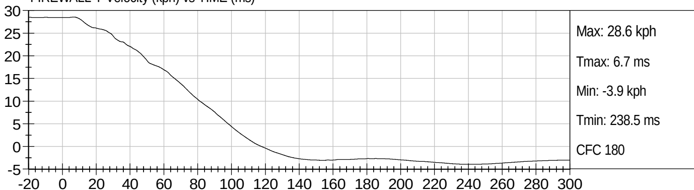
RIGHT FLOOR Y (G's) vs TIME (ms)
