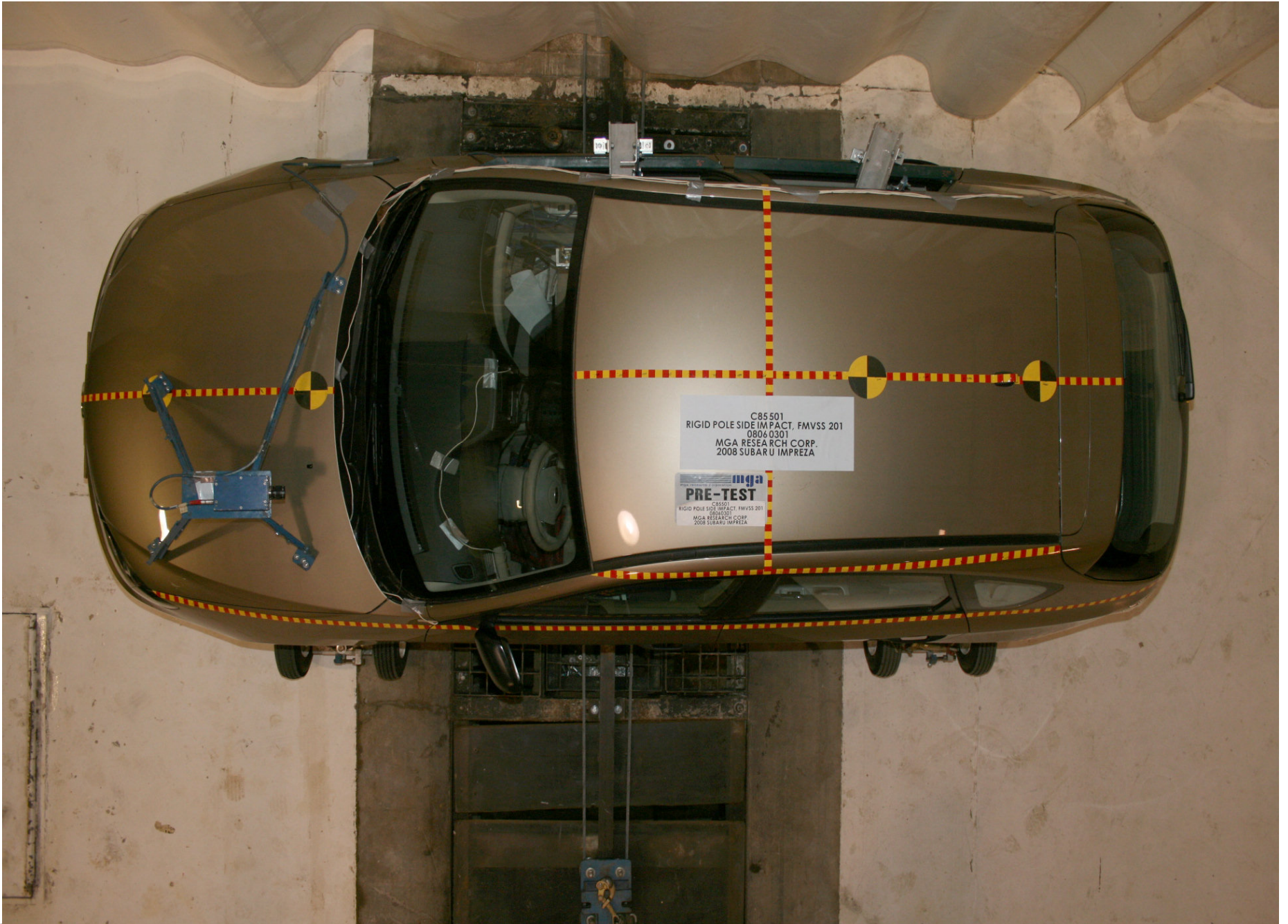
Pre-Test Overhead View of Test Vehicle
