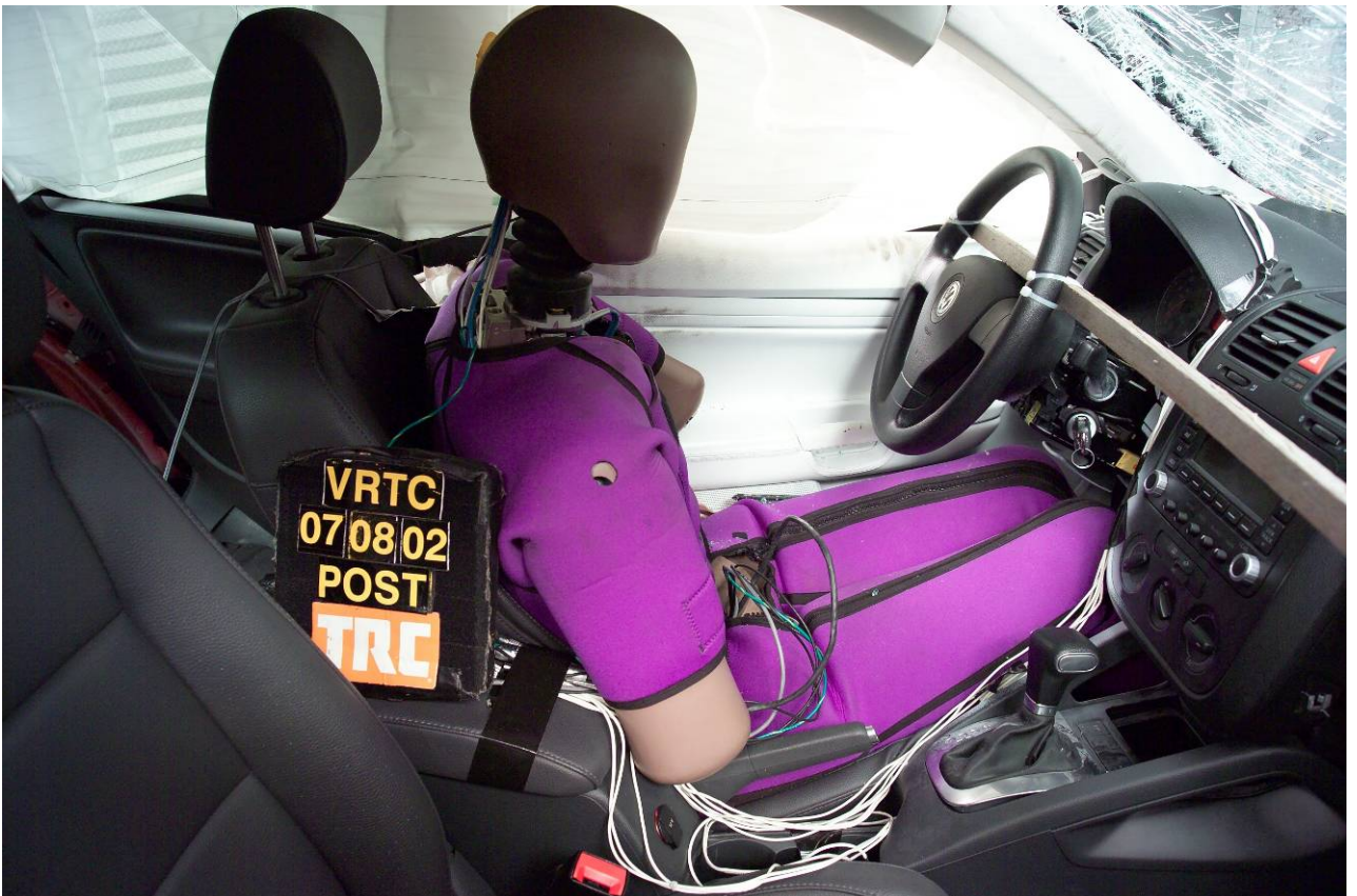
Figure A-27 Post-Test Right Side Dummy Occupant Compartment View
