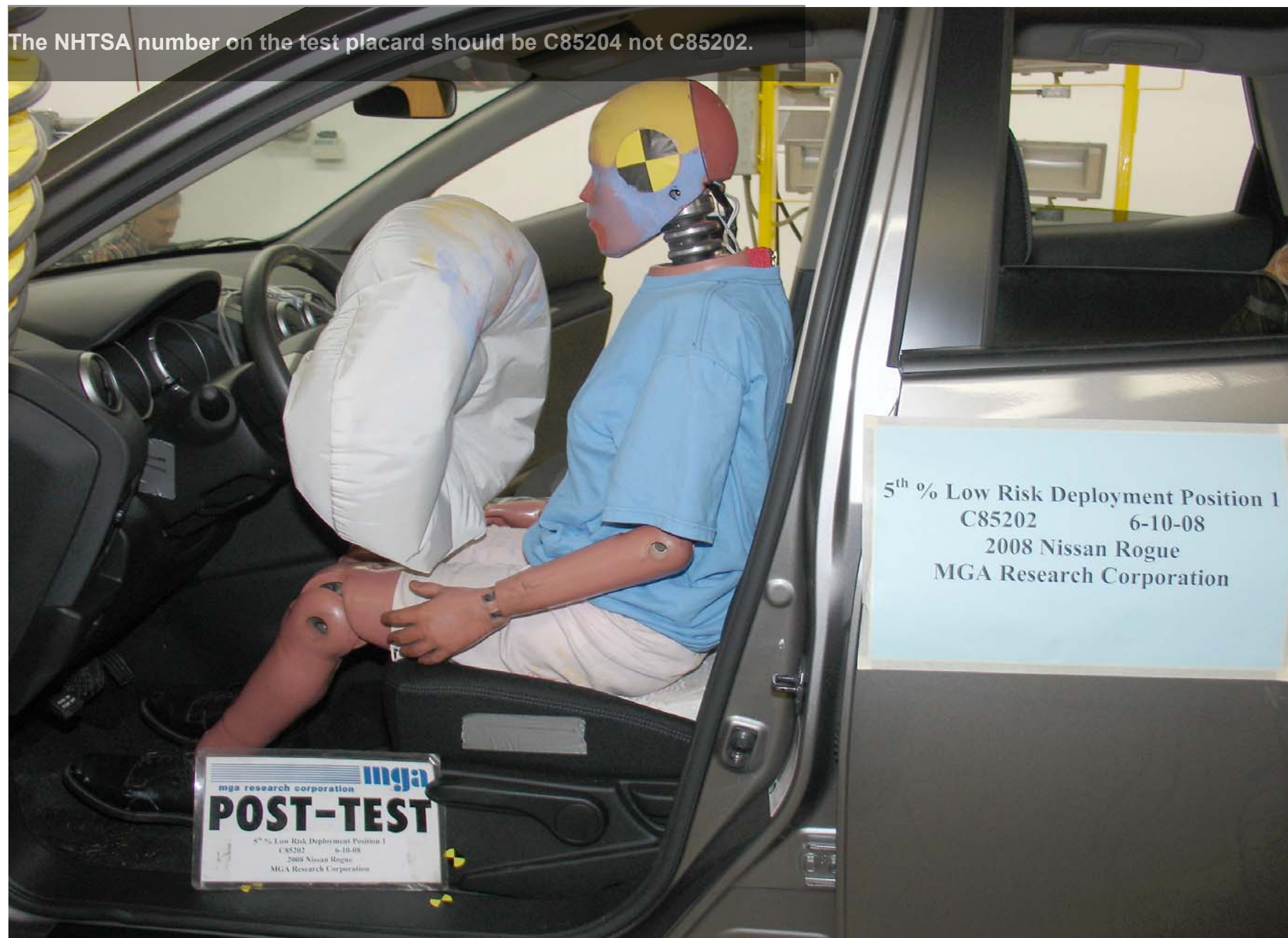
Post-Test 5th Fem. P1 Driver Dummy Left Side View
