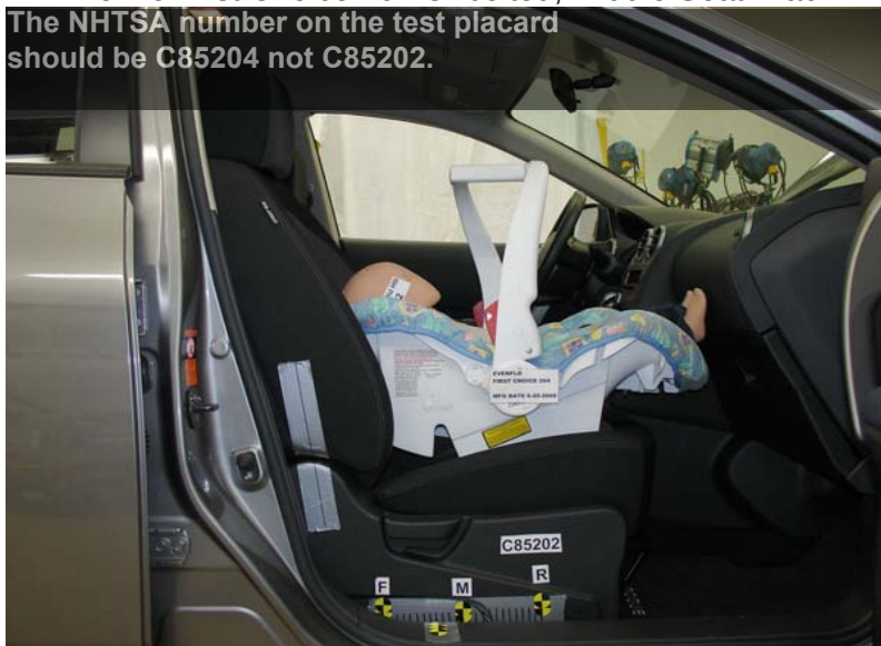
Evenflo First Choice 204 Forward Facing Unbelted, Forward Seat Track
