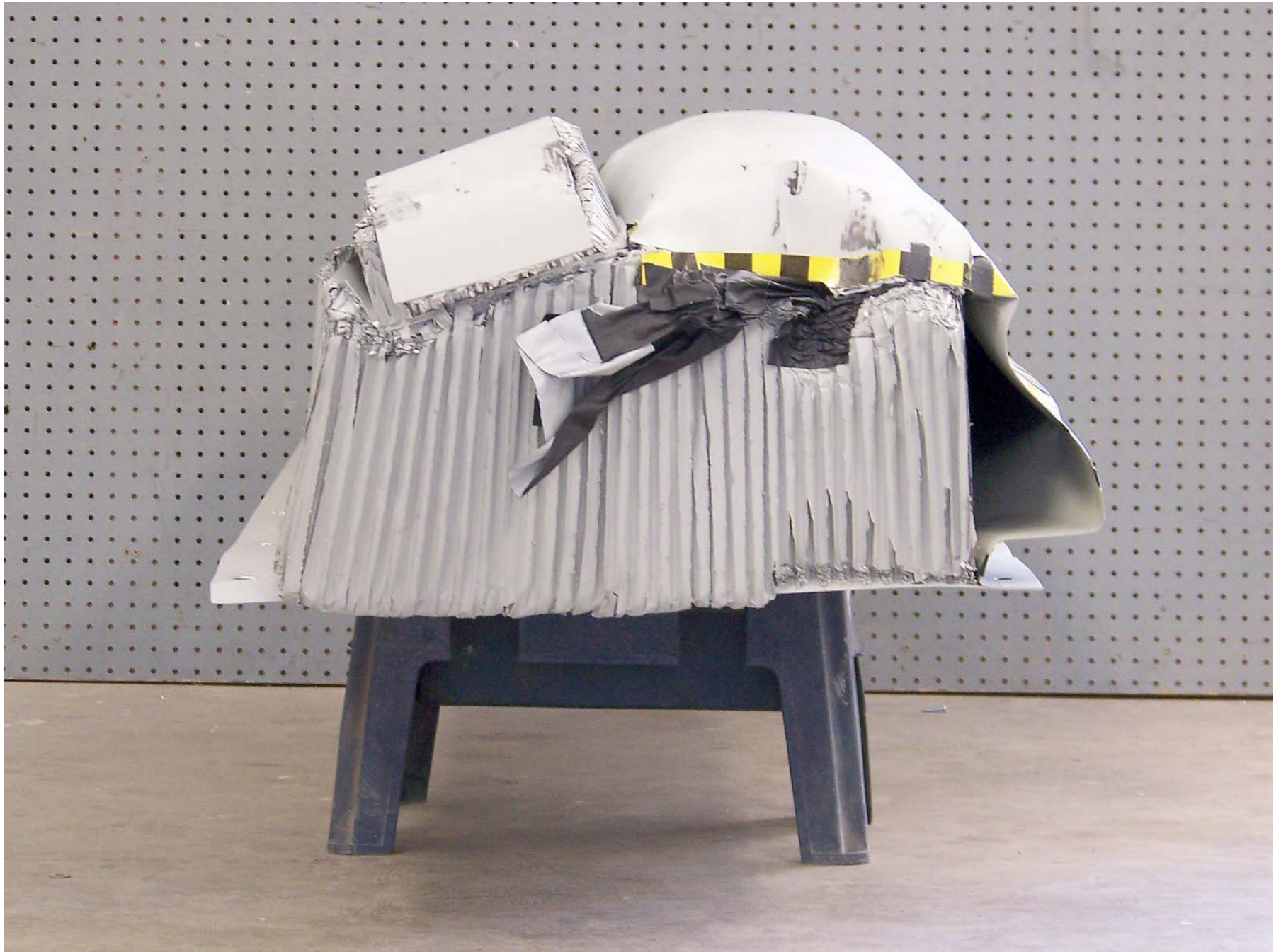
Figure A-59: Pre-Test Left Side View of Deformable Barrier
