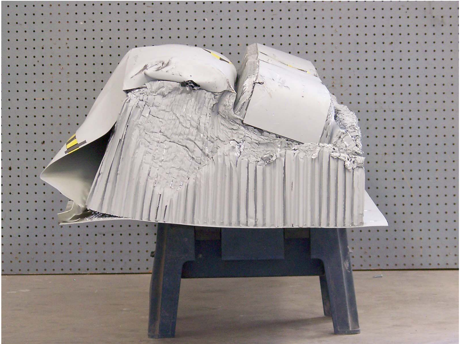
Figure A-57: Pre-Test Right Side View of Deformable Barrier
