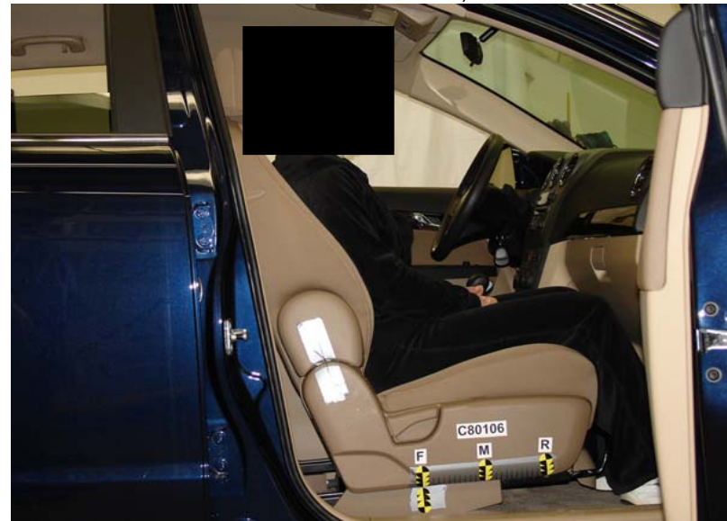
Unbelted 5th Percentile Female Dummy Reactivation, Forward Seat Track
