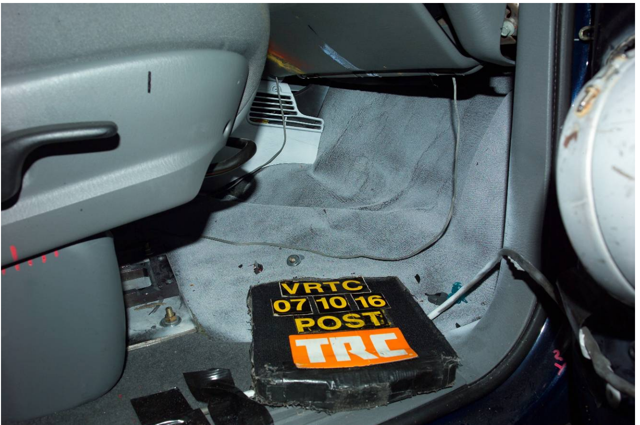
Figure A-68 Post-Test Passenger Floorpan Deformation View
