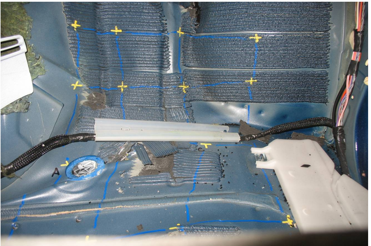
Figure A-112 Post-Test Passenger Floorpan – View 4
