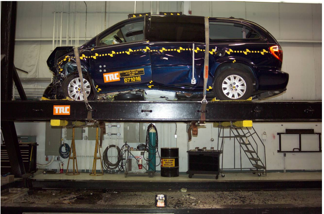
Figure A-91 Vehicle on Rollover Fixture – 360°
