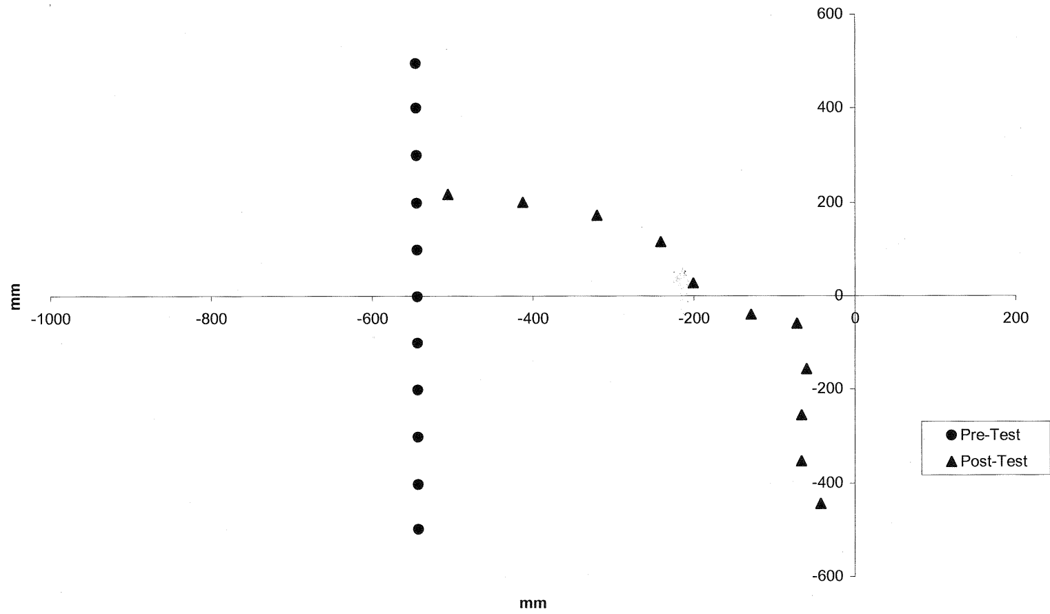
Deformable Barrier Face Profile 34-44
