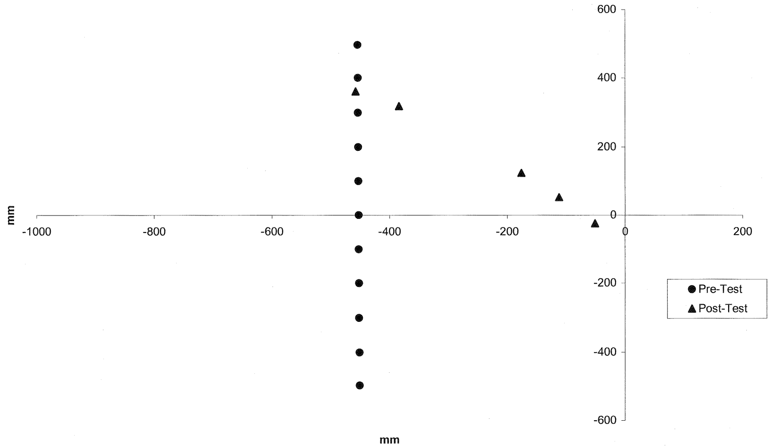
Deformable Barrier Face Profile 23-33
