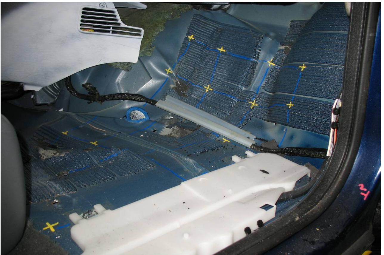
Figure A-110 Post-Test Passenger Floorpan – View 3
