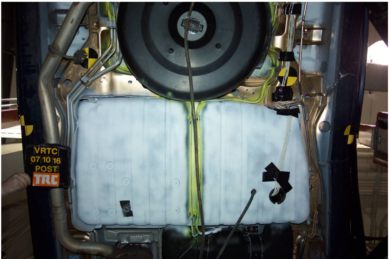
Figure A-24 Post-Test Mid Underbody View
