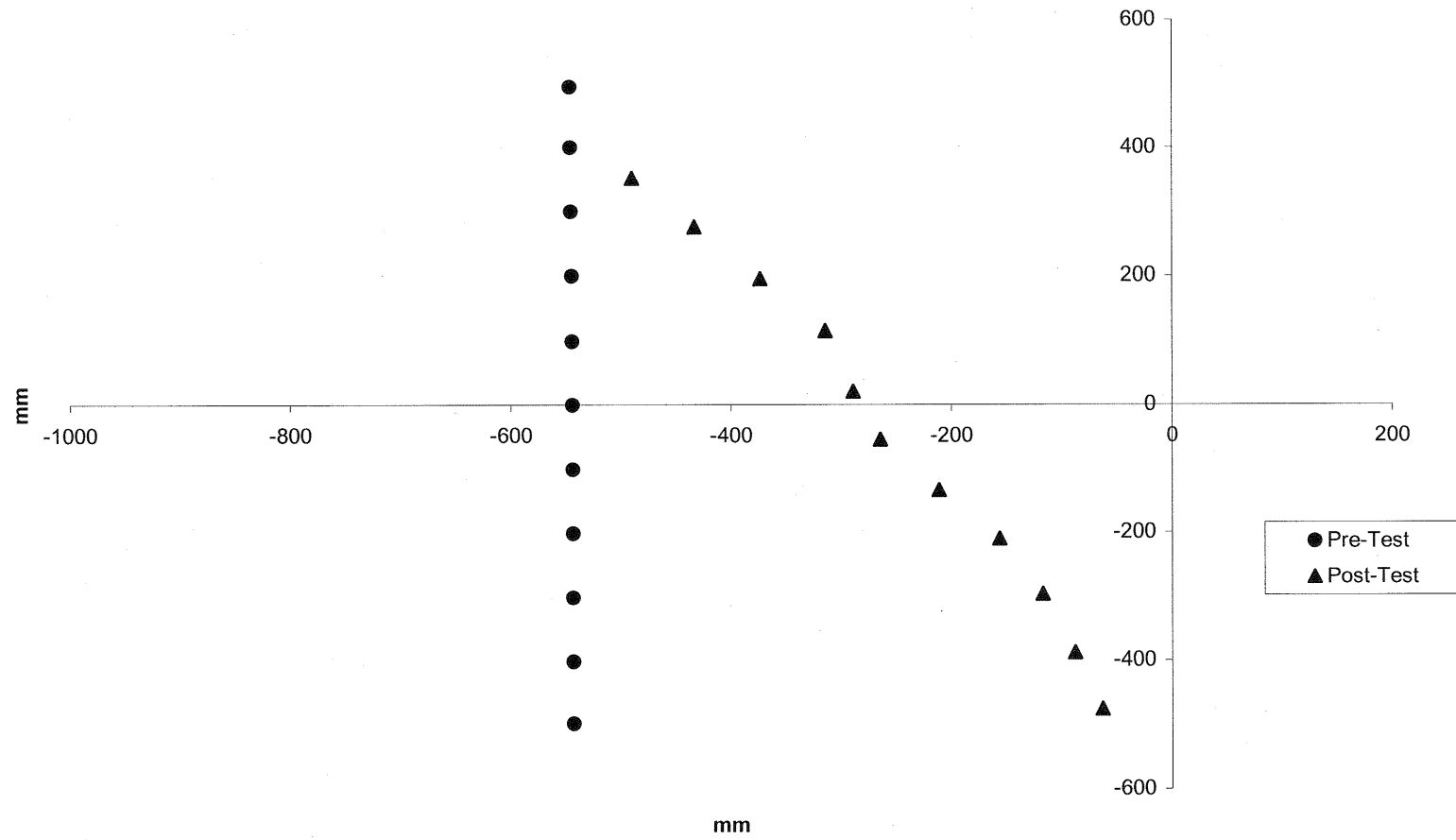
Deformable Barrier Face Profile 56-66
