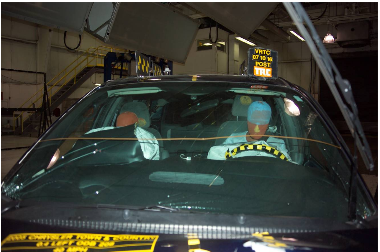
Figure A-40 Post-Test Driver and Passenger Dummies through Windshield View
