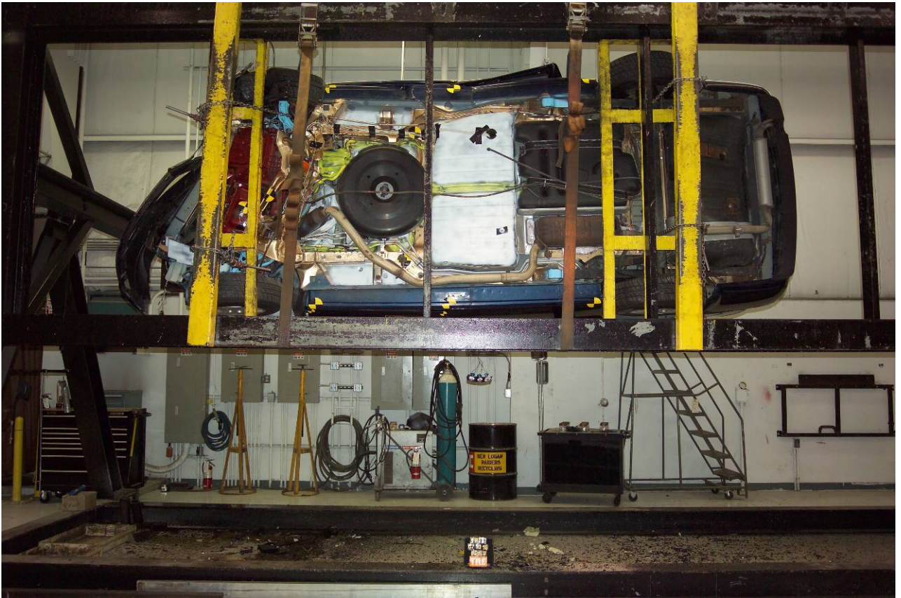
Figure A-90 Vehicle on Rollover Fixture – 270°
