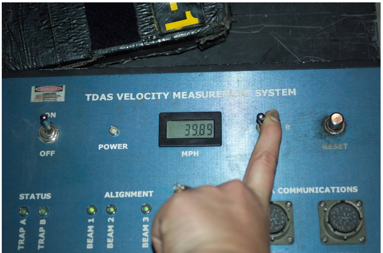
Figure A-86 Digital Light Trap Read-Out – View 2
