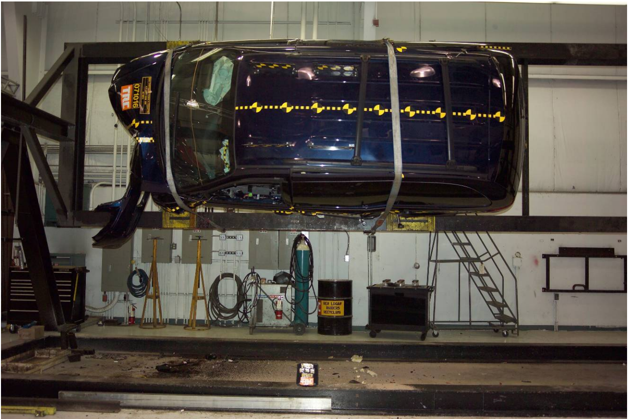
Figure A-88 Vehicle on Rollover Fixture – 90°
