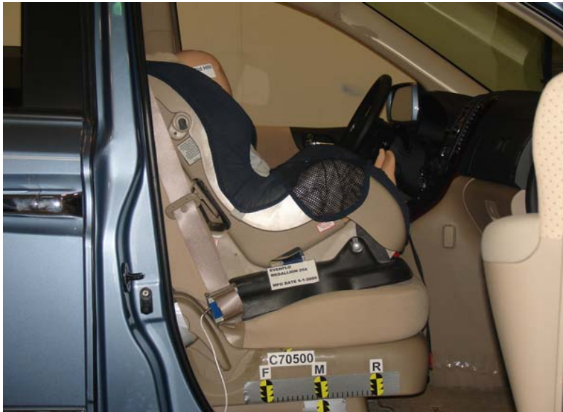
Evenflo Medallion 254 Forward Facing Unbelted, Middle Seat Track
