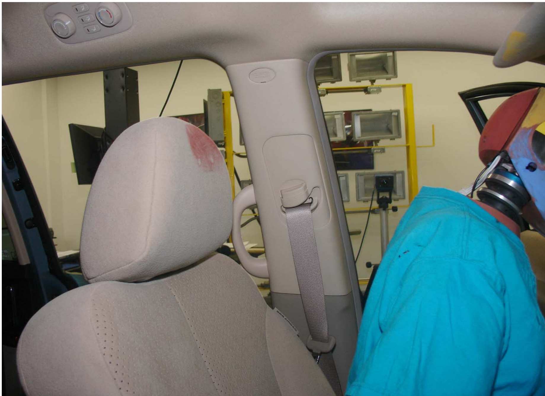
Post-Test 5th Fem. P2 Driver Dummy Head Contact (headrest)
