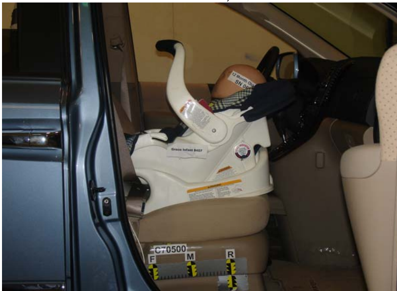
Graco Infant W/ Base Belted, Rearward Seat Track
