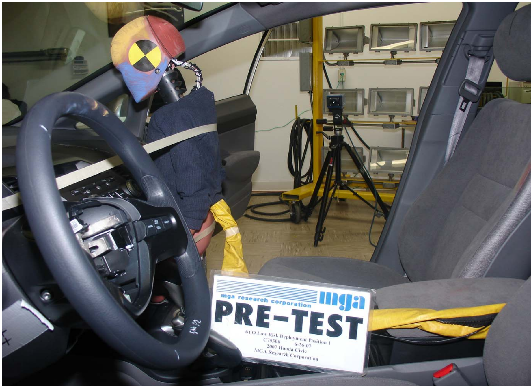
Pre-Test 6YO P1 Passenger Dummy Left Side View
