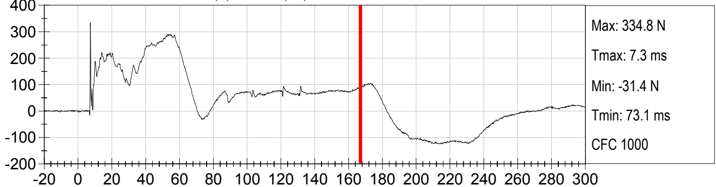
5TH FEM. DRIVER NECK FX (N) vs TIME (ms)
