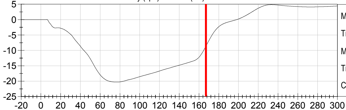
5TH FEM. DRIVER HEAD Y Velocity (kph) vs TIME (ms)
