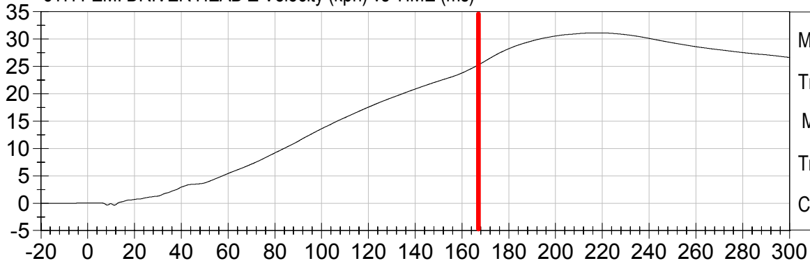
5TH FEM. DRIVER HEAD Z Velocity (kph) vs TIME (ms)
