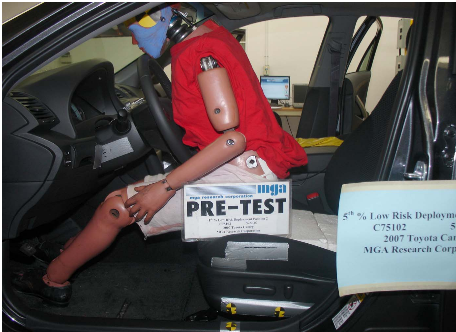
Pre-Test 5th Fem. P2 Driver Dummy Left Side View
