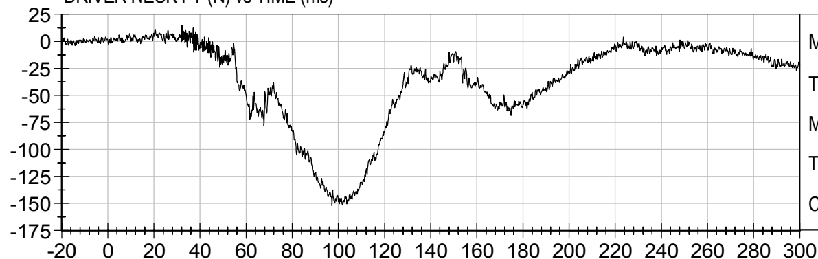
DRIVER NECK FZ (N) vs TIME (ms)
