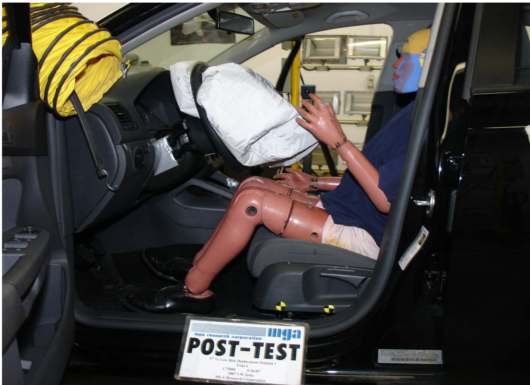
Post-Test 5th Fem. P1 Driver Dummy Left Side View (Trial 4)
