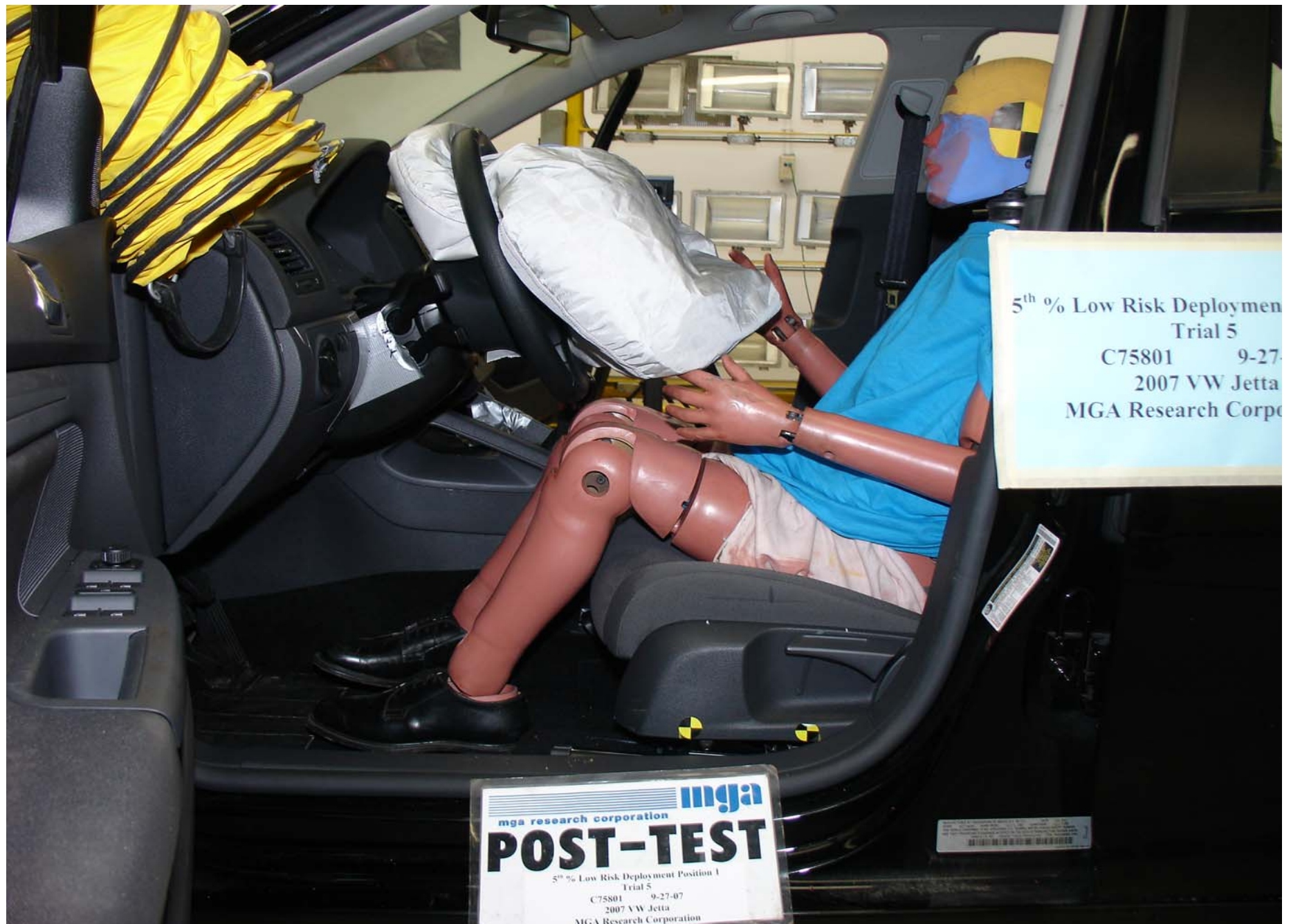
Post-Test 5th Fem. P1 Driver Dummy Left Side View (Trial 5)
