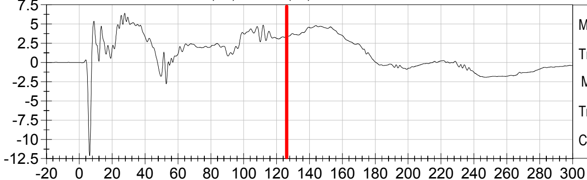
5TH FEM. DRIVER CHEST Resultant (G's) vs TIME (ms)
