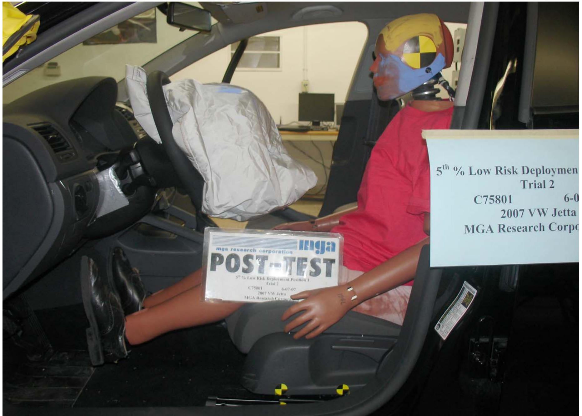
Post-Test 5th Fem. P1 Driver Dummy Left Side View (Trial 2)
