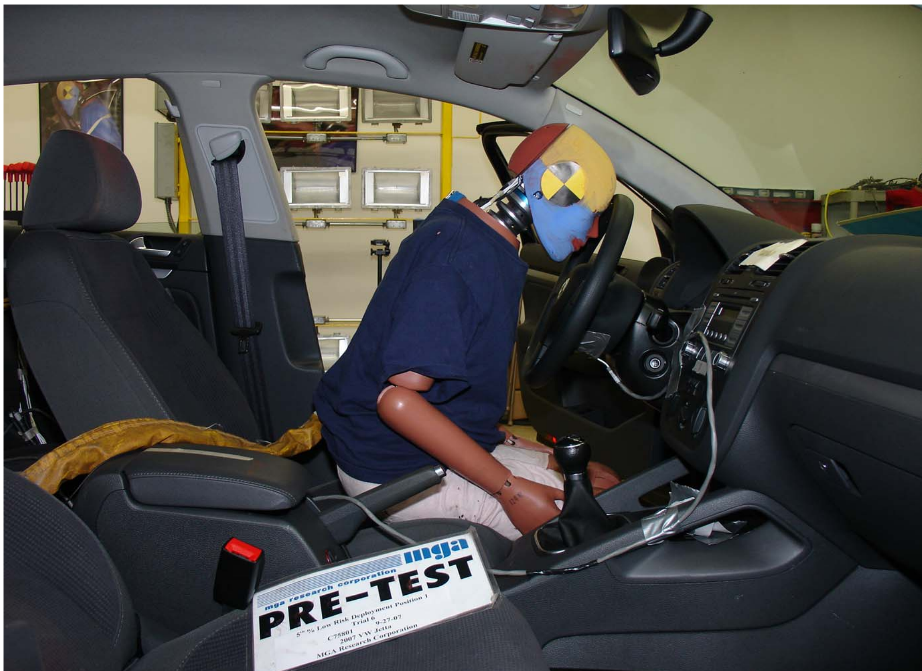
Pre-Test 5th Fem. P1 Driver Dummy Right Side View (Trial 6)
