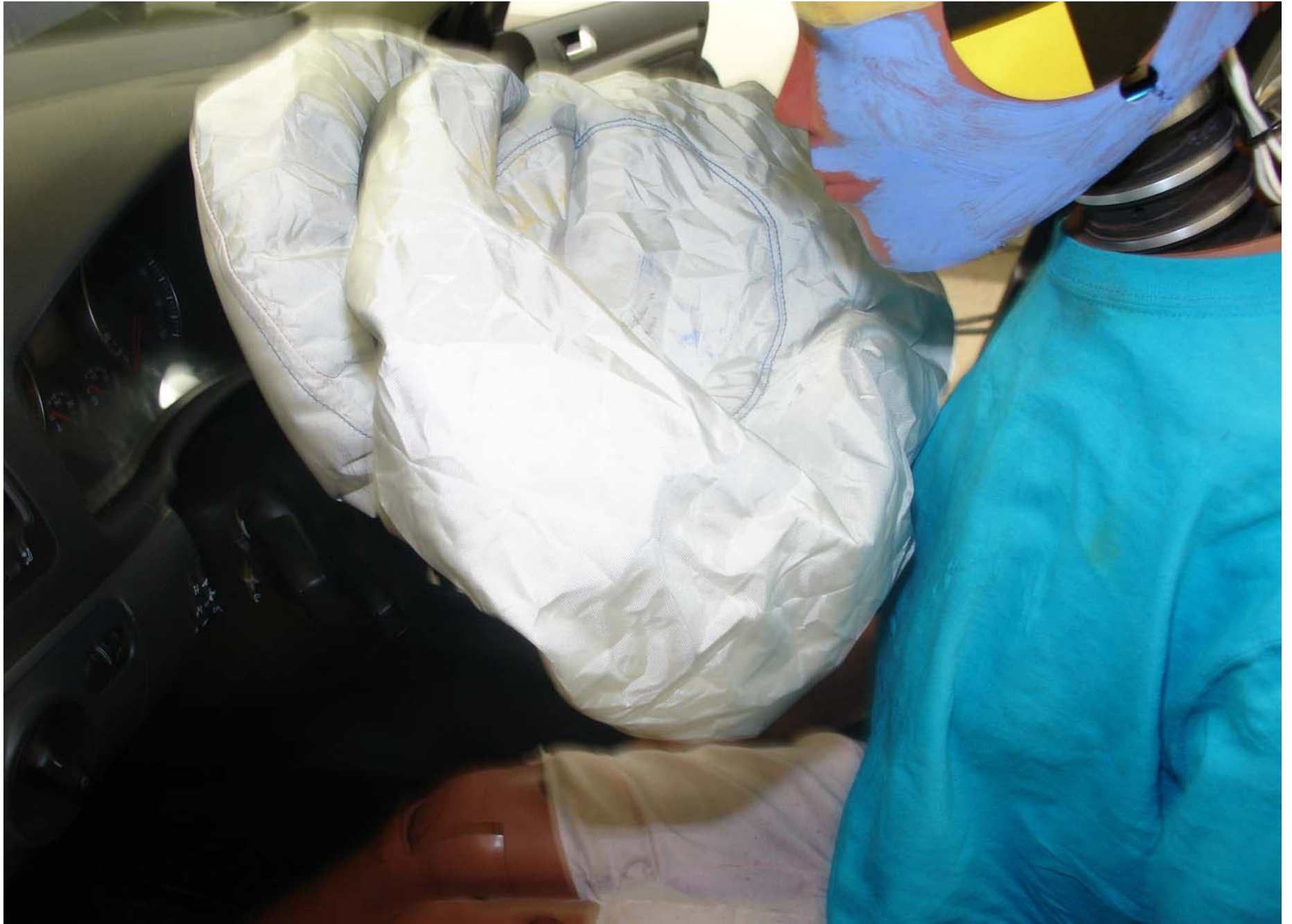
Post-Test 5th Fem. P2 Driver Dummy Airbag Left Side View (Trial 2)
