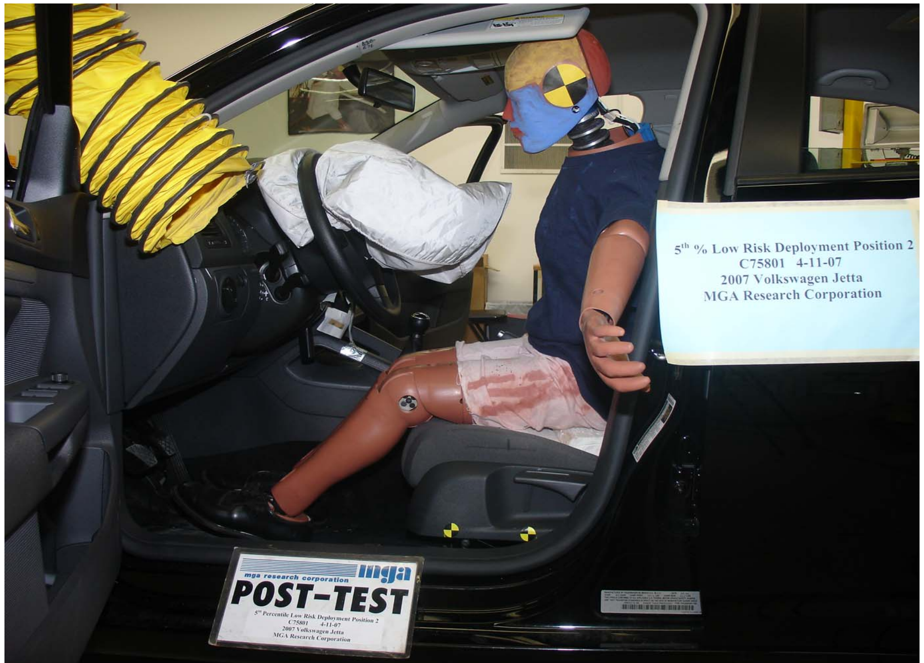
Post-Test 5th Fem. P2 Driver Dummy Left Side View (Trial 1)
