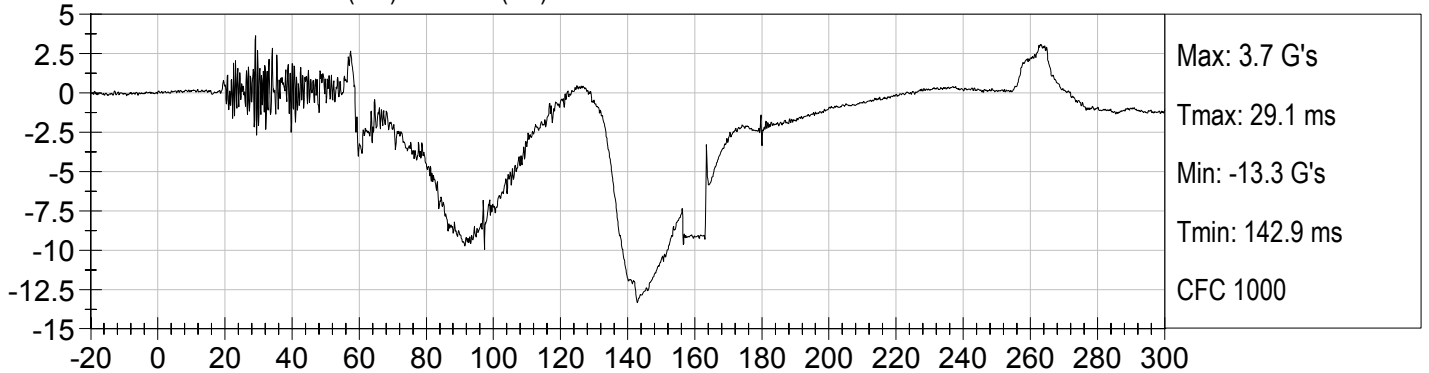
PASSENGER HEAD Y (G's) vs TIME (ms)
