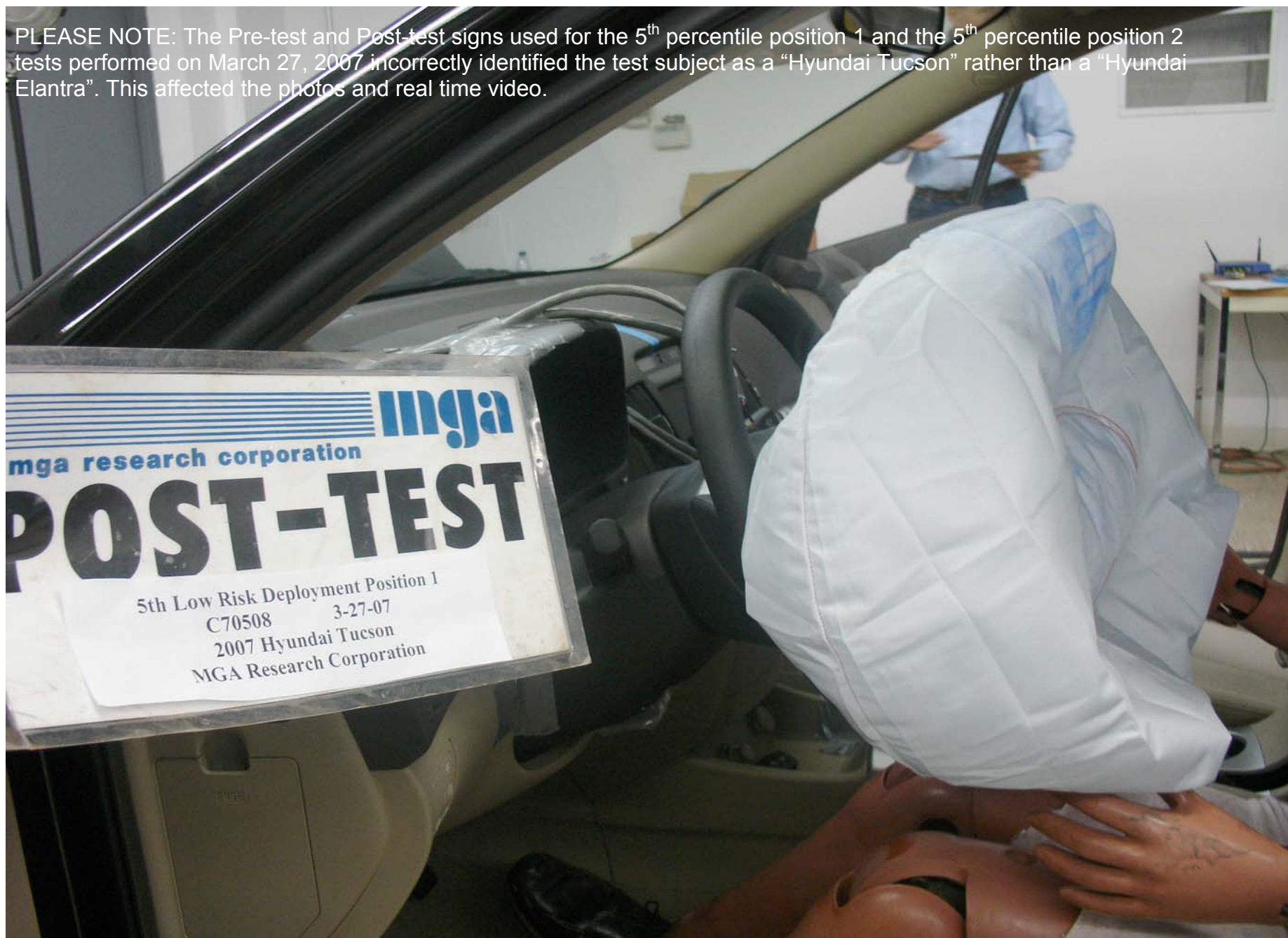
Post-Test 5th Fem. P1 Trial 1 Driver Dummy Airbag Left View
