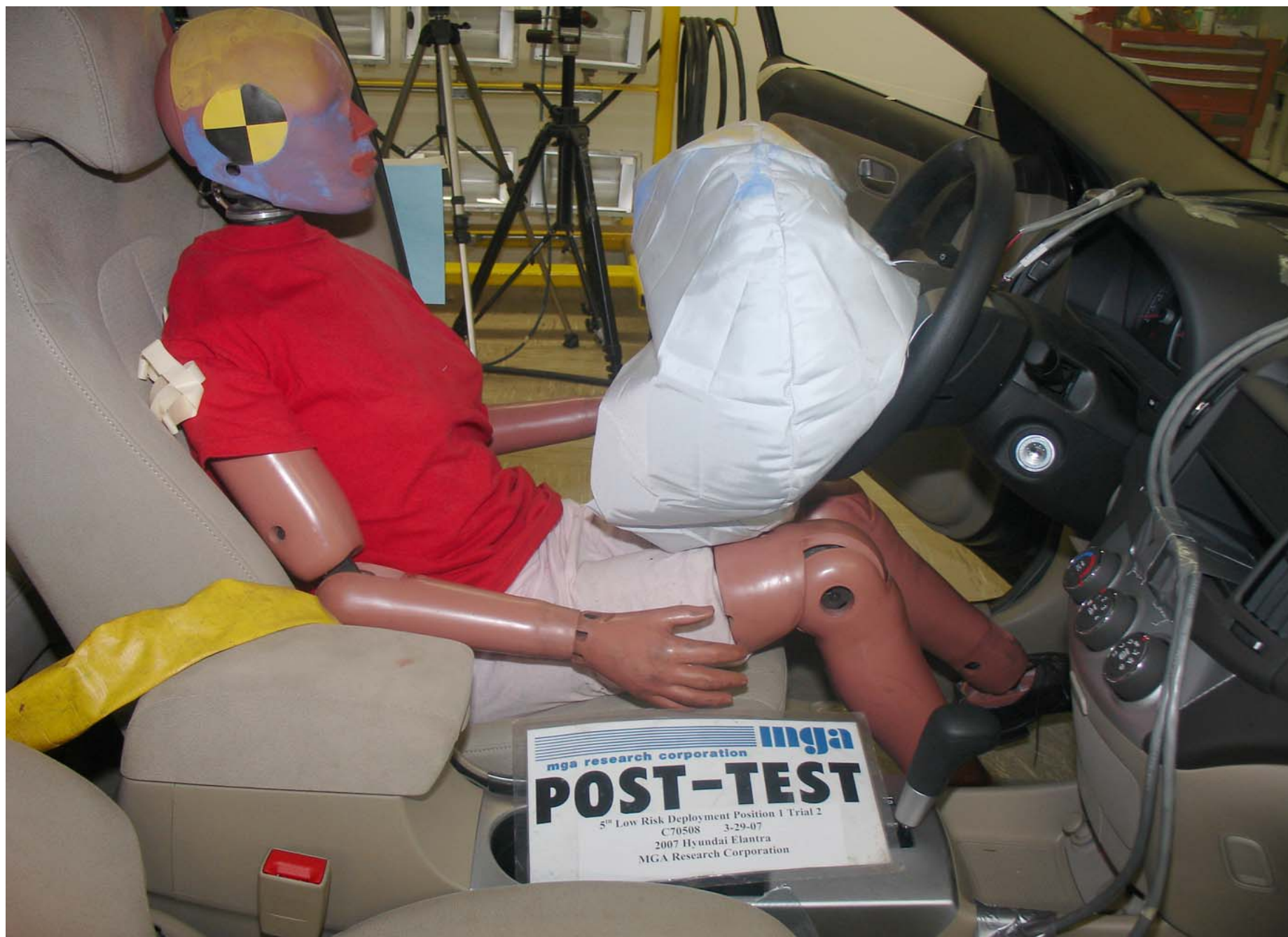
Post-Test 5th Fem. P1 Trial 2 Driver Dummy Right Side View (Door Open)
