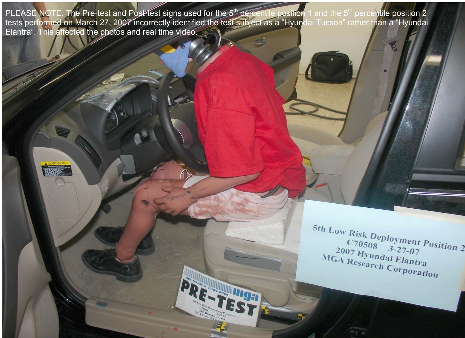
Pre-Test 5th Fem. P2 Driver Dummy Left Side View (Door Open)
