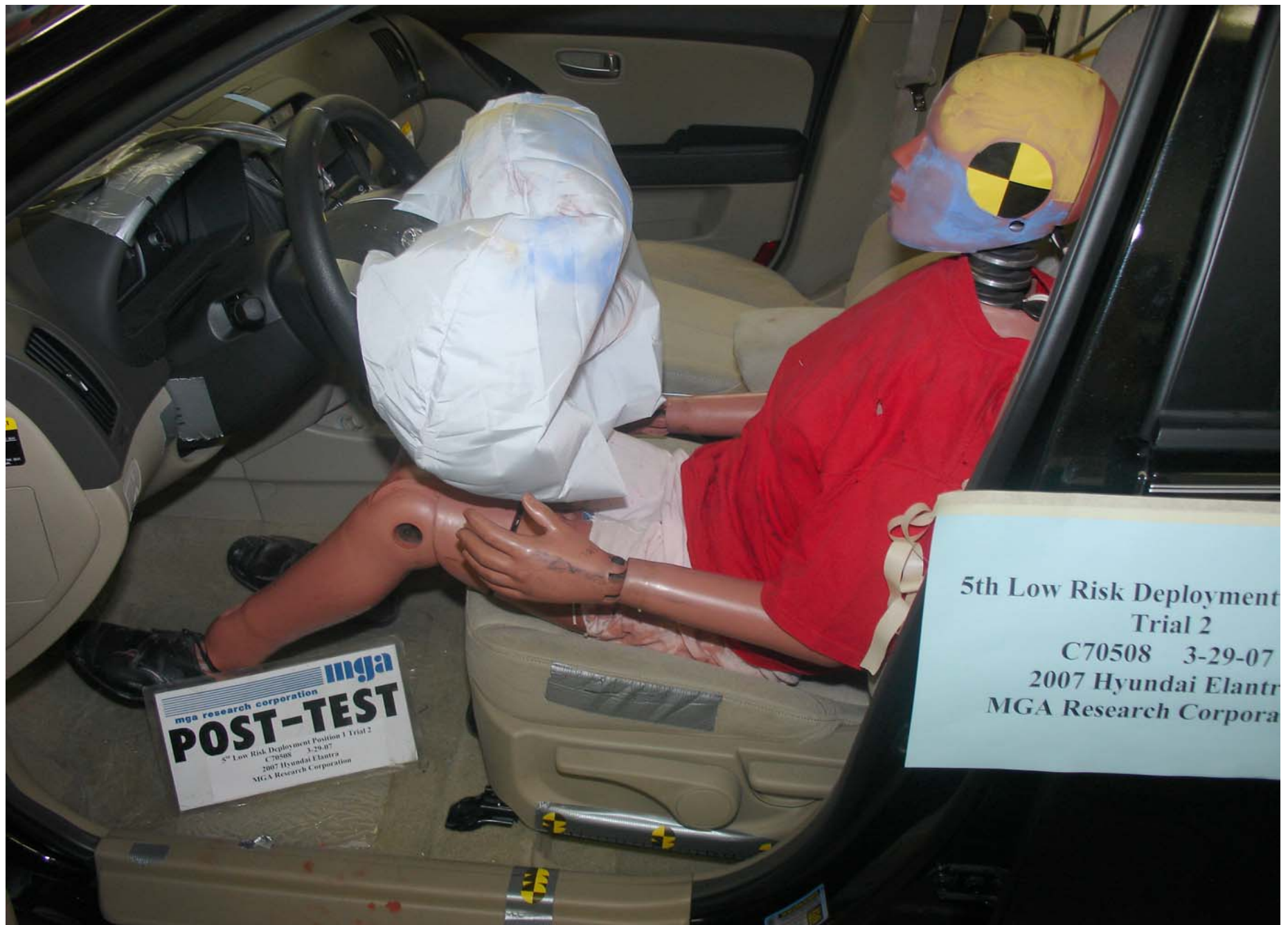
Post-Test 5th Fem. P1 Trial 2 Driver Dummy Left Side View (Door Open)
