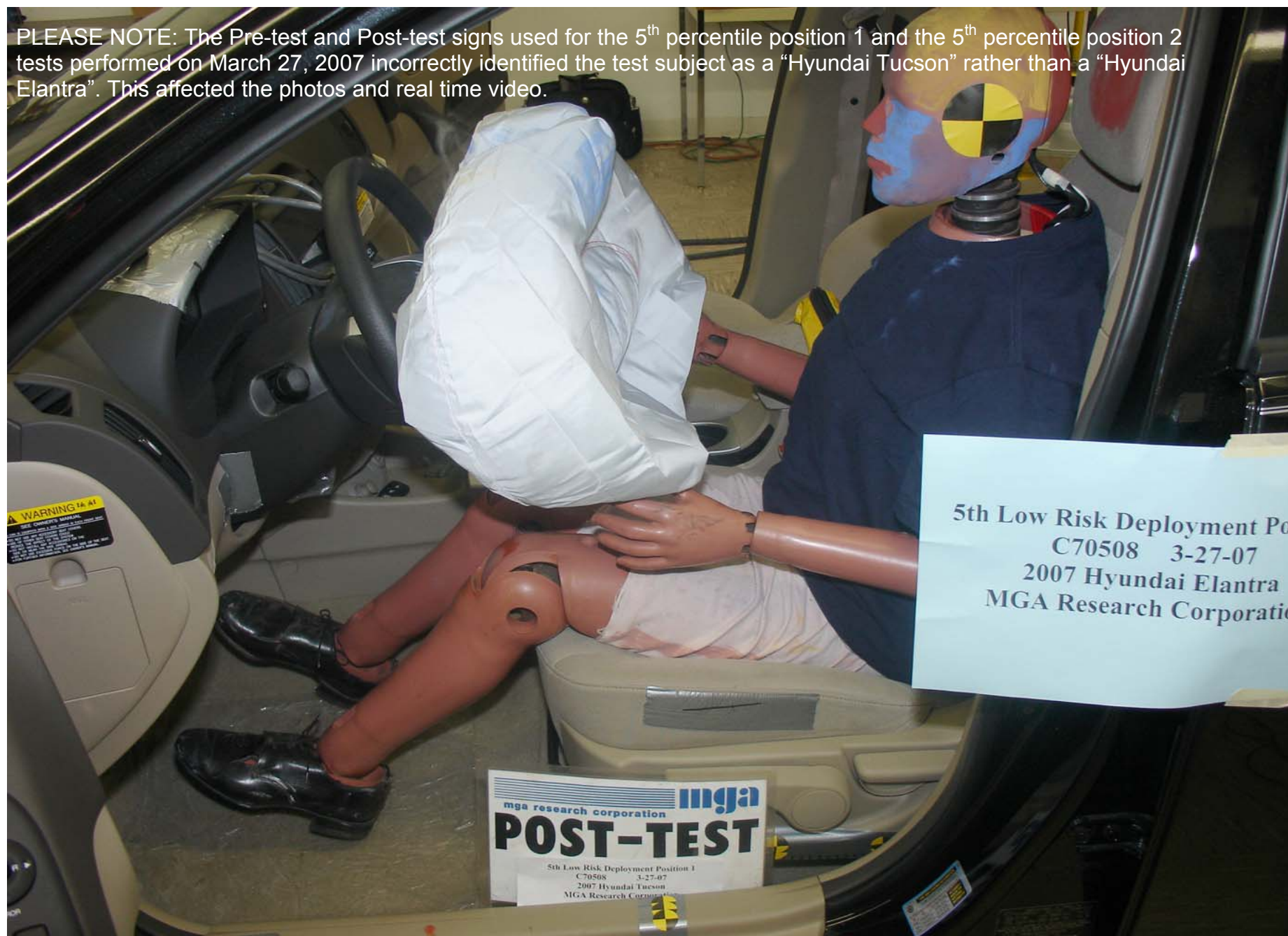
Post-Test 5th Fem. P1 Trial 1 Driver Dummy Left Side View (Door Open)
