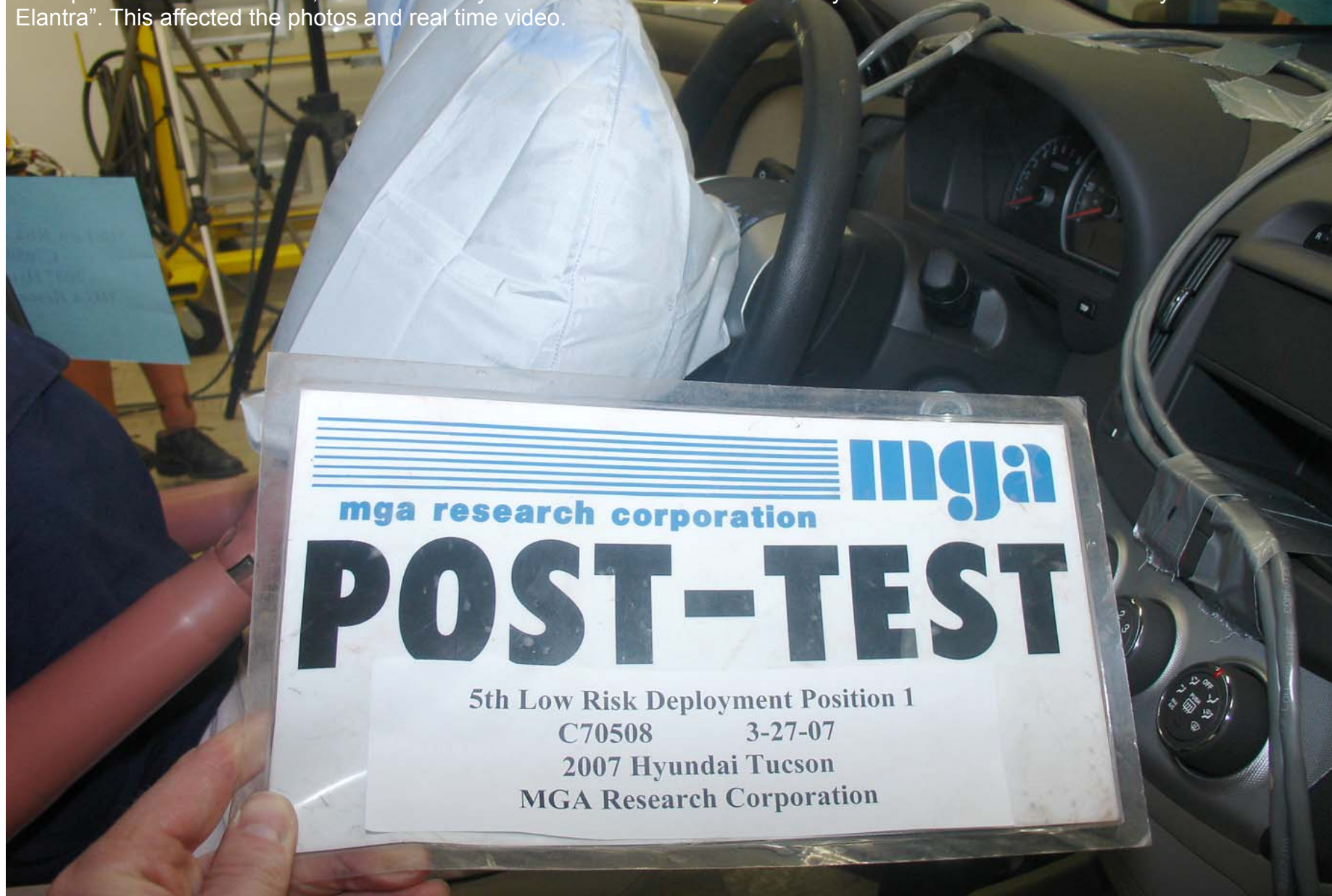
Post-Test 5th Fem. P1 Trial 1 Driver Dummy Airbag Right View
