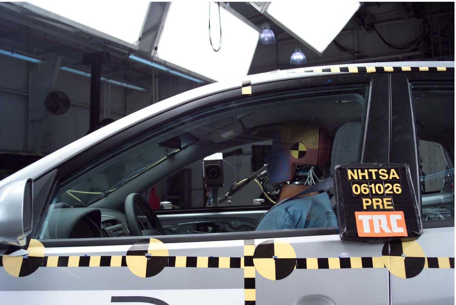
Figure A-41 Pre-Test Left View of Front SID HII
