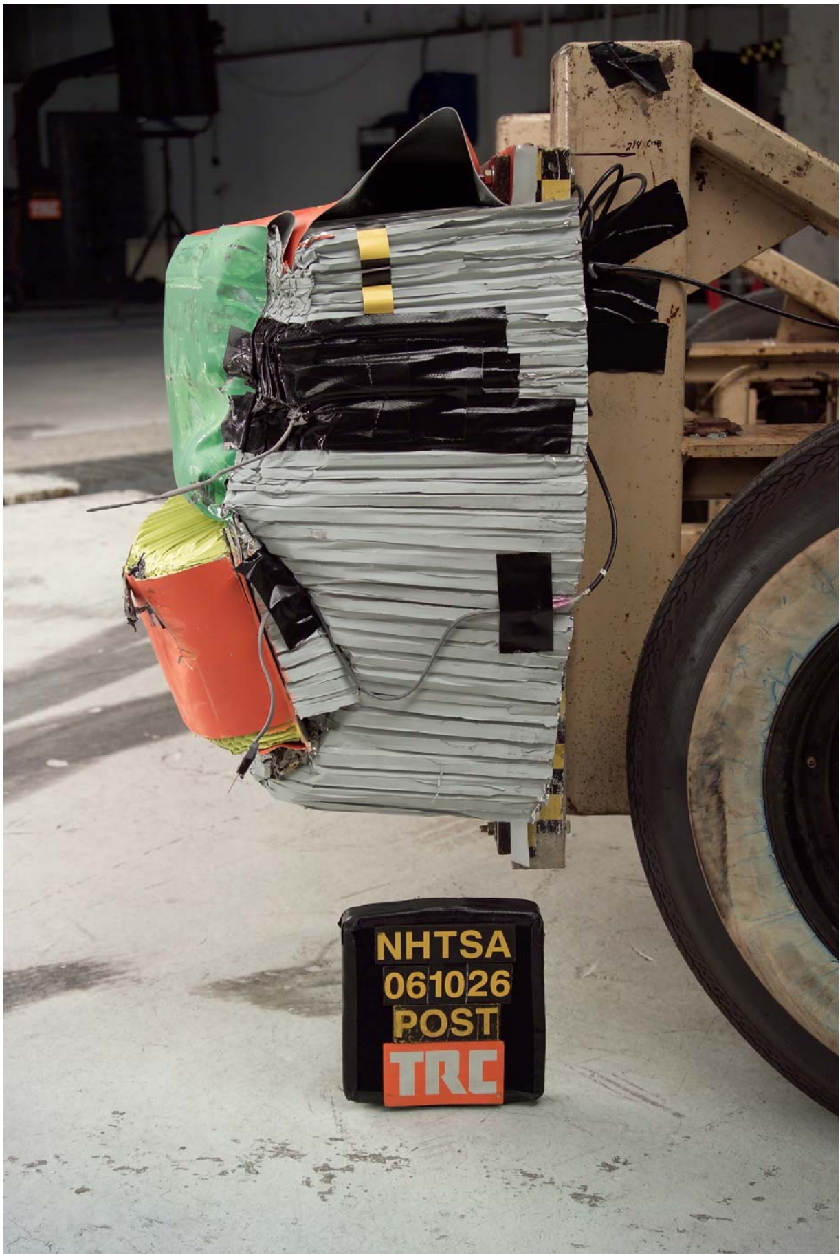
Figure A-22 Post-Test Left Side View of Impactor
