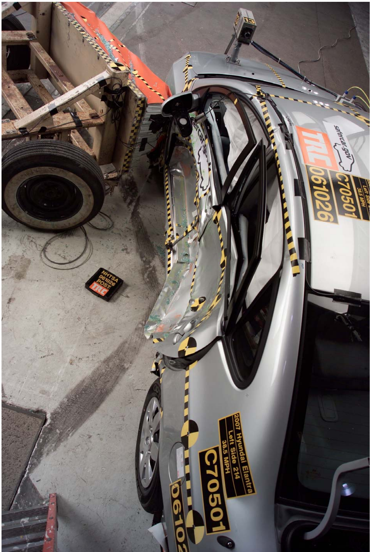
Figure A-36 Post-Test Overhead View of MDB and Vehicle
