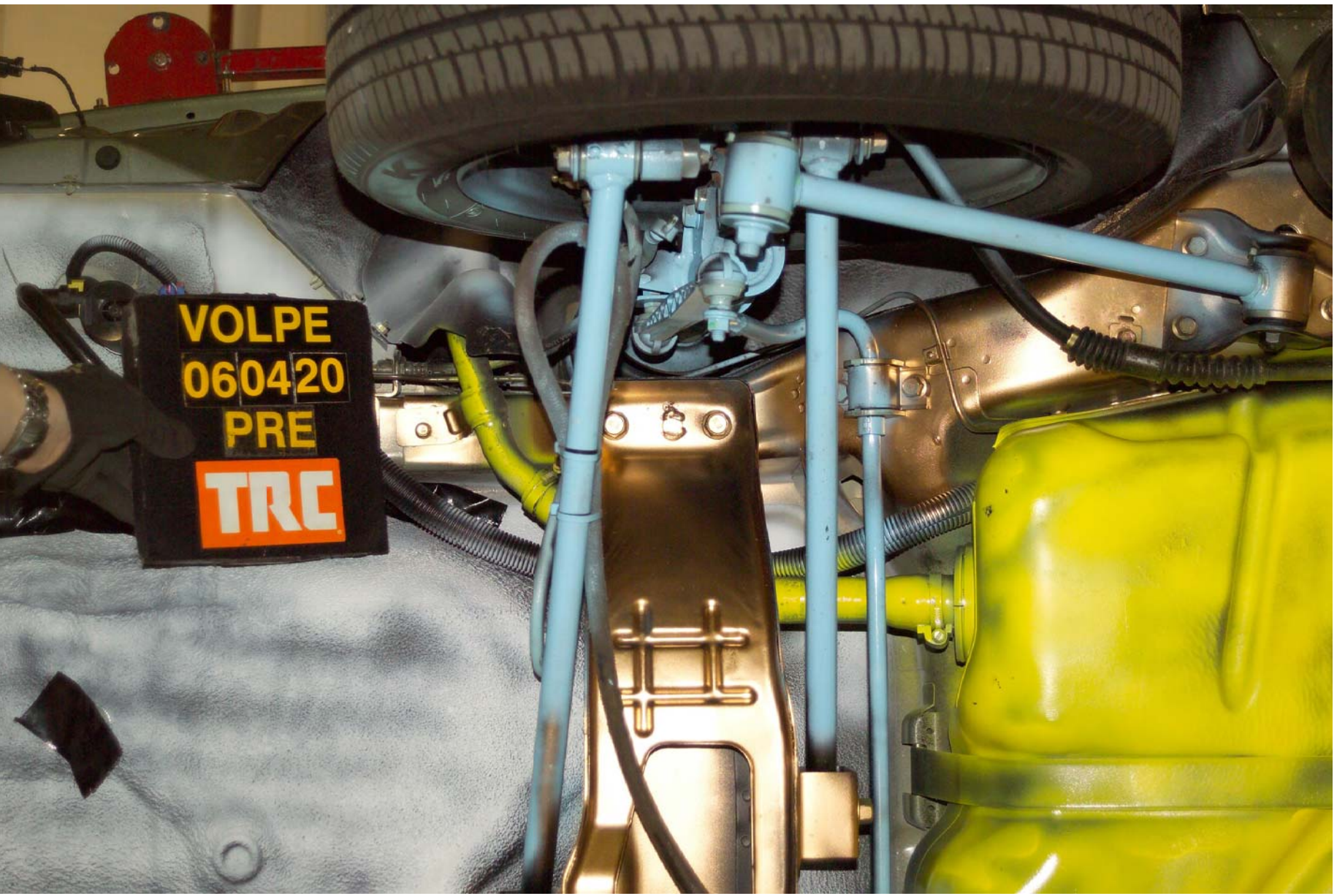
Figure A-35 Pre-Test Fuel Filler Neck View
