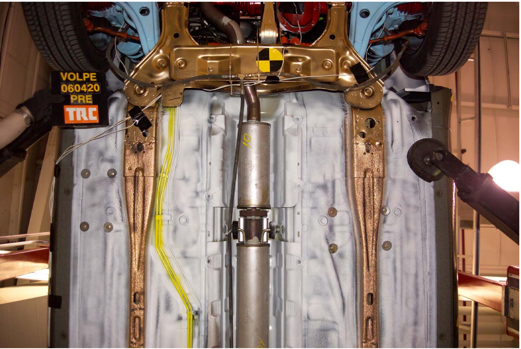
Figure A-25 Pre-Test Mid Front Underbody View
