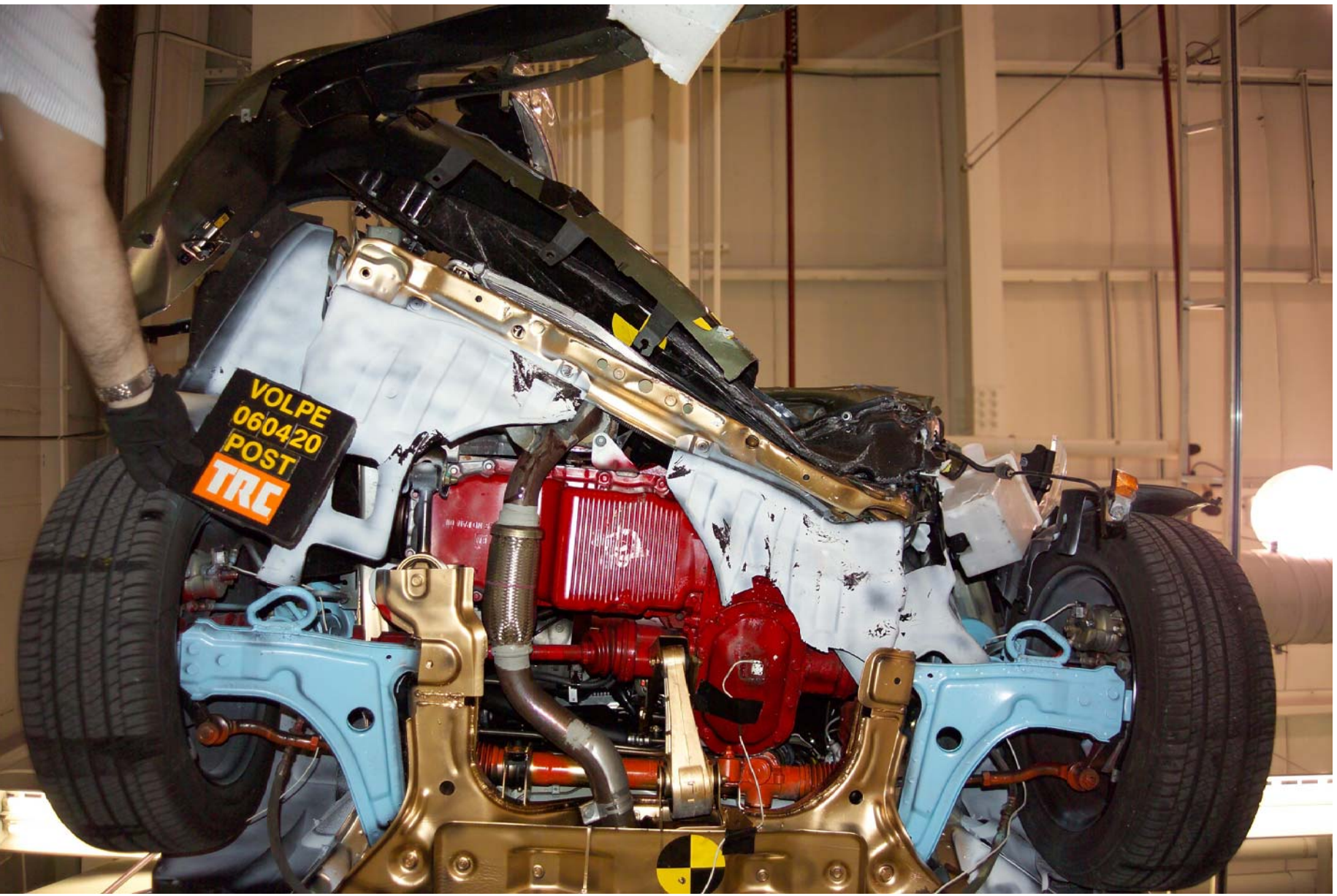
Figure A-24 Post-Test Front Underbody View
