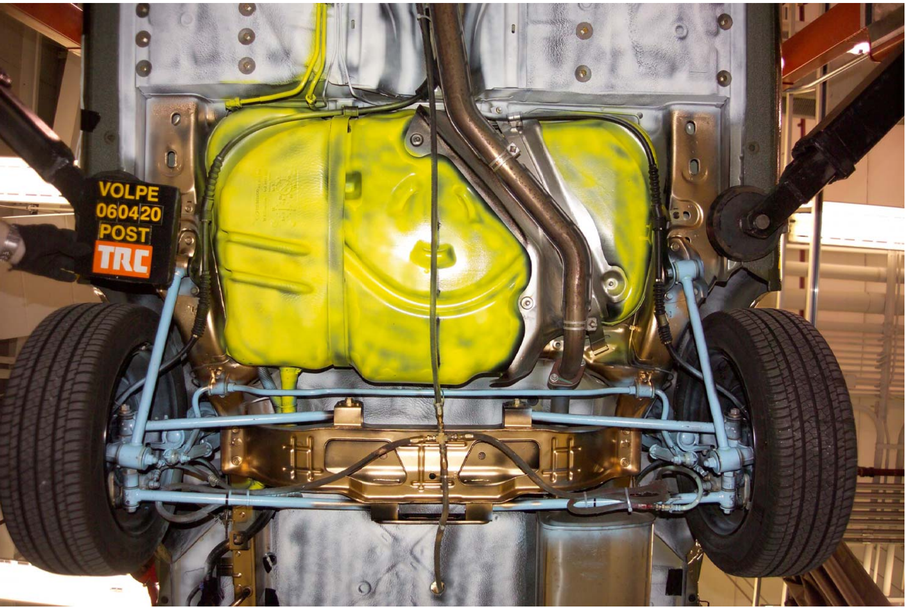
Figure A-30 Post-Test Mid Rear Underbody View
