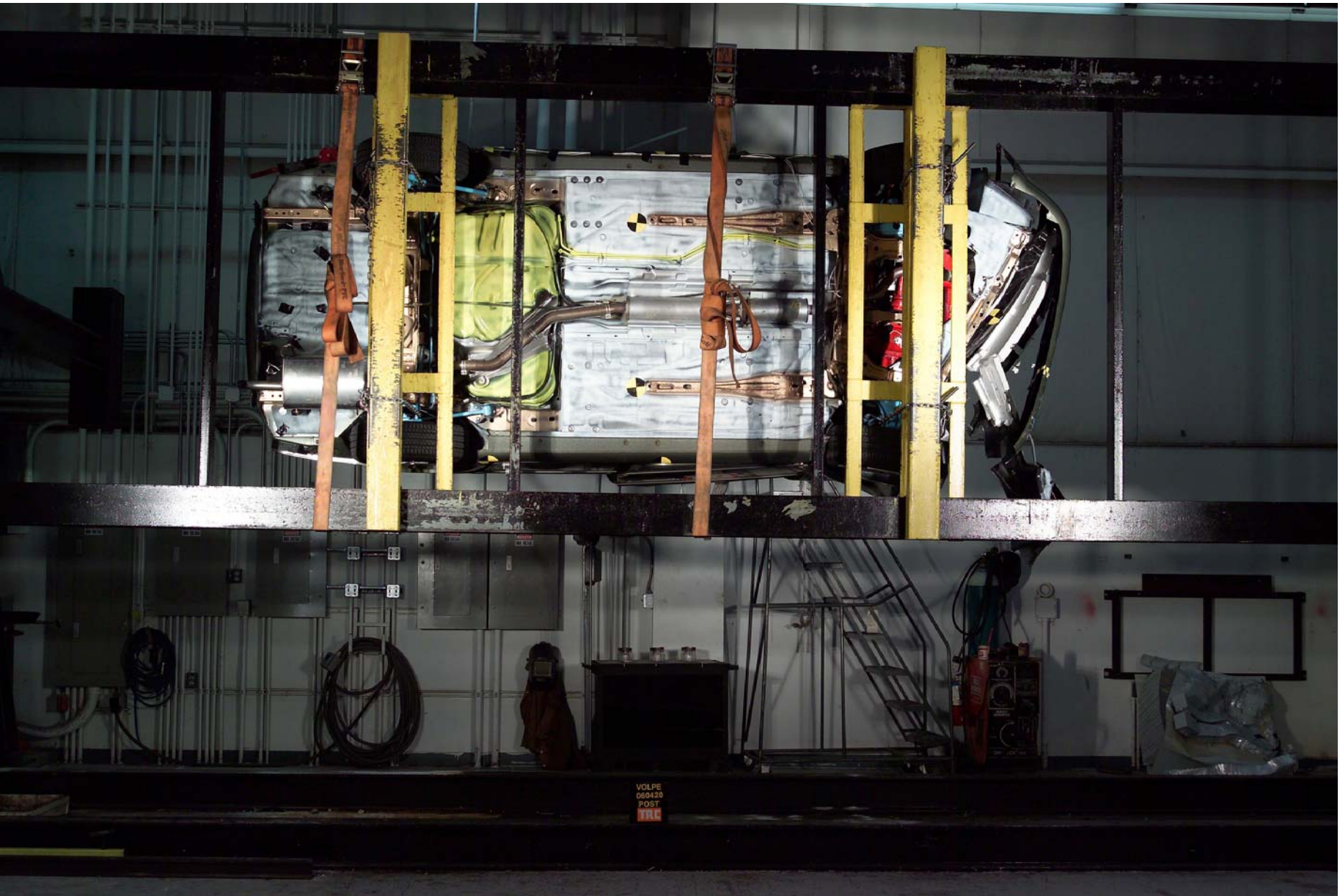
Figure A-69 Vehicle on Rollover Device - 270°
