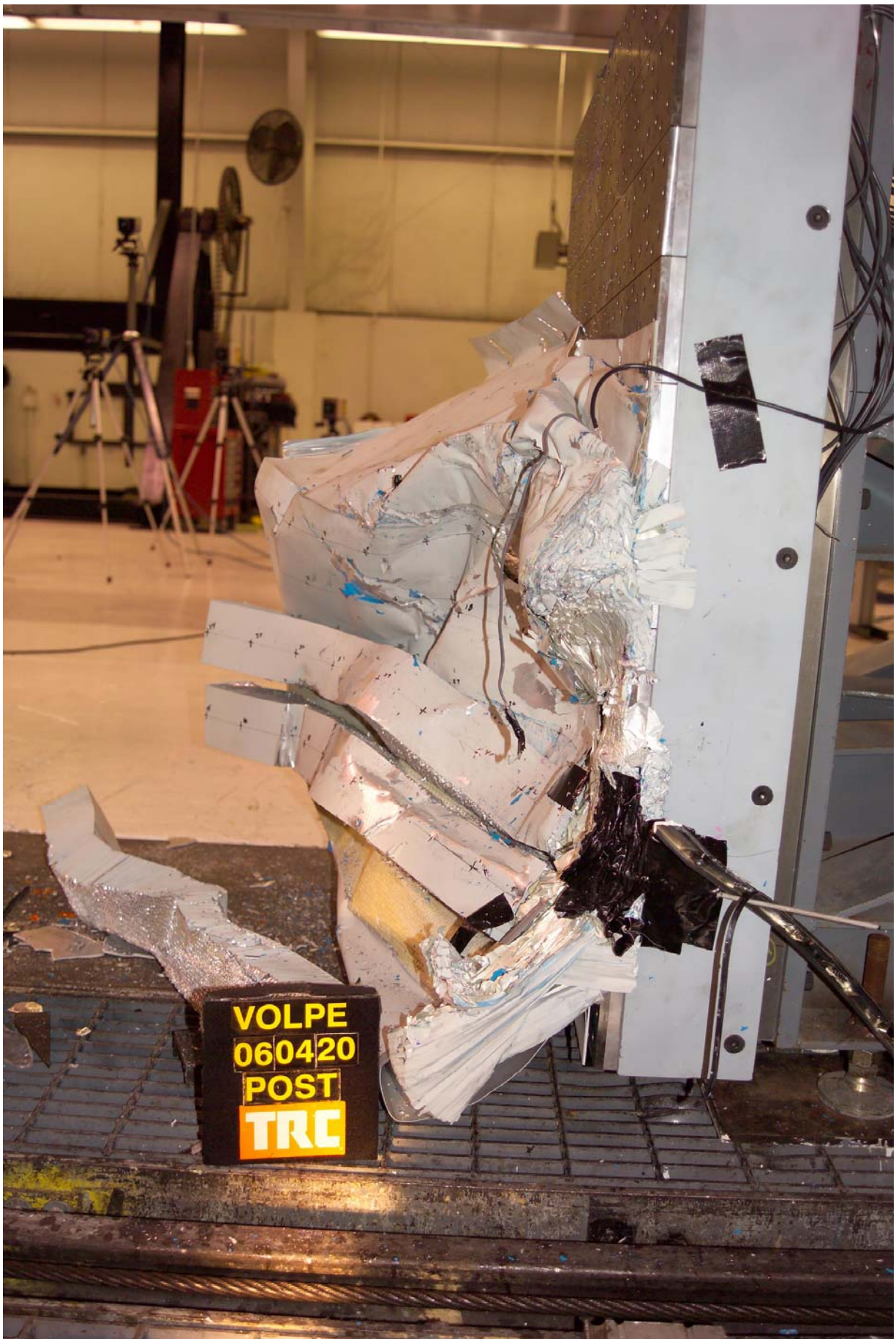
Figure A-64 Post-Test Barrier Right Side View
