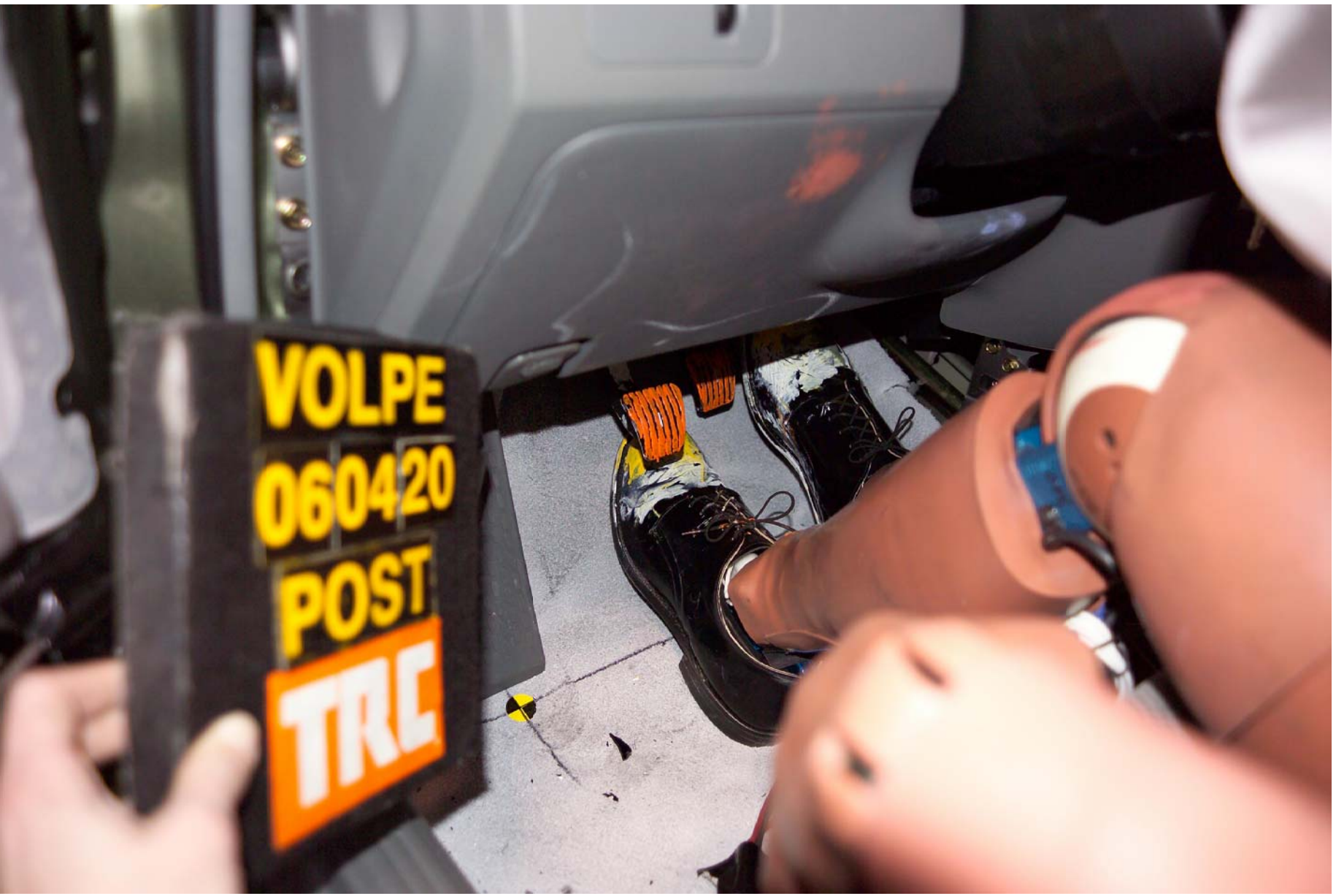
Figure A-50 Post-Test Driver Dummy Knee Contact - View 1
