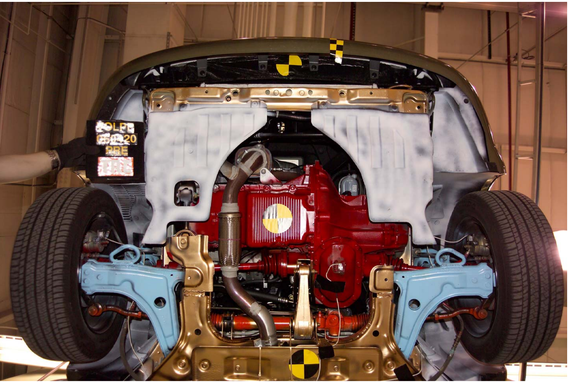
Figure A-23 Pre-Test Front Underbody View
