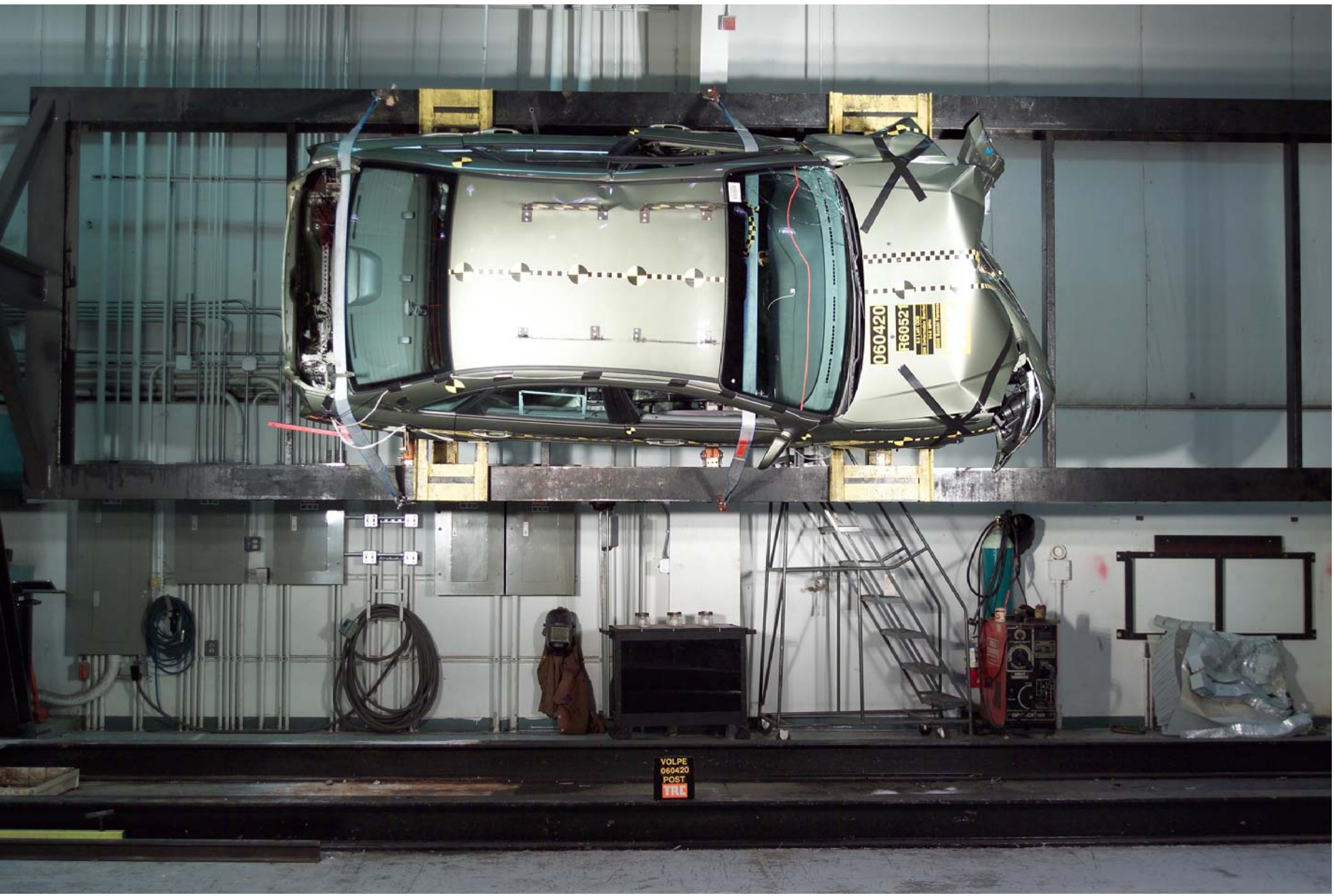
Figure A-67 Vehicle on Rollover Device - 90°
