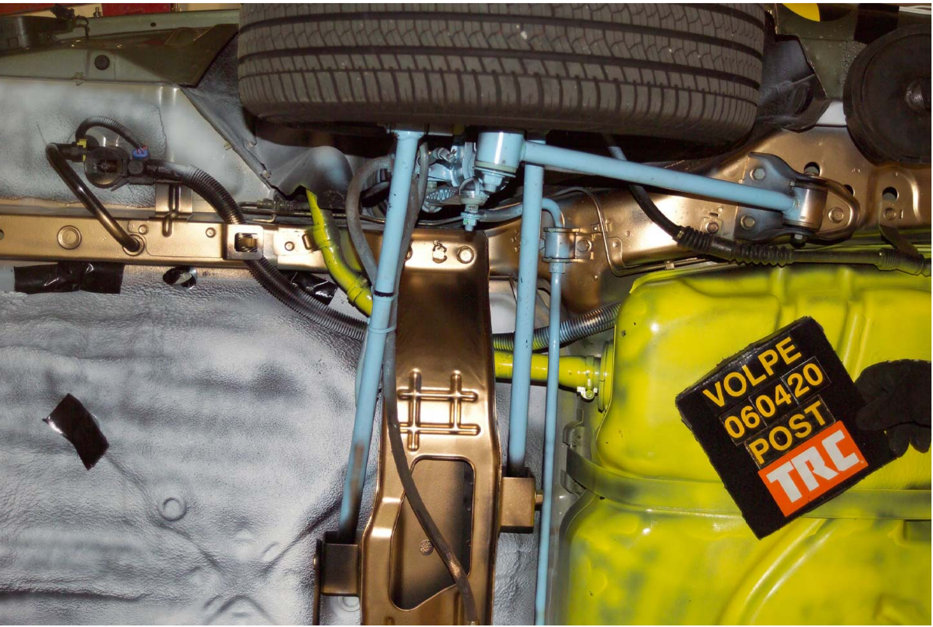
Figure A-36 Post-Test Fuel Filler Neck View
