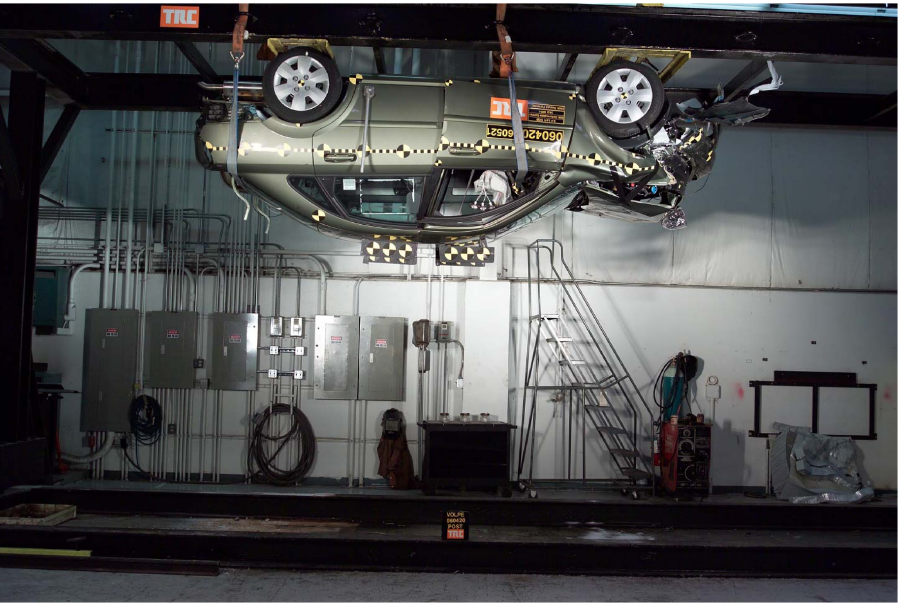
Figure A-68 Vehicle on Rollover Device - 180°
