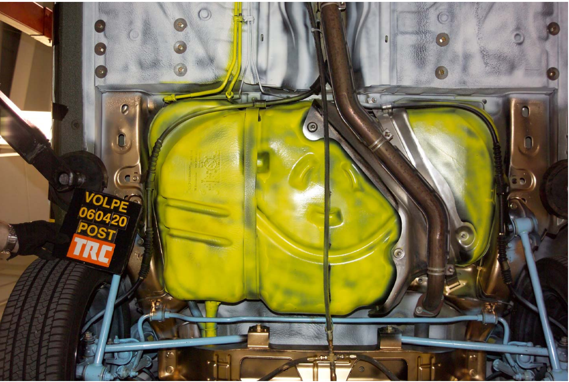
Figure A-34 Post-Test Fuel Tank View
