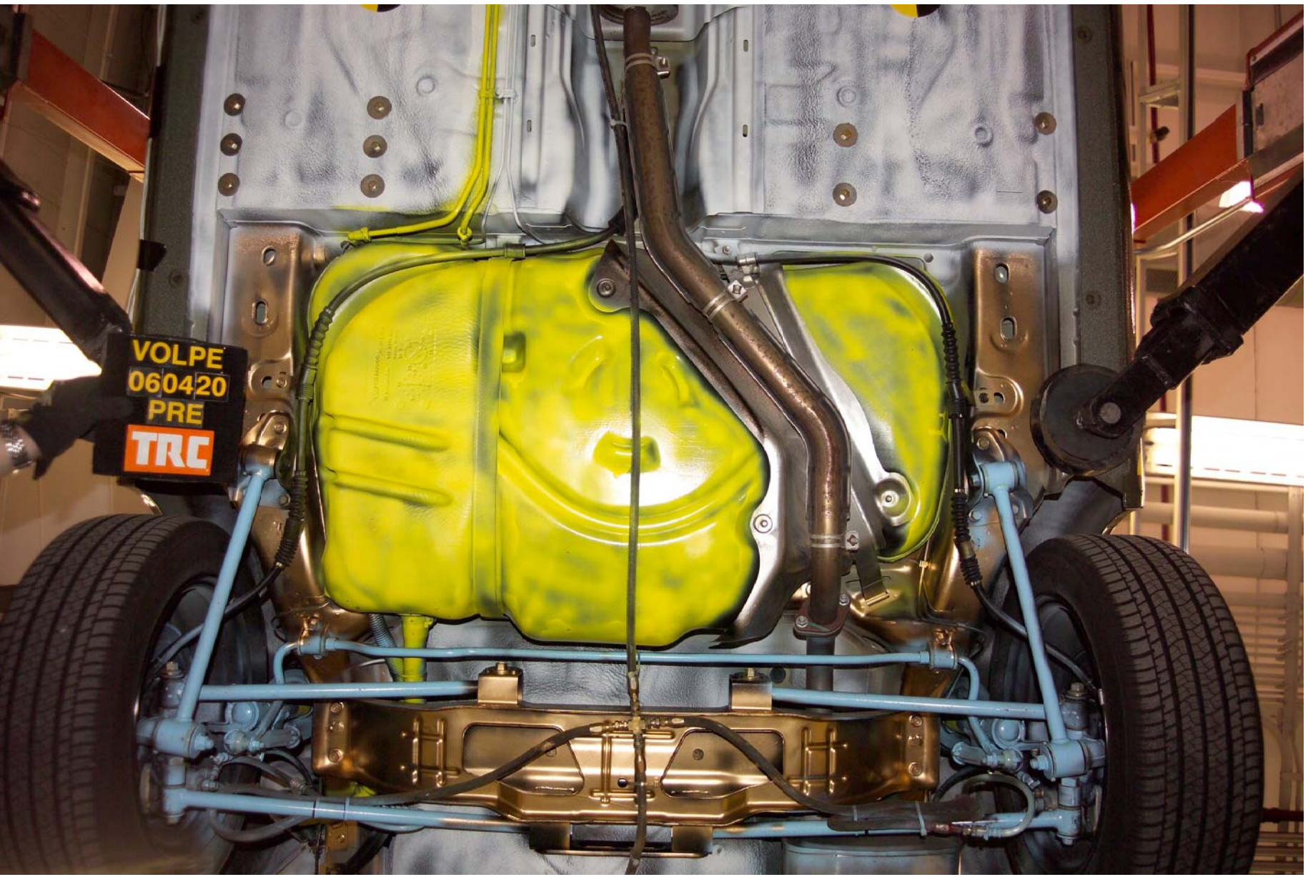
Figure A-29 Pre-Test Mid Rear Underbody View
