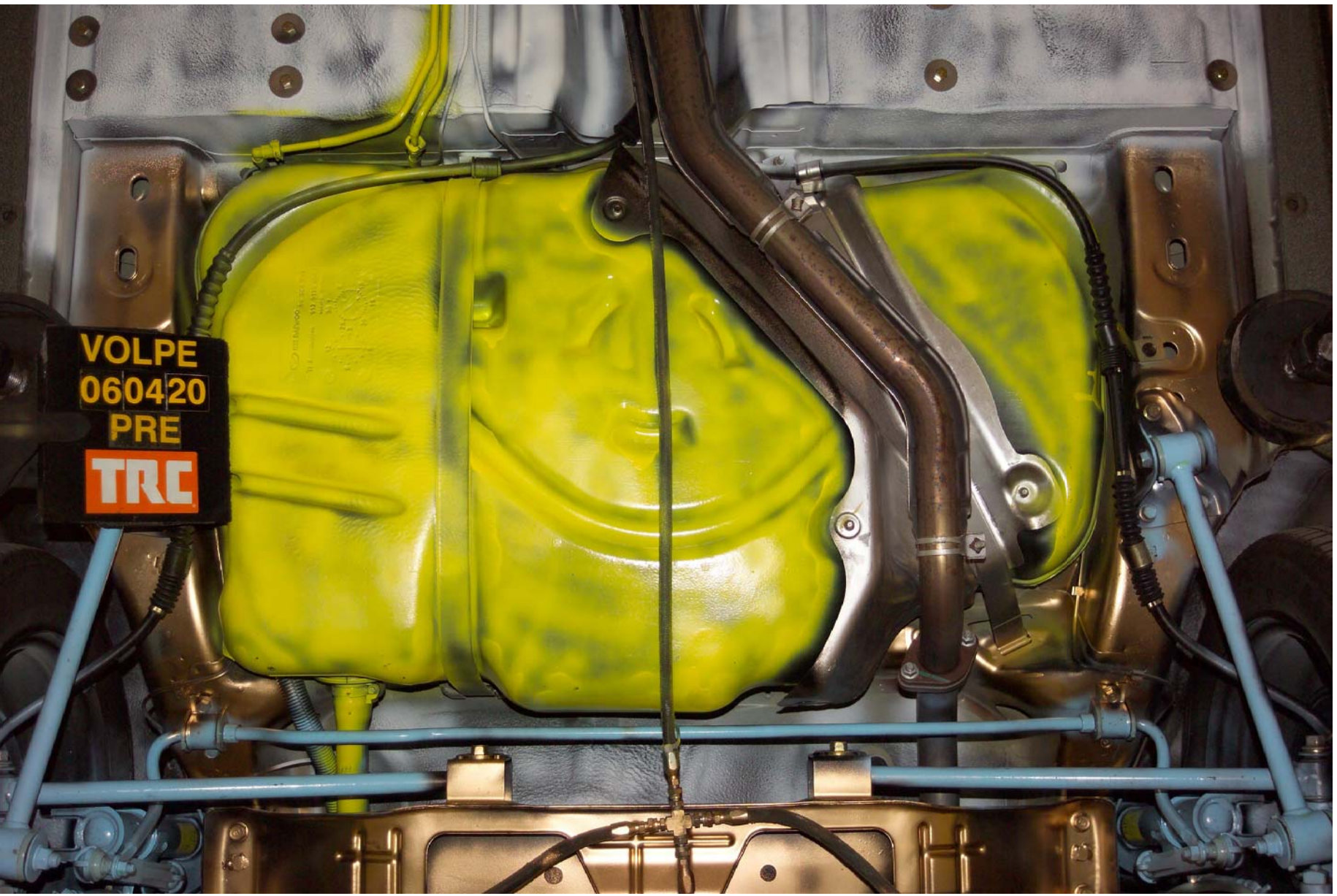
Figure A-33 Pre-Test Fuel Tank View
