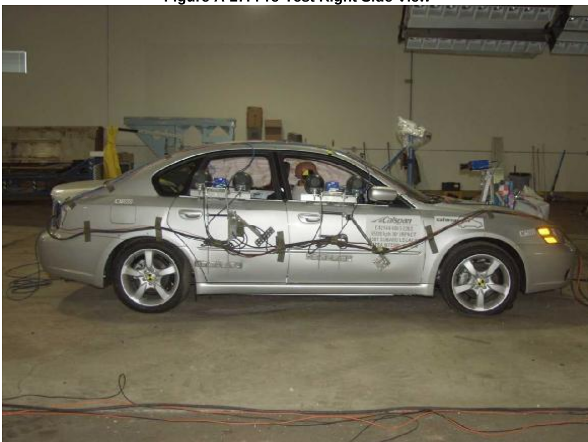
Figure A-18: Post-Test Right Side View
