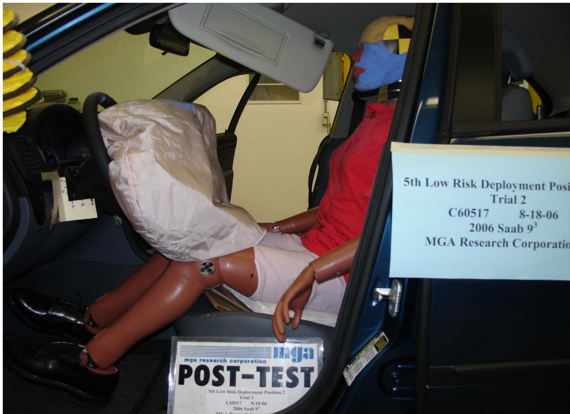
Post-Test 5th Fem. P2 Trial 2 Driver Dummy Left Side View (Door Open)
