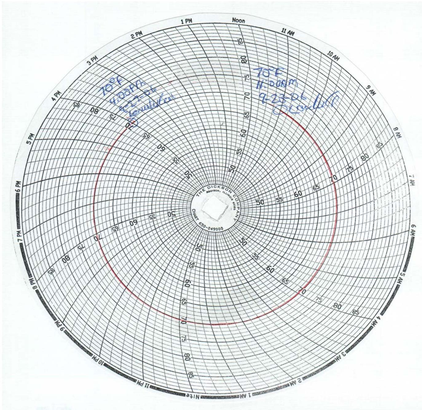
Temperature Plot
