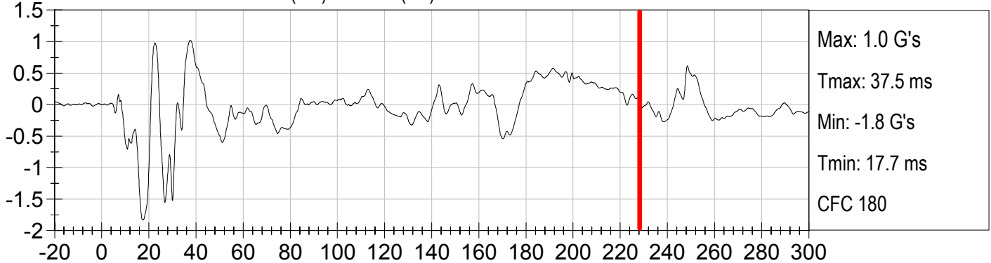
5TH FEM. DRIVER CHEST Z (G's) vs TIME (ms)
