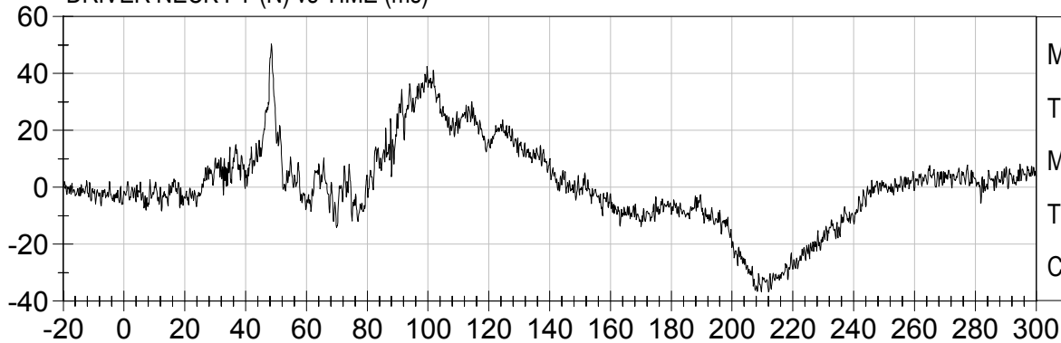
DRIVER NECK FZ (N) vs TIME (ms)
