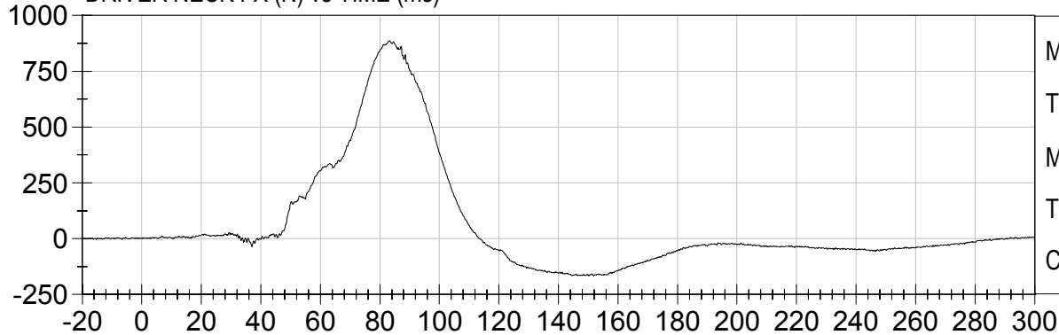
DRIVER NECK FY (N) vs TIME (ms)
