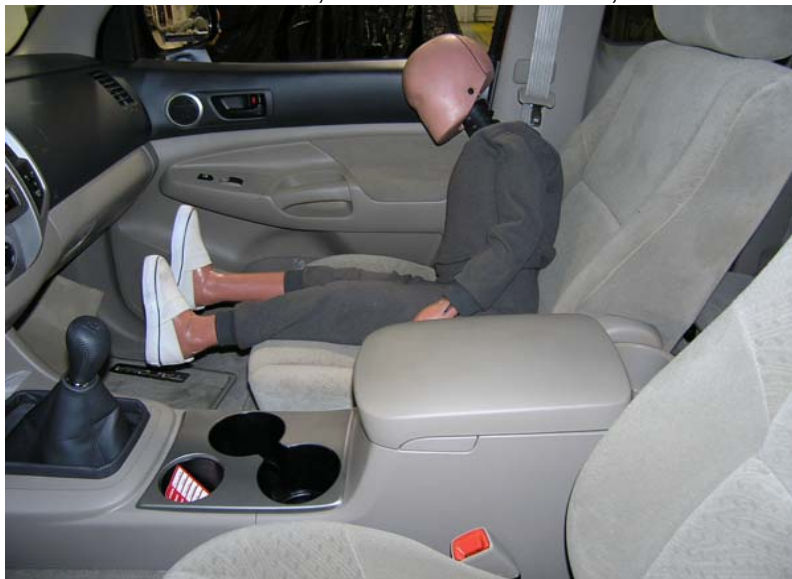
6-Year-Old Unbelted, Rearward Seat Track, Position 4, View 2
