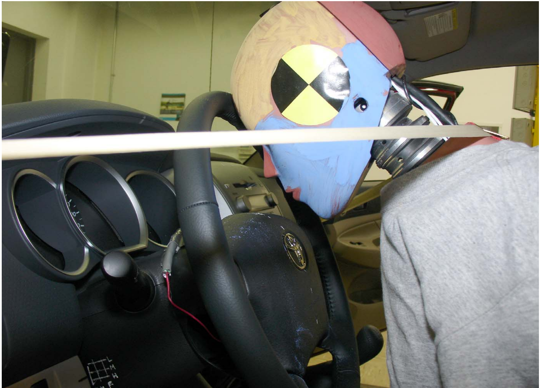
Pre-Test 5th Fem. P1 Driver Dummy Left Side Head Position View
