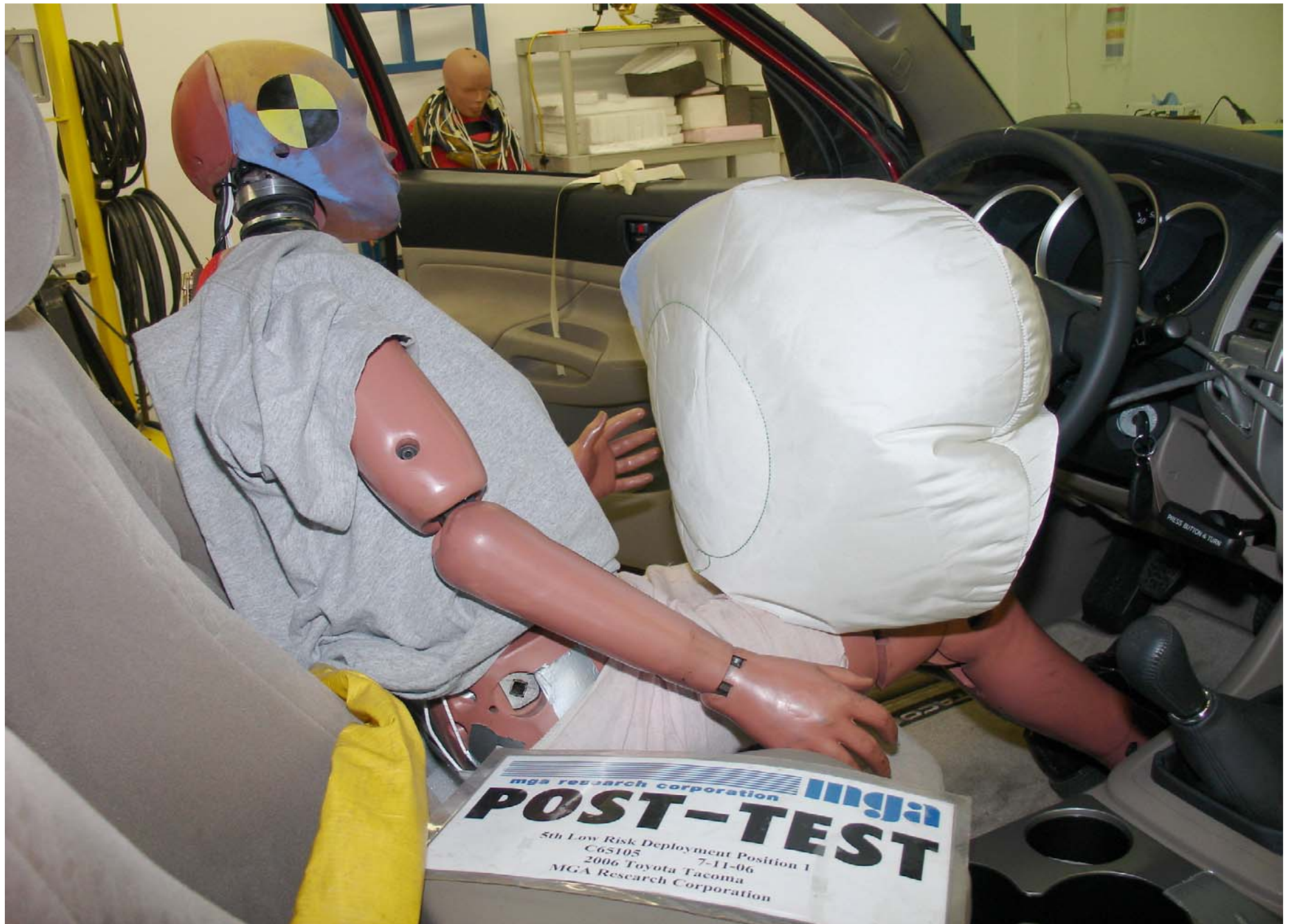
Post-Test 5th Fem. P1 Driver Dummy Airbag Right View
