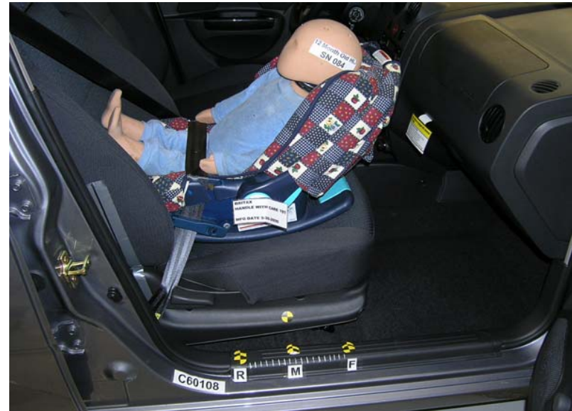
Britax Handle With Care 191 With Belt, Middle Seat Track, Handle Down
