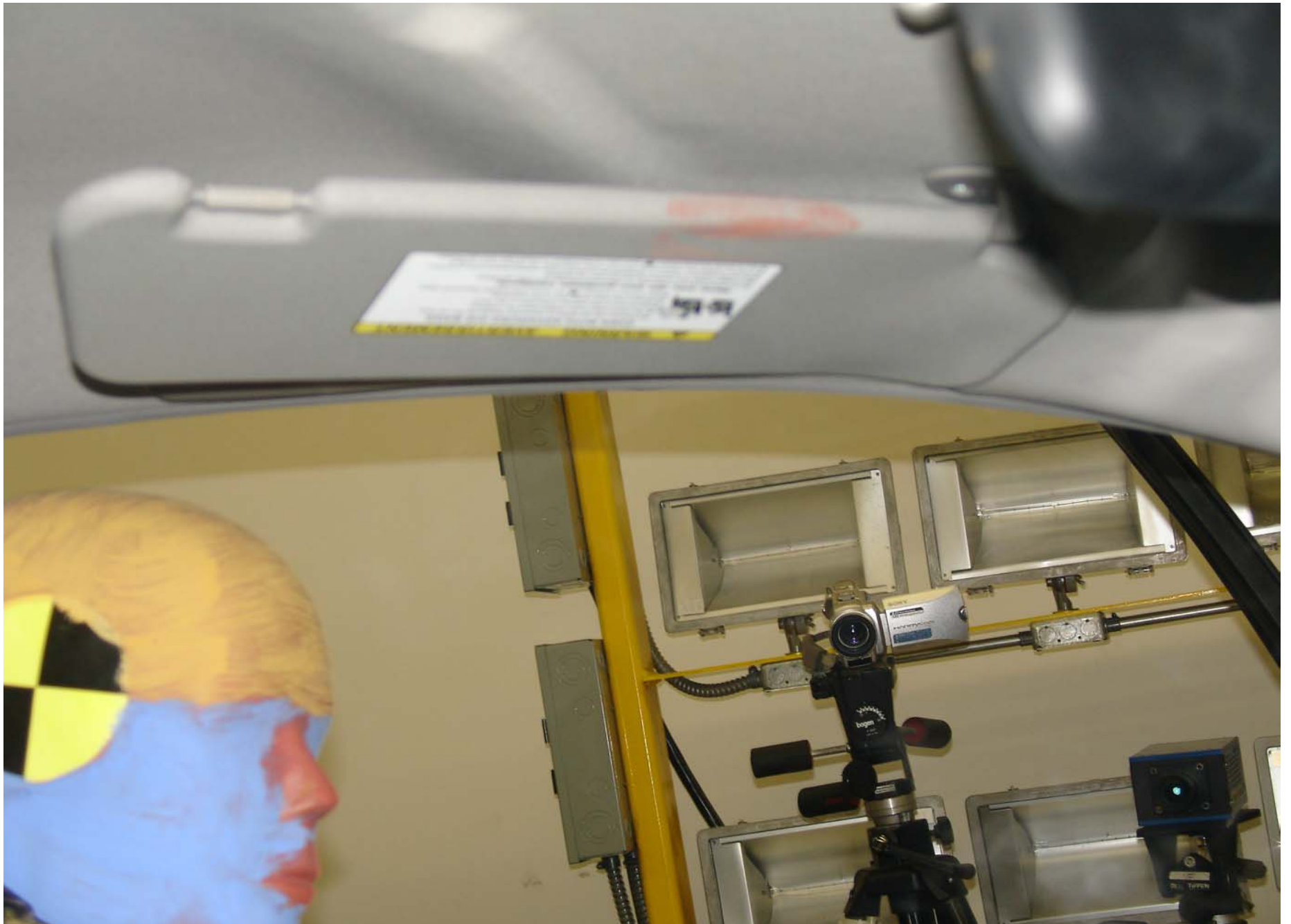
Post-Test 5th Fem. P2 Driver Dummy Head Contact (visor)
