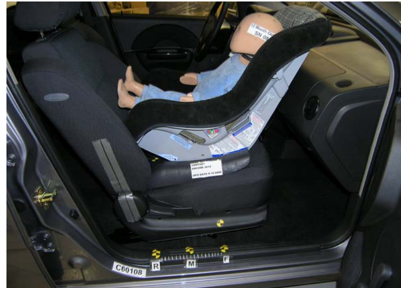
Century Encore Rear Facing Unbelted, Forward Seat Track
