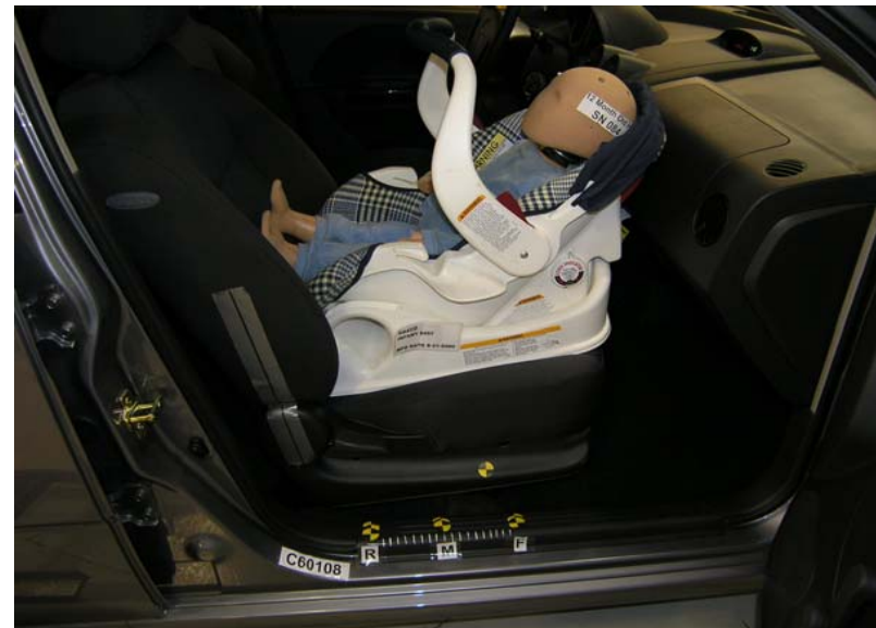
Graco Infant W/ Base Unbelted, Forward Seat Track, Handle Up
