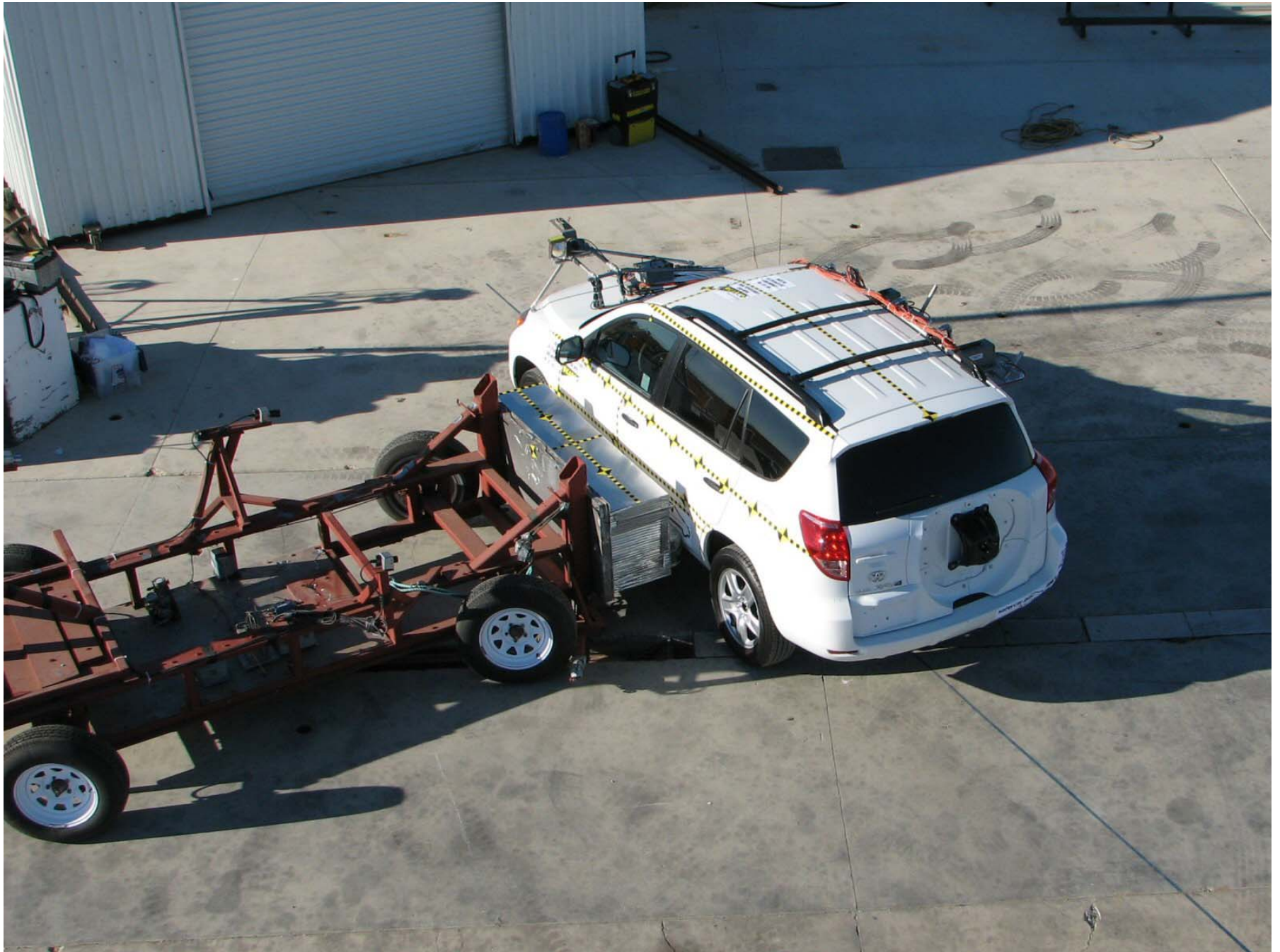
Figure A-21: Pre-Test Overhead View
