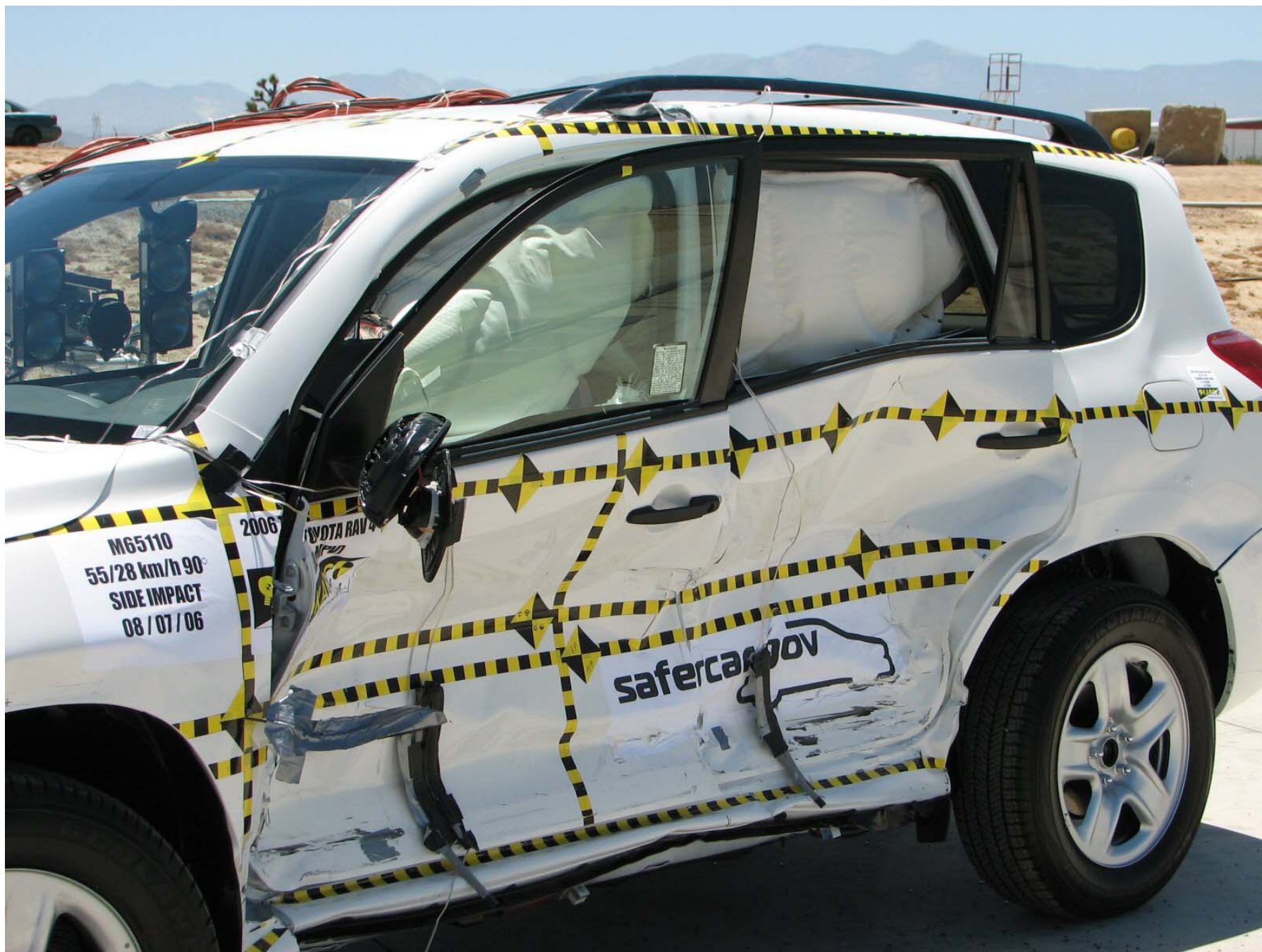
Figure A-28: Post-Test Front \frac{3}{4} View of Left Side Door
