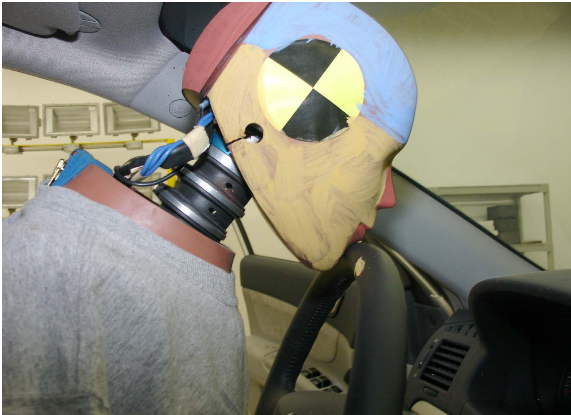
Pre-Test 5th Fem. P2 Driver Dummy Right Side Head Position View Trial 2
