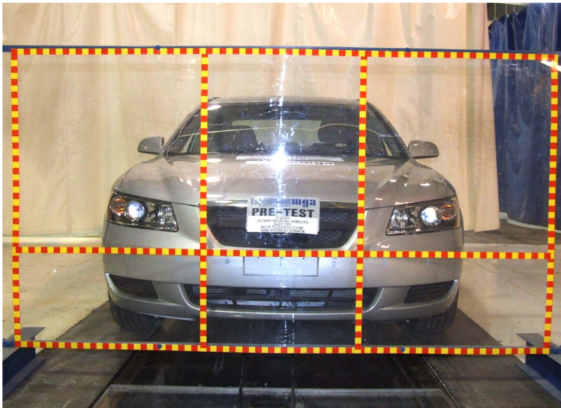
Vehicle in Relation to The Load Cell Grid
