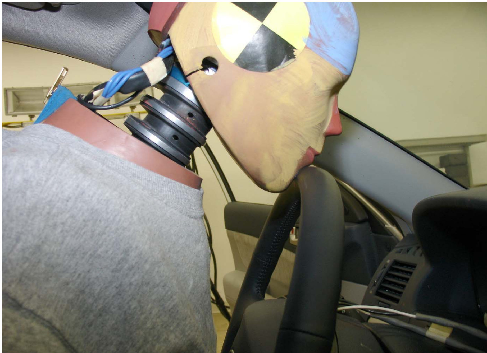
Pre-Test 5th Fem. P2 Driver Dummy Right Side Head Position View Trial 3
