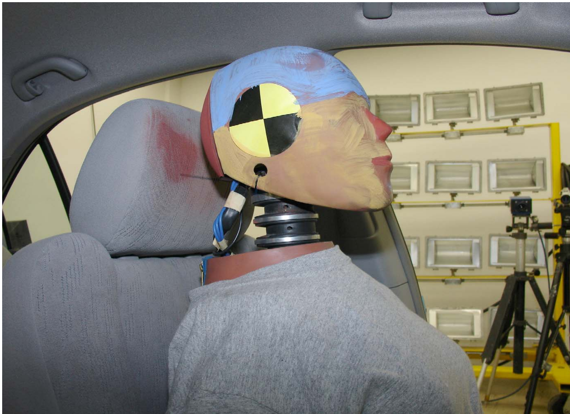
Post-Test 5th Fem. P2 Driver Dummy Right Side Head Position View Trial 3
