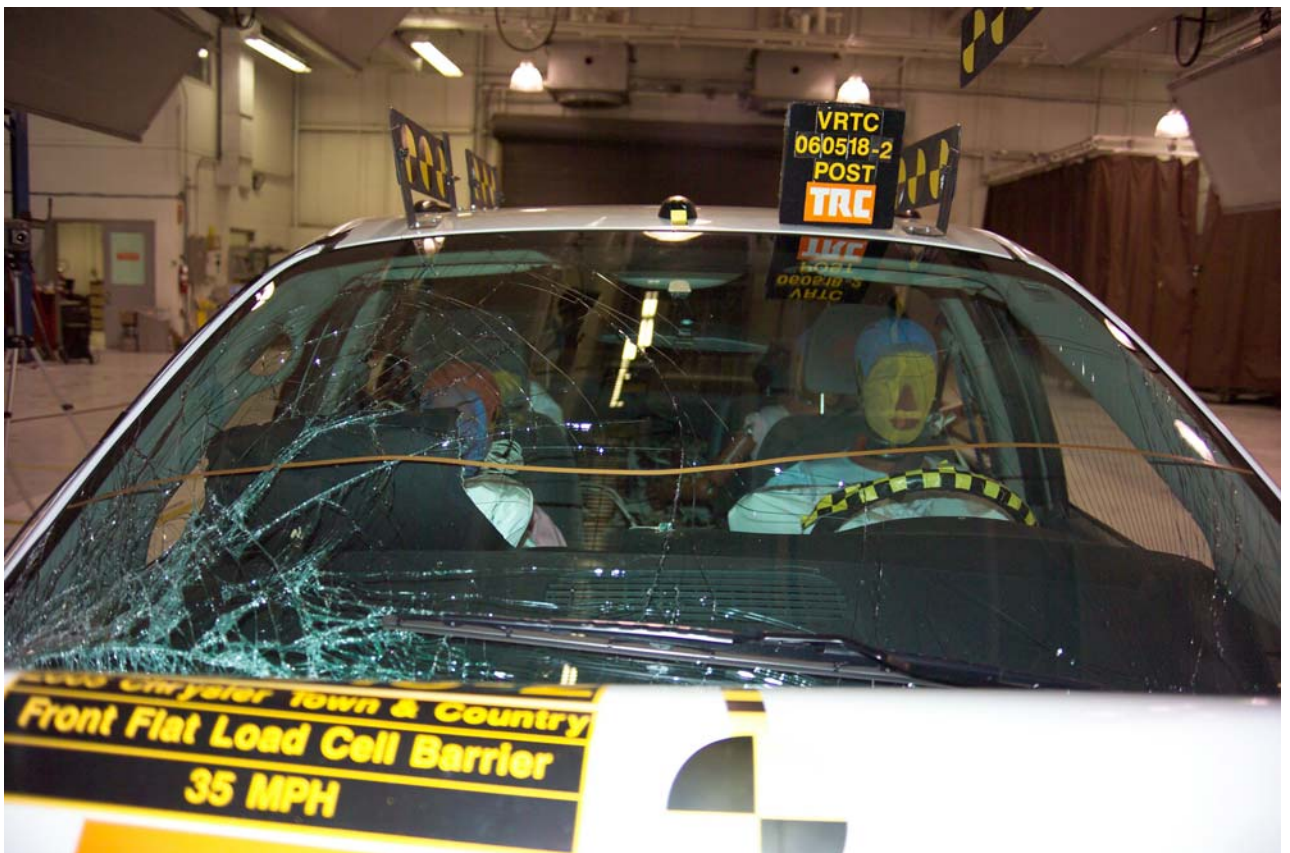
Figure A-31 Post-Test Windshield View
