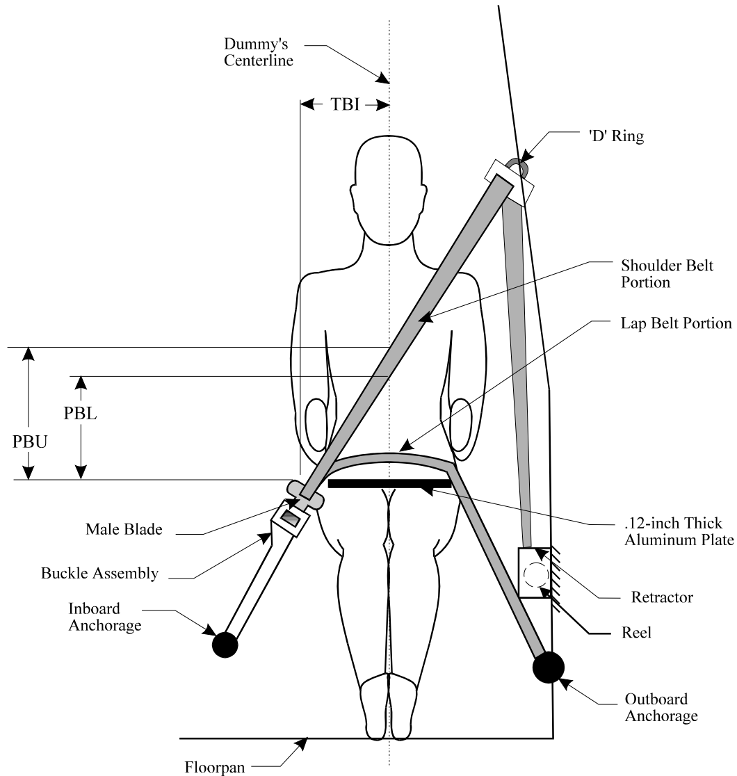
Figure 4 Seat Belt Positioning Data, Continued
