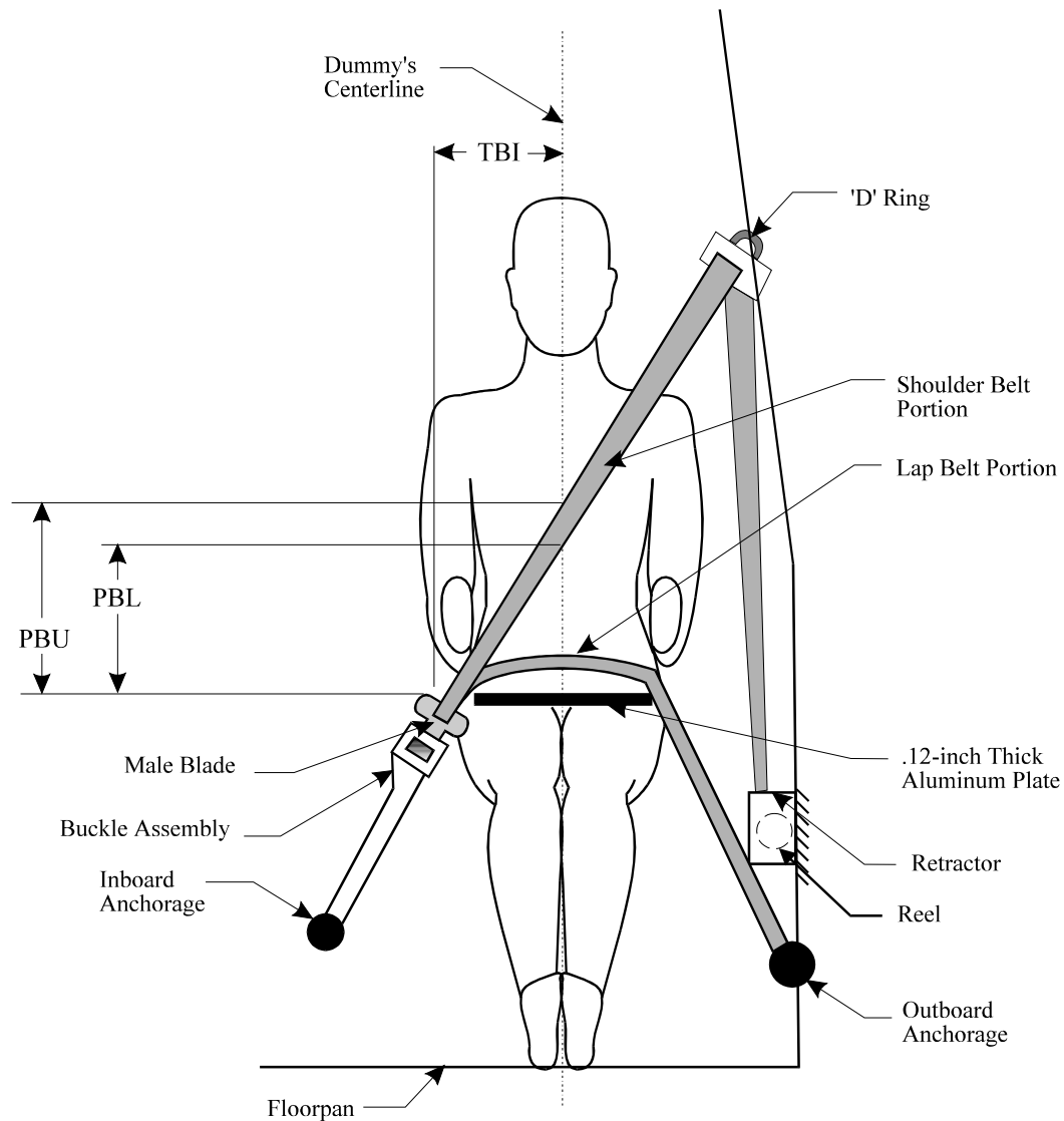
Figure 4 Seat Belt Positioning Data
