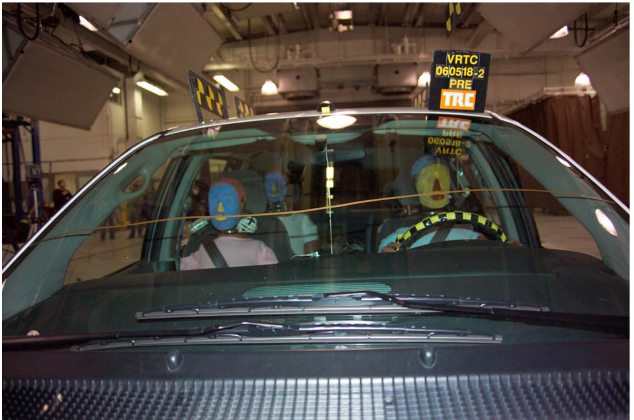
Figure A-30 Pre-Test Windshield View
