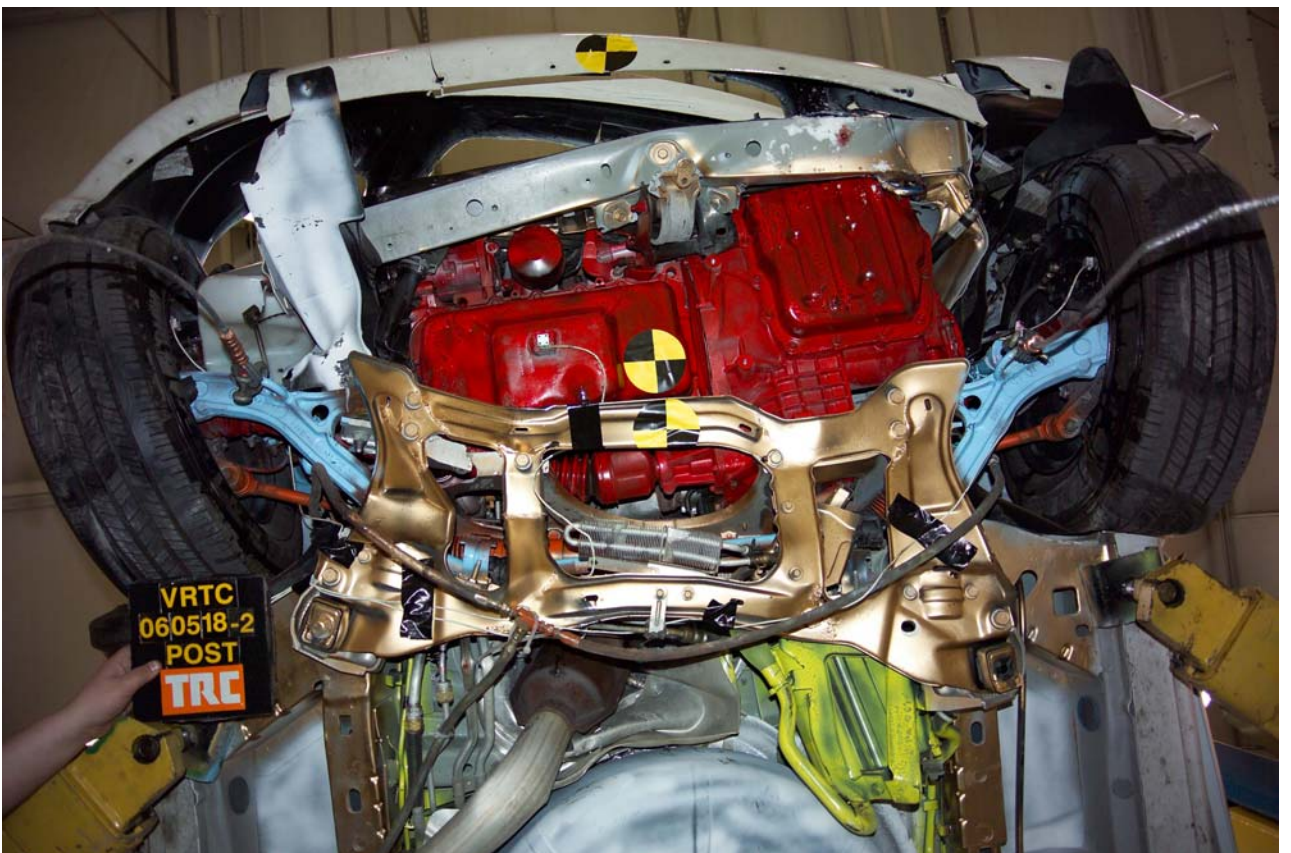
Figure A-21 Post-Test Front Underbody View
