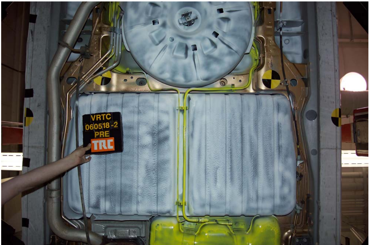
Figure A-24 Pre-Test Mid Underbody View
