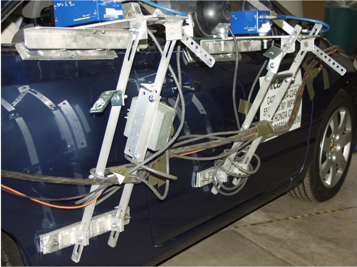
Figure A-49: Pre-Test Left Rear \frac{3}{4} View of Left Side Door
