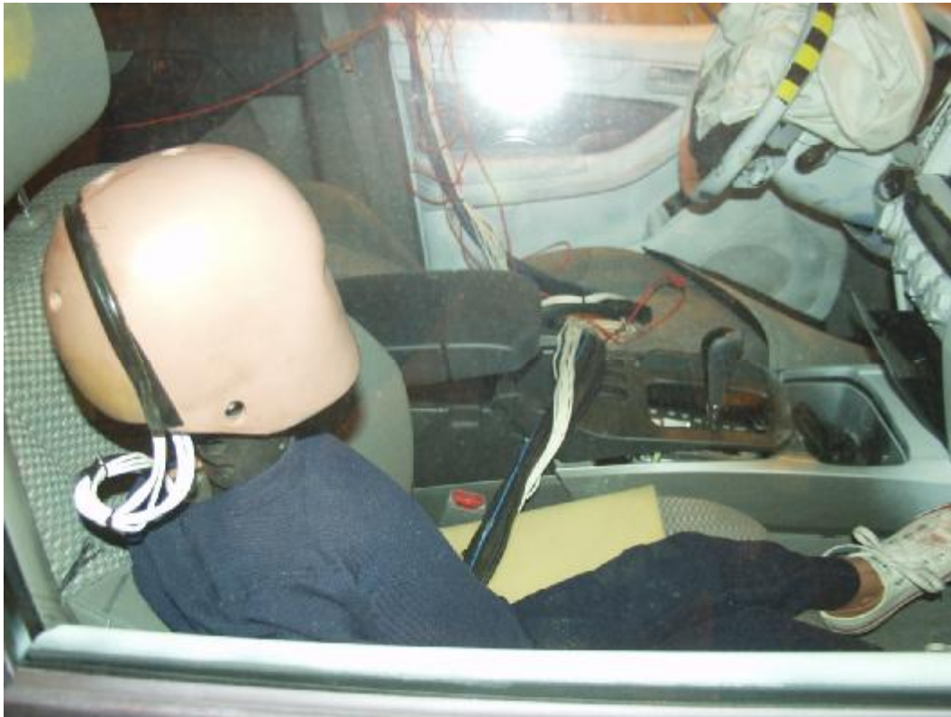
Figure A-9: Pre-Test Right Side of Dummy View
