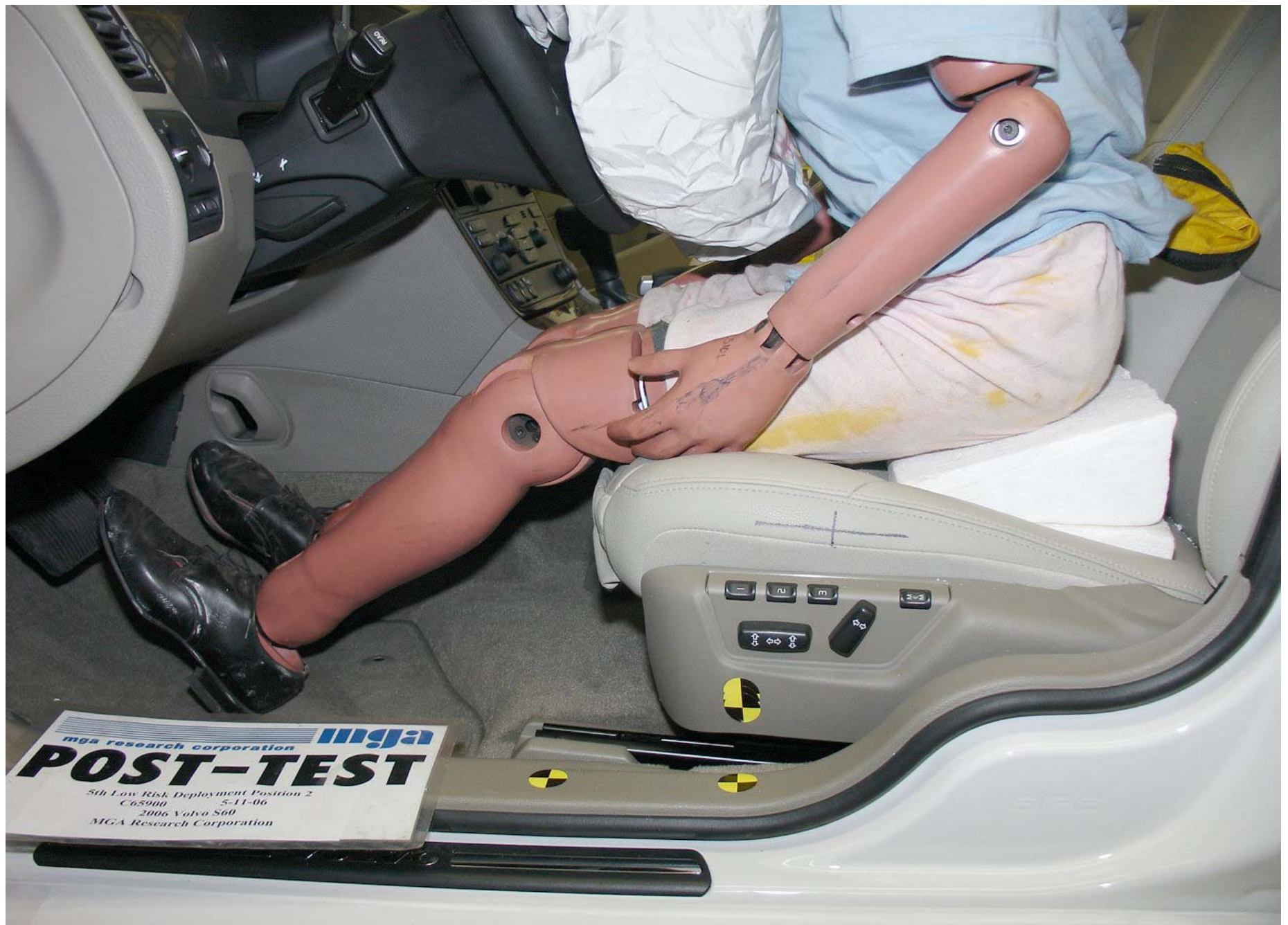
Post-Test 5th Fem. P2 Driver Dummy Left Side Mid Position View
