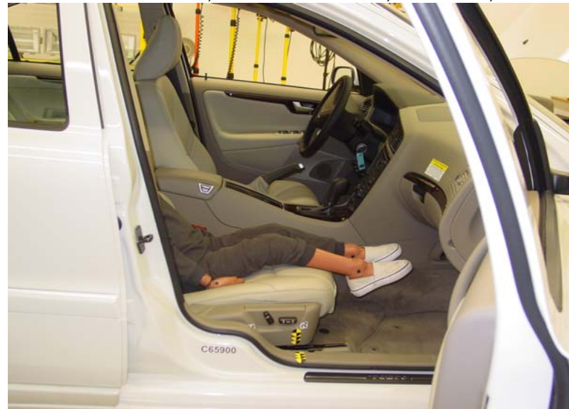
6-Year-Old Unbelted, Rearward Seat Track, Position 2
