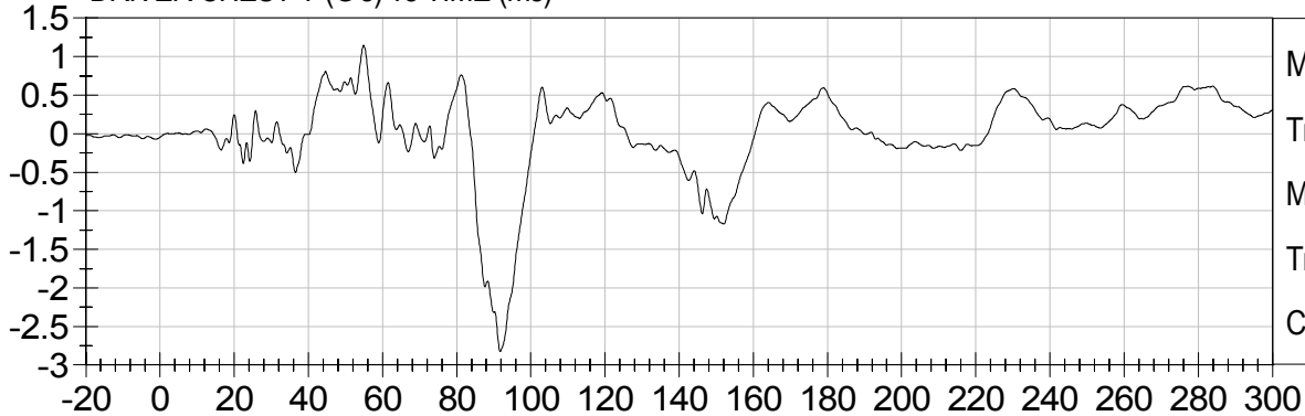
DRIVER CHEST Z (G's) vs TIME (ms)
