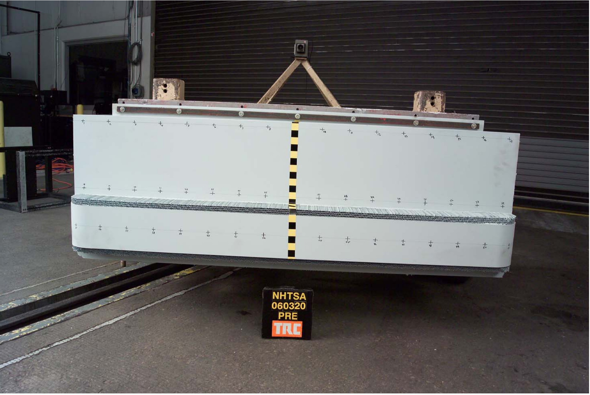
Figure A-24 Pre-Test Front View of Impactor
