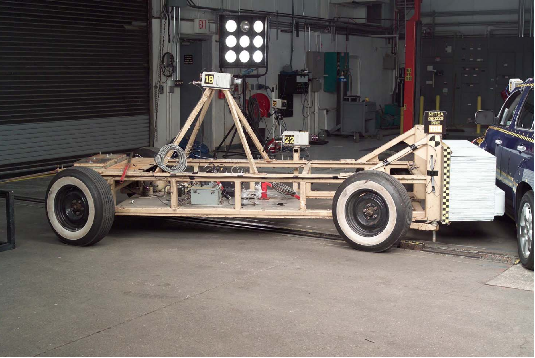
Figure A-34 Pre-Test Right Side Overall View of Impactor A-38
