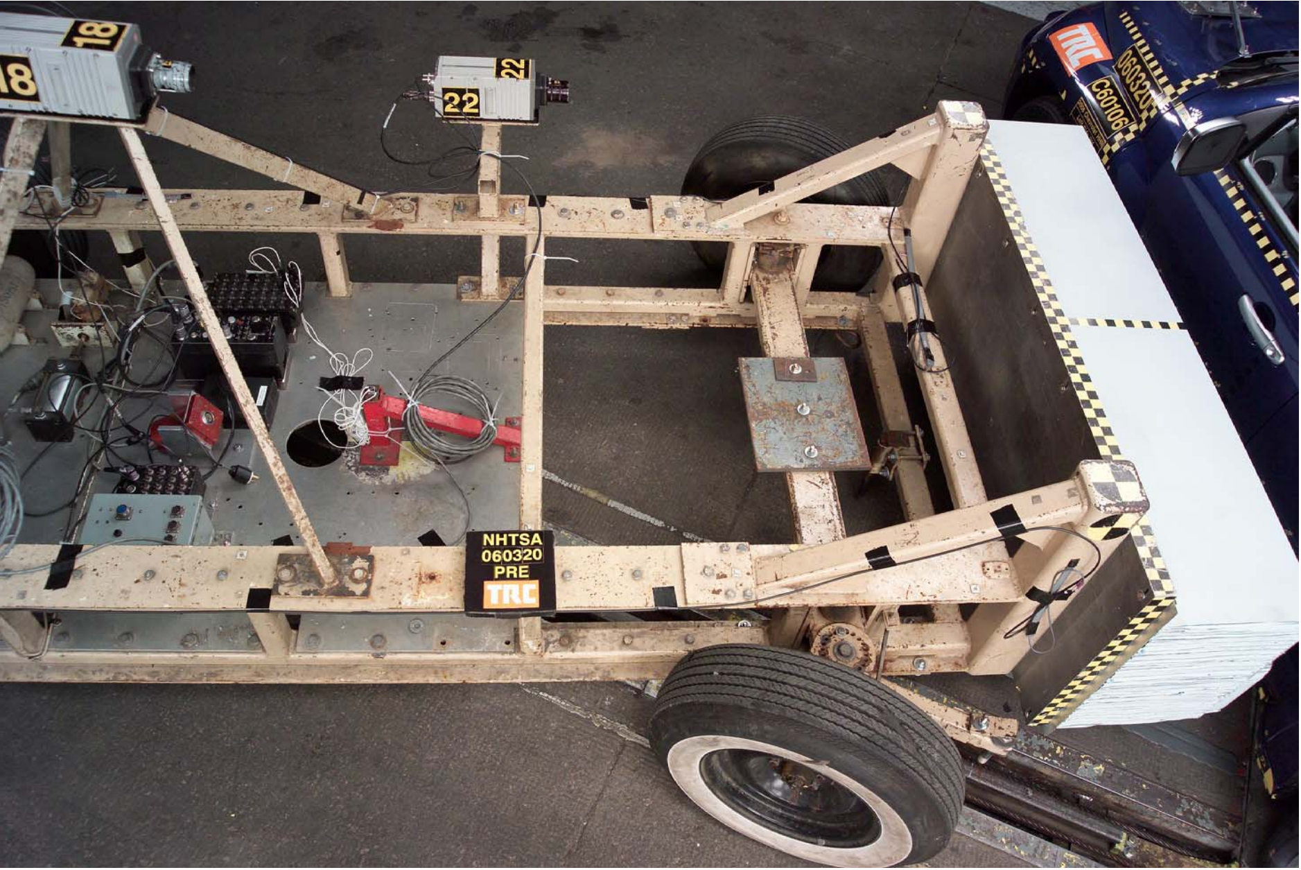
Figure A-36 Pre-Test Top Overall View of Impactor A-40
