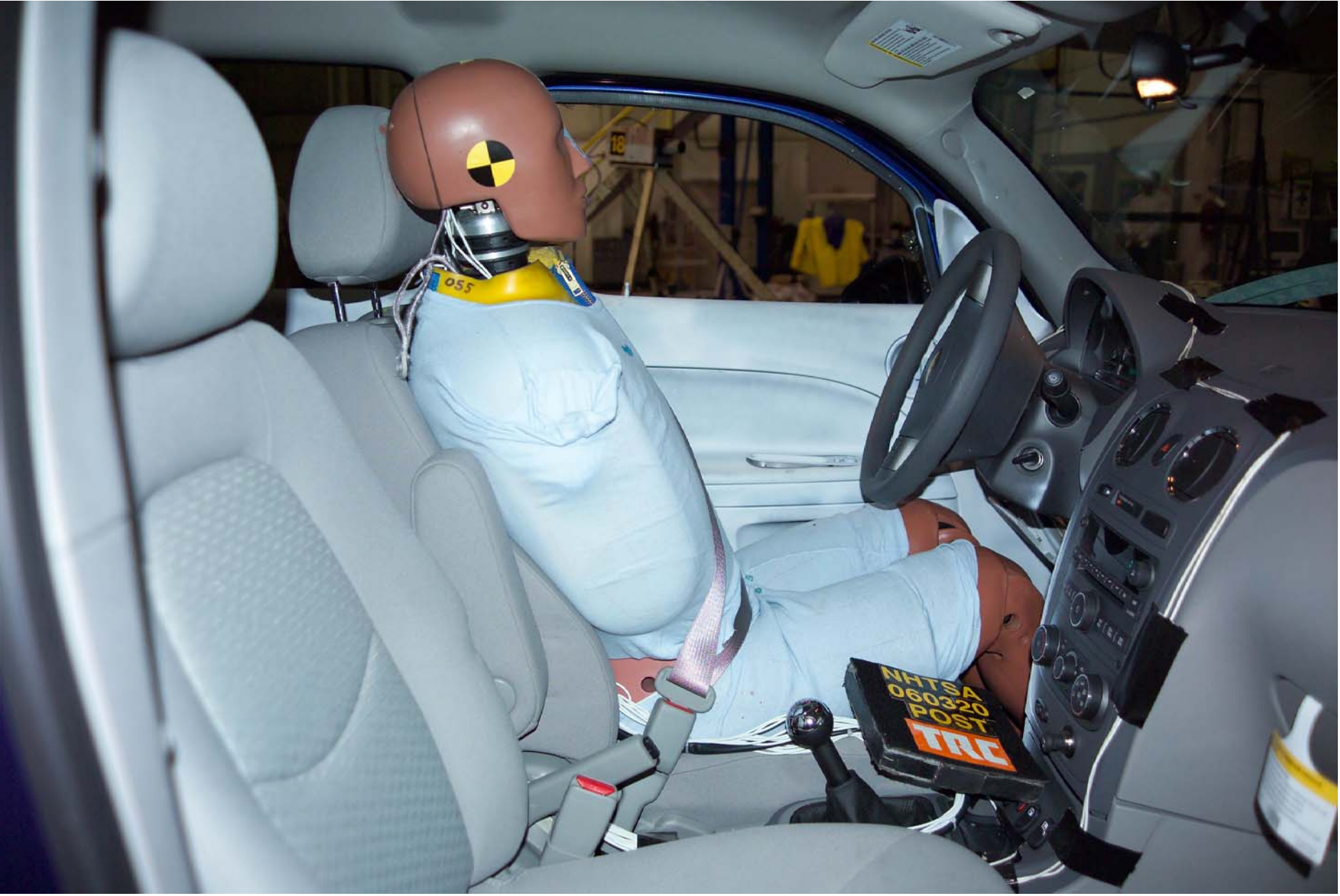
Figure A-41 Post-Test Right Occupant Compartment View of Front SID HIII A-45
