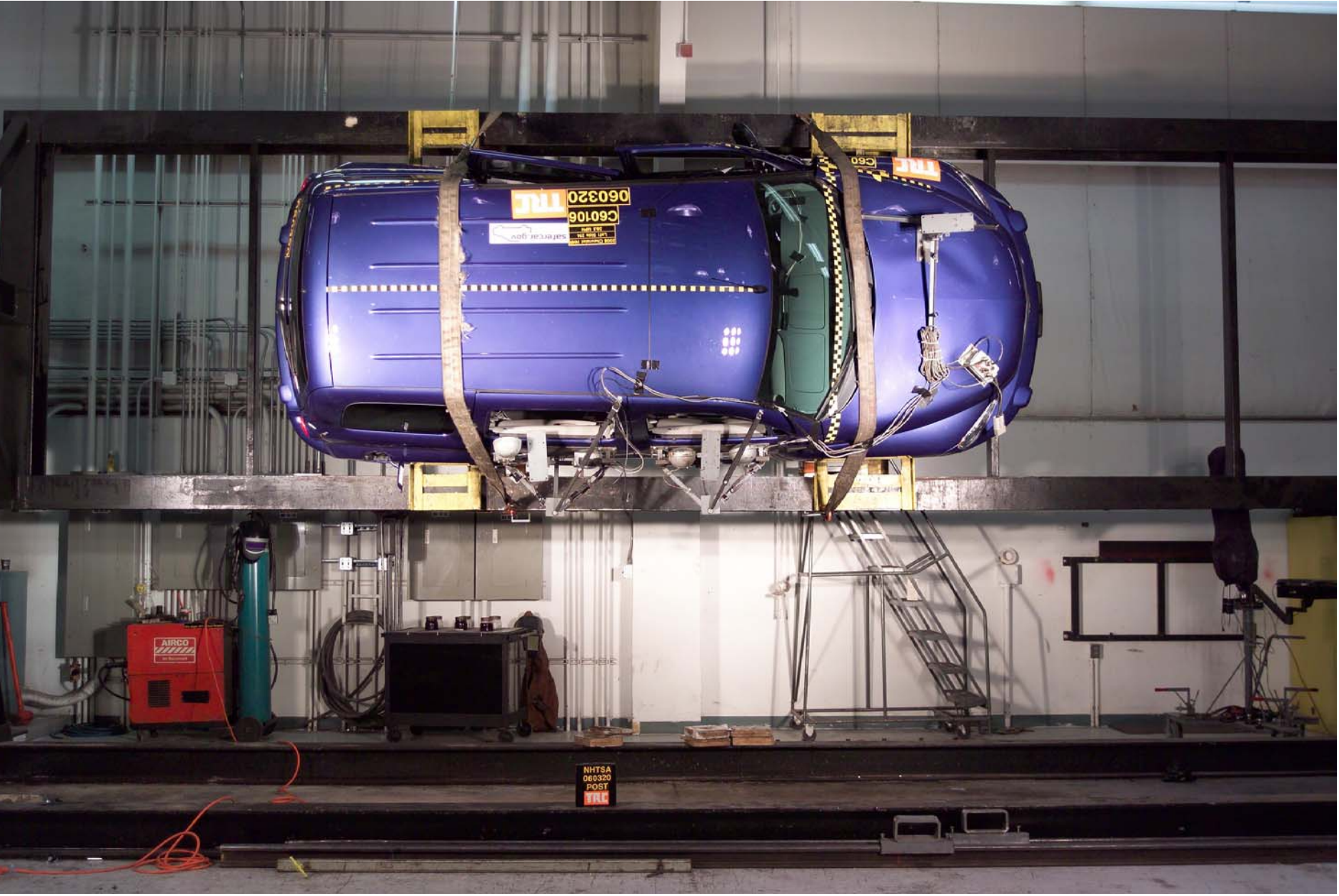
Figure A-80 FMVSS 301 Rollover View at 90°
