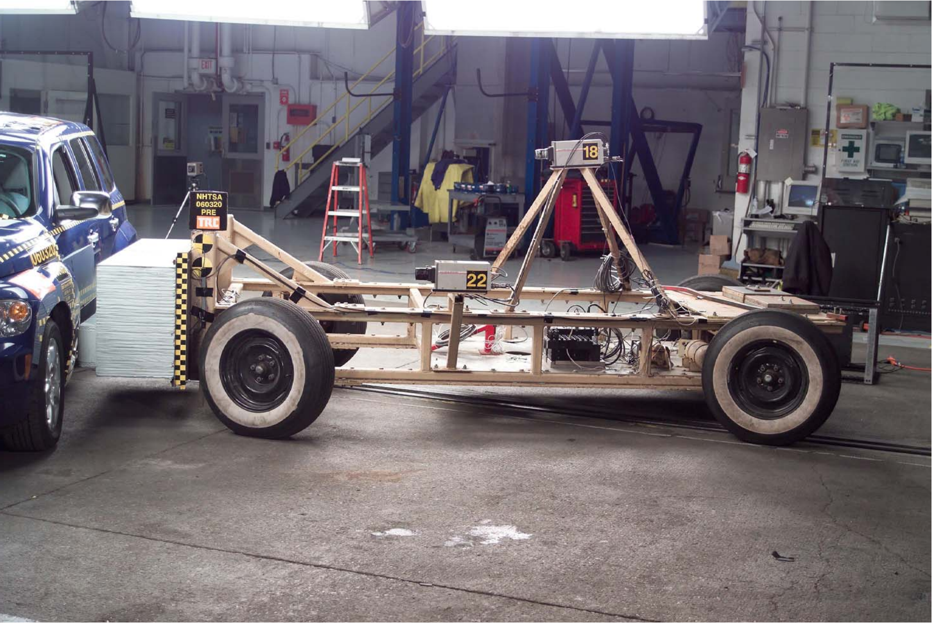
Figure A-32 Pre-Test Left Side Overall View of Impactor A-36
