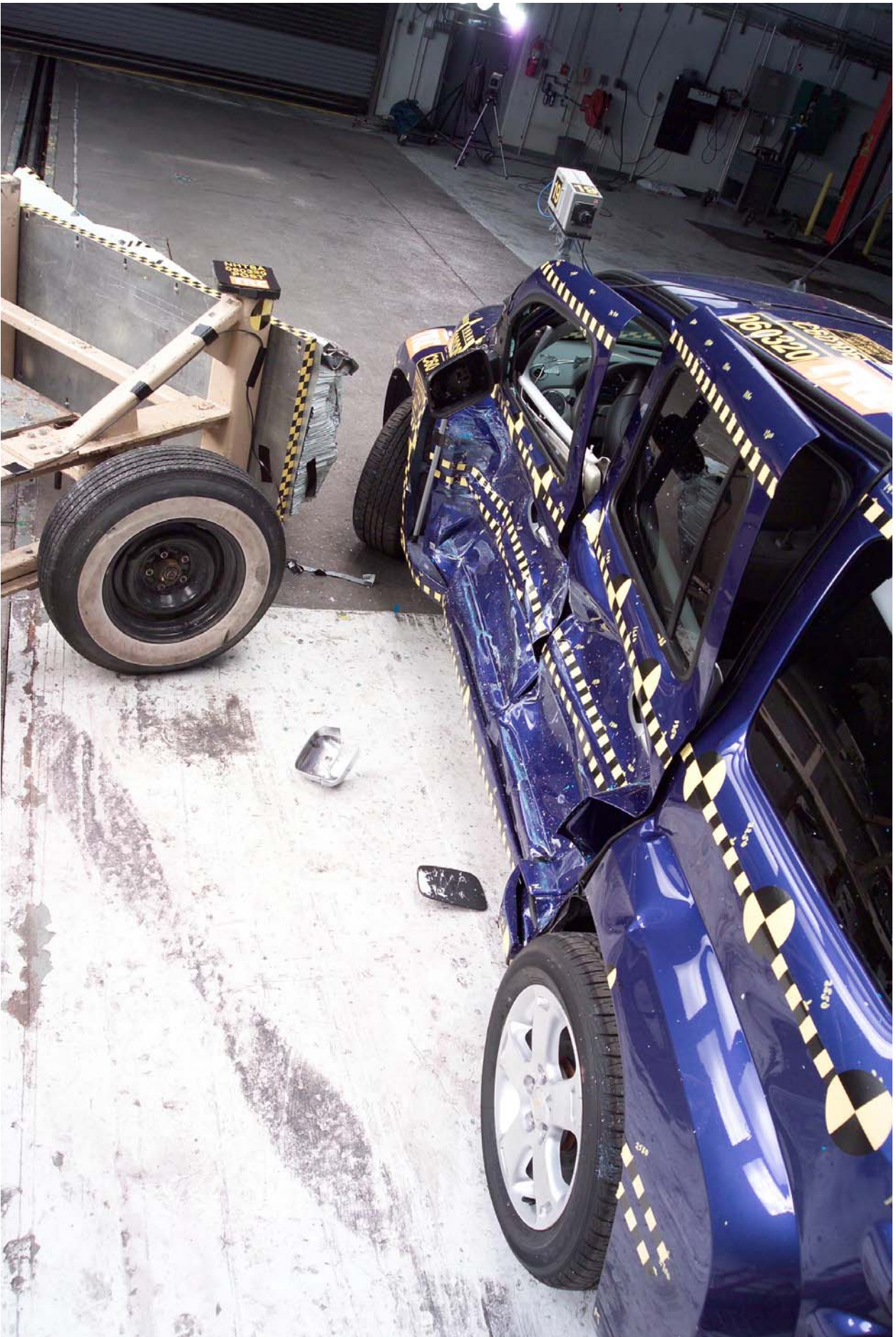
Figure A-39 Post-Test Overhead View of MDB and Vehicle
