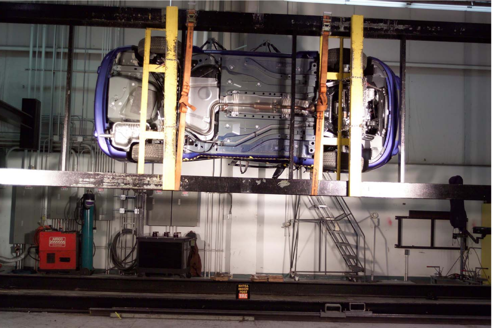
Figure A-82 FMVSS 301 Rollover View at 270°
