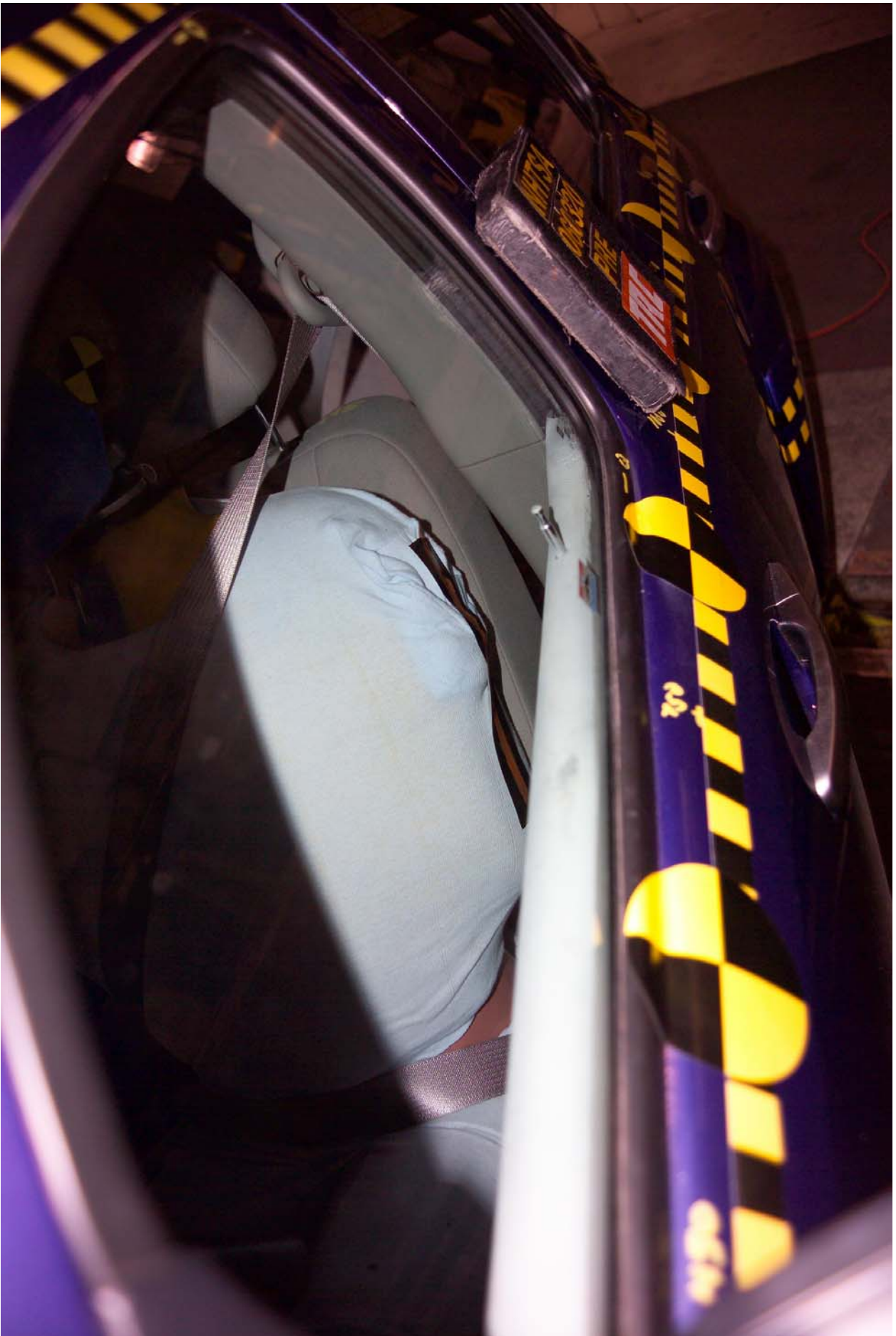
Figure A-47 Pre-Test Left View of Front SID HIII and Door Clearance
