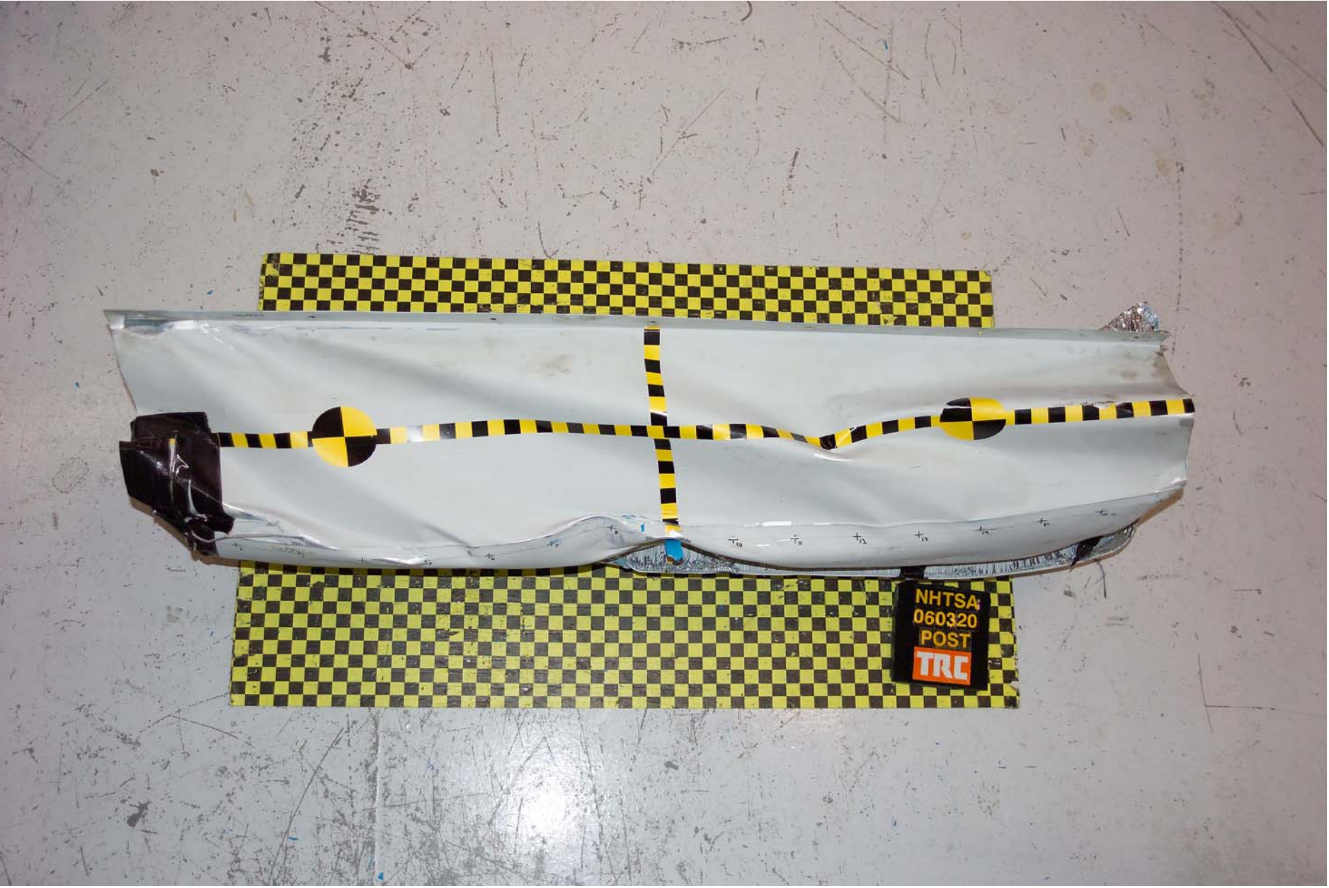
Figure A-23 Post-Test Top View of Impactor Face A-27
